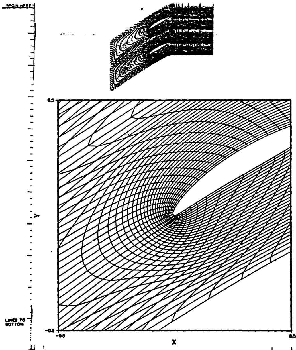
Fig. 6 Highly skewed C-grid for cascade.
