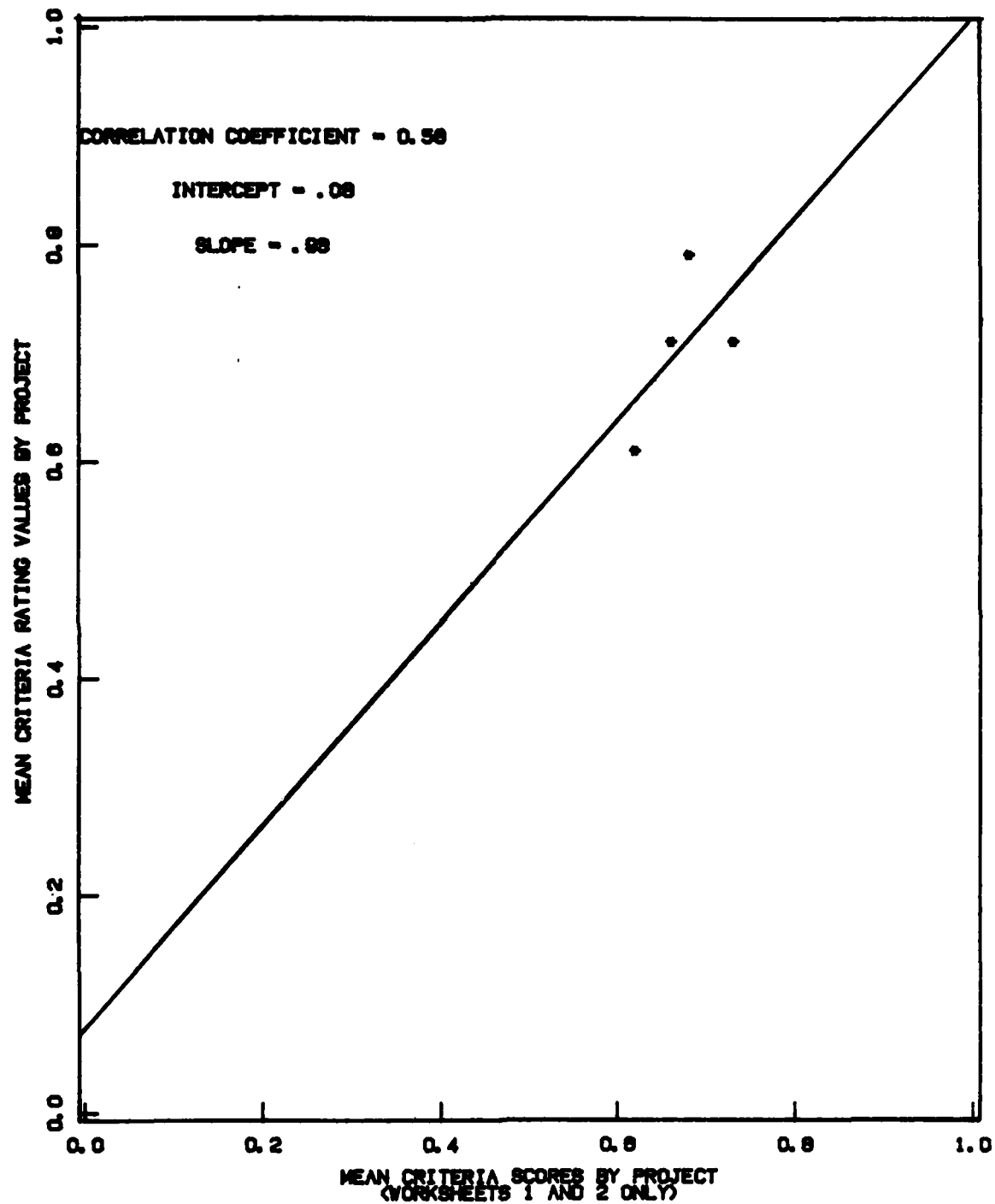
Figure 5.4.8 Survivability Mean Criteria Scores vs. Mean Criteria Rating Values
