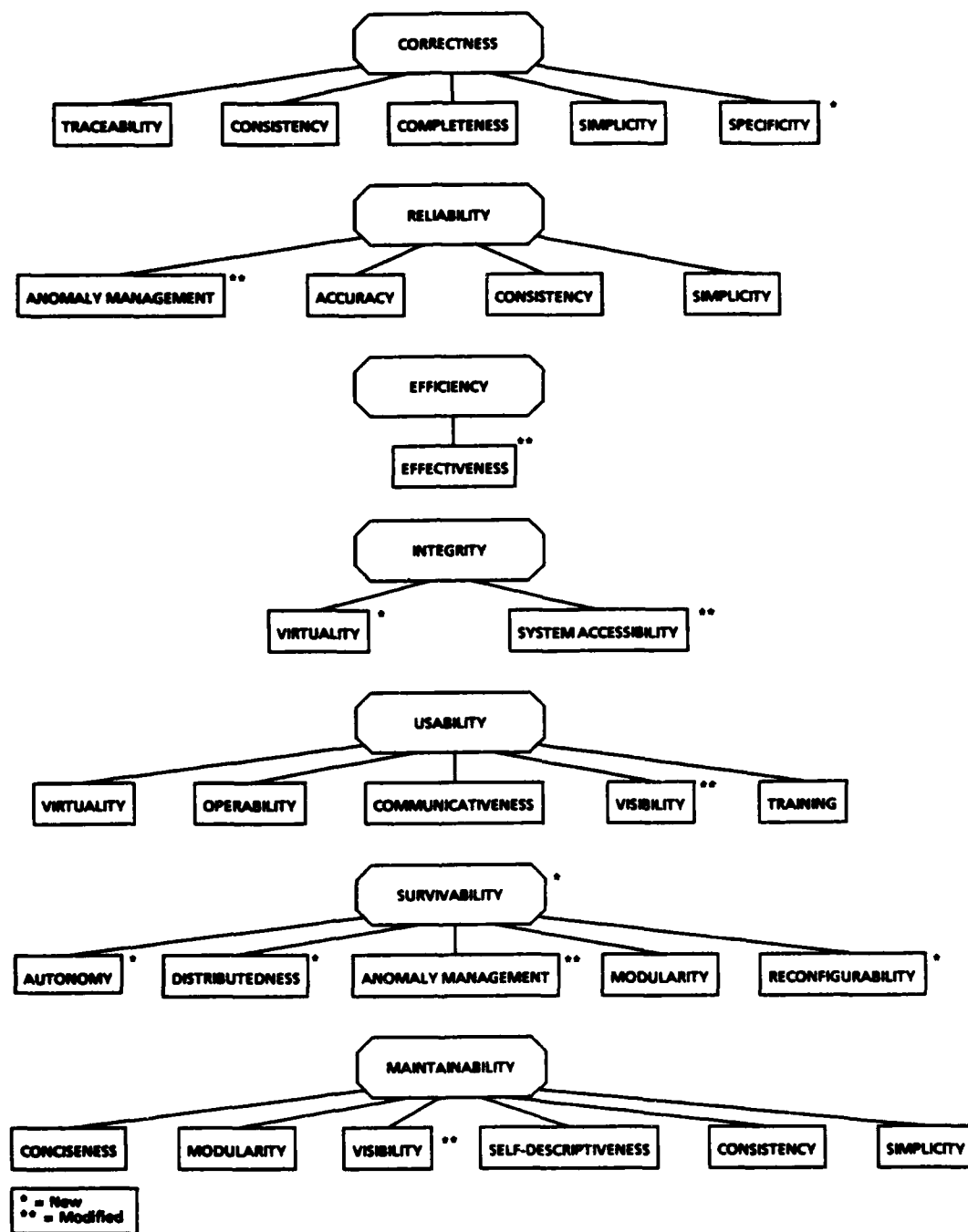
Figure 3.1-1 Relationship of Criteria to Software Quality Factors
