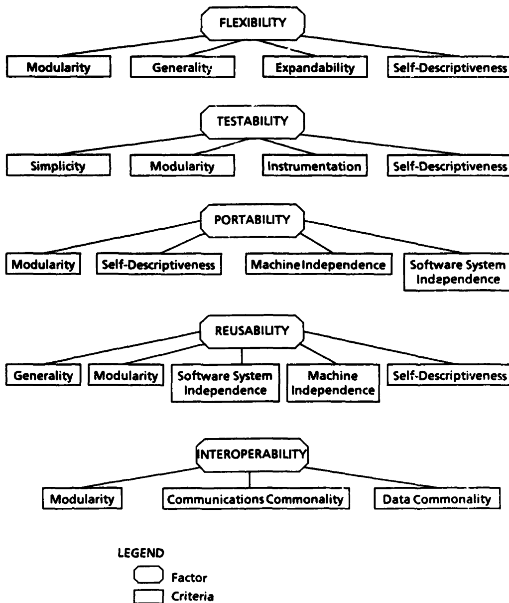
Figure 2.1-1 Relationship of Criteria to Software Quality Factors (Continued)
