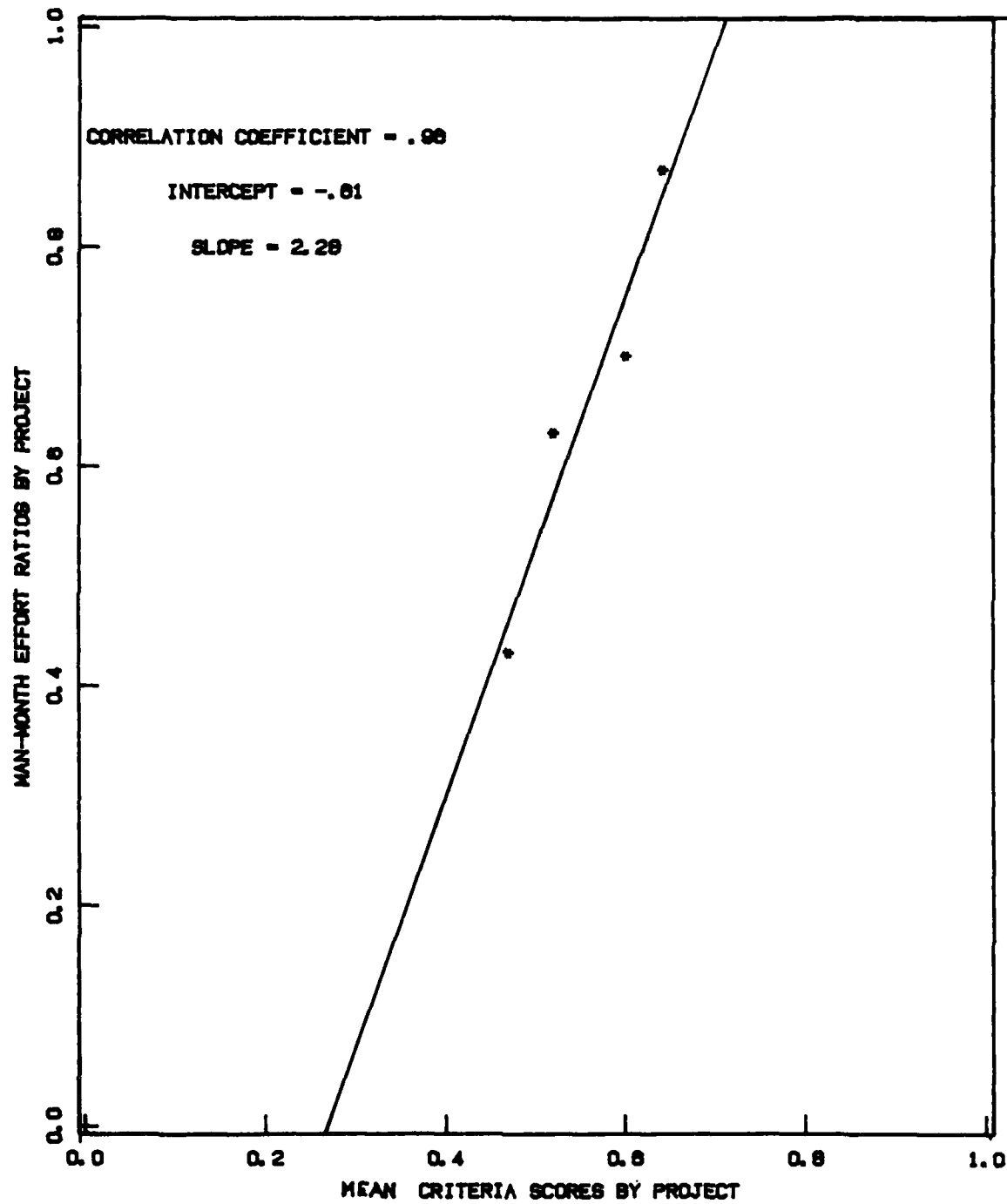
Figure 5.4-4 Expandability Mean Criteria Scores vs. Man-month Ratios
