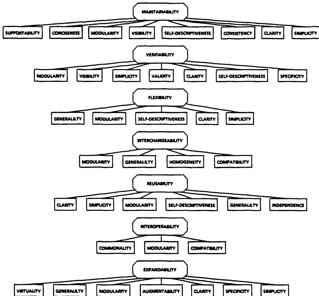
Figure 3.2-1 Relationship of Criteria to System Quality Factors (Continued)
