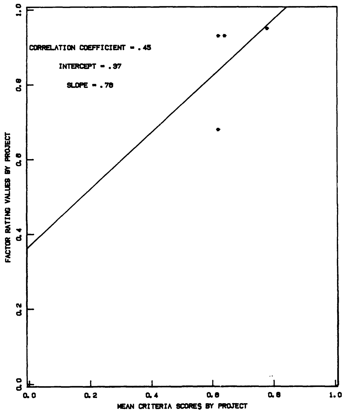
Figure 5.4-7 Survivability Mean Criteria Scores vs. Factor Rating Values
