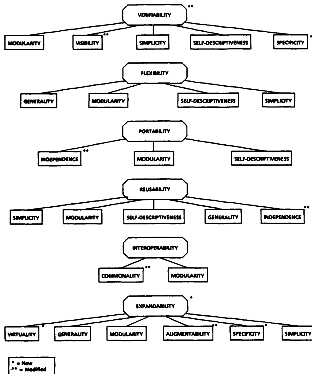
Figure 3.1-1 Relationship of Criteria to Software Quality Factors (Continued)
