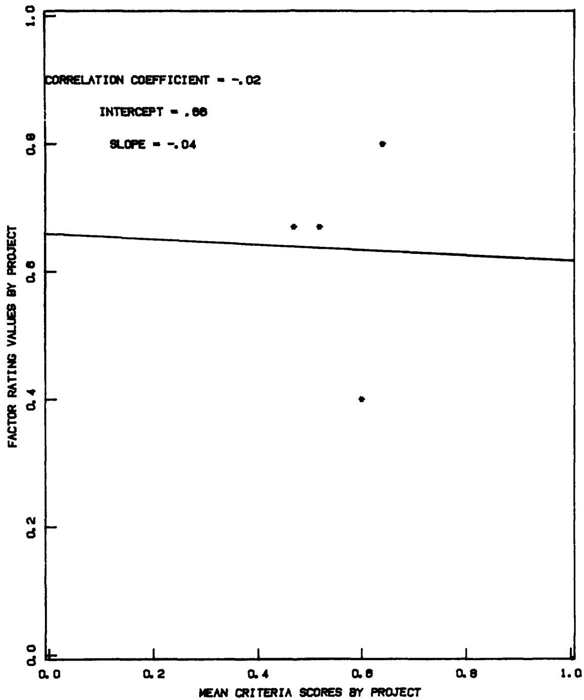
Figure 5.4-3 Expandability Mean Criteria Scores vs. Factor Rating Values
