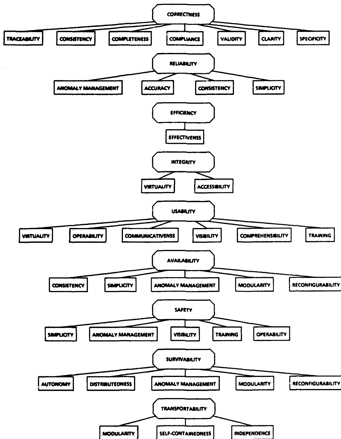
Figure 3.2-1 Relationship of Criteria to System Quality Factors
