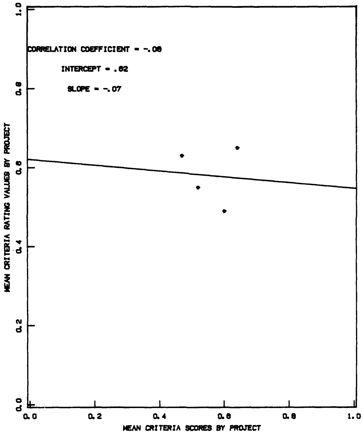
Figure 5.4-2 Expandability Mean Criteria Scores vs. Mean Criteria Rating Values
