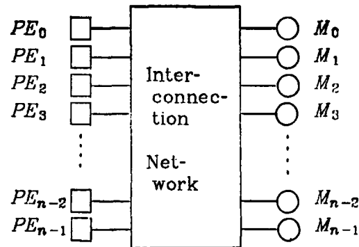
Figure 4-2. PIM machine as a model of parallel computation.
