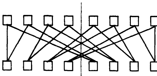
Figure C-1. The schematic perfect shuffle of n data items between two rows of n/2 processors, n = 16 .
