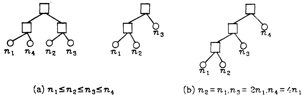
Figure 6-6. Weight-balanced trees.
