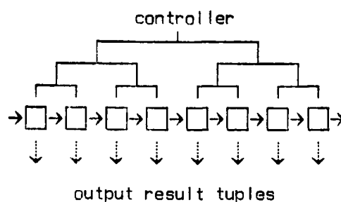
Figure 3-3. Logical structure of the easy-catch system for performing join operations.
