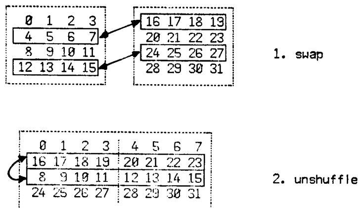
Figure 5-2. Rearrangement merge of two 4x4 regions.
