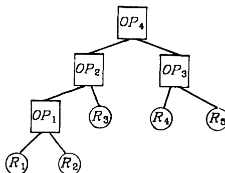
Figure 6-1. An operation tree from parsing a query.
