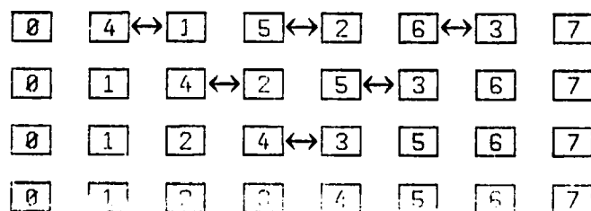
Figure 5-3. A triangular interchange scheme to perform unshuffle.
