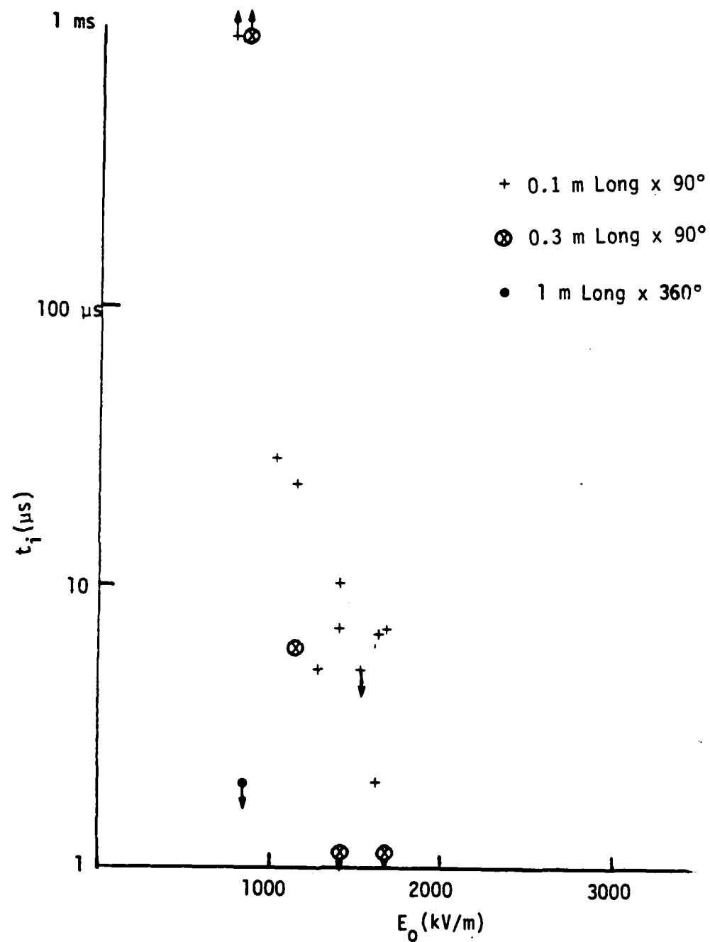
Figure 16. Time to breakdown t_i for three geometries.*
