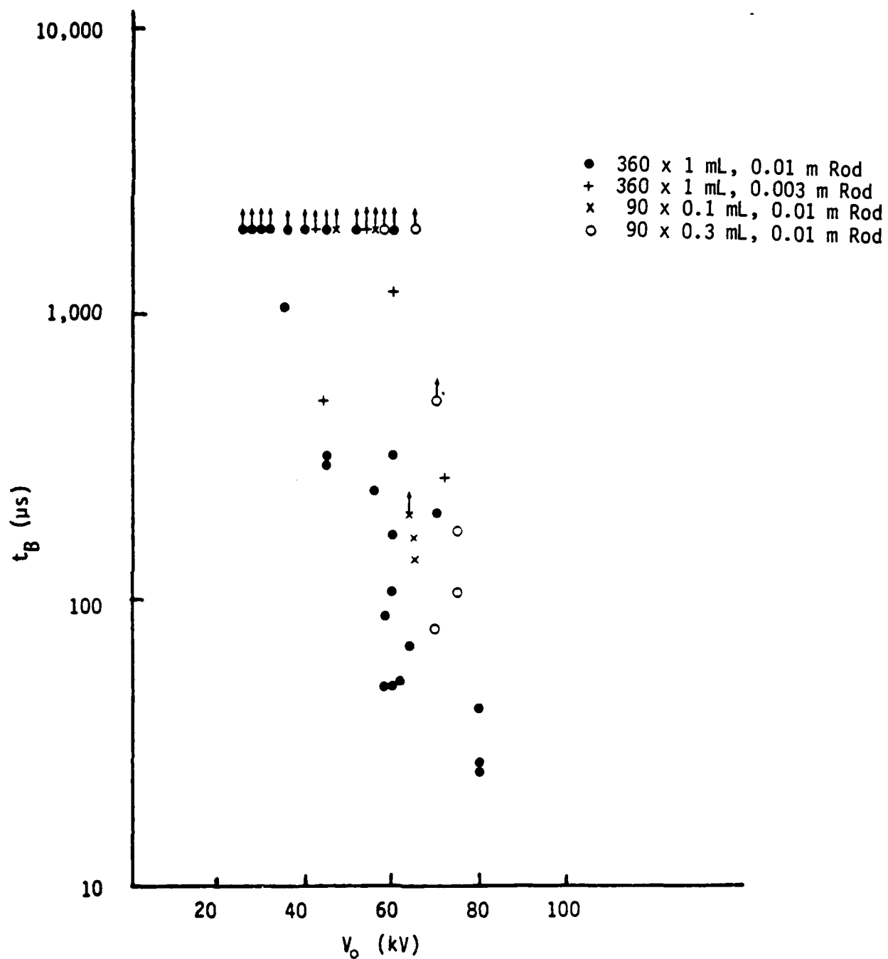
Figure 32. Time t_B for attachment to occur. x and o: corona attachment; streamer attachment.
