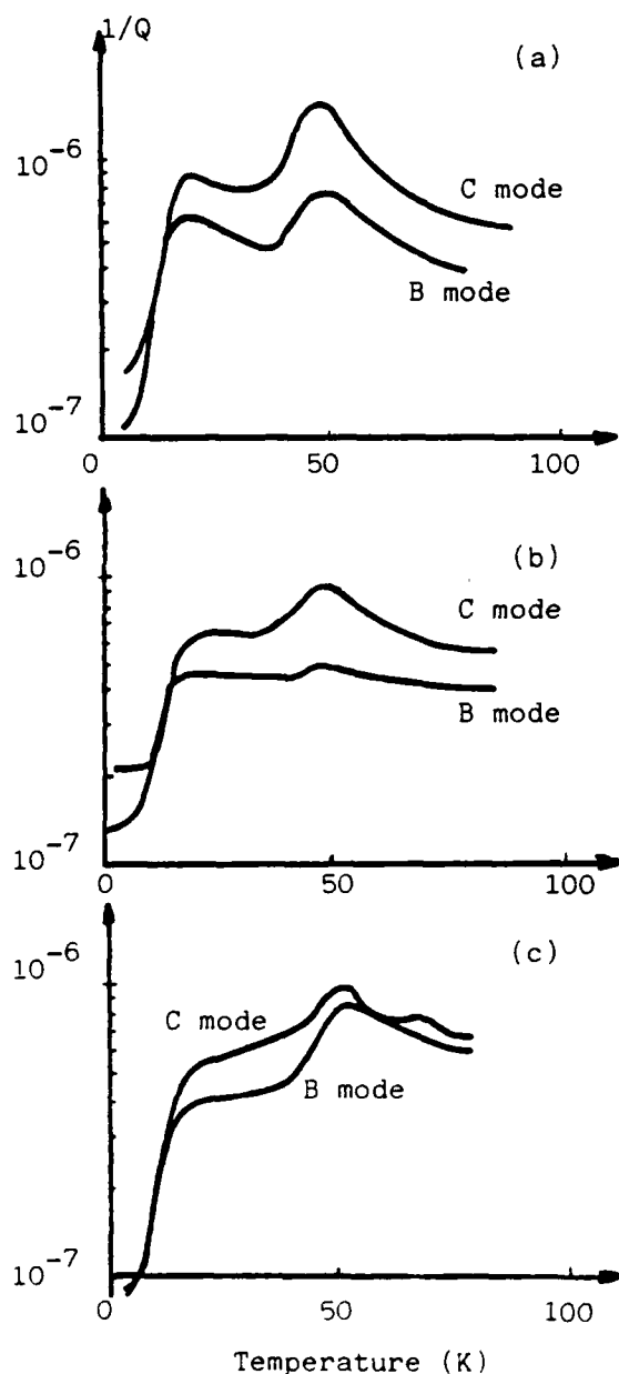
Fig. 2 Low temperature acoustic losses for the two shear modes a) FC cut 246 b) FC cut 247 c) SC cut 206
