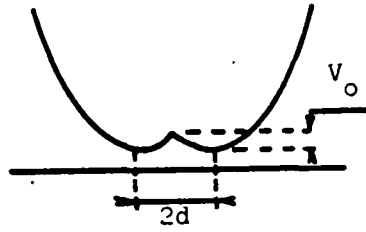
Fig. 1 Double-well potential
