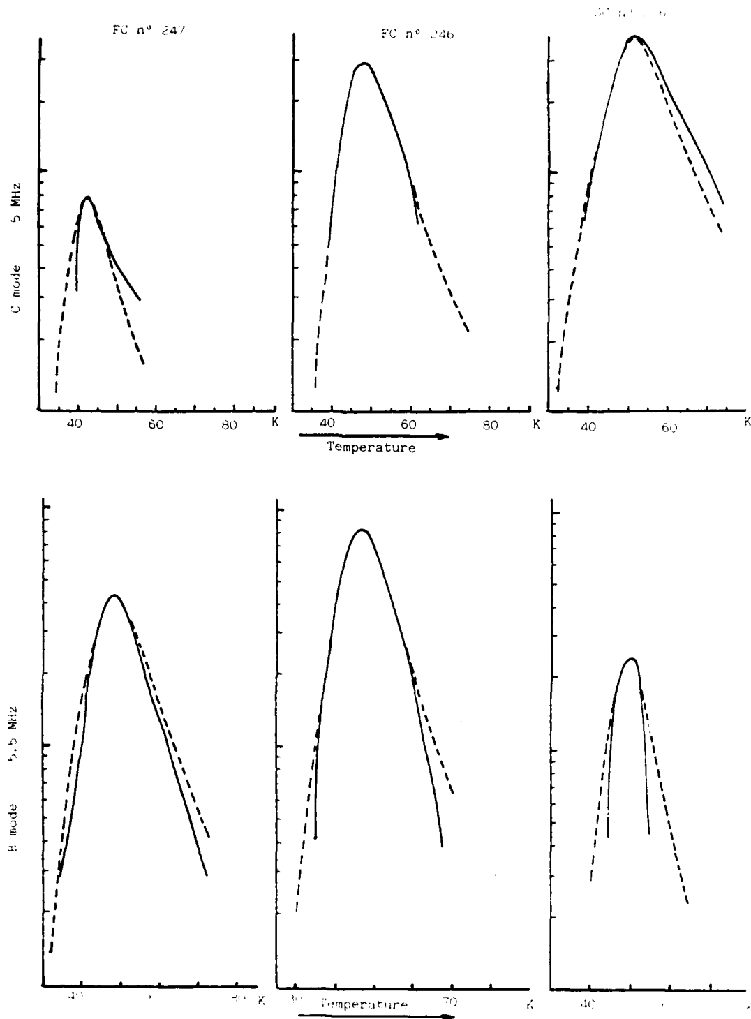
Fig. 3 Na + relaxation peaks in FC and SC-cut resonators
