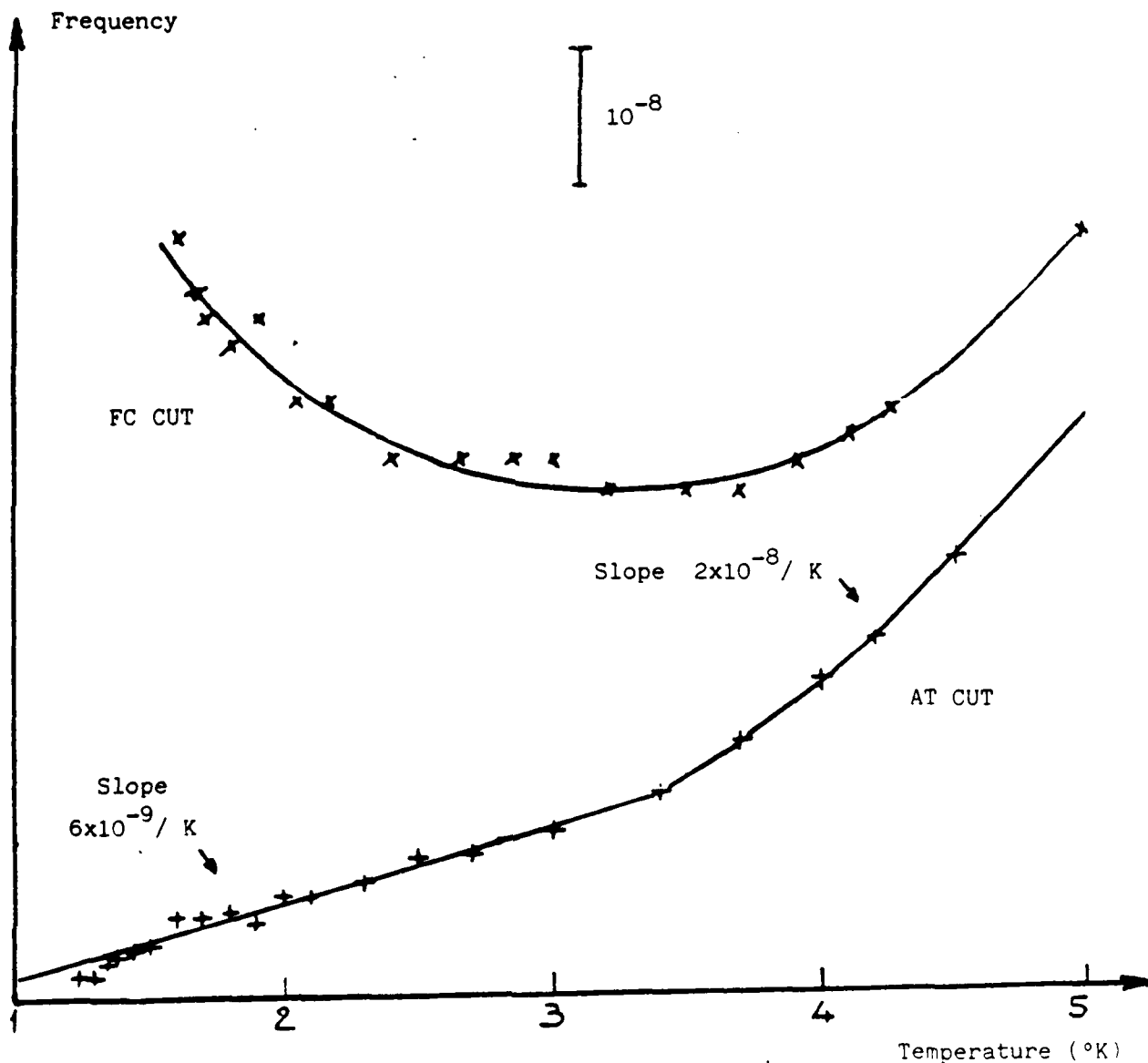
Fig. 13 Frequency vs temperature for FC and AT cut
