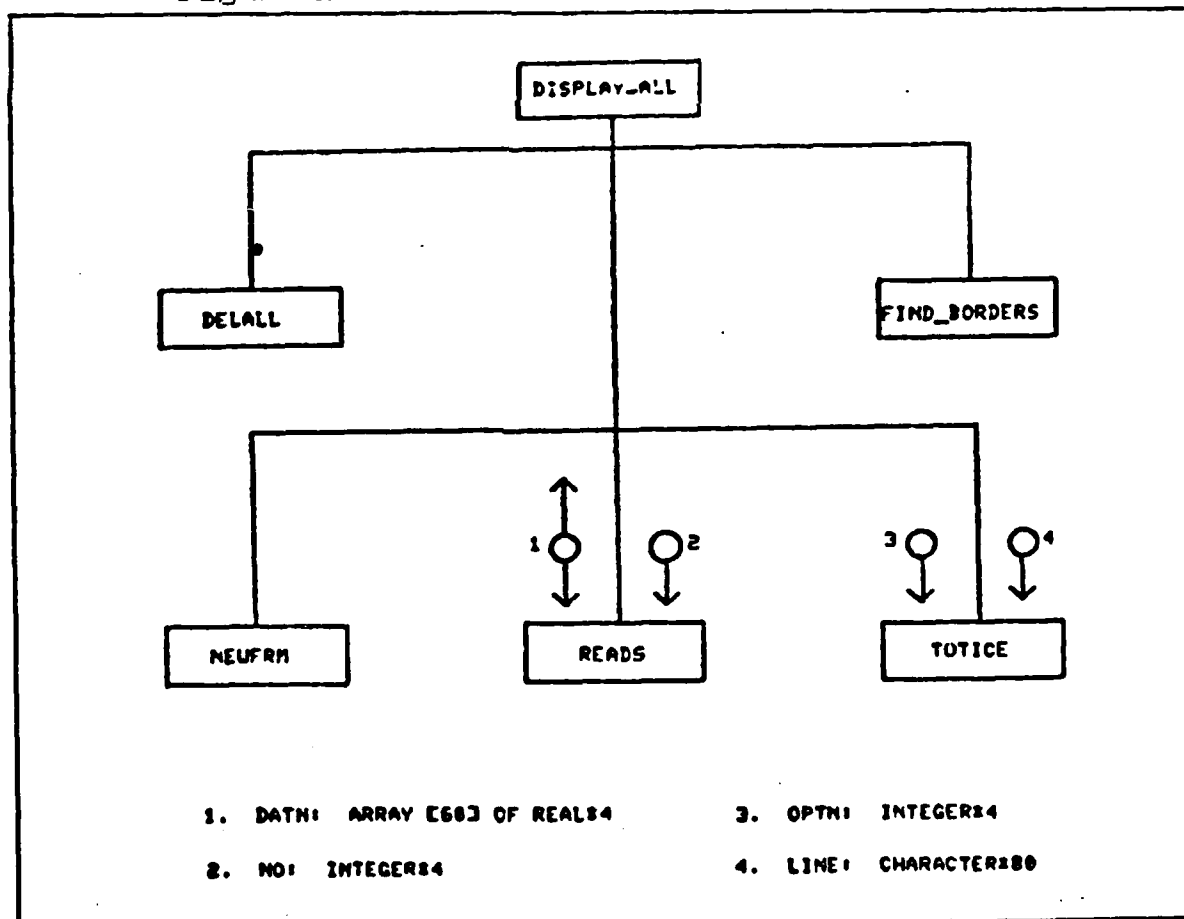
Figure A-25. Structure Chart for DISPLAY ALL
