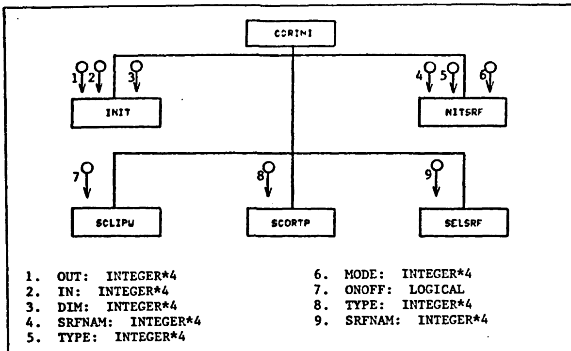
Figure A-24. Structure Chart for CORINI
