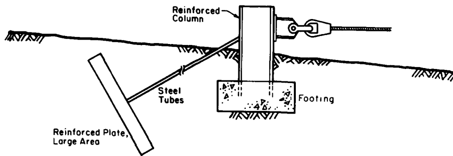
a. Deadman and pedestal (end, land).
