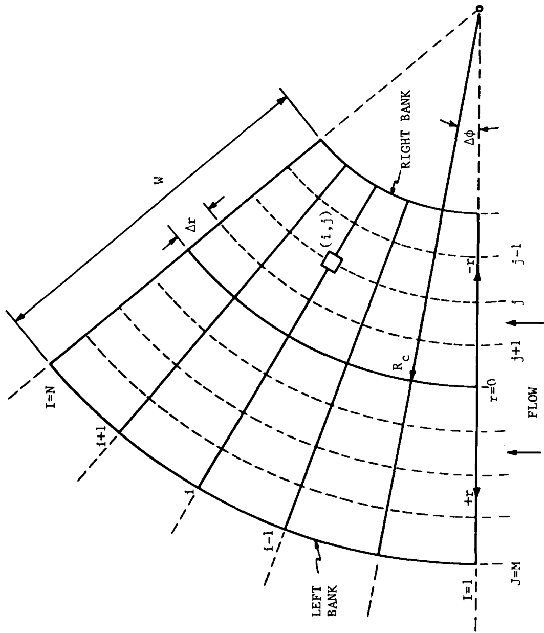
Figure 4 Coordinate-grid layout for numerical analysis
