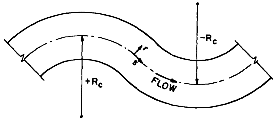
Figure 3 General coordinate system
