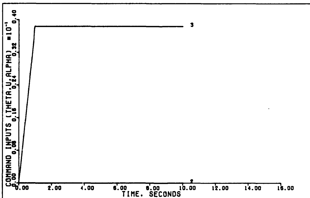
Figure 27. 0.8 g Vertical Translation (0.6 Mach)
