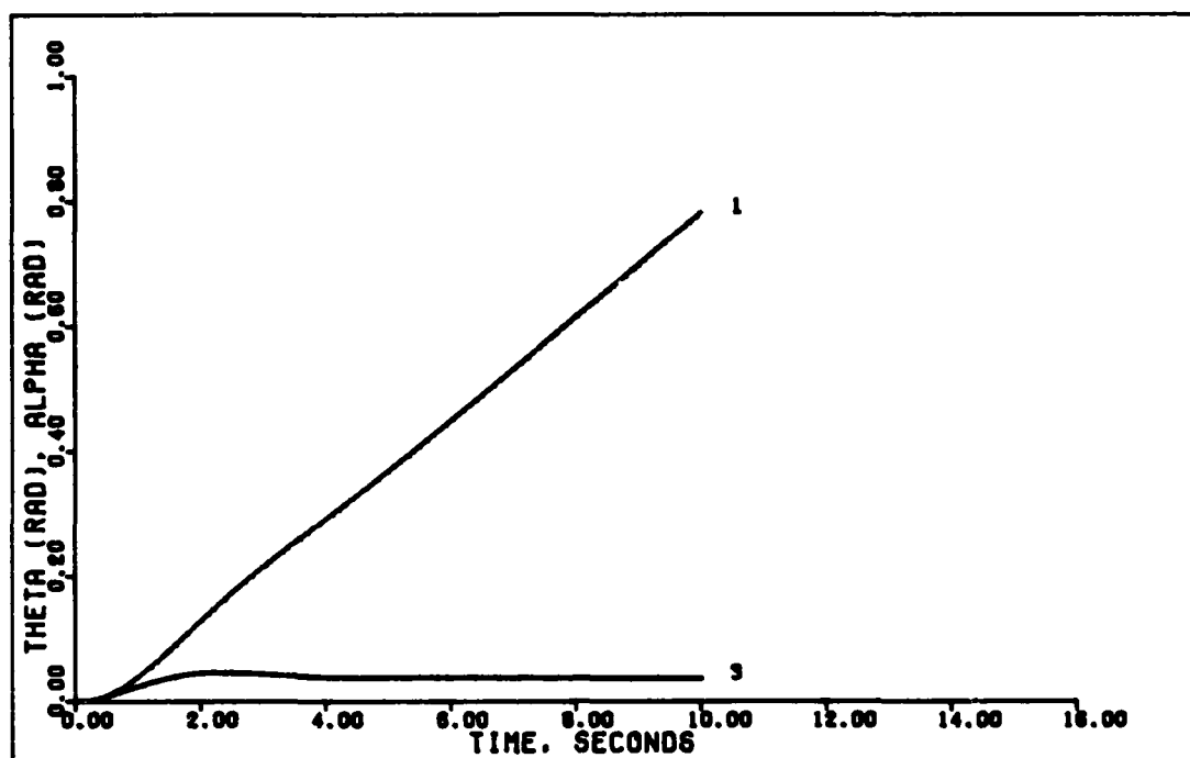
2.4 G DIRECT LIFT (0. ALPHA=4. 0.9 MACH)
