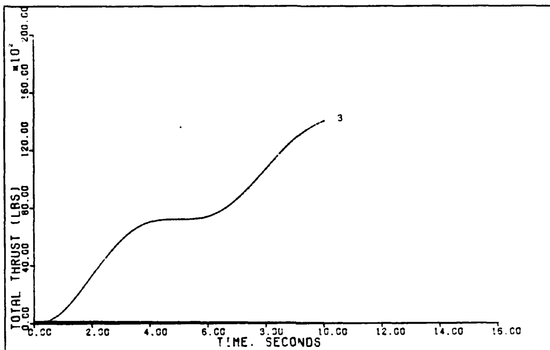
Figure 36. 2.4 g Direct Lift (0.9 Mach)
