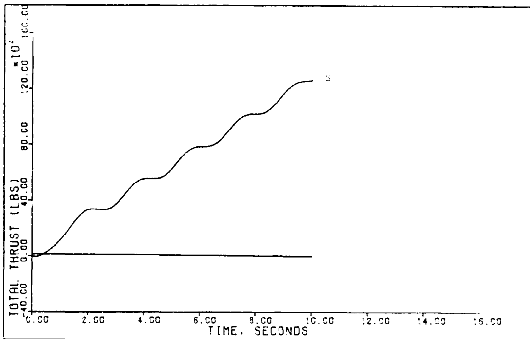
Figure 26. 1.8 g Direct Lift (0.6 Mach)
