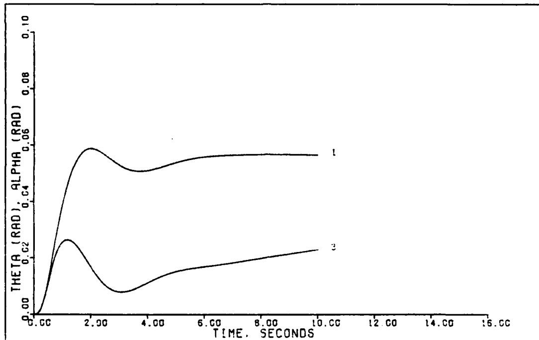
3 DEGREE PITCH POINTING (0.9 MACH, 0 FT)
