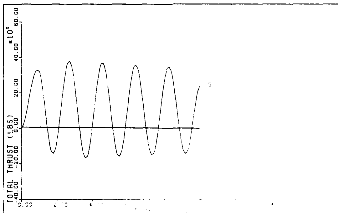
Figure 29. 0.8 g Vertical Translation (0.6 Mach)
