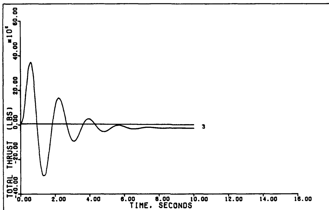
Figure 14. 1.75 Degree Pitch Pointing (0.15 Mach)
