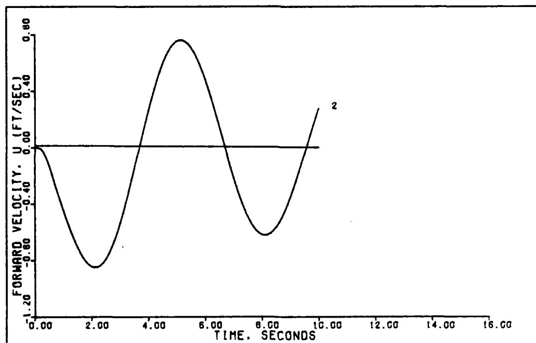
Figure 45. 1.75 Degree Pitch Pointing With Universal Controller (0.6 Mach, 0 Ft.)
