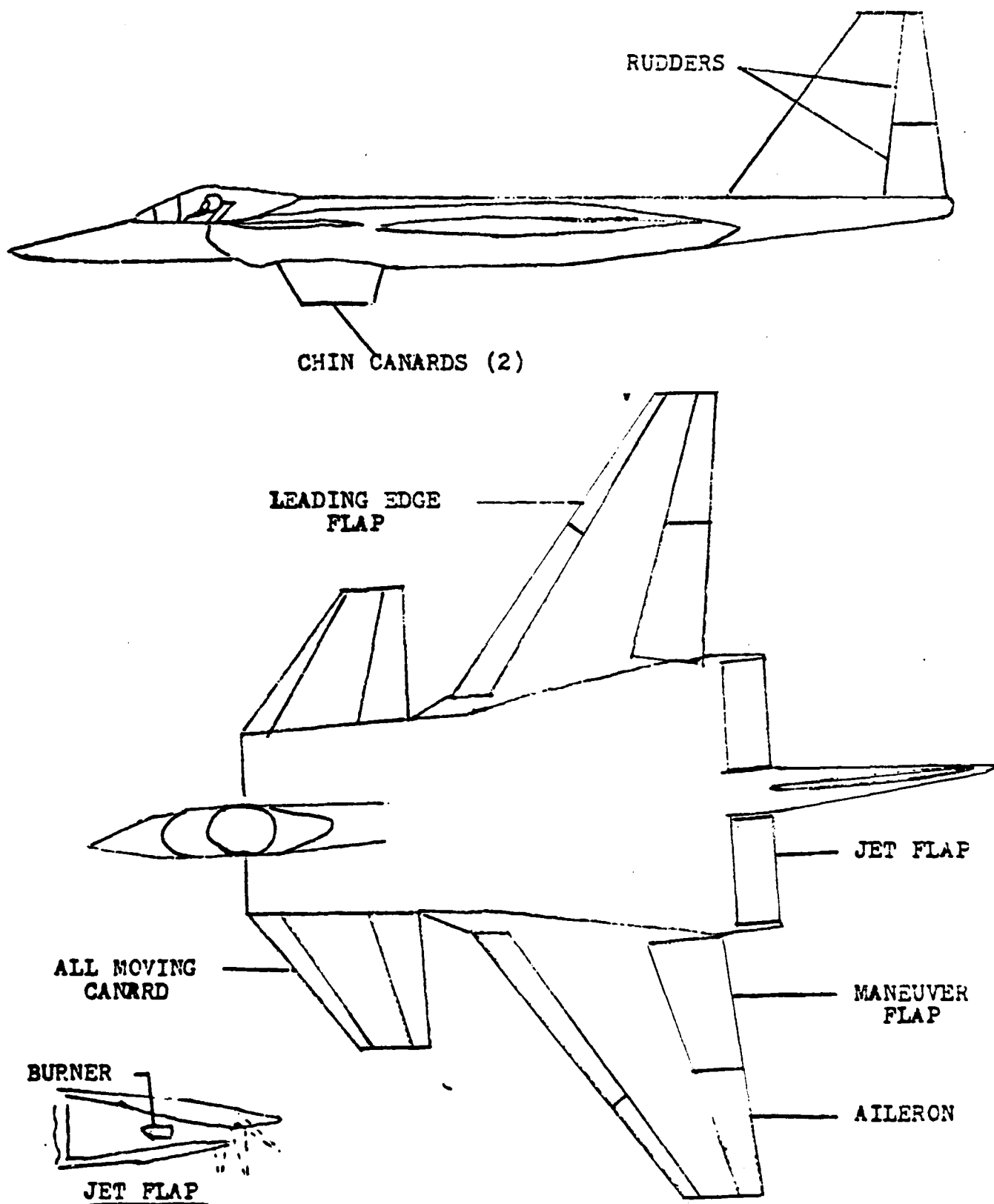
FIGURE 4. TPCC Aircraft
