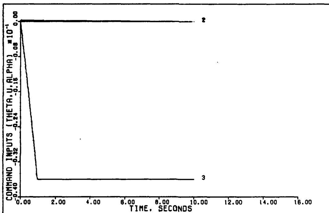
Figure 37. 1 g Vertical Translation (0.9 Mach)
