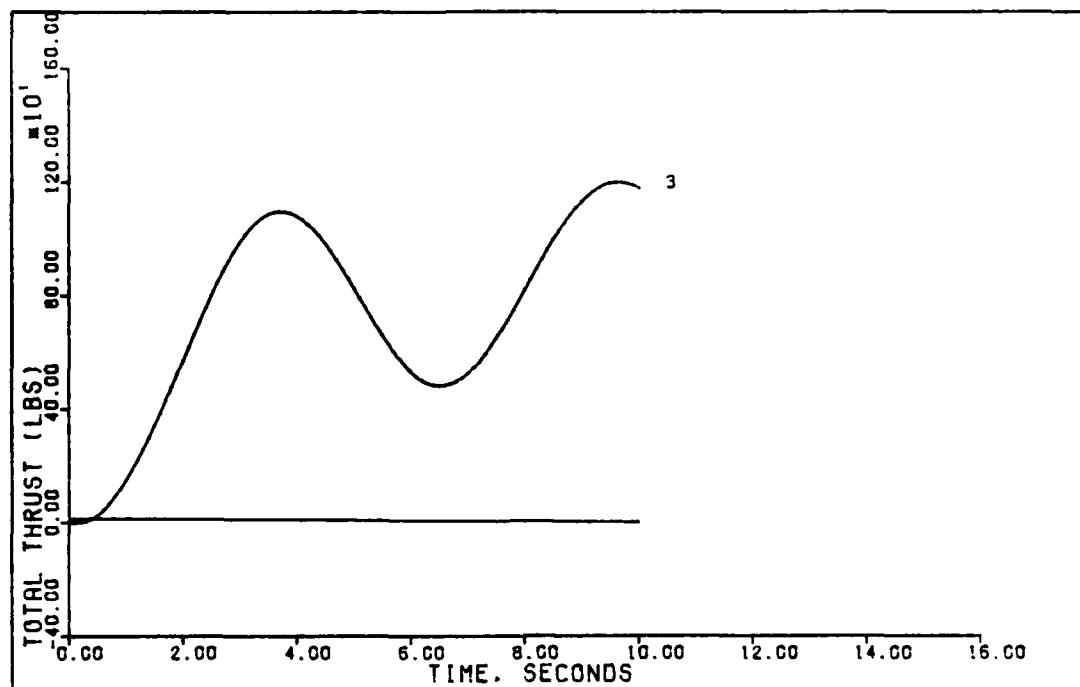
Figure 46. 1.75 Degree Pitch Pointing With Universal Controller (0.6 Mach, 0 Ft.)
