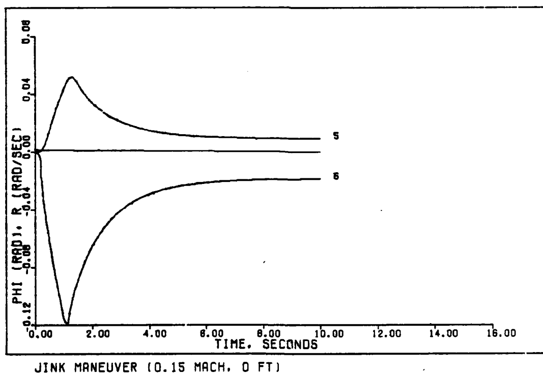
Figure 41. Jink Maneuver (0.15 Mach)
