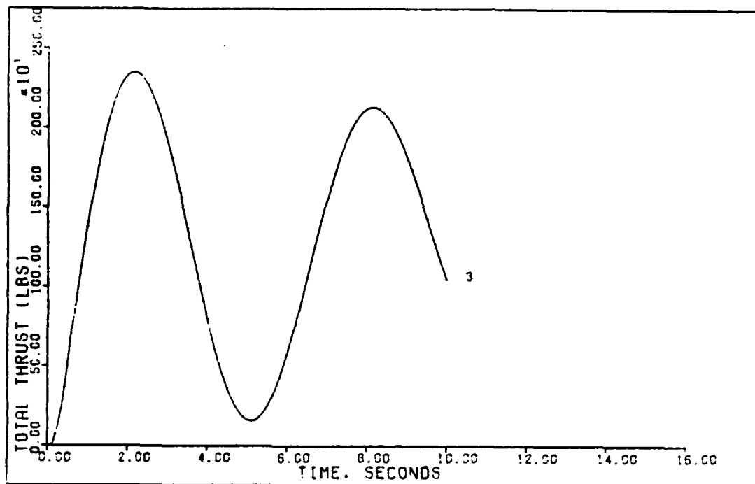
Figure 32. 3 Degree Pitch Pointing (0.9 Mach)
