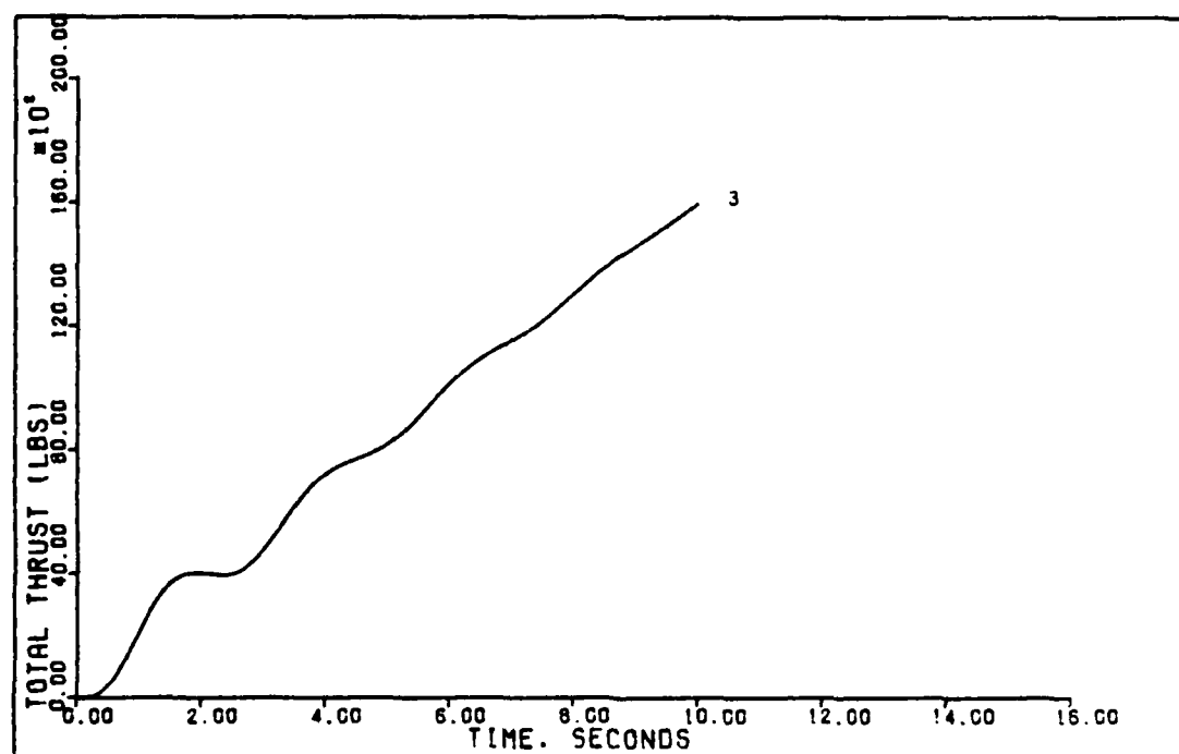
Figure 58. 0.5 G Direct Lift With Delay (0.15 Mach, 0 Ft.)
