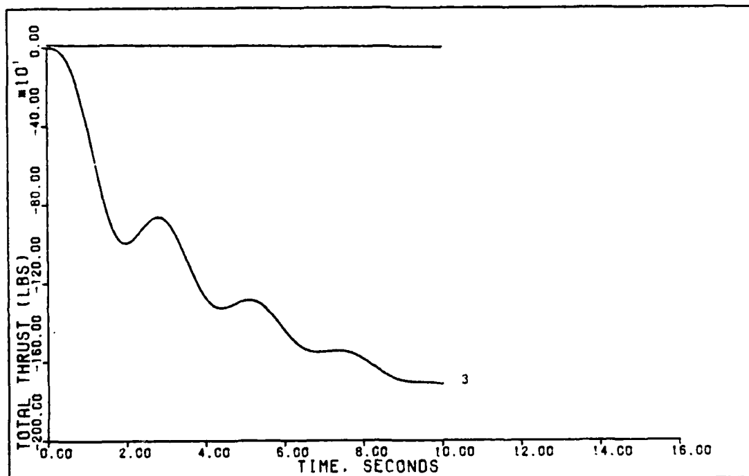
Figure 61. 0.5 G Vertical Translation With Delay (0.15 Mach, 0 Ft.)
