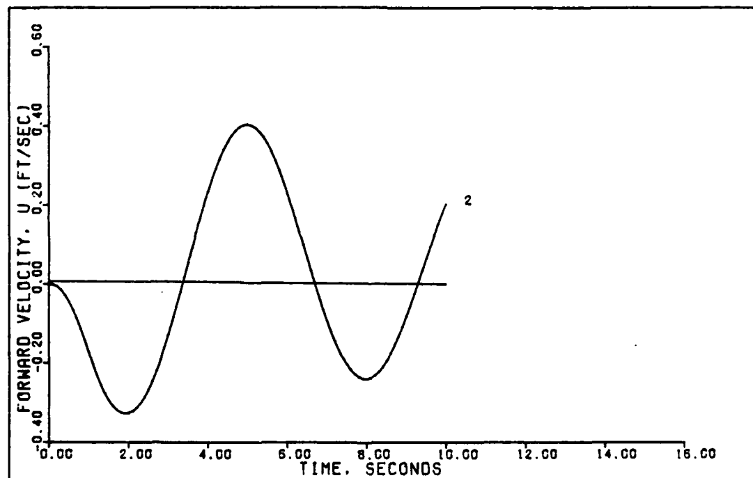
Figure 51. 0.8 G Vertical Translation With Universal Controller (0.6 Mach, 0 Ft.)
