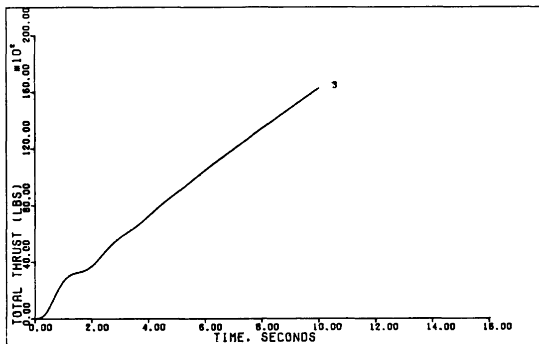
Figure 97. 0.5 G Direct Lift With Reduced Controller Matrices (0.15 Mach, 0 ft.)
