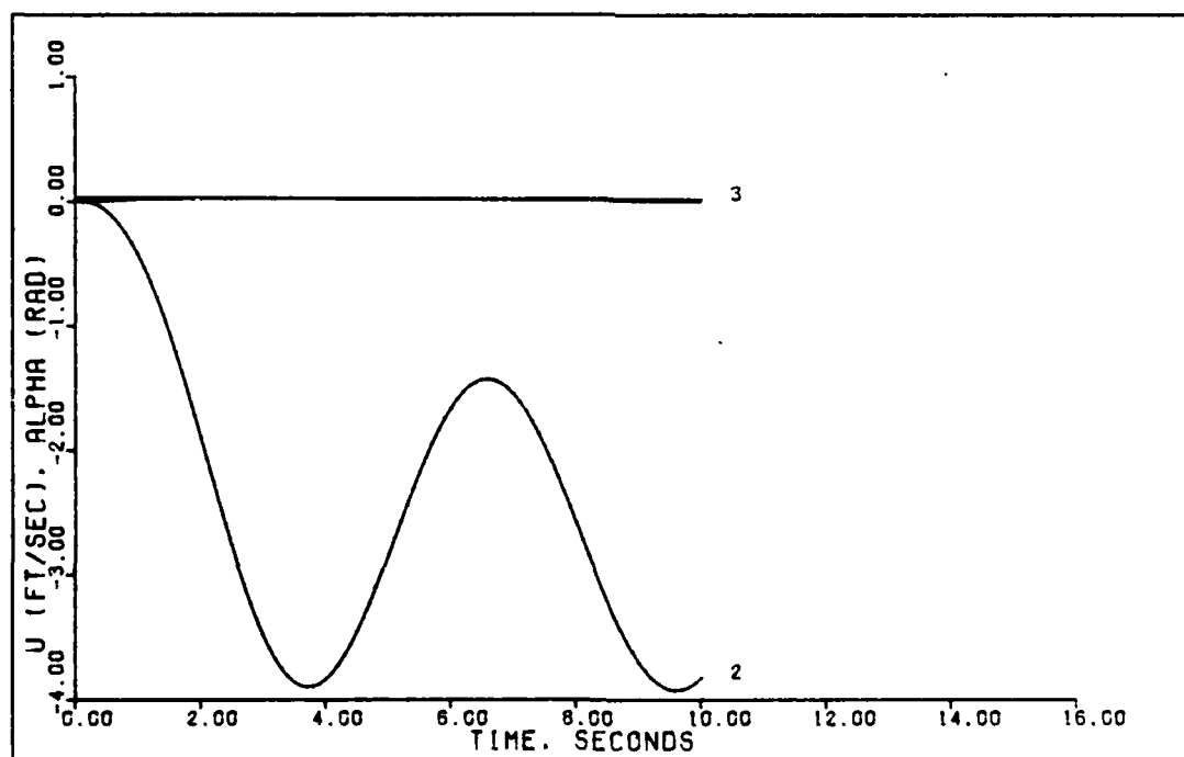
Figure 48. 1.8 G Direct Lift With Universal Controller (0.6 Mach, 0 Ft.)
