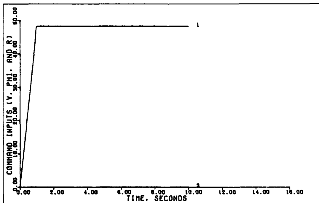
Figure 5. 1.5 g Horizontal Translation (0.15 Mach)
