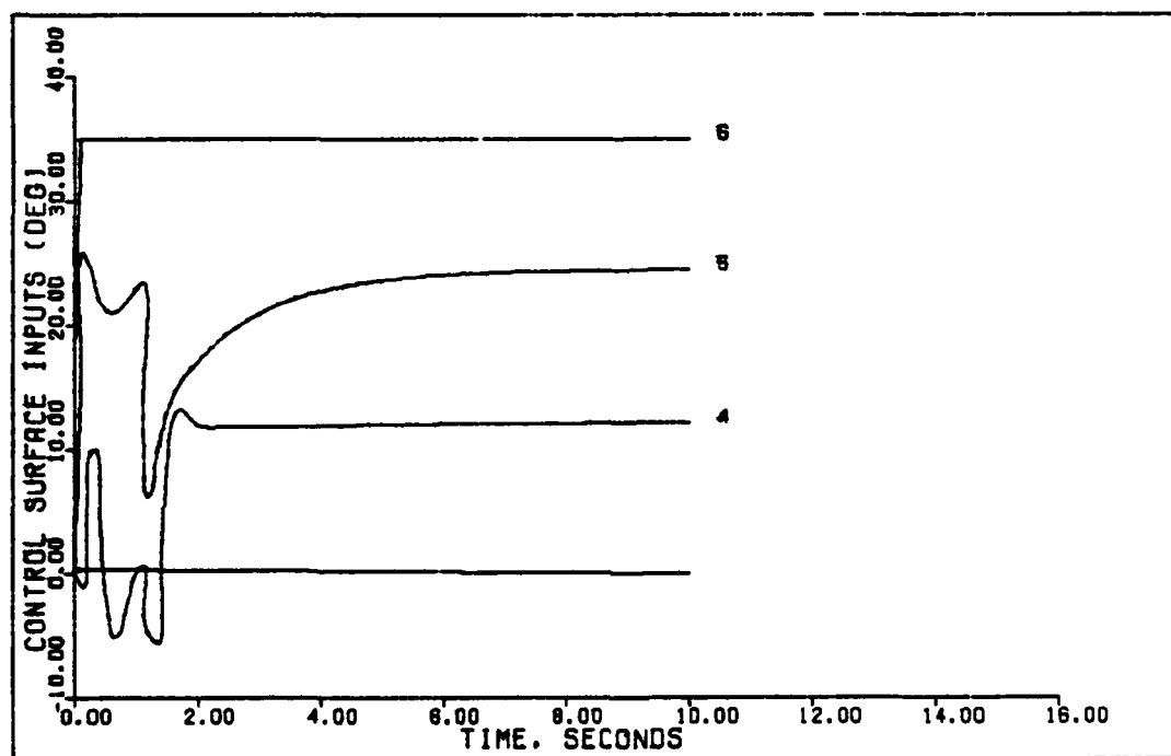
Figure 43. Jink Maneuver (0.15 Mach, 0 ft.)
