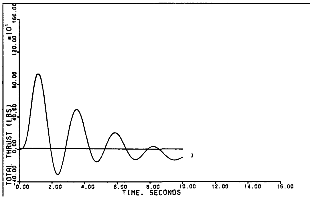
Figure 55. 1.75 Degree Pitch Pointing With Delay (0.15 Mach, 0 Ft.)
