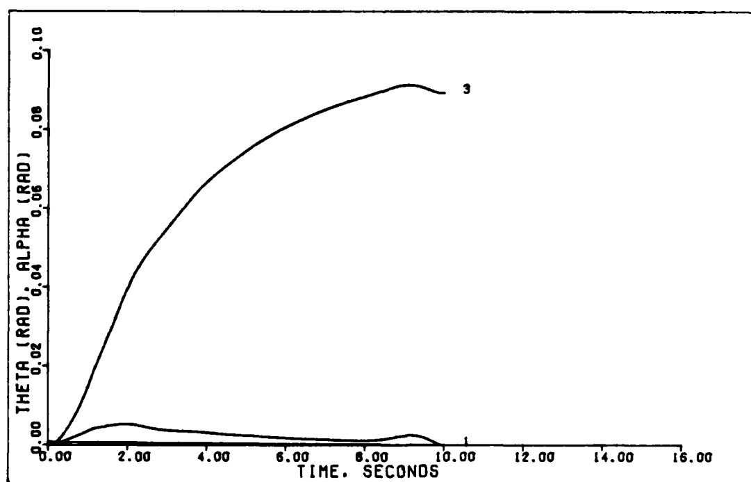
Figure 98. 0.5 G Vertical Translation With Reduced Controller Matrices (0.15 Mach, 0 ft.)
