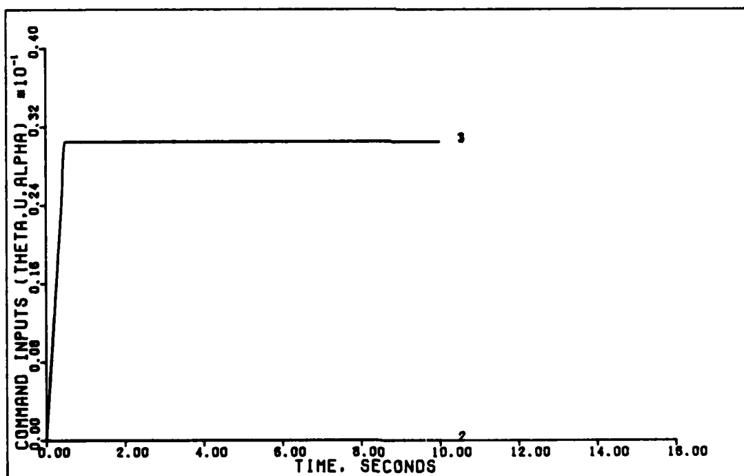
Figure 21. 1.75 Degree Pitch Pointing (0.6 Mach)
