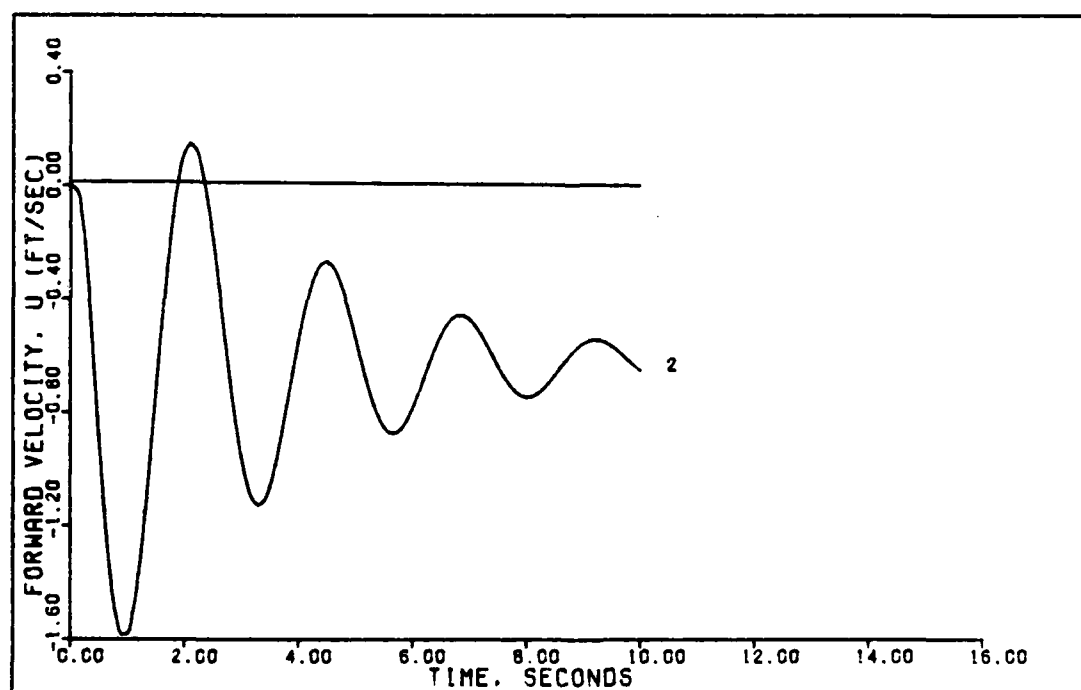
Figure 57. 0.5 G Direct Lift With Delay (0.15 Mach, 0 Ft.)
