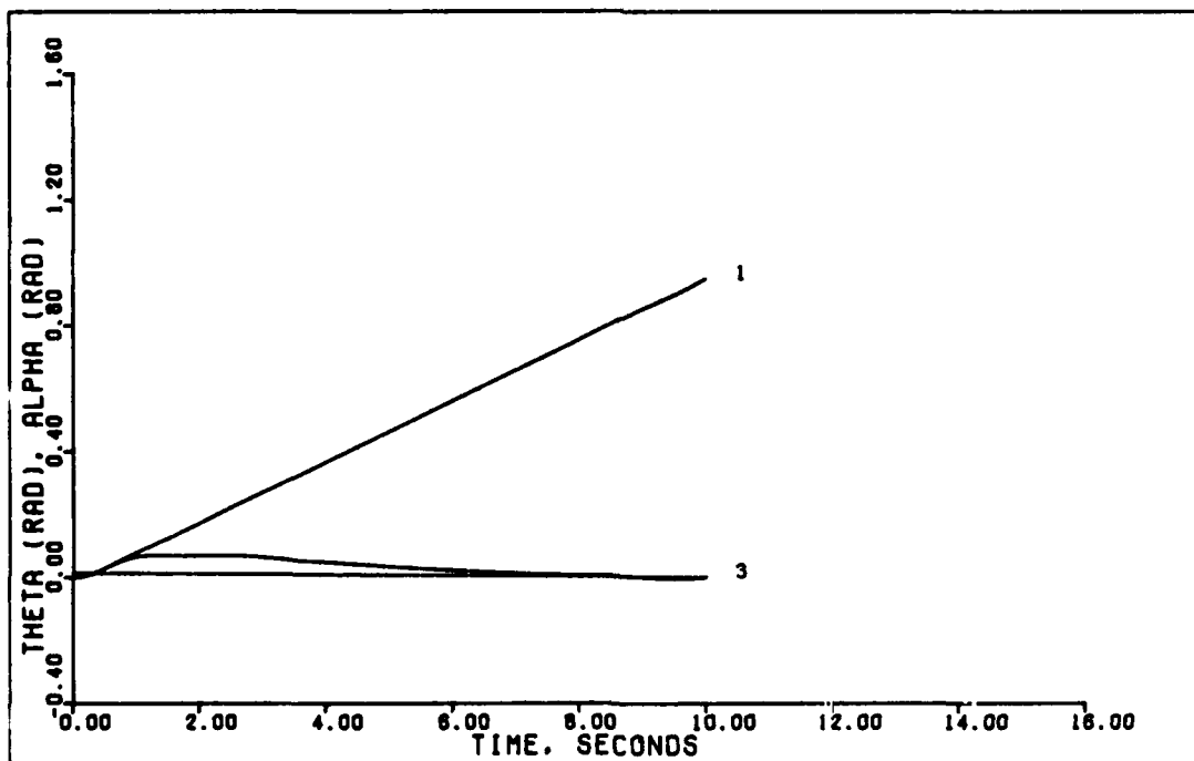
Figure 16. 0.5 g Direct Lift (0.15 Mach)
