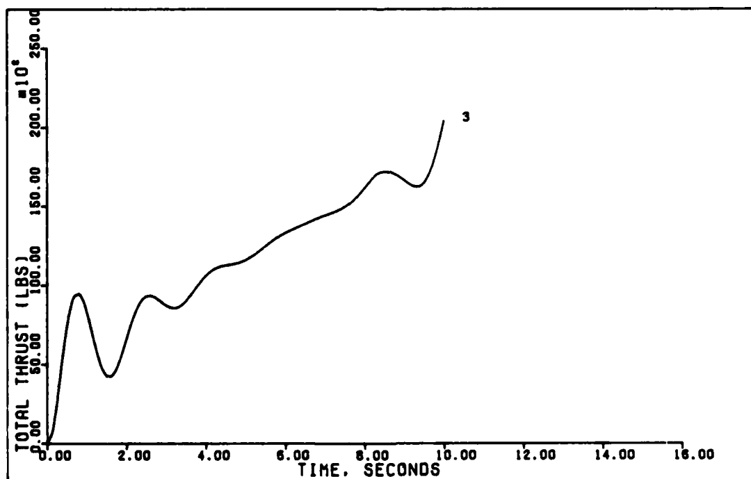
Figure 17. 0.5 g Direct Lift (0.15 Mach)
