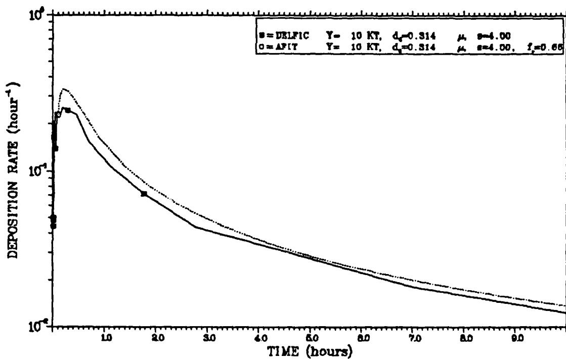
Figure C-13 Deposition Rates for the LYSTND Distribution
