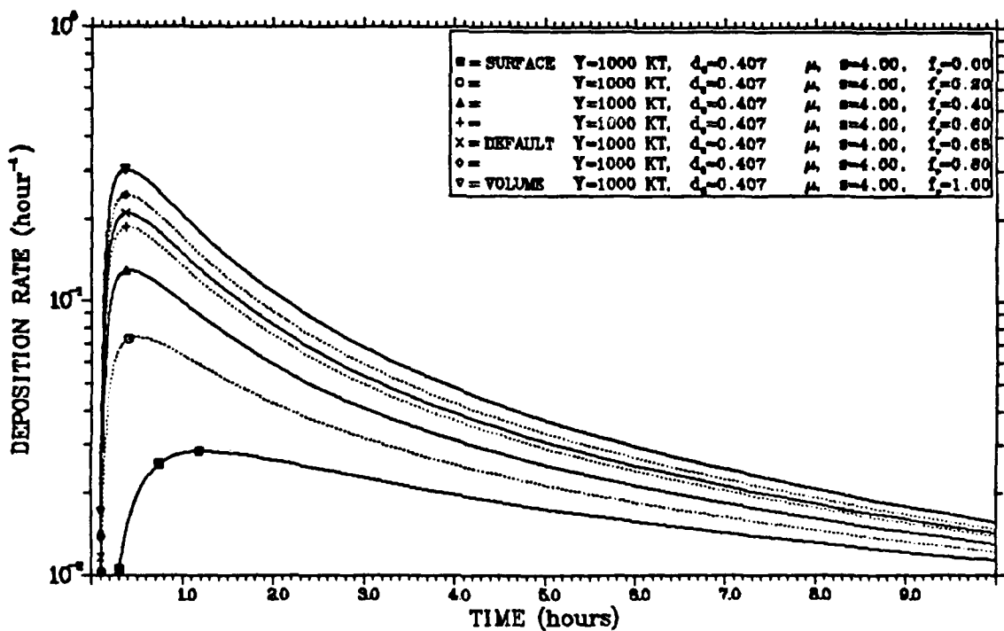
Figure V-2 Deposition Rate Sensitivity to Fractionation
