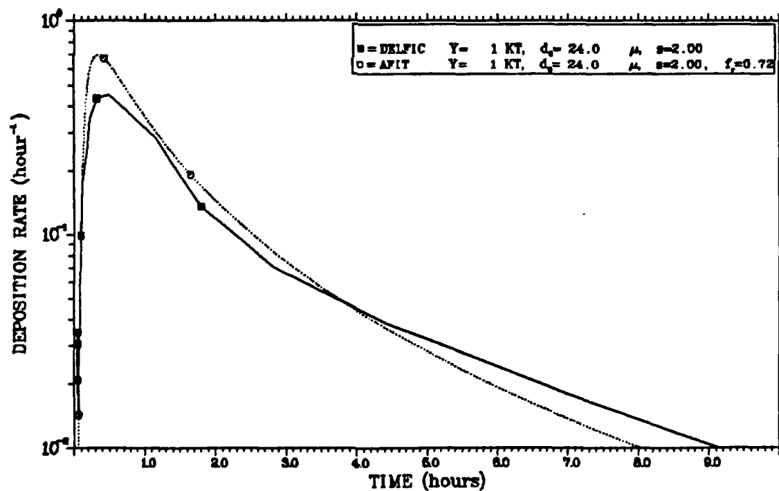
Figure C-21 Deposition Rates for the WSEG-10 Distribution
