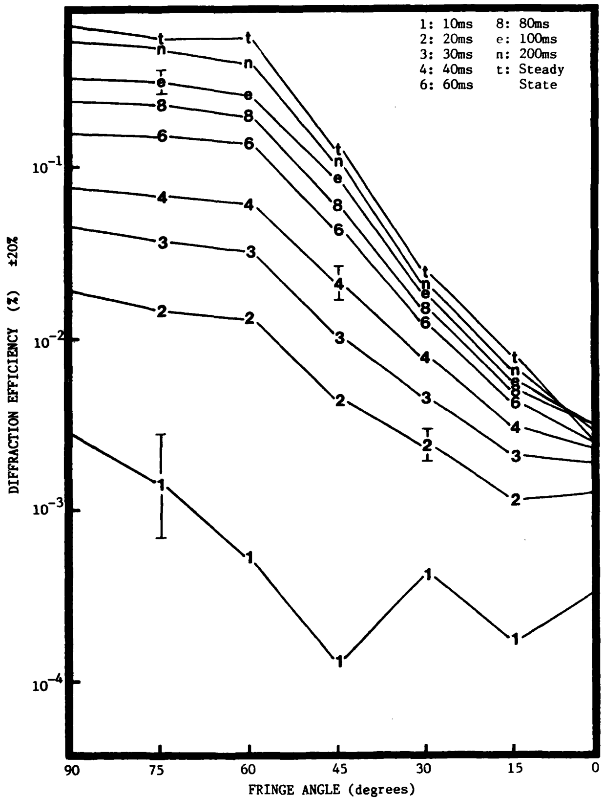
Figure 35. Diffraction efficiency versus fringe angle: M=0.82 , V=3kV , \Lambda=5\mu , horizontally polarized read beam, many write times
