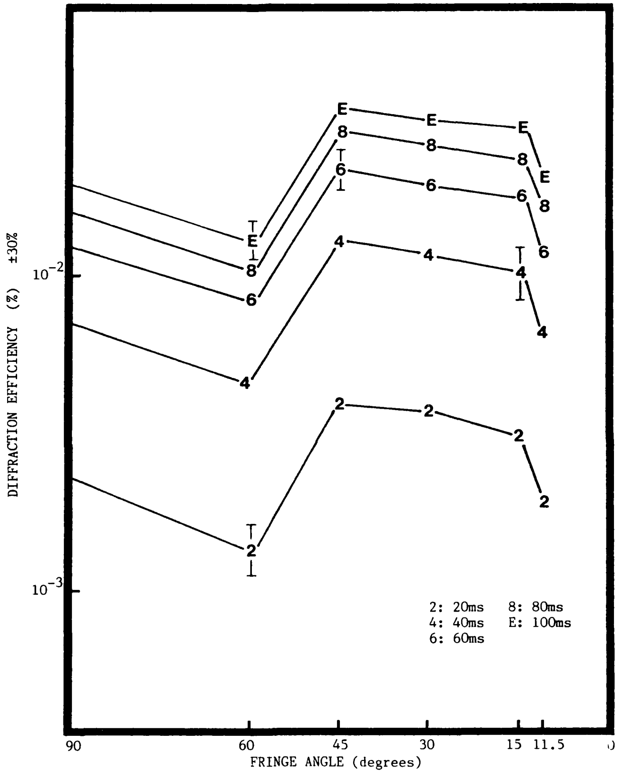
Figure 20. Diffraction efficiency versus fringe angle: M=0.82 , scaled V , \lambda=3\mu , vertically polarized read beam, many write times
