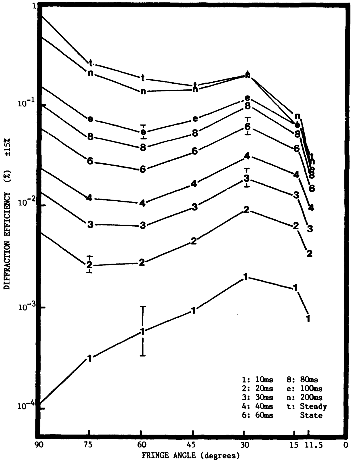
Figure 36. Diffraction efficiency versus fringe angle: M=0.45 , V=5\text{keV} , \lambda=5\mu , vertically polarized read beam, many write times
