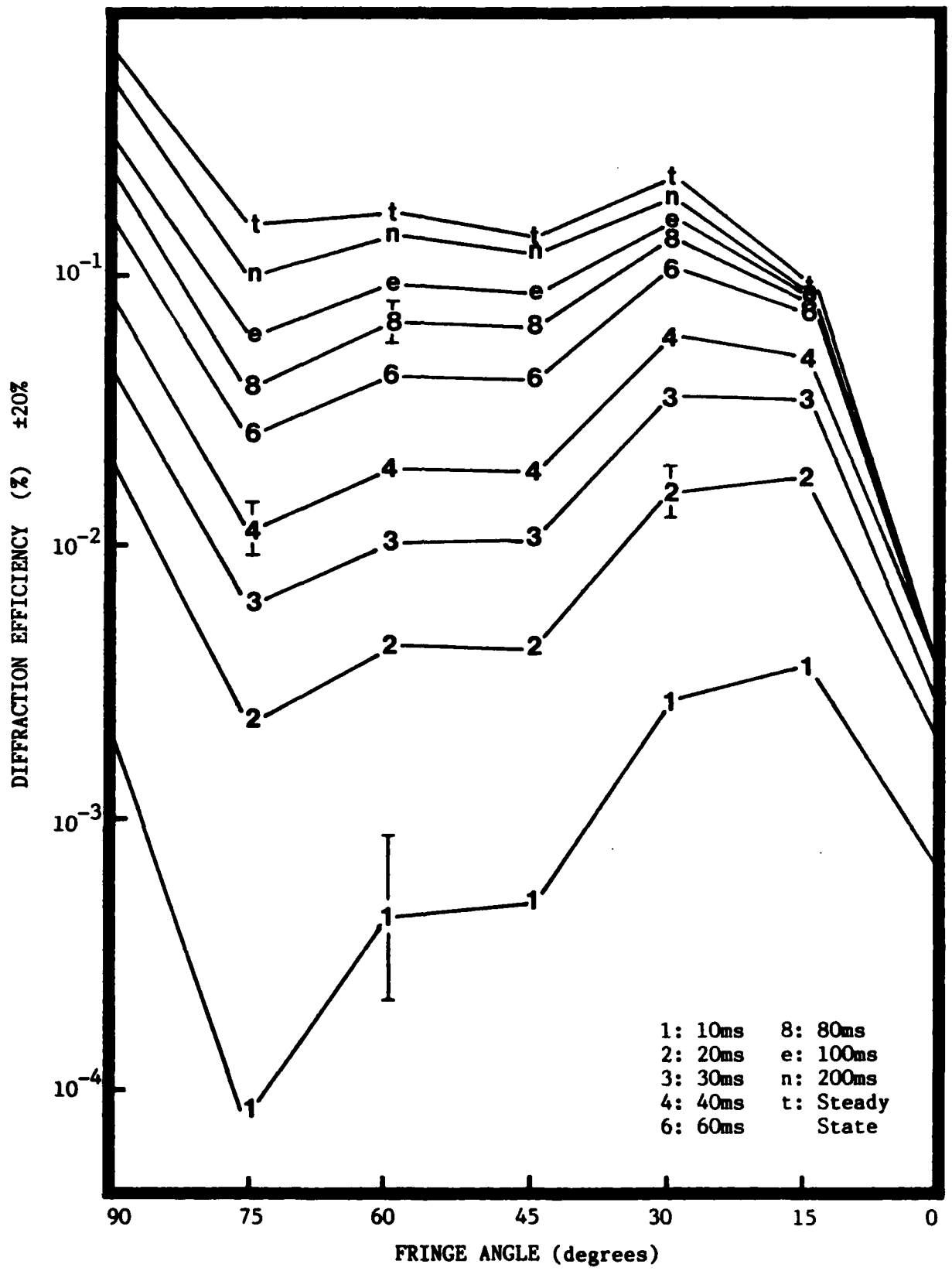
Figure 34. Diffraction efficiency versus fringe angle: M=0.82 , V=3kV , \lambda=5\mu , vertically polarized read beam, many write times
