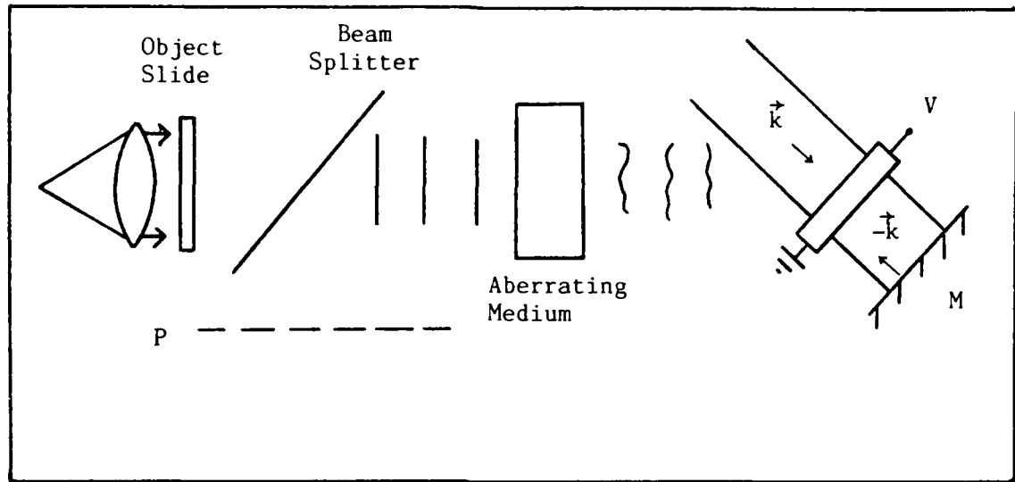
Figure 29. Setup for phase conjugate wavefront generation
