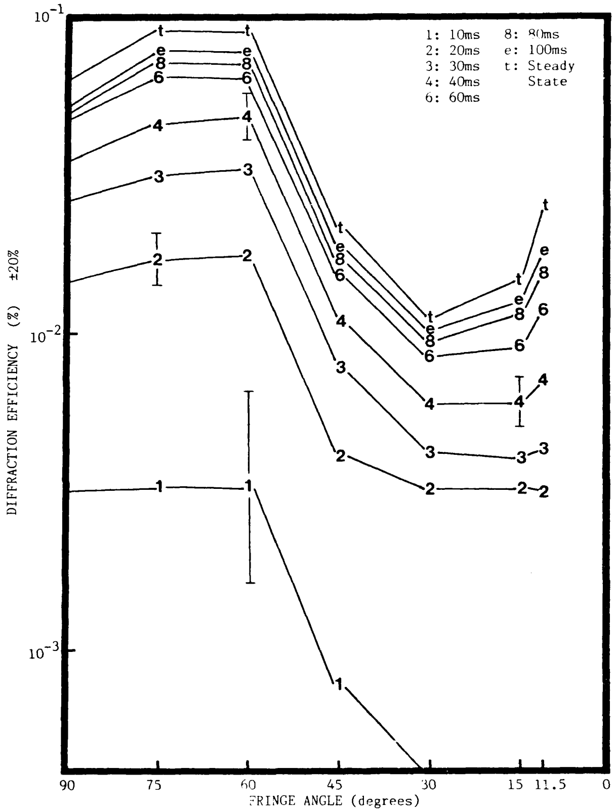
Figure 31. Diffraction efficiency versus fringe angle: M=0.82 , scaled \nu , \lambda=5\mu , horizontally polarized read beam, many write times
