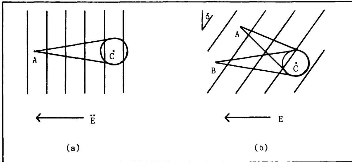
Figure 4. Electron migration in BSO for a sinusoidal intensity pattern: (a) perpendicular to applied field, (b) non-perpendicular to applied field
