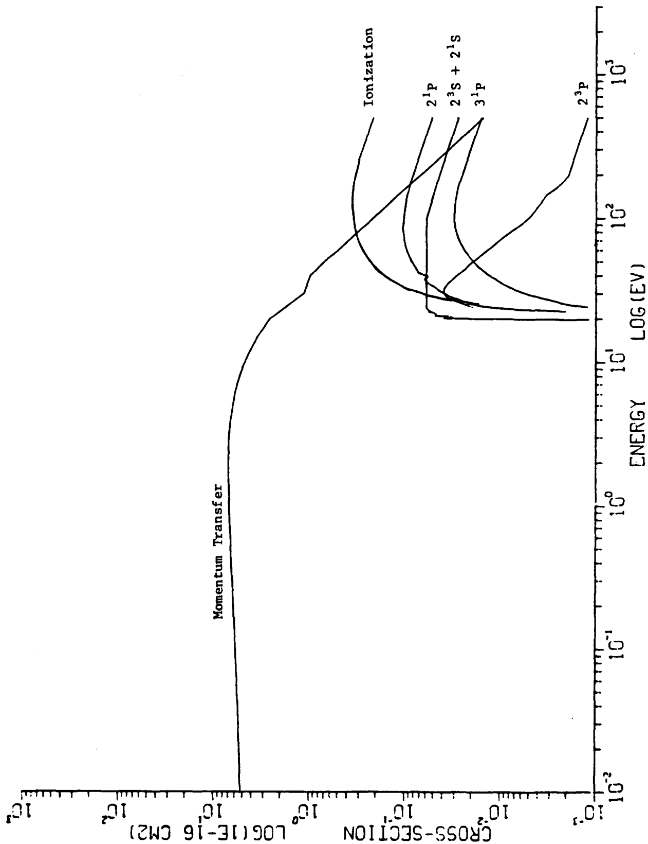
FIG C-2 ELECTRON IMPACT CROSS SECTIONS IN He
