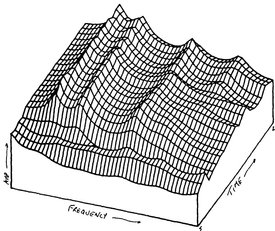
Figure 4-7 Formant Trajectory of the utterance "five." No added noise. Frames 2-25 shown. (SNR = 20 dB).
