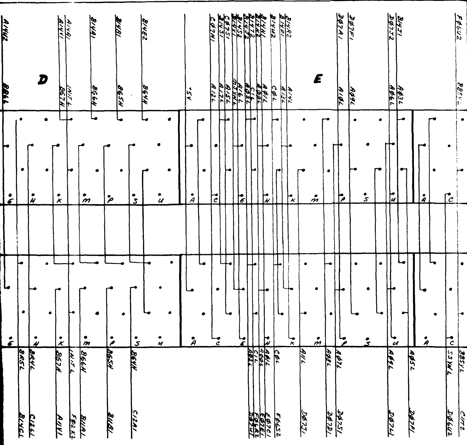
Figure 10. TTY/SPC Input and Output Signals on Backplane
