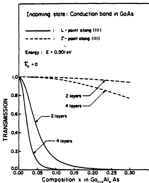
FIG. 4. Transmission coefficient T(k_{||}, E) as a function of alloy composition for two different \text{Ga}_{1-x}\text{Al}_x\text{As} barrier thicknesses. The incoming electron is either derived from the GaAs L point (solid line), or from the GaAs \Gamma point (dashed line). The energy of the incoming state is E = 0.501 eV above the GaAs \Gamma -point conduction band minimum and k_{||} = 0 . Layers are measured in units of a/\sqrt{3} , where a is the GaAs lattice constant.
