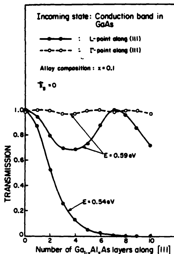
FIG. 3. Transmission coefficient T(k_{\parallel}, E) as a function of the number of layers forming the central \text{Ga}_{1-x}\text{Al}_x\text{As} barrier for various energies of the incoming electron. The incoming electron is either derived from the GaAs L point (solid line), or from the GaAs \Gamma point (dashed line). The alloy composition is x = 0.1 . Energy is measured with respect to the GaAs \Gamma -point conduction band minimum and k_{\parallel} = 0 . Layers are measured in units of a/\sqrt{3} , where a is the GaAs lattice constant.
