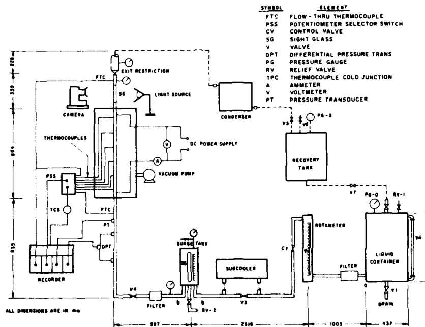
Figure 1 Schematic Drawing of the Experimental System
