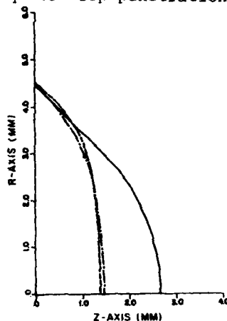
Fig. 1 Shape of weldpools after 8 sec of welding.
