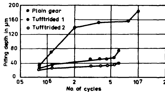
Fig. 2 Influence of tufftriding on durability
