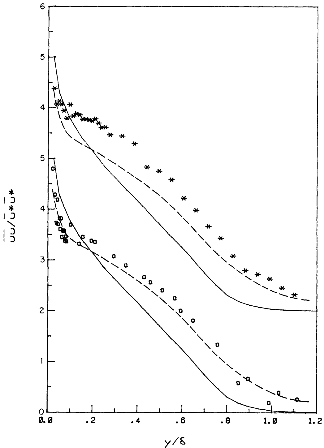
Figure 3.13. Time-mean distribution for \langle u^2 \rangle at station 4. Symbols as in Fig. 3.12.
