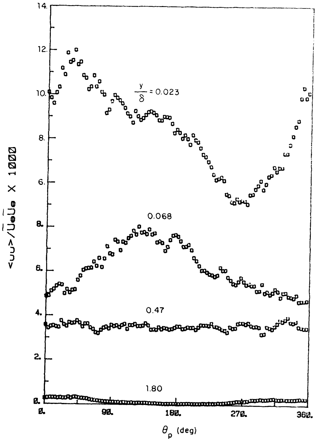
Figure 3.43. Phasewise variation of \langle u^2 \rangle at station 5 and f = 2 Hz.
