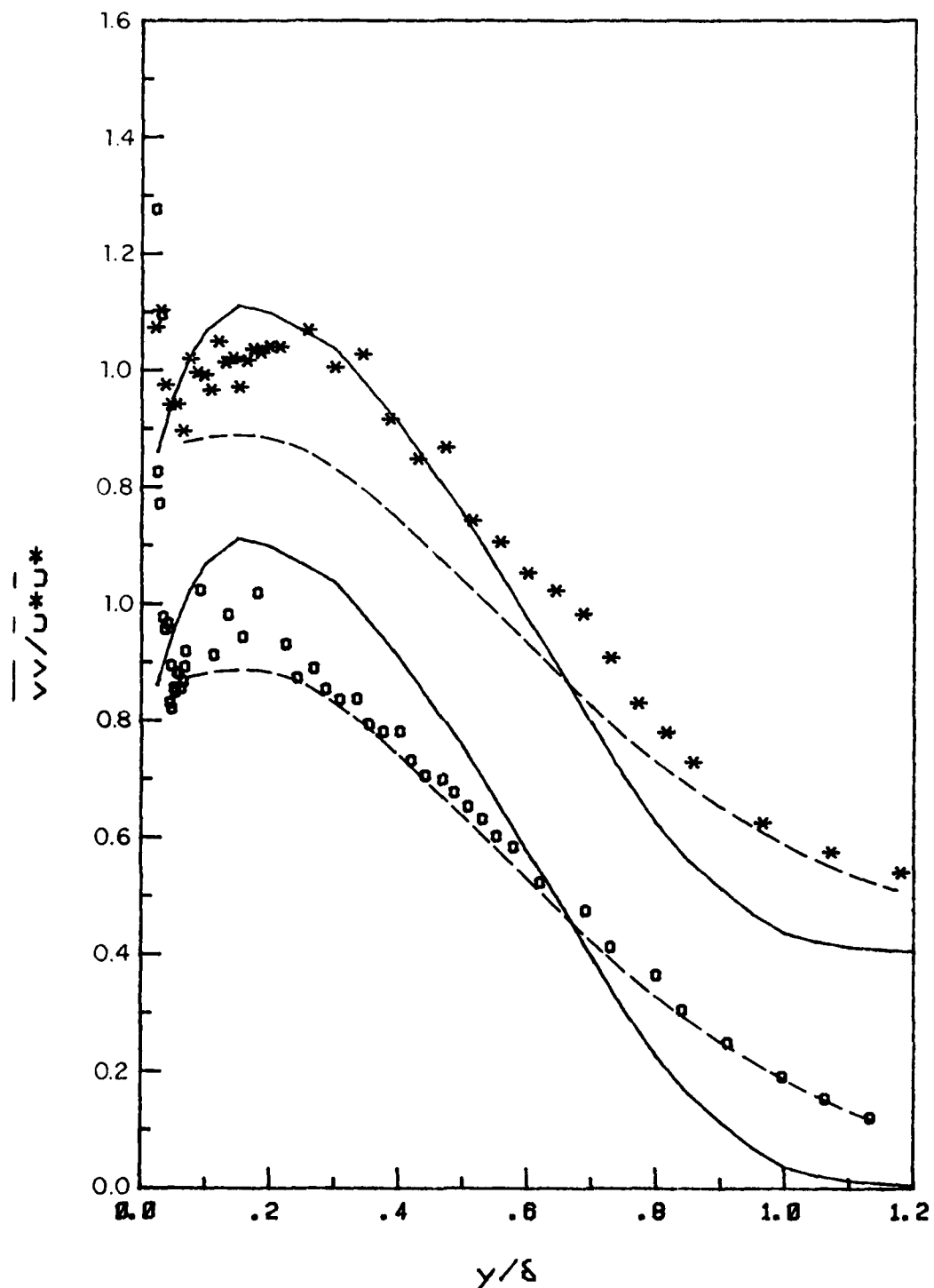
Figure 3.17. Time-mean distribution for \langle v^2 \rangle at station 5. Symbols as in Fig. 3.12.
