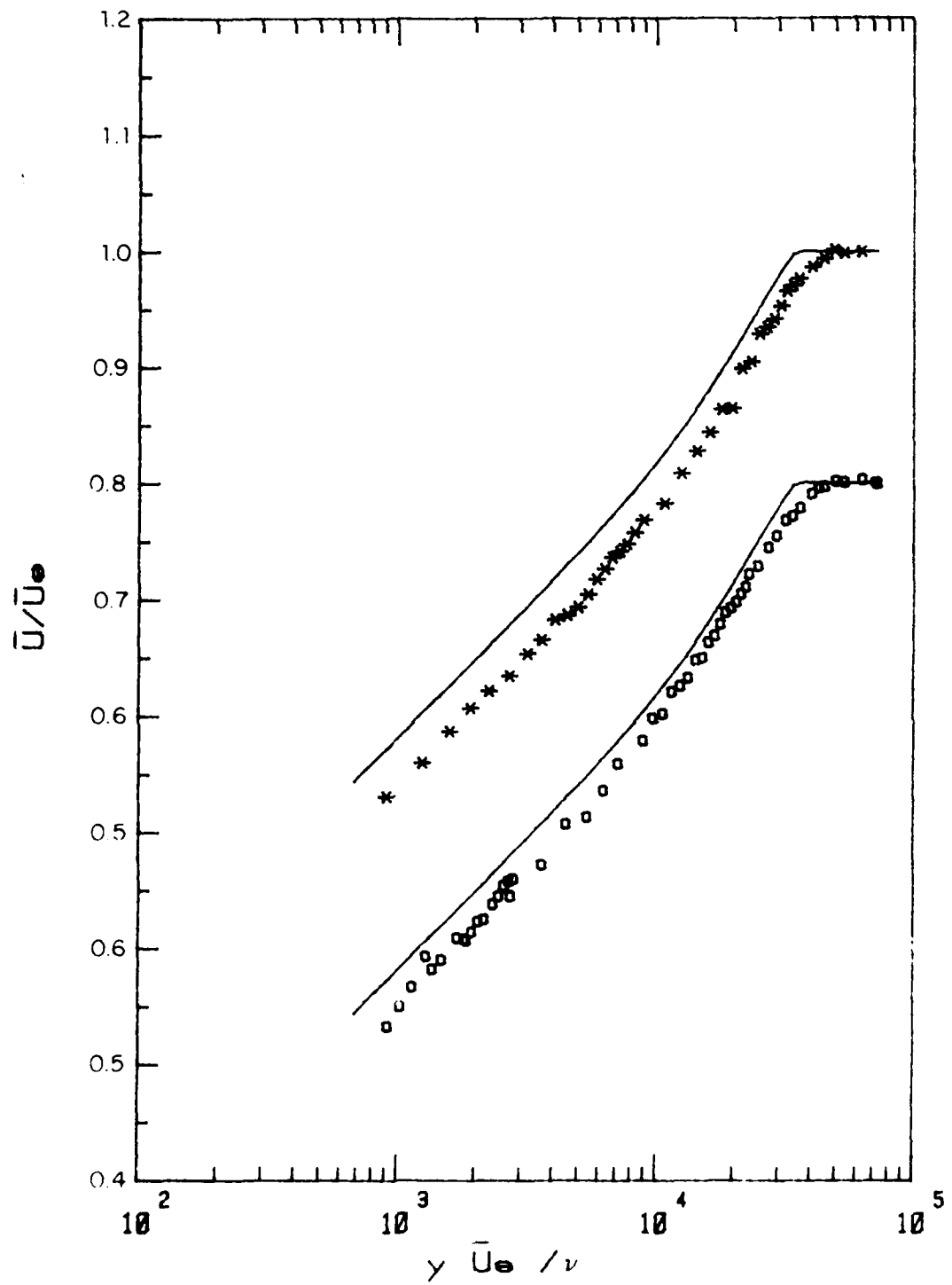
Figure 3.1. Time-mean velocity profile at station 5. * , f = 0.5 Hz; \circ , f = 2 Hz; —, quasi-steady.
