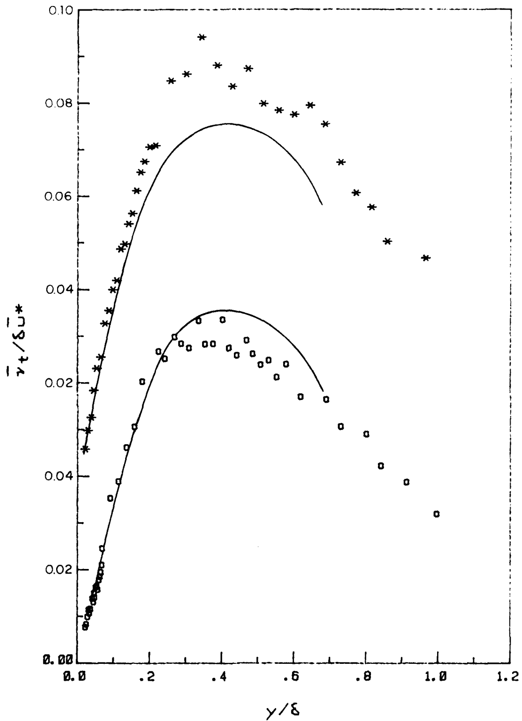
Figure 3.51. Time-mean distribution for \langle v_t \rangle . *, f = 0.5 \text{ Hz} , o, f = 2 \text{ Hz} ; —, quasi-steady
