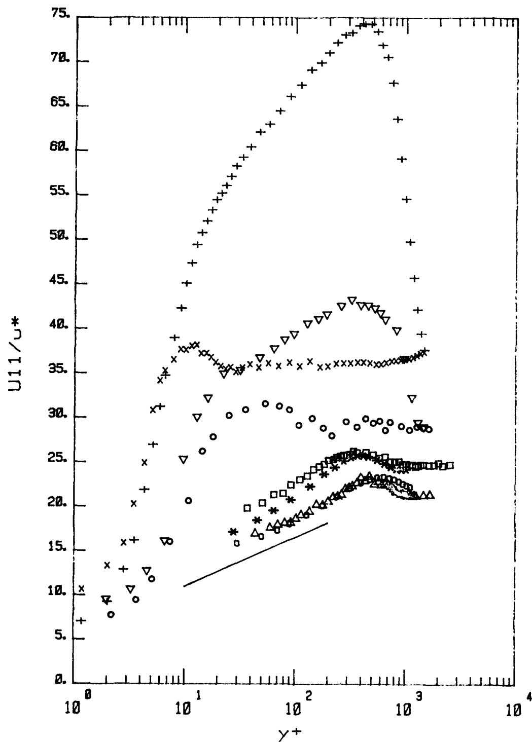
Figure 5.1. In-phase velocity component for the low and low/intermediate frequency regime. \Delta , experiment M1; \square , M5; * , CA; \circ , T1; \nabla , J1; \nabla , J2; + , J3; \times , J4; —, universal logarithmic law.
