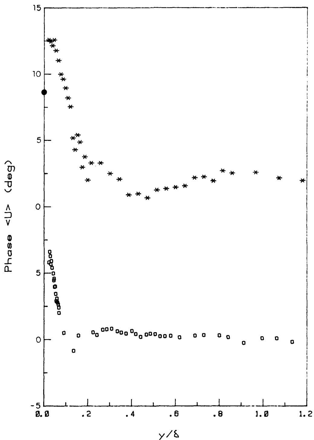
Figure 3.23. Phase distribution for the velocity at station 5. \bullet , phase of the wall shear stress for f = 0.5 Hz. Other symbols as in Fig. 3.21.
