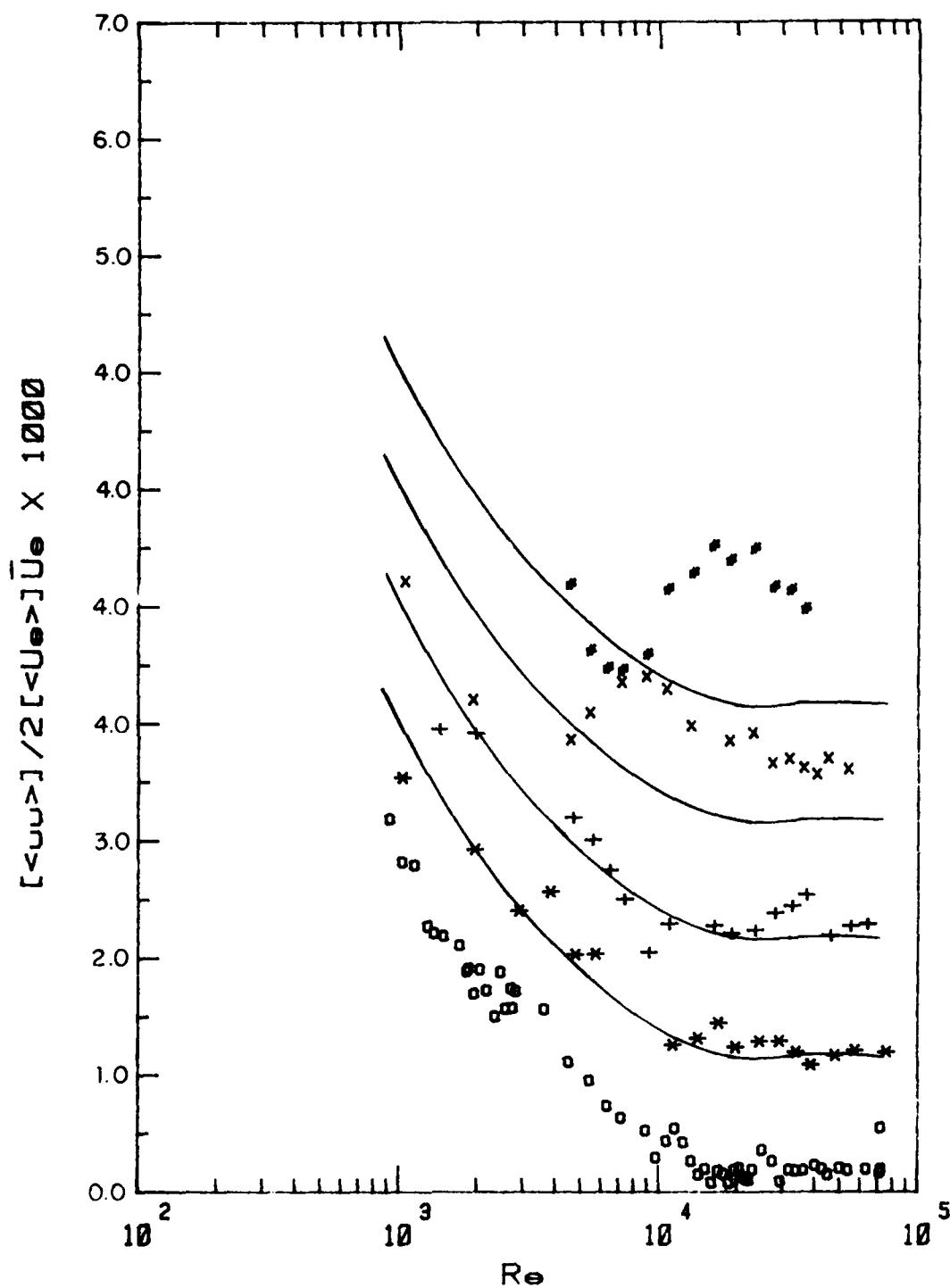
Figure 2.16. Check of two-dimensionality for [\langle u^2 \rangle] . Symbols as in Fig. 2.8.
