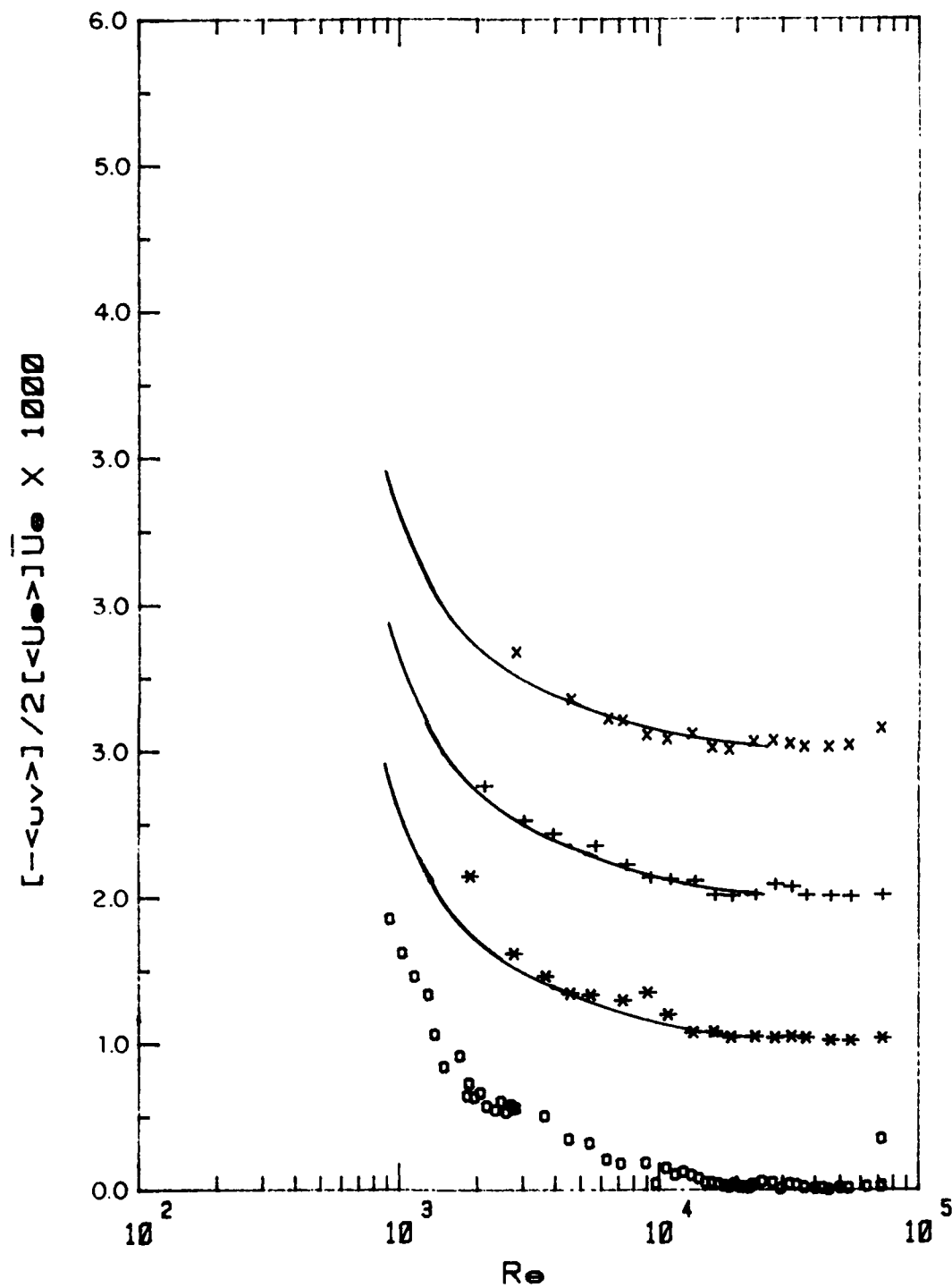
Figure 2.19. Check of two-dimensionality for [-\langle uv \rangle] . Symbols as in Fig. 2.7.
