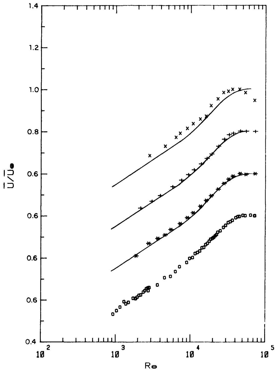
Figure 2.7. Check of two-dimensionality for \bar{U} . o, ---, z = 18.9 cm; *, z = 16.2 cm; +, z = 13.6 cm; x, z = 8.3 cm.
