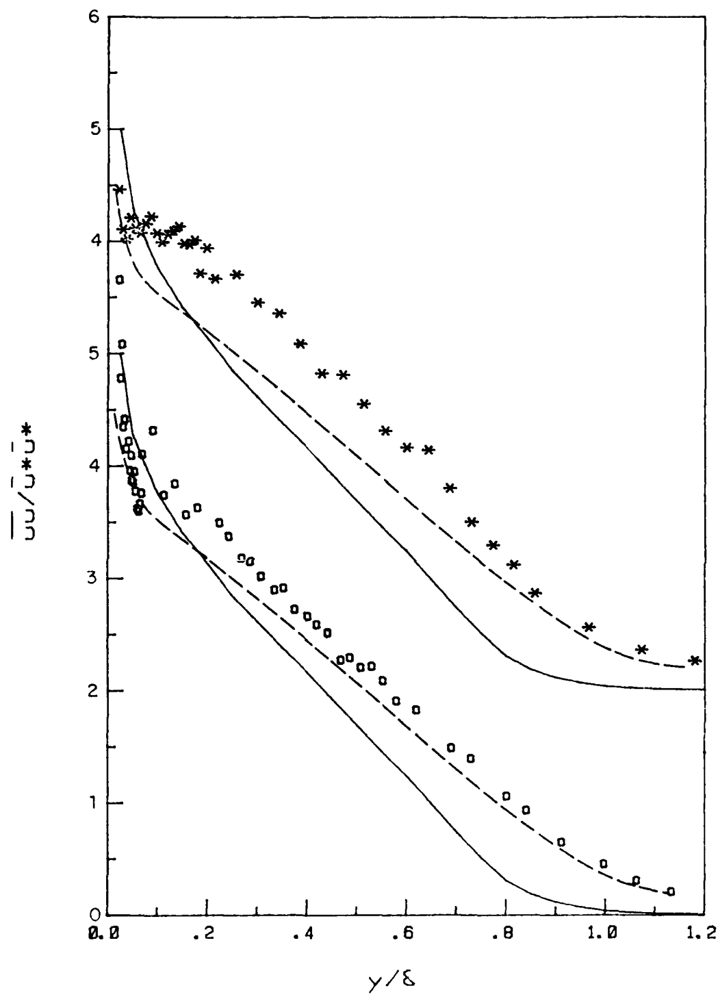
Figure 3.12. Time-mean distribution for \langle u^2 \rangle at station 5. *, f = 0.5\text{ Hz} ; \circ , f = 2\text{ Hz} ; ---, steady flow; —, Klebanoff's data (1954).
