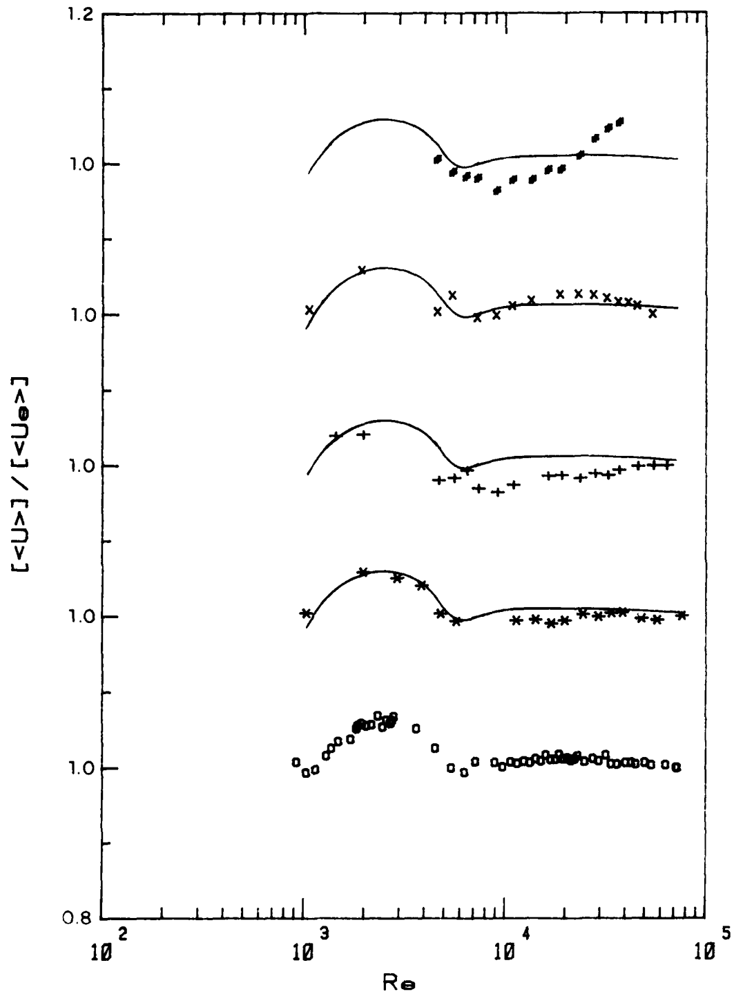
Figure 2.10. Check of two-dimensionality for [\langle U \rangle] . Symbols as in Fig. 2.8.
