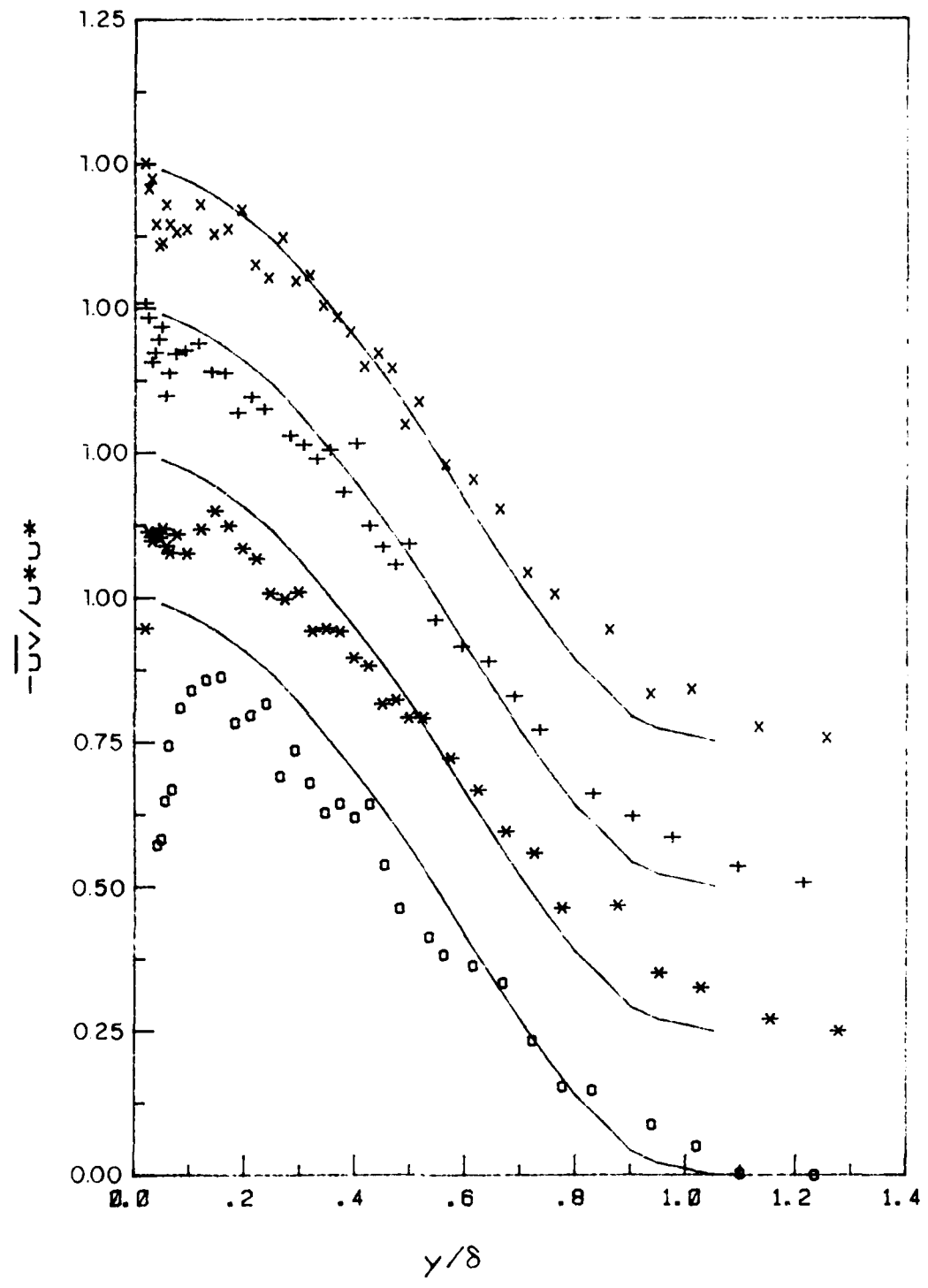
Figure 2.30. Steady-flow distribution for -\overline{uv} at station 5. Symbols as in Fig. 2.27.
