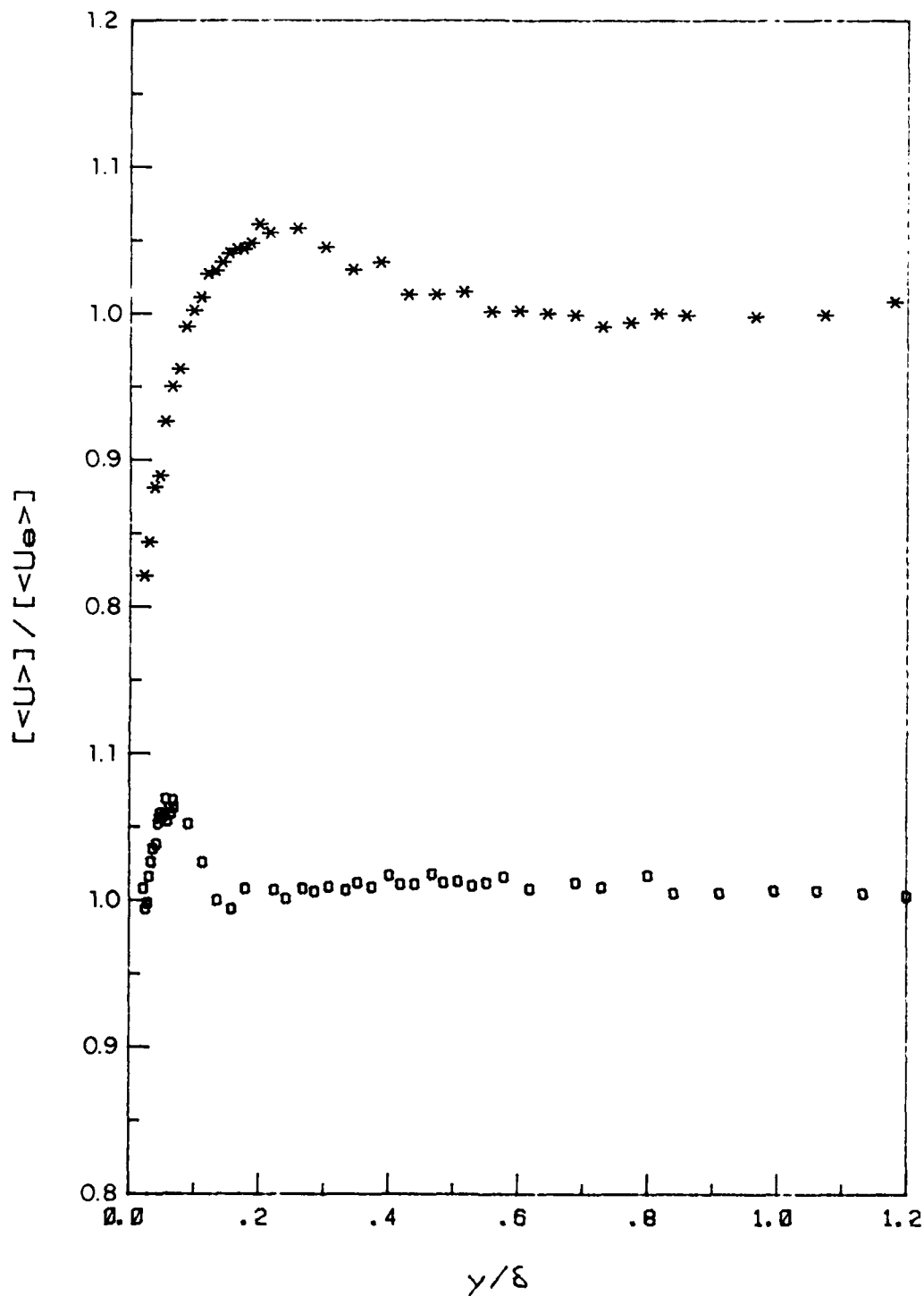
Figure 3.21. Amplitude distribution for the velocity at station 5. *, f = 0.5 \text{ Hz} ; o, f = 2 \text{ Hz} .
