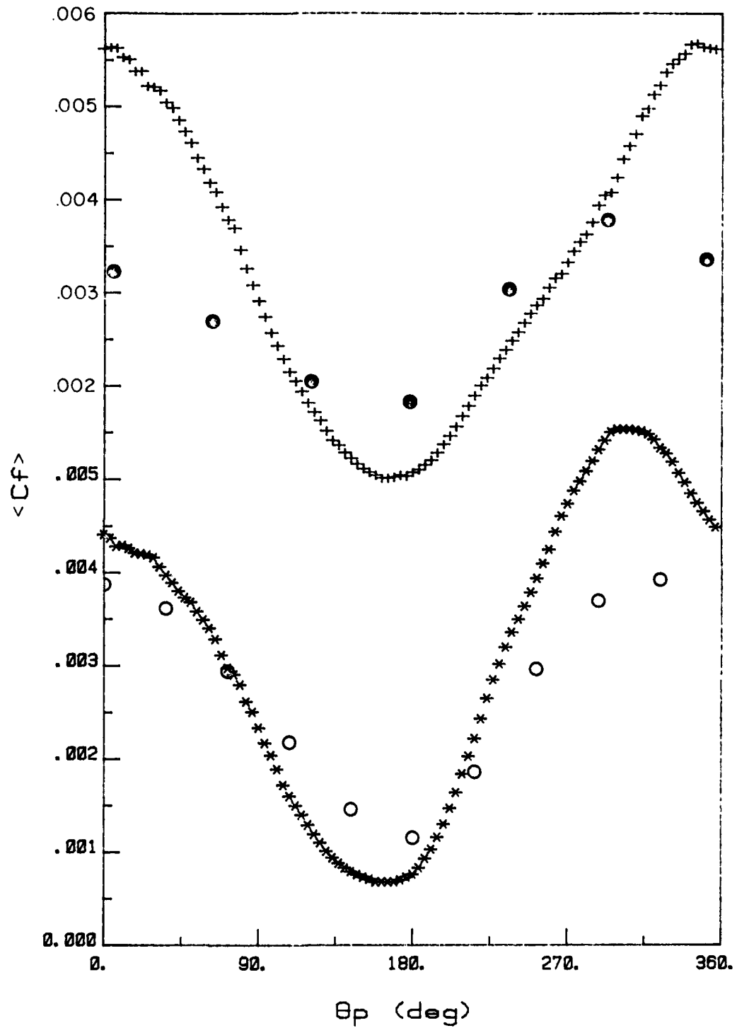
Figure 3.50. Phasewise distribution of \langle C_f \rangle . \circ , f = 2 Hz, from Clouser-plot; \bullet , f = 0.5 Hz, from Clouser-plot; * , f = 2 Hz, measured; + , f = 0.5 Hz, measured.
