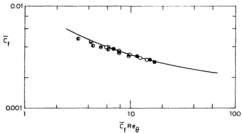
Figure 2.25. Correlation between \bar{c}_f and Re_\theta for steady flow. \circ , station 1; \bullet , 2; \square , 3; \triangle , 4; \diamond , 5; —, 'normal' curve [Coles (1962)].
