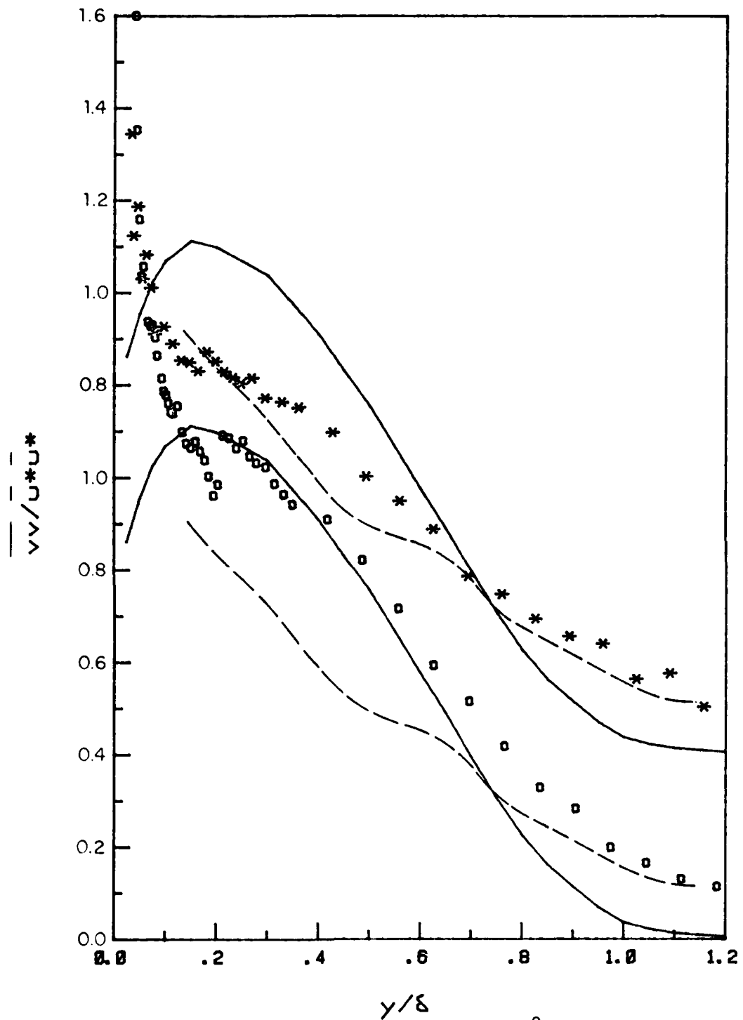
Figure 3.18. Time-mean distribution for \overline{v^2} at station 3. Symbols as in Fig. 3.12.
