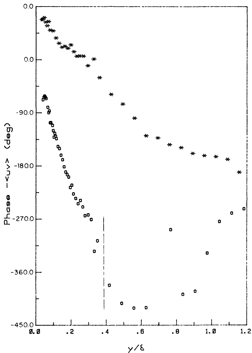
Figure 3.36. Phase distribution for - \langle uv \rangle at station 3. ---, edge of unsteady layer. Other symbols as in Fig. 3.21.
