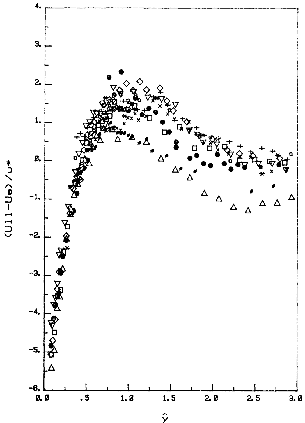
Figure 5.4. In-phase velocity component in the unsteady layer coordinates. \bullet , experiment M1; \diamond , M2; \nabla , M3; \triangle , M4; \square , M5; * , M6; \times , M7; + , M8; * , M9; \circ , M10.
