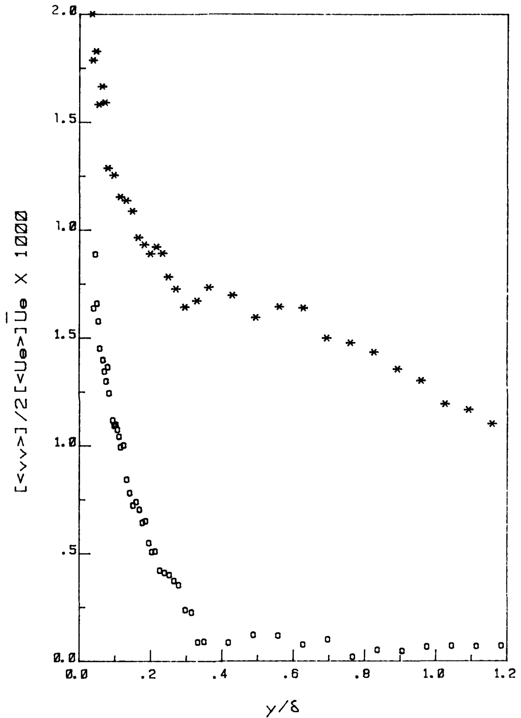
Figure 3.30. Amplitude distribution for \langle v^2 \rangle at station 3. Symbols as in Fig. 3.21.
