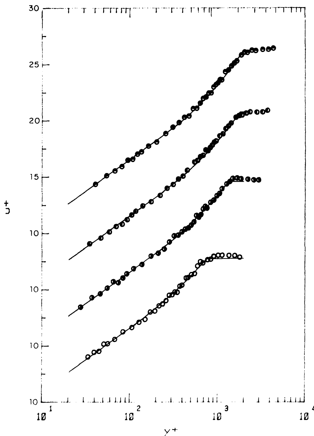
Figure 2.24. Steady velocity profiles at station 5 in the inner coordinates. \circ , U_e = 50.69 cm/s; \bullet , U_e = 90.18 cm/s; \ominus , U_e = 119.74 cm/s; \bullet , U_e = 141.77 cm/s; ---, Coles' fit.
