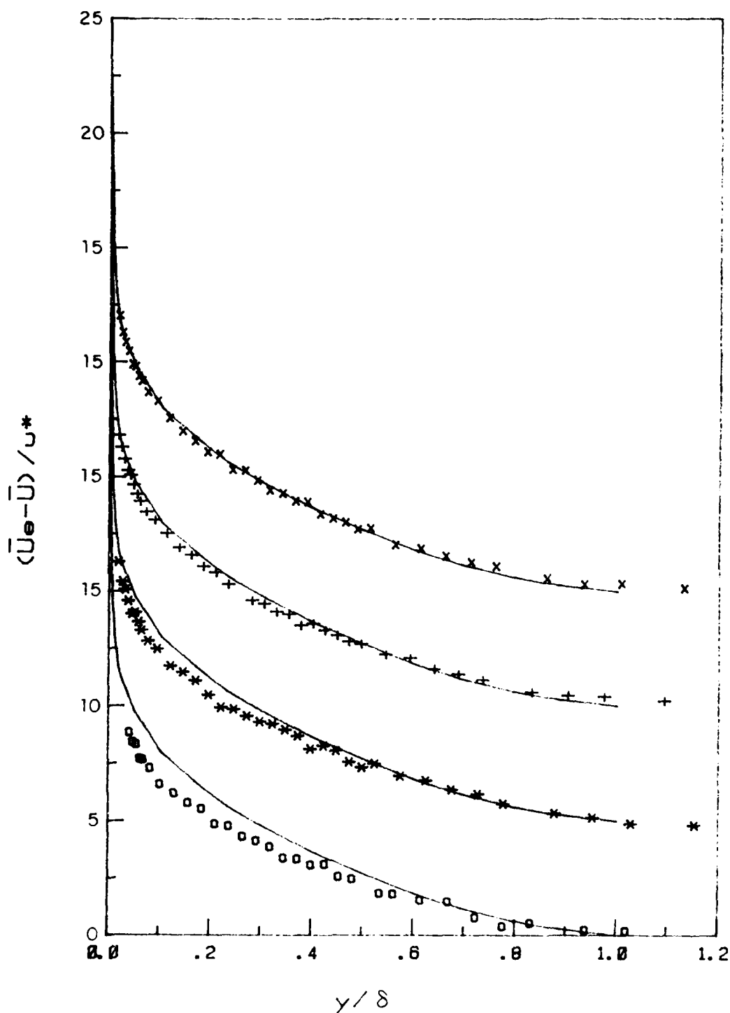
Figure 2.27. Steady velocity profiles at station 5 in the outer coordinates. \circ , \bar{U}_e = 50.69 cm/s; * , \bar{U}_e = 90.18 cm/s; + , \bar{U}_e = 119.74 cm/s; \times , \bar{U}_e = 141.77 cm/s; —, Klebanoff's data (1954).
