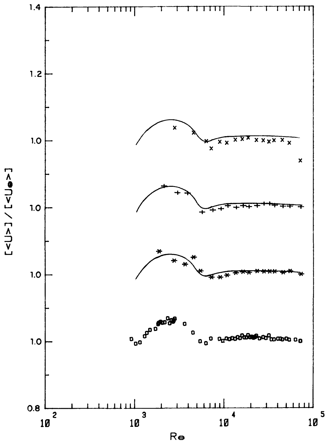
Figure 2.9. Check of two-dimensionality for [\langle U \rangle] . Symbols as in Fig. 2.7.
