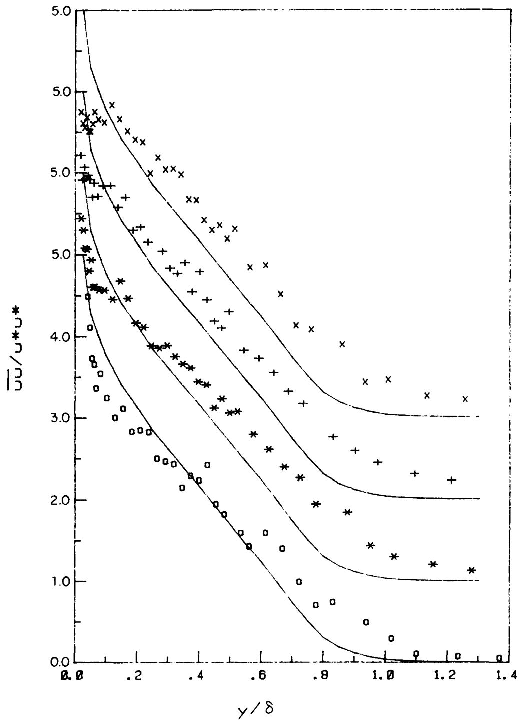
Figure 2.28. Steady-flow distribution for \overline{u^2} at station 5. Symbols as in Fig. 2.27.
