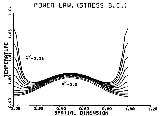
Figure (V.19.b) - Temperature profiles for the problem defined in Fig. (V.19.a).
