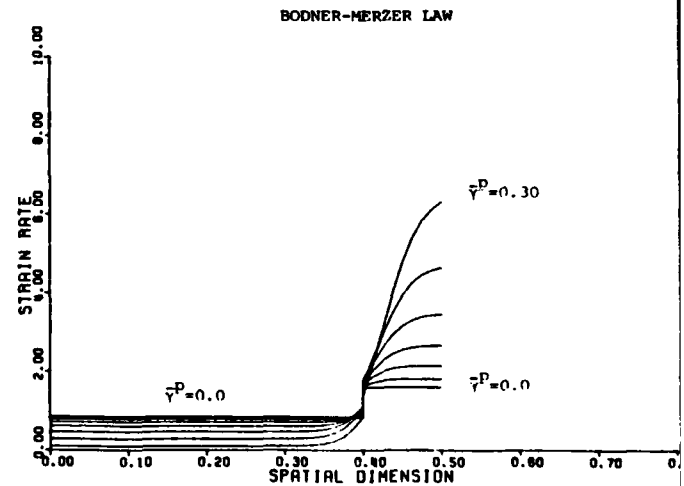
Figure (V.17.d) - strain rate profiles for Merzer's Model.
