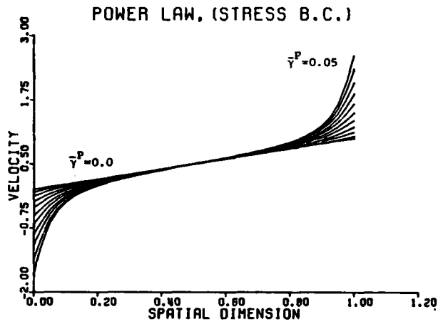
Figure (V.19.a) - Initial temperature perturbation, \epsilon=0.005 , \nu=-0.75 , m=-0.95 , n=1 ; stresses are prescribed at the boundaries. Plots are obtained for intervals of \bar{\gamma}^P=0.005 .
