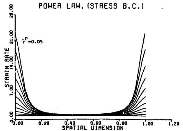
Figure (V.19.d) - strain rate profiles for the problem defined in Fig. (V.19.a). Notice the intense deformation rates near the boundaries.
