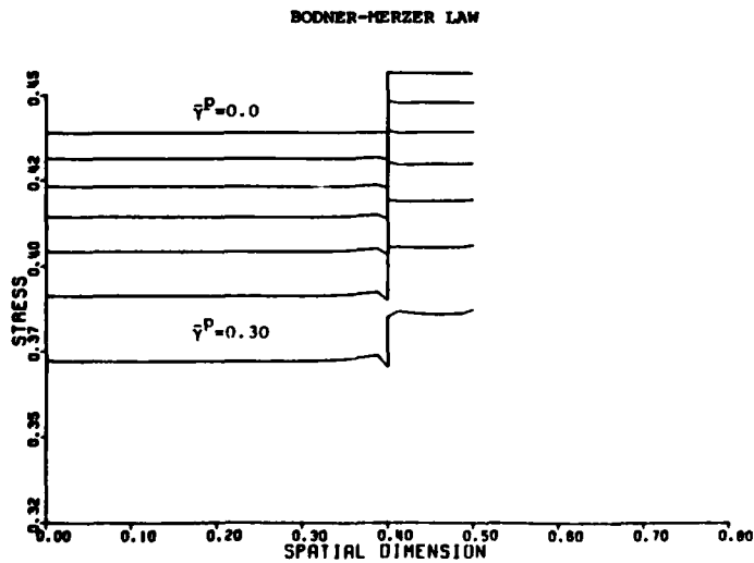
Figure (V.17.c) - stress profiles for Merzer's Model.
