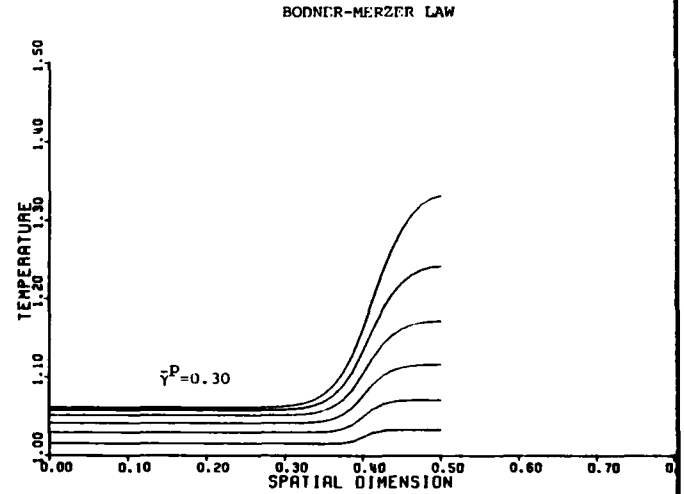
Figure (V.17.b) - Temperature profiles for Merzer's Model.
