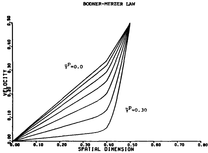
Figure (V.17.a) - Merzer's Model, \delta = 0.1 , \lambda = 1.04 , same parameters as in Merzer's Calculation; profiles are obtained for intervals of ( \bar{\gamma}^P = 0.05 ).
