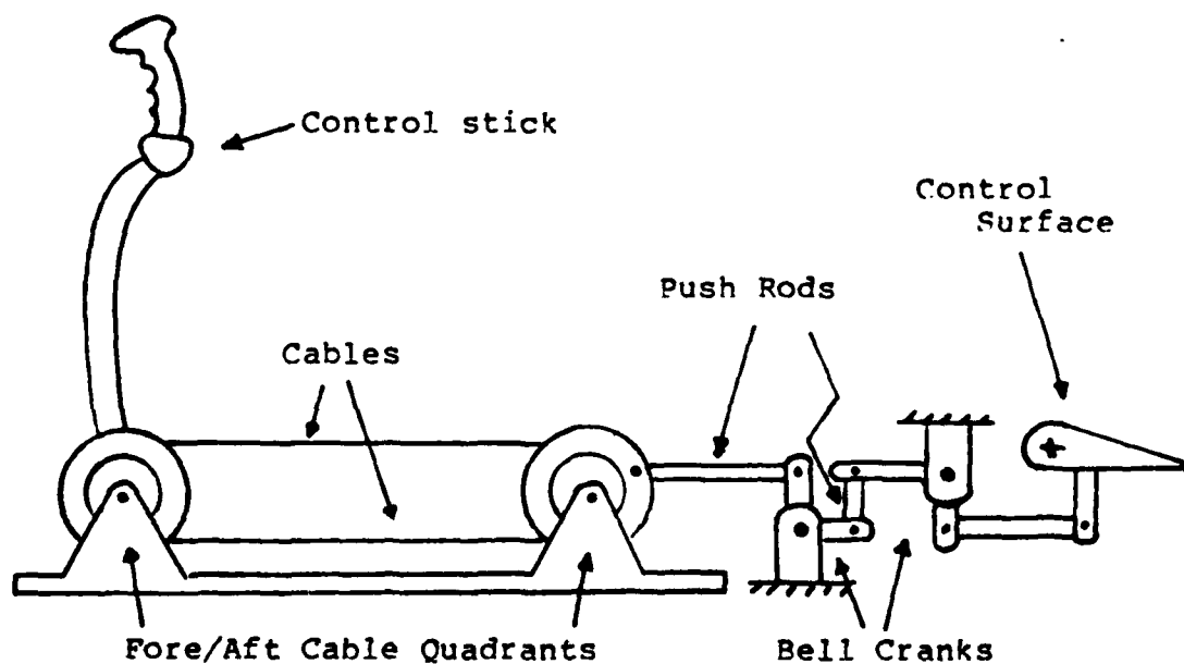
Figure 3.3. Mechanical Longitudinal Control System
