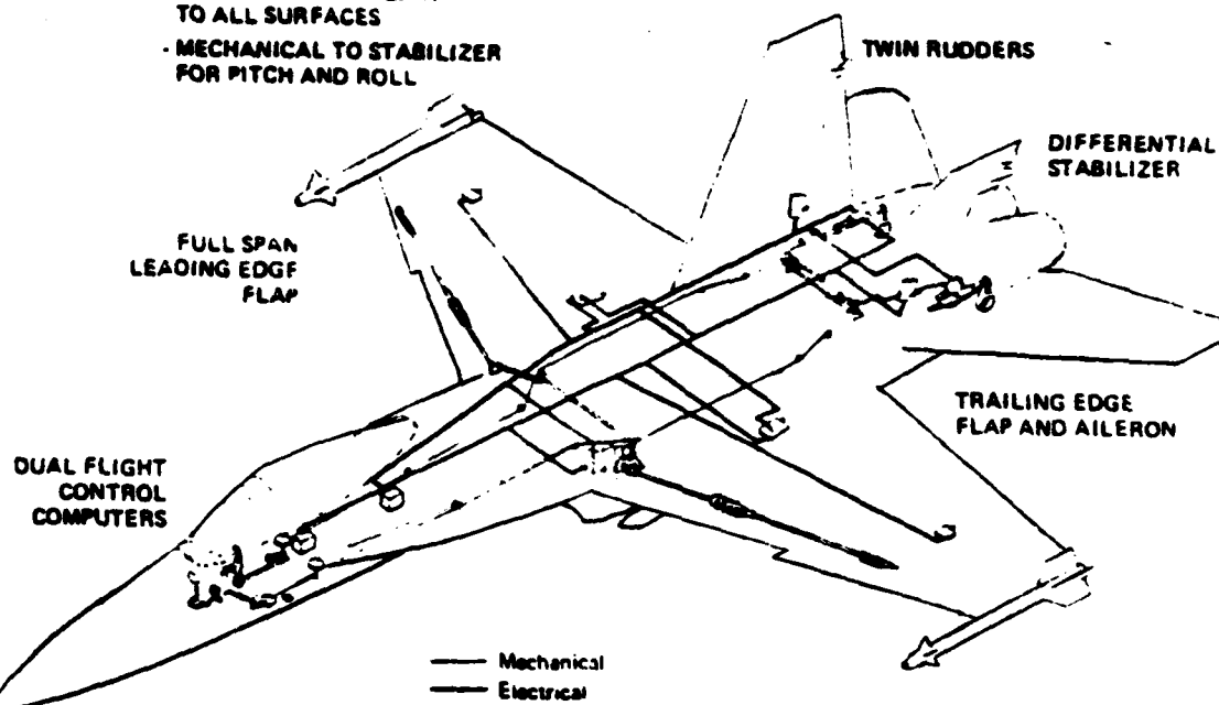
Figure 3.8. F/A-18 FCS Elec/Hech Subsystem Diagram
