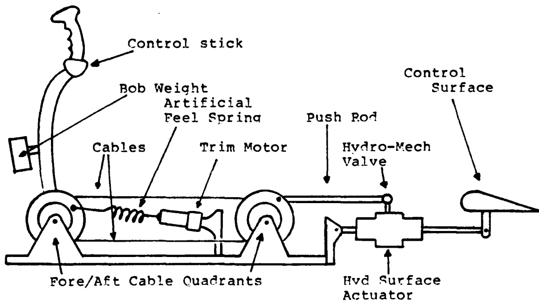
Figure 3.5. Hydraulic Powered Longitudinal Control System
