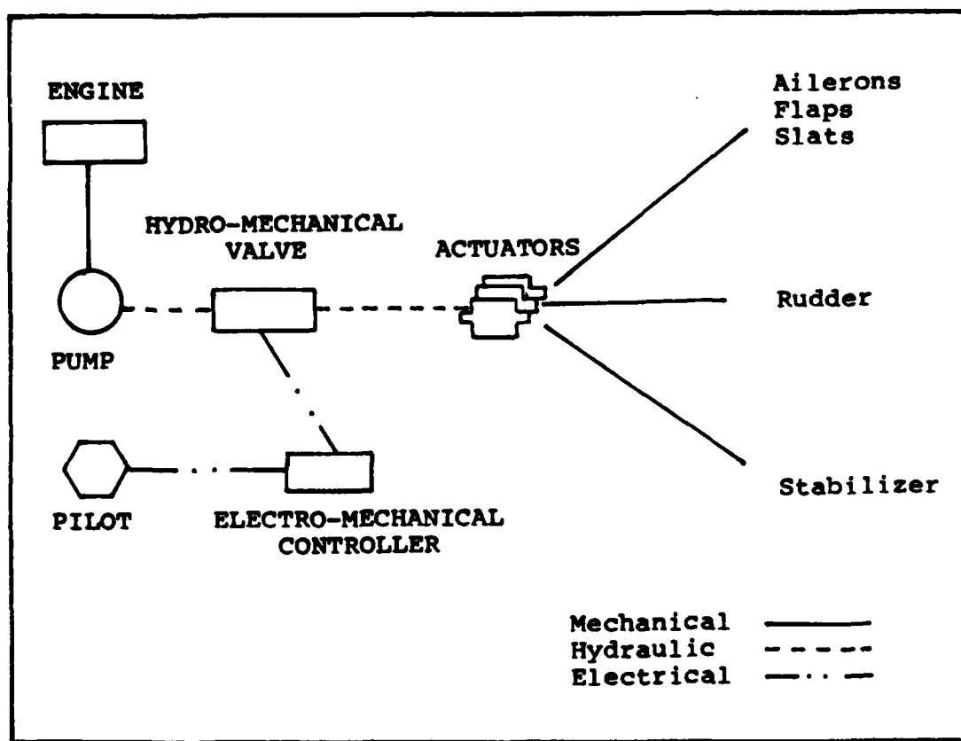
Figure 4.1. Generic DFBW FCS Illustration
