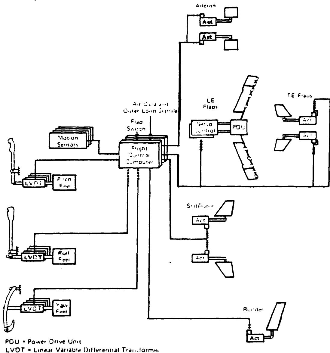
Figure 4.2. Technical/Functional Interfaces - DFBW PCS
