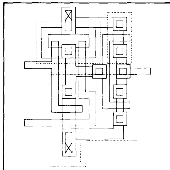
FIGURE 3. One possible layout of a CMOS NAND-plus-inverter module.
