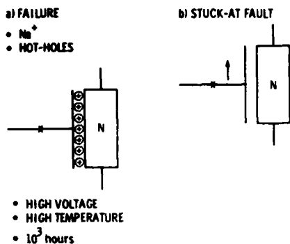
Fig. 7 An open connection to a gate of a transistor in the presence of positive charges in the gate oxide is modeled as a stuck-at fault
