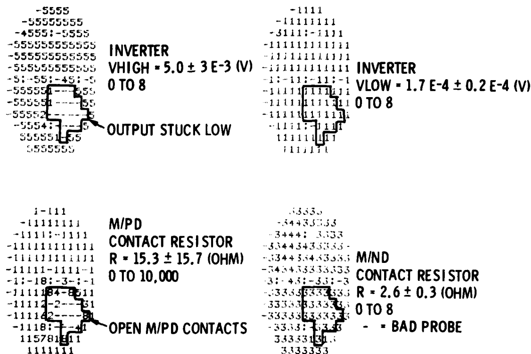
Figure 2.5.2-1. Wafer maps of CMOS-bulk inverters and contact resistors showing that some inverter outputs are stuck low due to open metal to p-diffusion contacts (wafer 1102).
