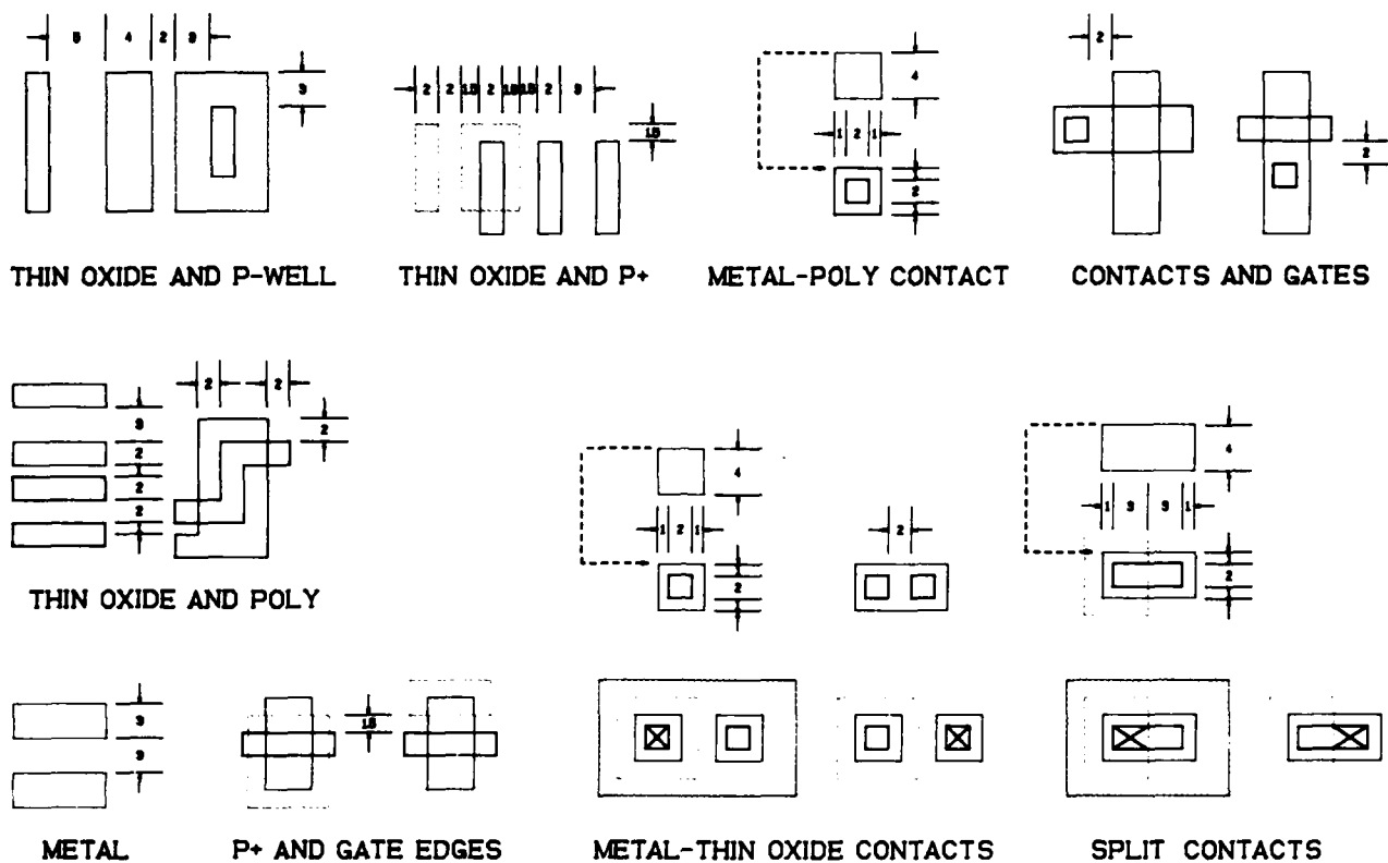
FIGURE 2. Bulk CMOS geometrical design rules (p-well process).
