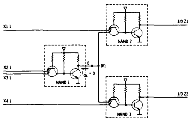
b) SINGLE STUCK-AT FAULT
