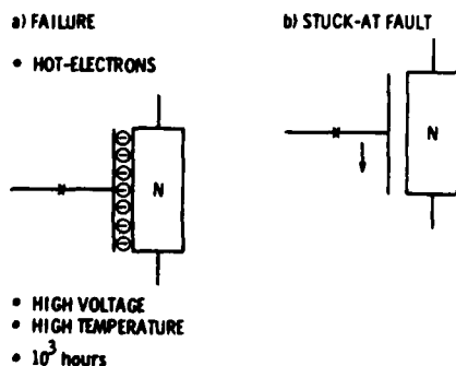
Fig. 8 An open connection in the presence of negative charges in the gate oxide and its stuck-at fault model
