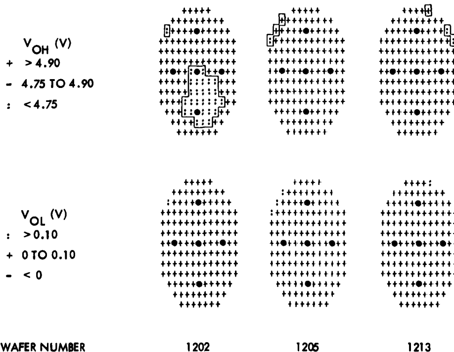
Figure 2.5.2-2. Wafer maps of CMOS-bulk inverters from run 1 showing the regions where the inverters failed to toggle properly.
