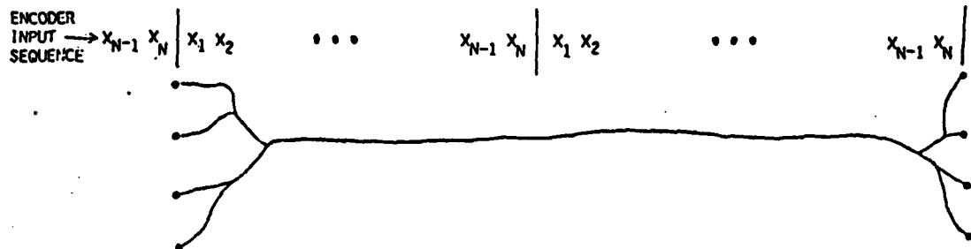
B) TRELLIS WITH TWO DECODING PASSES. MERGED PATHS IN THE CENTER PORTION OF THE TRELLIS PROVIDE A RELIABLE ESTIMATE OF THE DATA BLOCK.
