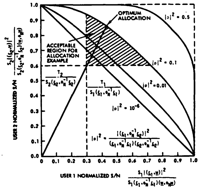
Figure 7. Achievable S/N Pairs for Two Multiple Access Users
