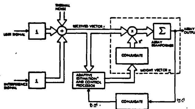
Figure 1. Adaptive Spatial Filter Concept
