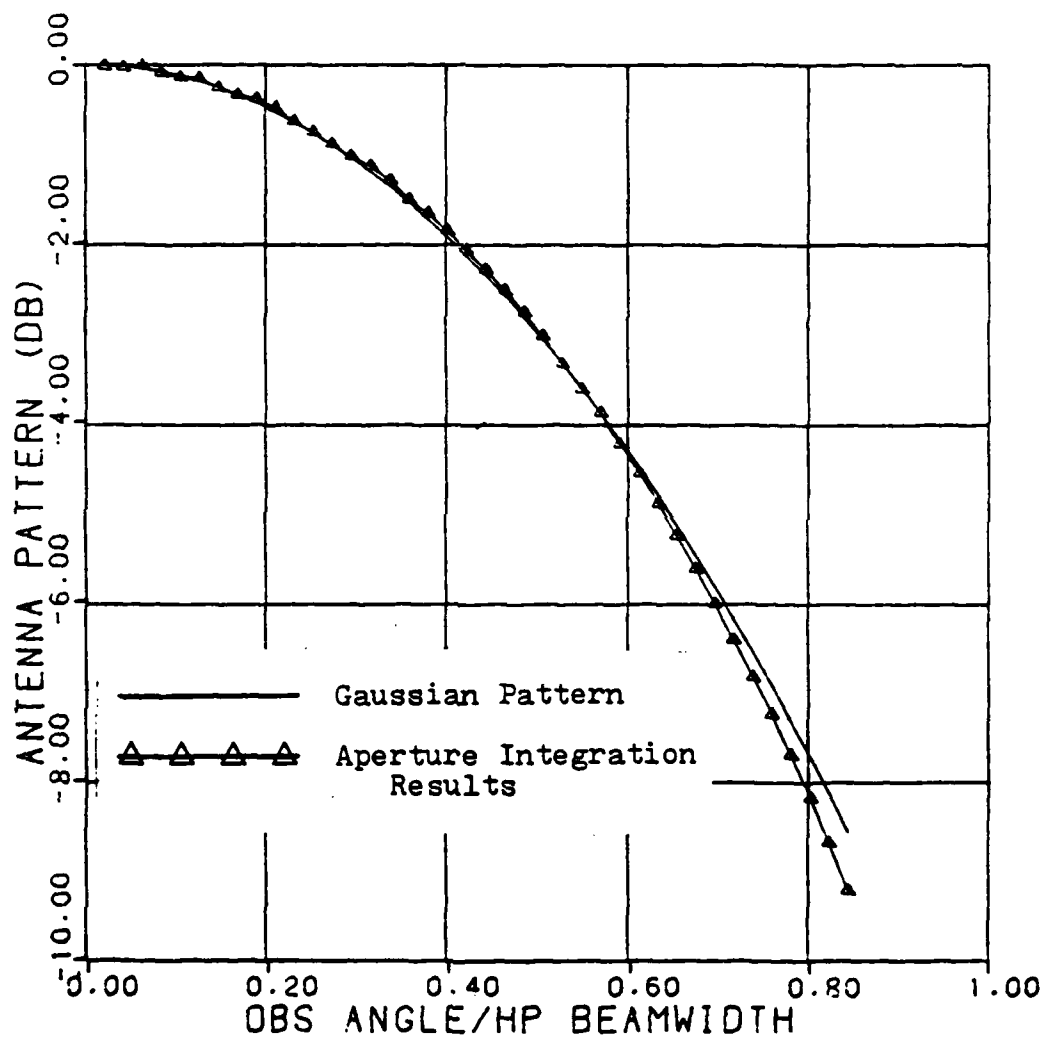
Fig. VII-2. Comparison of the Horizontal Antenna Pattern and the Gaussian Pattern ( C=.1 , a=1.828\text{m} , D=.347\text{m} , \theta_T=.5 deg, \sigma=.03125\text{m} )
