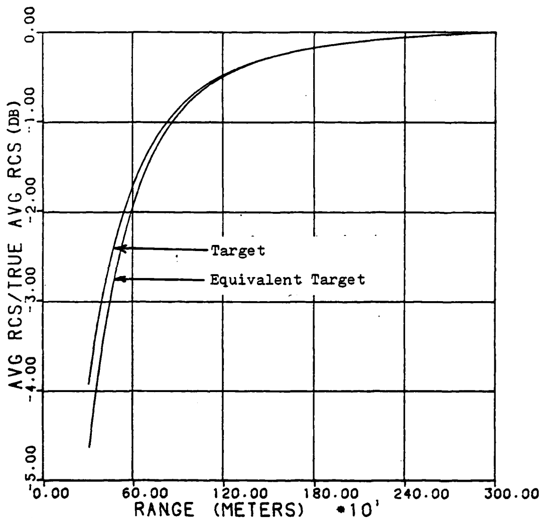
Fig. VIII-19. Comparison of Average RCS Variation for a Specific Target and its Equivalent Length Target (Target Distribution- p_G(\bar{y}) , SD=4.57m , L=18.28m ; Equivalent Target- L'_G=14.0m ; \theta_3=1.18 deg)
