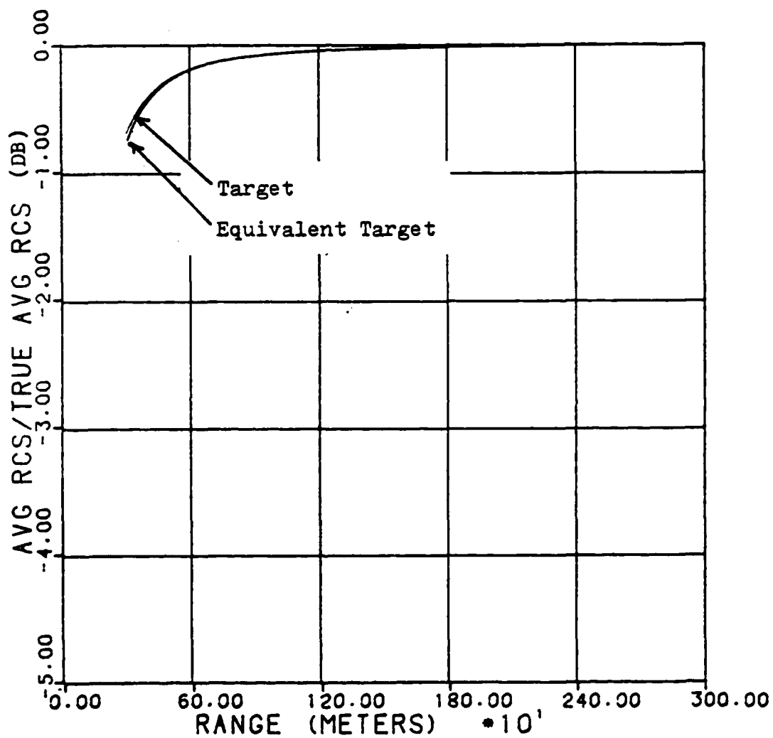
Fig. VIII-21. Comparison of Average RCS Variation for a Specific Target and it's Equivalent Length Target (Target Distribution- p_G(y) , SD=1.14m , L=18.28m ; Equivalent Target- L_G^*=4.2m ; \theta_3=1.18 deg)
