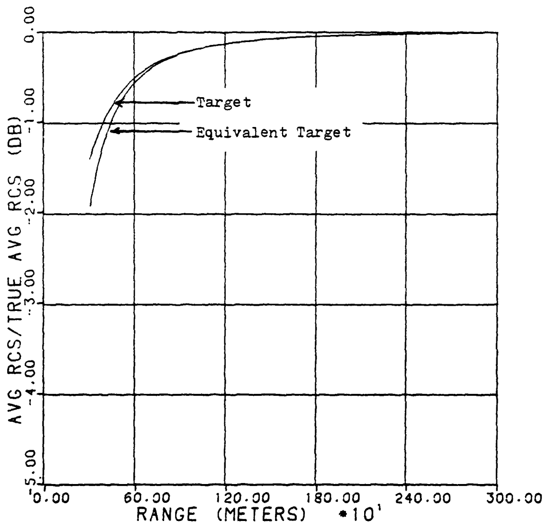
Fig. VIII-8. Comparison of Average RCS Variation for a Specific Target and its Equivalent Length Target (Target Distribution- p_a(y) , x=1/2 , L=9.144m , W=.9144m ; Equivalent Target- L'_a=6.84m ; \theta_3=1.18 deg)
