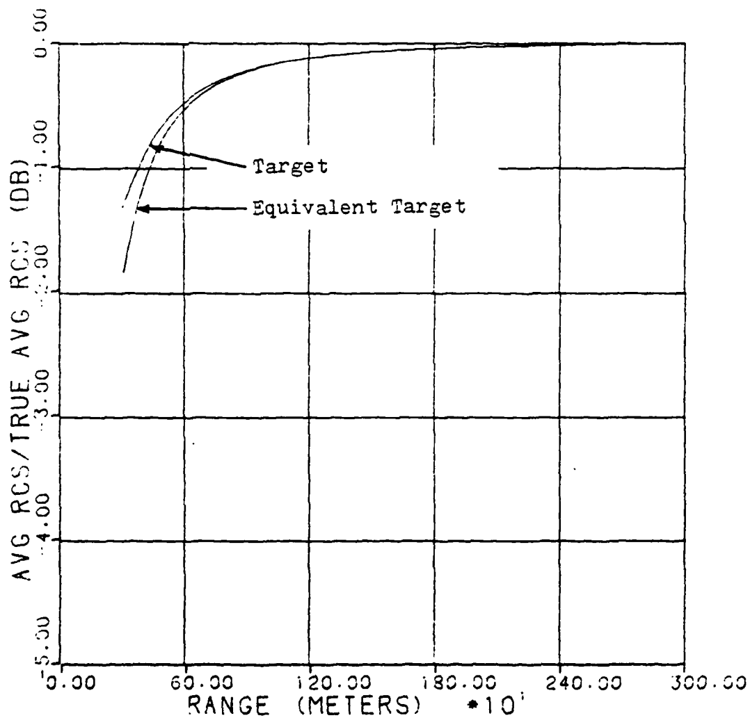
Fig. VIII-14. Comparison of Average RCS Variation for a Specific Target and its Equivalent Length Target (Target Distribution- p_b(y) , m=10 , L=9.144m , W=.9144m ; Equivalent Target- L'_b=6.66m ; \theta_3=1.18 deg)
