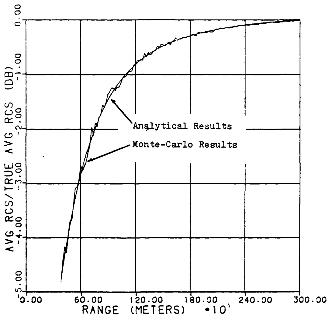
Fig. VIII-1. Average Measured RCS Normalized by the True Average RCS versus Range for an Uniformly Distributed Target (L=18.28m, 3 db Beam-width=1.18 deg)
