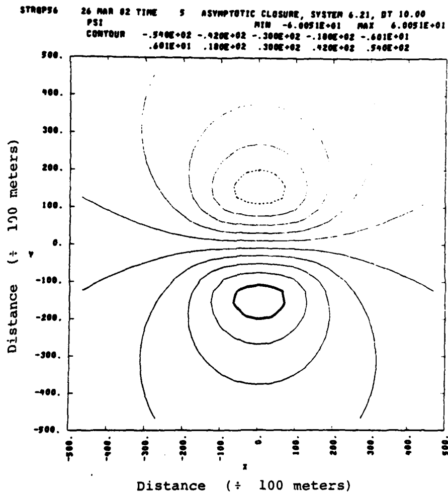
Figure 2-21. Results of the first potential solution step. Free space boundary conditions have been implemented.
