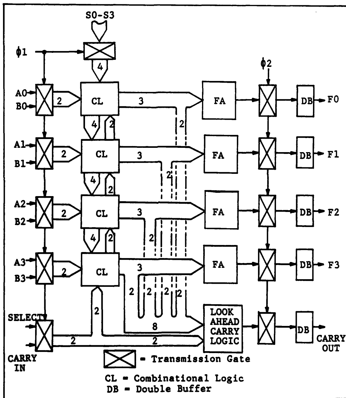
Figure IV-1 4-Bit ALU Block Diagram
