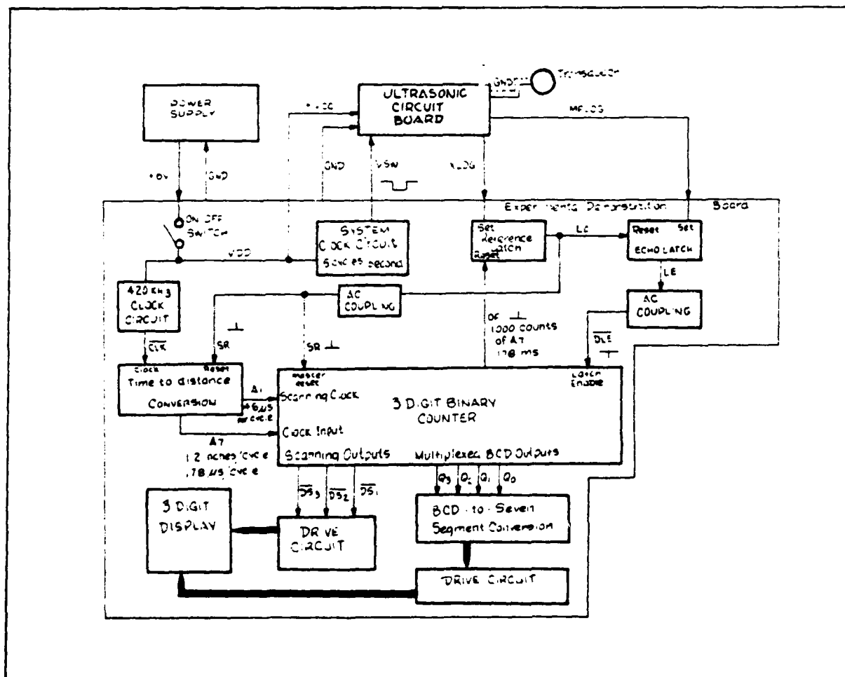
FIGURE 18. BLOCK DIAGRAM
