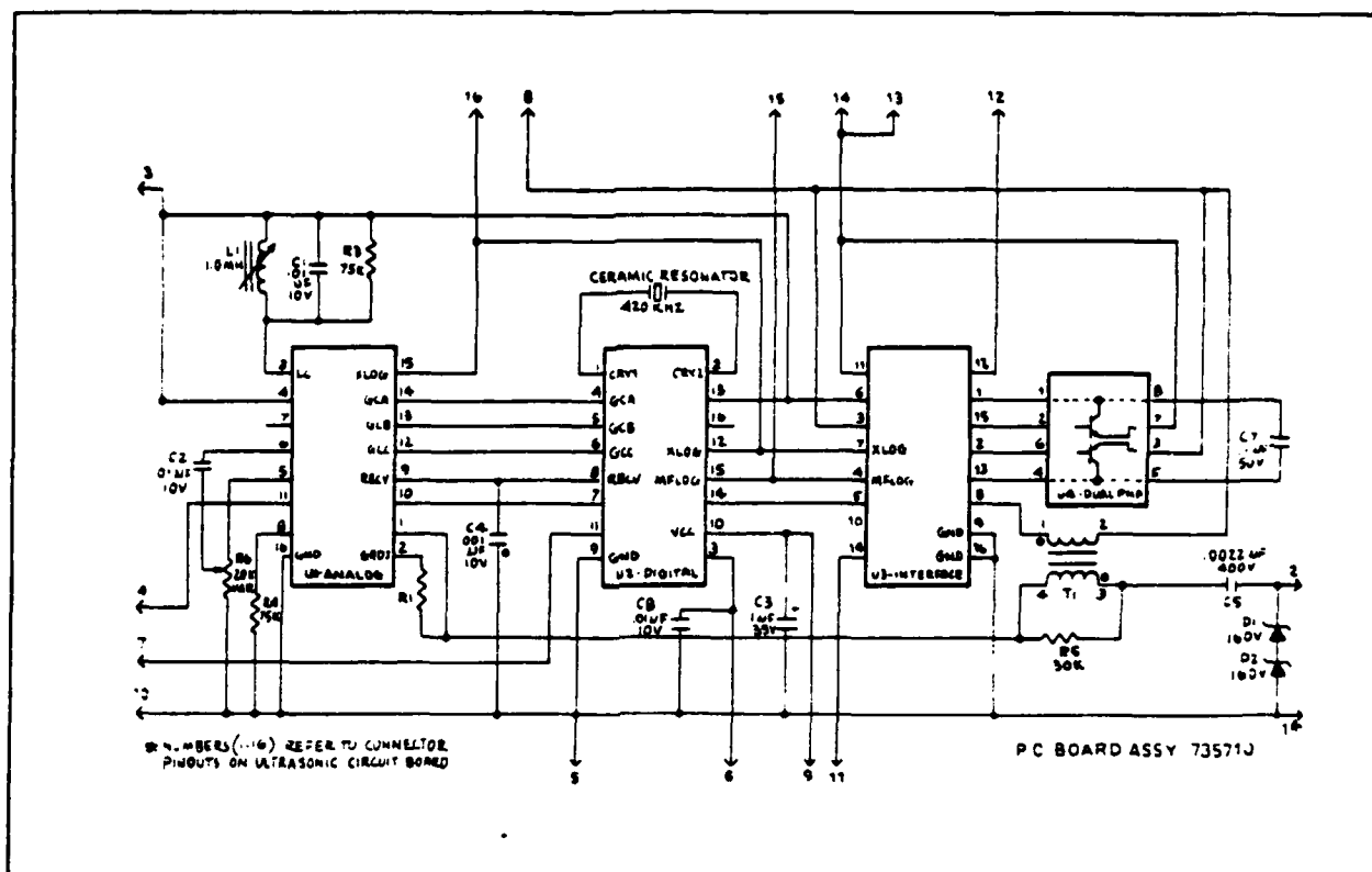
FIGURE 6. ULTRASONIC CIRCUIT BOARD SCHEMATIC (MODIFIED)
