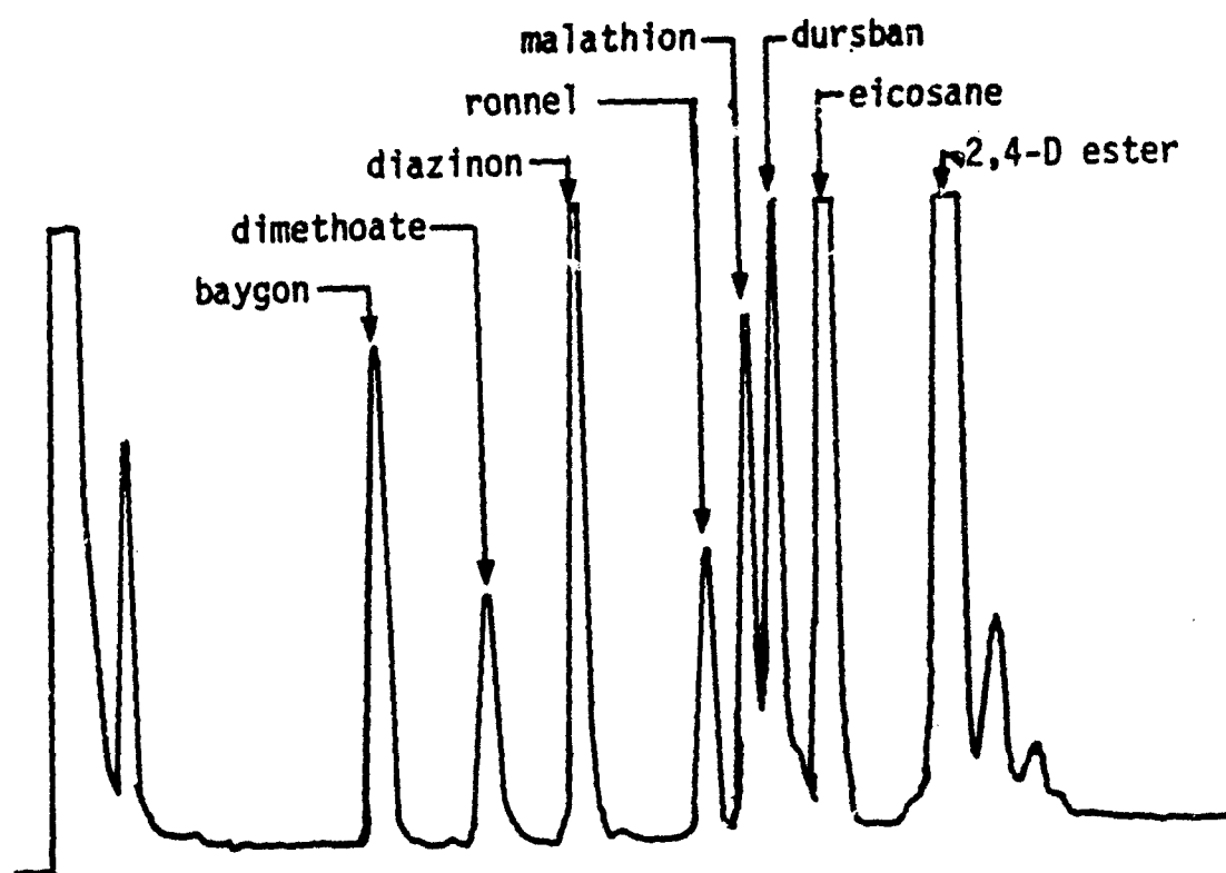
Figure 5. Gas chromatogram showing separation of seven pesticides. Conditions: 6', 3% OV-1 on GAS CHROM Q, 100-200 mesh, 160^{\circ} \xrightarrow{16^{\circ}/\text{min}} 240^{\circ}\text{C}.
