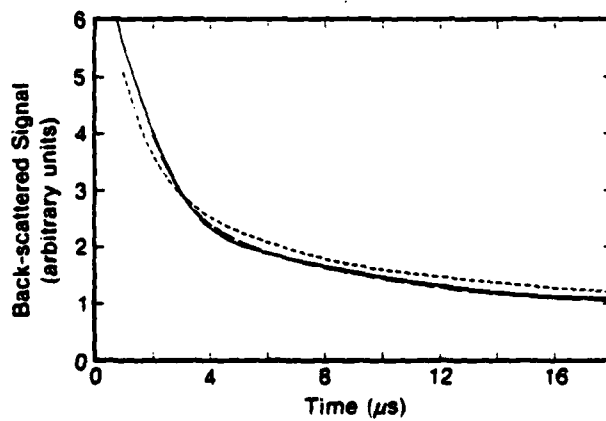
Figure 6. (a) Back-scattering radiometry signal for a piece of 107 \mu\text{m} thick Co-Netic magnetic steel. (b) Theoretical fits of (a) using Eq. (19) (long-dash line) and Eq. (11) (short-dash line). The solid line is the true experimental infrared signal obtained by subtracting the two curves in (a).
