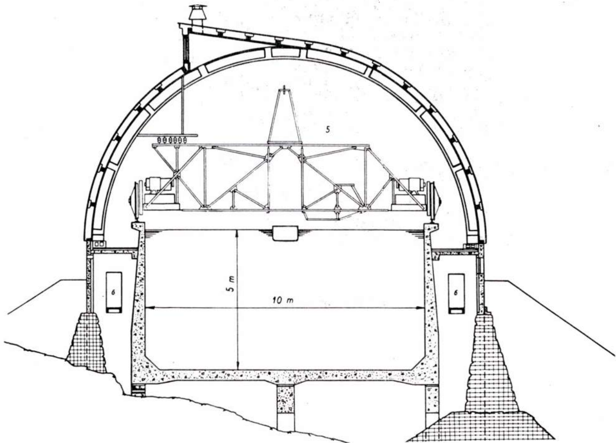
Figure 1 - Main Towing Tank at the Swedish Maritime Research Centre (From Edstrand 4 )
