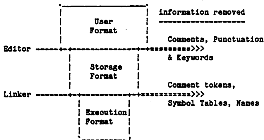
Figure 3: Storage Format Conversion.
