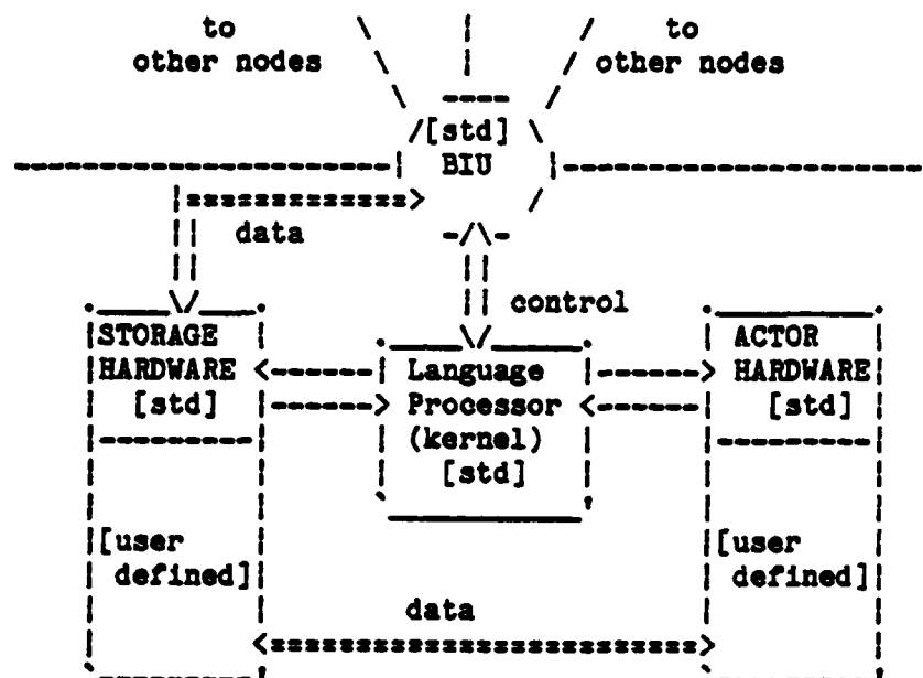
Figure 4: A Multiprocessing Node.
