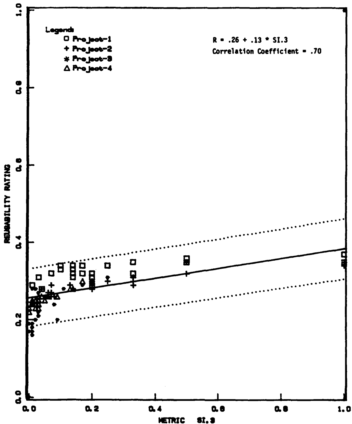
Figure C-11 : Reusability Rating vs. Metric SI.3
