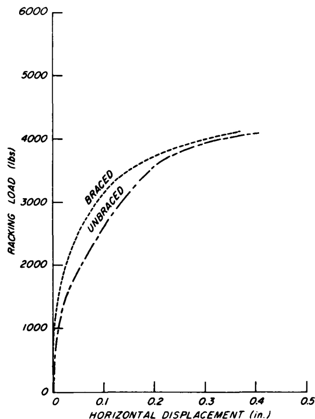
Figure 8.—Comparison of racking performance for braced versus unbraced 24-foot-long walls with vertically applied 1/2-inch gypsum wallboard. (M151740)
