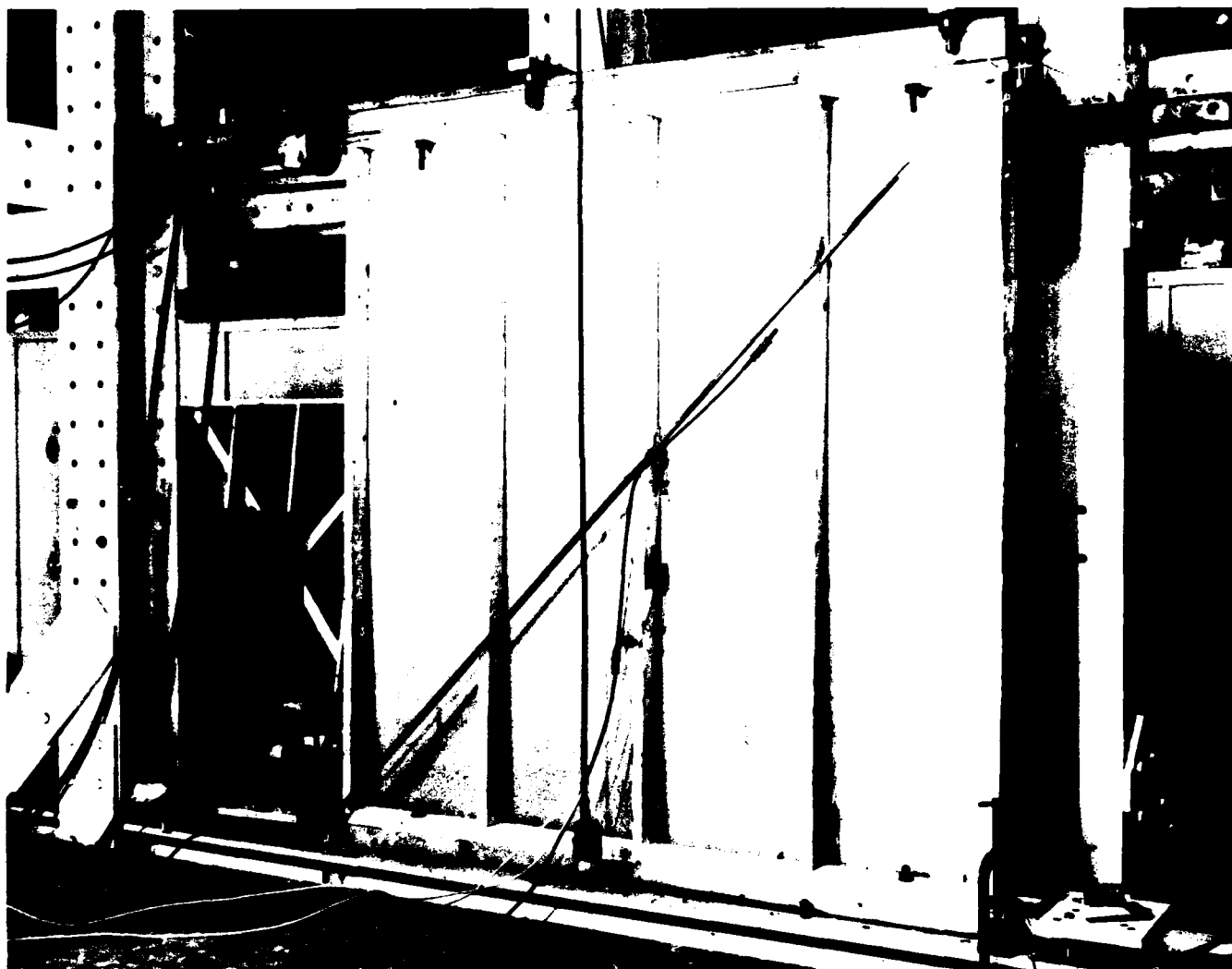
Figure 1.—Typical test setup showing an 8 by 8 wall with 2 by 4 studs spaced 24 inches O.C. with the cable holddown at the lower left and a hydraulic loading cylinder at the upper left corner. (M147997)
