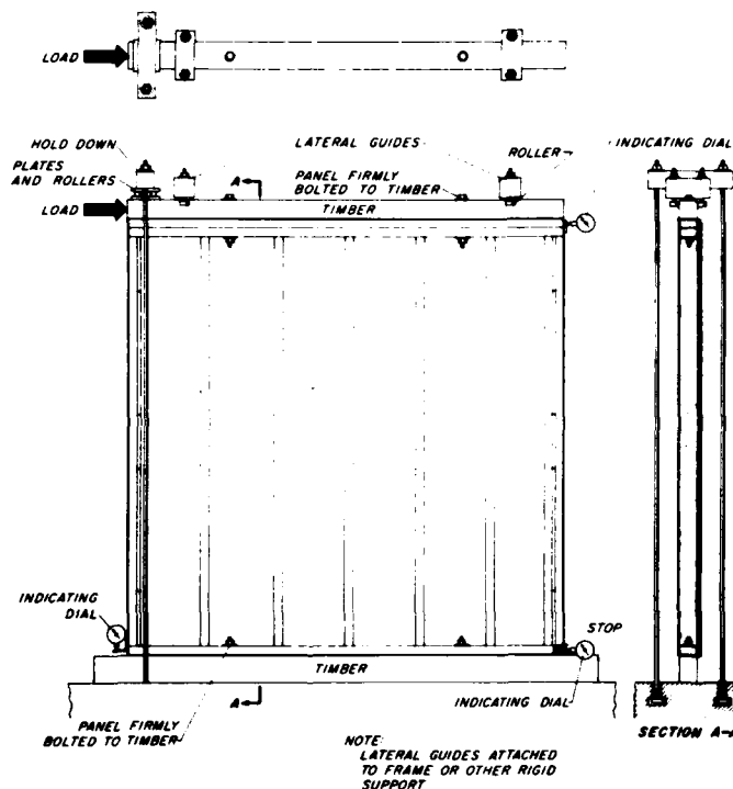
Figure A-1.—Standard ASTM E 72 test assembly. (M123922)
