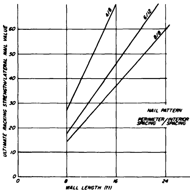
Figure A-3.—Dependence of racking strength on nailing pattern. Plots compare the strength versus length relationship for three nailing patterns predicted using the energy model for wall racking (23). (M151720)
