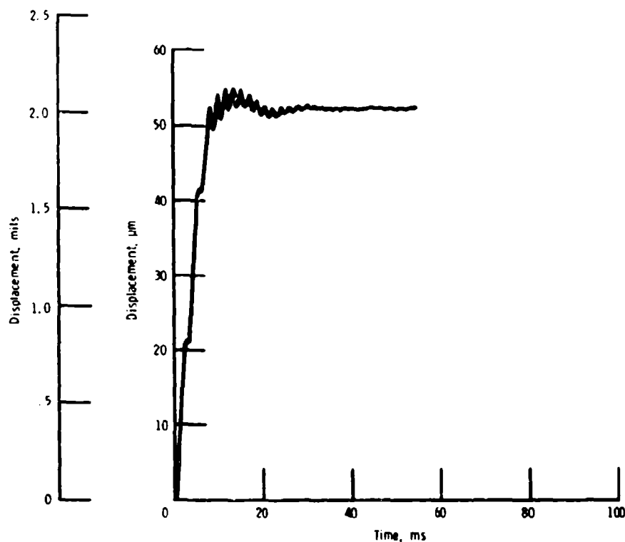
Figure 10. - Amplitude of displacement of center disk as function of time after blade loss for abradable model (low-energy case).
