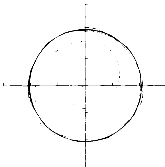
Figure 11. - Orbit of center disk after blade loss for abradable model (low-energy case). (Full scale equals 75\text{ }\mu\text{m} (3 mil).)
