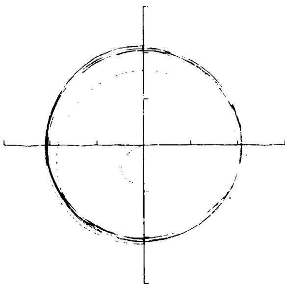
Figure 5. -- Orbit of center disk after blade loss for smearing model (low-viscosity case). (Full scale equals 75 \mu\text{m} (3 mil).)
