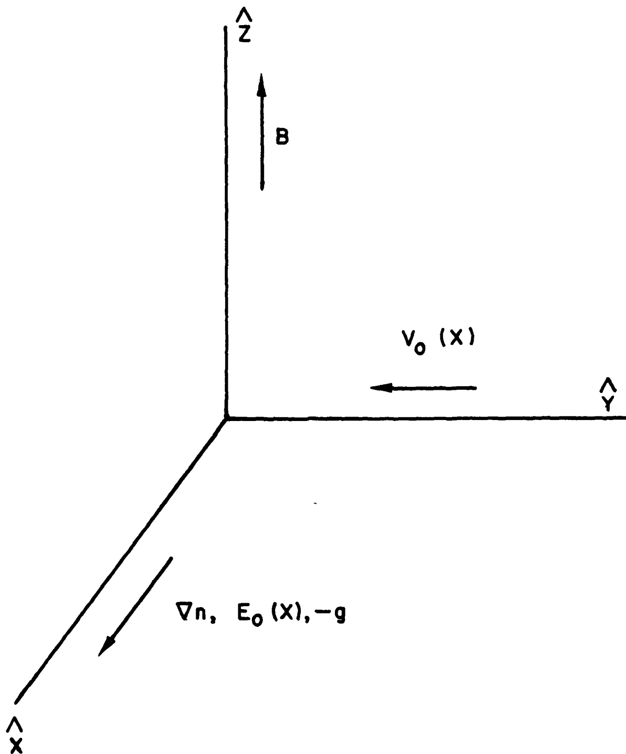
Figure 1. Plasma configuration and slab geometry used in the analysis.
