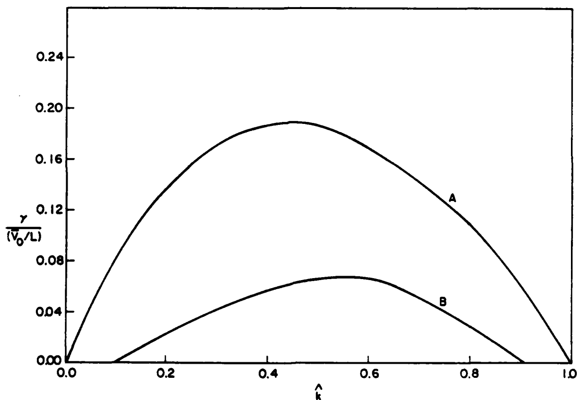
Figure 5. Growth rate \gamma/(\bar{V}_0/L) vs \hat{k} \equiv k_y L for the Kelvin-Helmholtz mode. Curve A represents the case \hat{v} = 0 , \nabla n = 0 ; Curve B represents the case \hat{v} = 0 , and n_0 = \bar{n}_0 \exp(-x/L) .
