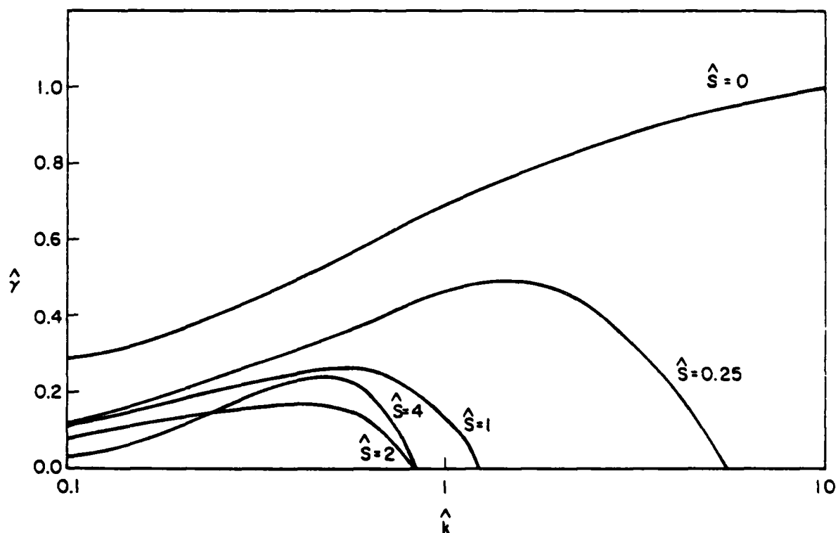
Figure 10. Study of the growth rate as a function of the mode number in the collisional domain \hat{\gamma} vs \hat{k} and for \hat{s} = 0, 0.25, 1.0, 2.0 , and 4.0 . We have used \chi_0 = -0.55 , \hat{v} = 0.5 , and \epsilon = 0.8 .
