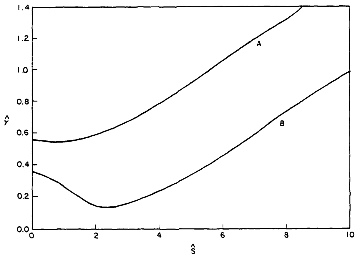
Figure 12. Study of \hat{\gamma} versus \hat{s} , for \hat{k} = 0.45 where the Kelvin-Helmholtz instability has maximum growth rate. Curves A and B refer to \hat{v} = 0.0 and 0.5 respectively.
