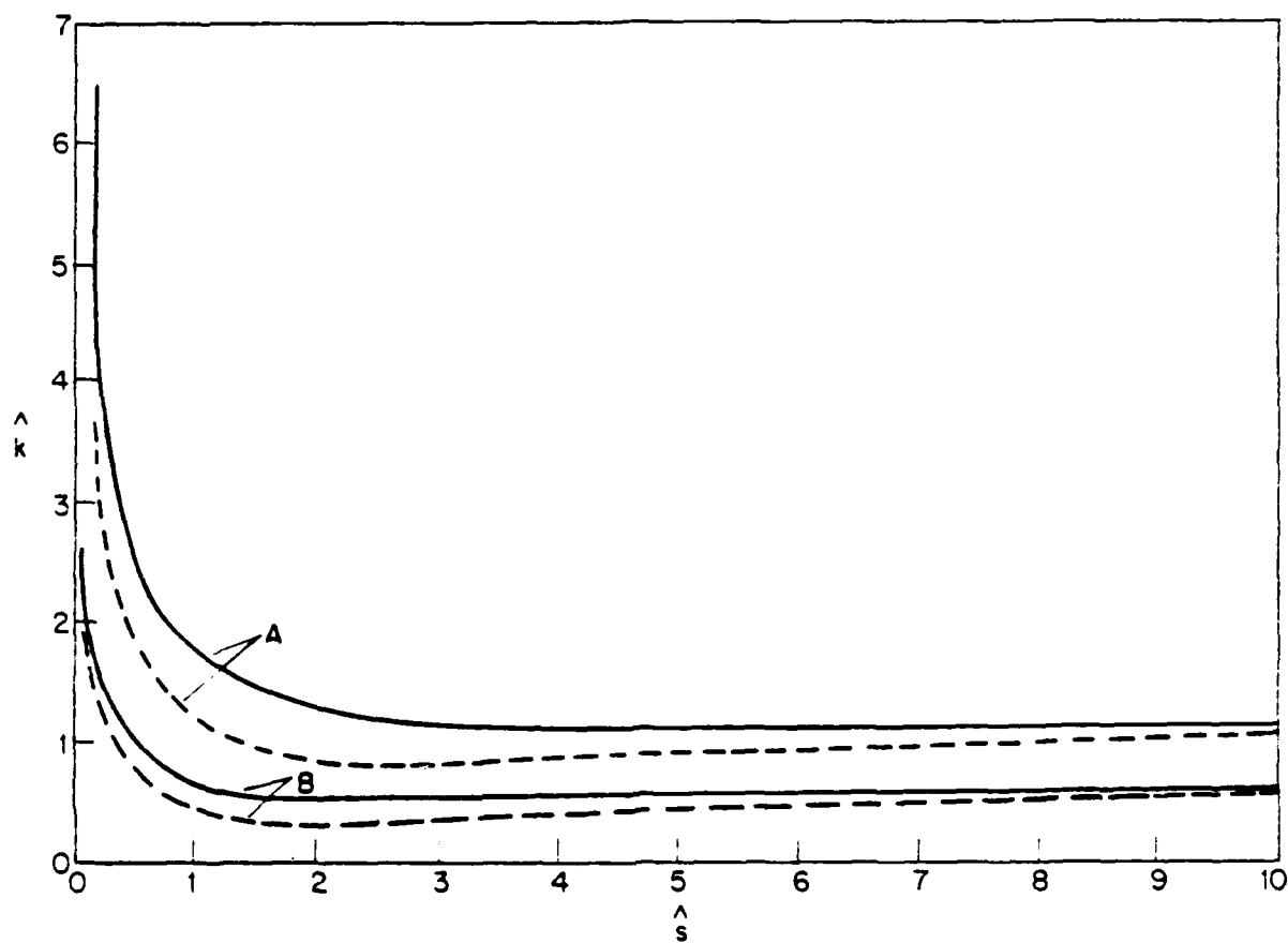
Figure 13. Plots of \hat{k}_c (cut-off mode numbers) and \hat{k}_m (mode numbers where the growth rate maximizes) as a function of \hat{s} . The solid and dashed lines correspond to the collisionless and collisional ( \hat{\nu} = 0.5 ) cases respectively. Curves A and B refer to \hat{k}_c and \hat{k}_m , respectively.
