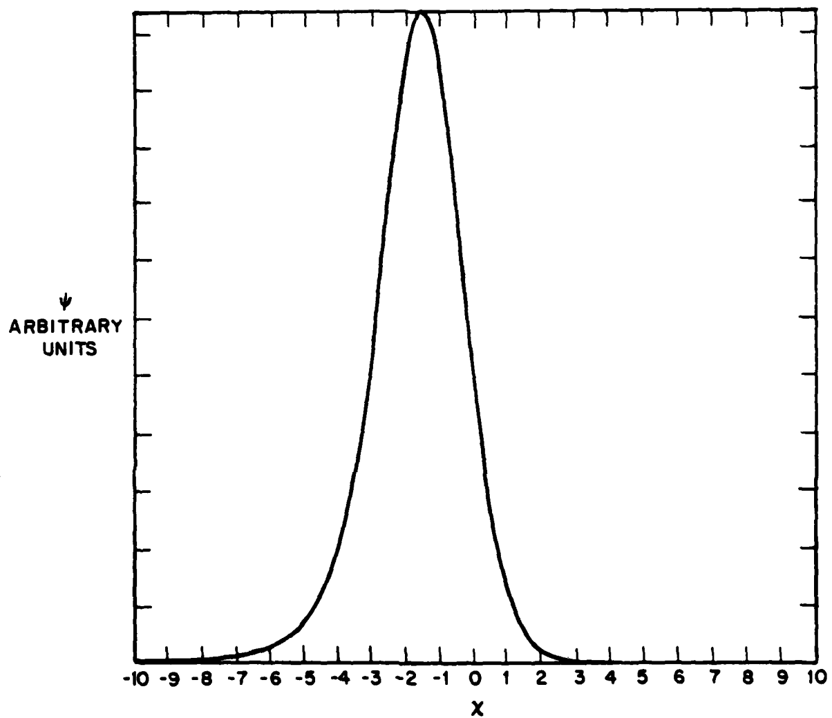
Figure 4. Plot of the wavefunction for \hat{\omega}_r = 0 , \hat{\gamma} = .693 , \hat{k} = 1.0 , and for the collisional case and density profile used in Fig. 2.
