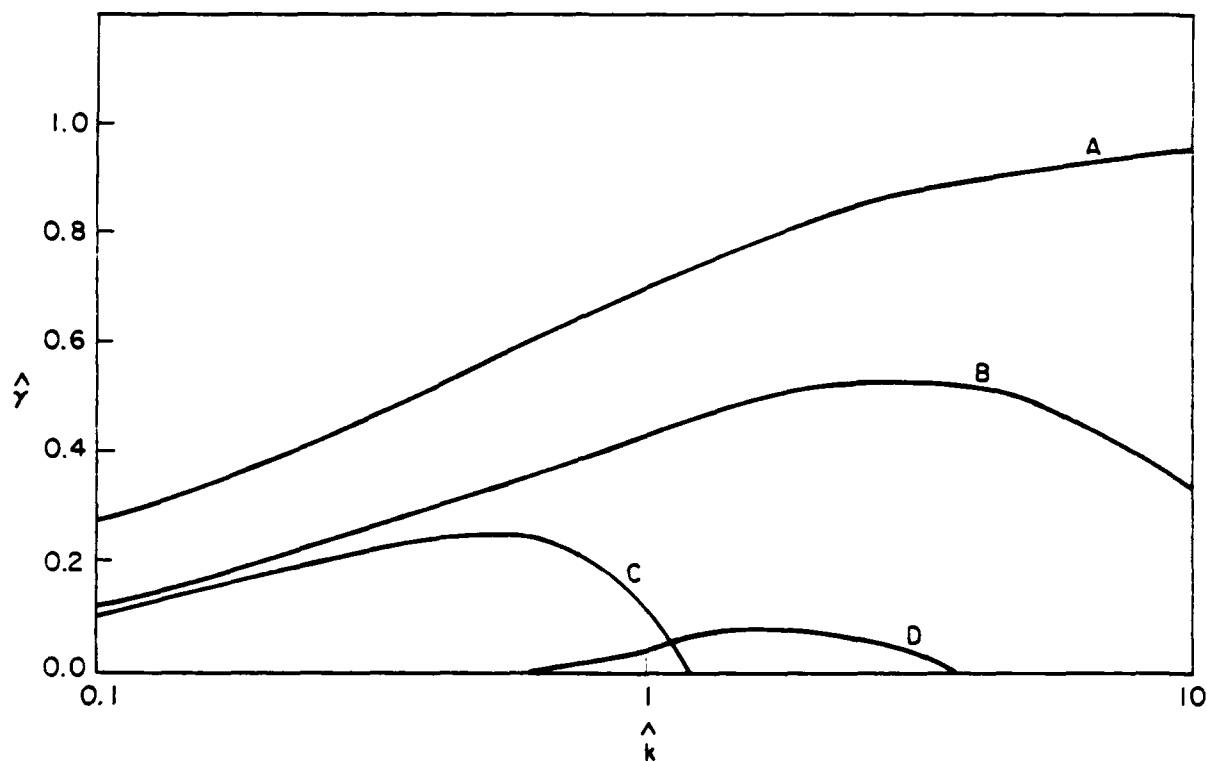
Figure 9. Variation of the dispersion curve, \hat{\gamma} vs \hat{k} , for different transition points ( \chi_0 ), of the flow velocity profile given by V = \bar{V}_0 \tanh(\chi - \chi_0) for \chi_0 = -0.5, -2.0 , and 0.0 . Parameters used are \hat{s} = 1, \hat{v} = 0.5, \epsilon = 0.8 , and for the profiles given in Eqs. (39) and (40). Curve A corresponds to shear-free case ( \hat{s} = 0 ) where as curves B, C, and D correspond to \hat{s} = 1.0 and \chi_0 = -2.0, -0.55 , and 0.0 respectively.
