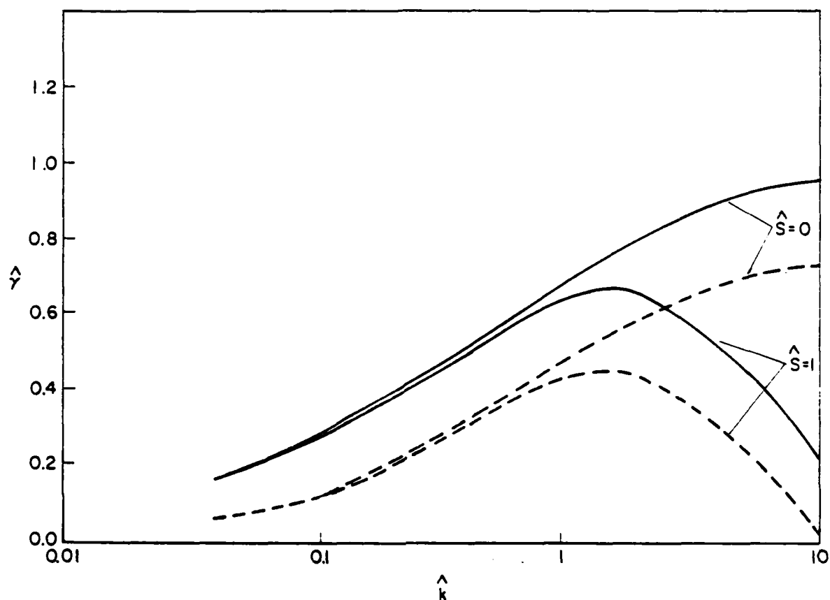
Figure 6. Growth rate \hat{\gamma} vs \hat{k} for the generalized Rayleigh-Taylor instability. Solid lines represent the collisionless case ( \hat{v} = 0.0 , \hat{s} = 0.0 , and 1.0 ); dashed lines represent the collisional case ( \hat{v} = 0.5 , \hat{s} = 0.0 , and 1.0 ). The profiles used are the self-consistent profiles, Eqs. (34) and (35).
