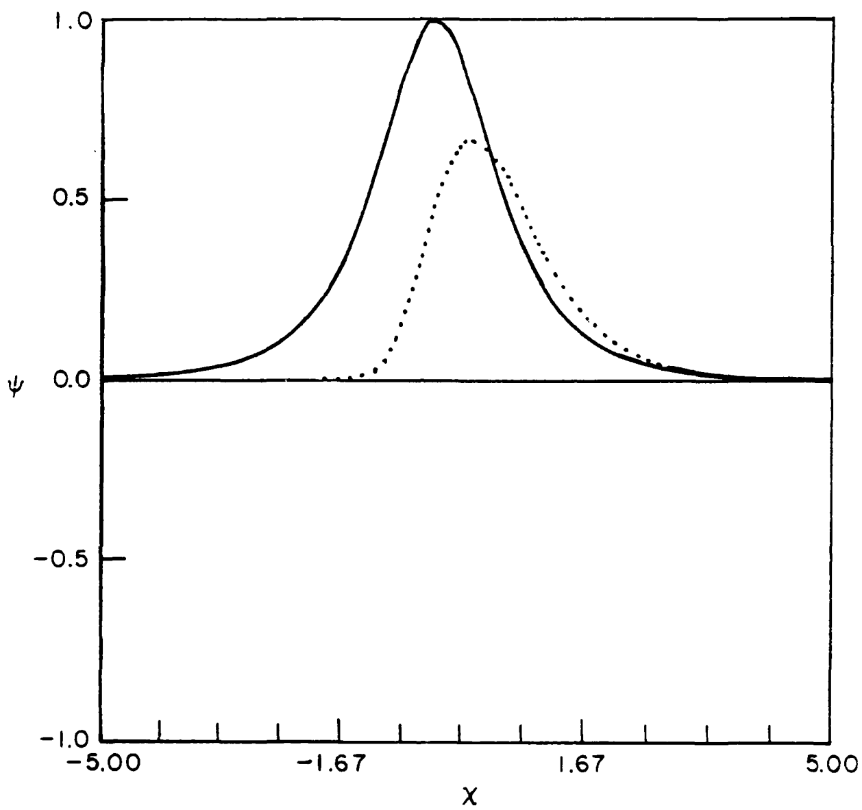
Figure 8. Real and imaginary parts of the wavefunction, corresponding to Fig. 6 (dotted line, \hat{s} = 1.0 ) and \hat{k} = 0.5 .
