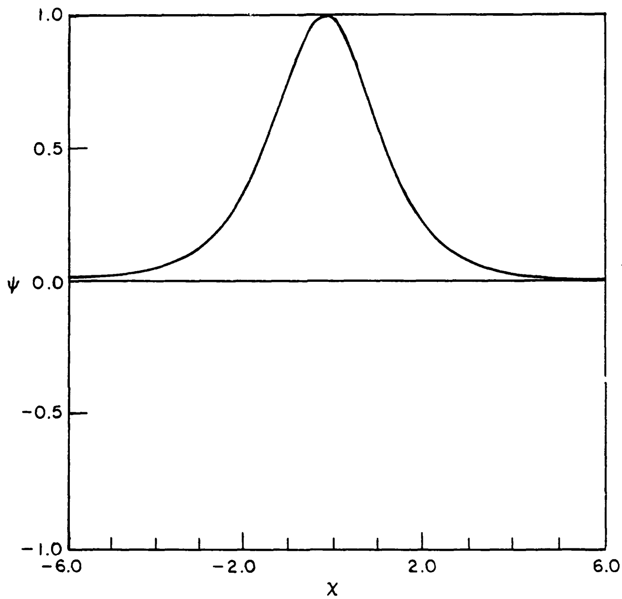
Figure 7. The wave function corresponding to Fig. 6 (solid line; \hat{s} = 0 ) and \hat{k} = 0.5 .
