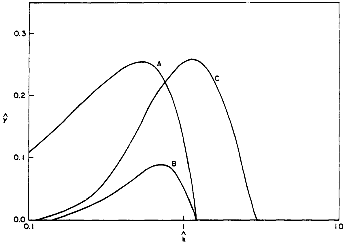
Figure 14. Normalized growth rate versus the normalized wavenumbers for the case of a spatially dependent collision frequency. The density and velocity profiles are given in Eqs. (39) and (40). The parameters used are \varepsilon = 0.8 , \chi_0 = -0.55 , and \hat{v} = 0.5 . Curve A refers to constant collision frequency, \hat{v} = 0.5 , and \hat{s} = 1.0 . Curves B and C refer to \hat{v} = 0.5 \exp(-\chi) and for \hat{s} = 1.0 and 0.5 respectively.
