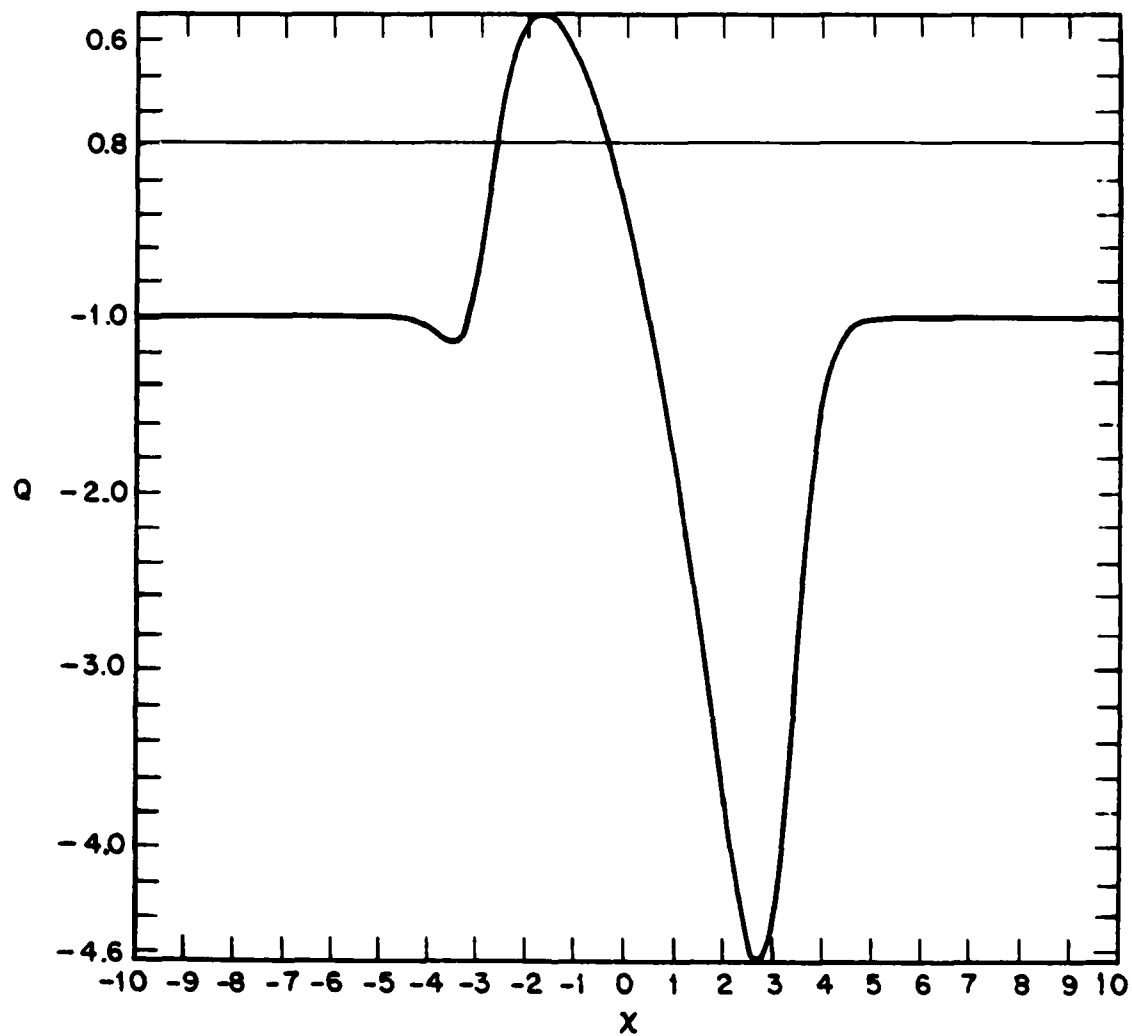
Figure 3. Plot of potential term, Q(\chi) , as a function of \chi for the collisional case and density profile used in Fig. 2.
