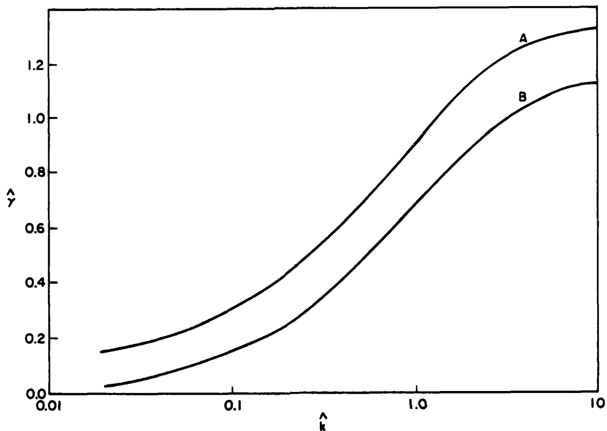
Figure 2. Normalized growth rate \hat{\gamma} \equiv \gamma/\sqrt{g/L} vs \hat{k} \equiv k_y L for the Rayleigh-Taylor instability. Curve A represents the collisionless mode ( \hat{v} = 0 ); curve B represents the collisional mode ( \hat{v} = 0.5 ), where \hat{v} = v/\sqrt{g/L} . The density profile used is a Gaussian-like profile n_0 e^{-x^2/2L^2} + \Delta n , with \Delta n/n_0 = 0.01 .
