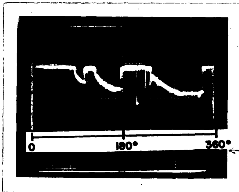
FIGURE 12a. 125.7 rad/sec
