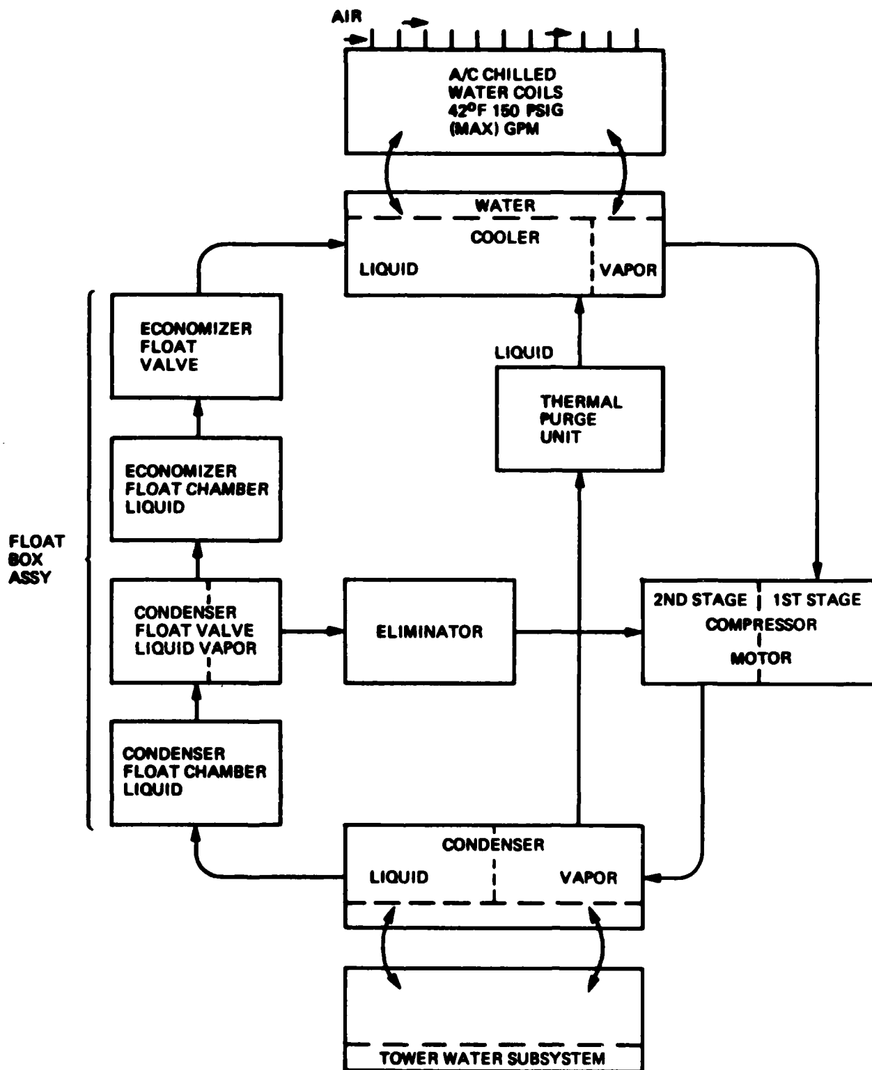
Figure 6.1-2. Functional Diagram of Chilled Water Air Conditioning
