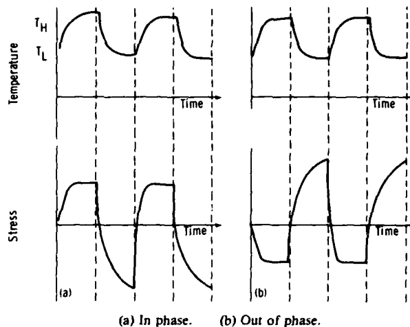
Figure 2. - Schematics of in-phase and out-of-phase thermomechanical fatigue cycles.
