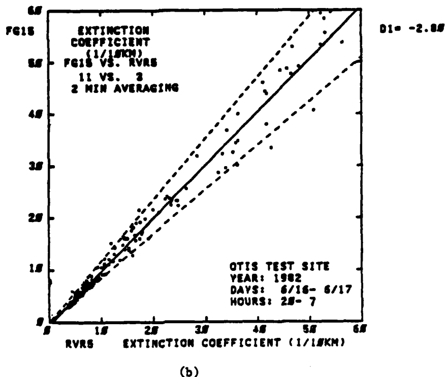
FIGURE 5-20. SCATTER PLOTS FOR EVENT #1: FOG-15 (SN 015) versus 1000-FOOT BASELINE RVR 500: NEW CALIBRATION: (a), (b) EXTINCTION COEFFICIENT: (c), (d) VISIBILITY.
