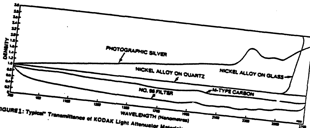
FIGURE : Typical* Transmittance of KODAK Light Attenuator Materials.
