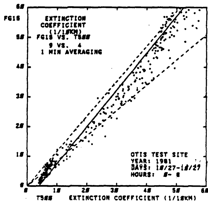
FIGURE 5-27. FOG RESPONSE OF EARLIER MODEL FOG-15 COMPARED WITH THE 500-FOOT RVR 500.
