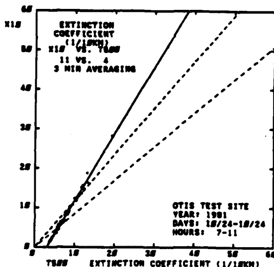
Fig. 2. Comparison of forward-scatter sensor measurements with transmissometer measurements in pure rain.
