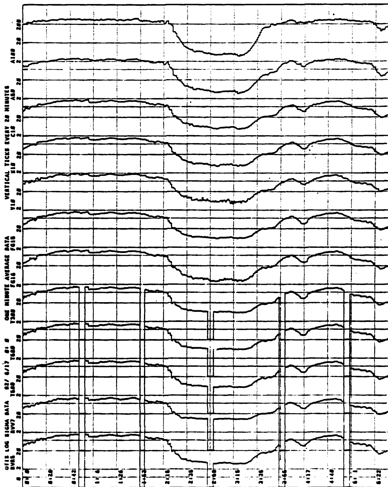
FIGURE 5-2. EXTINCTION COEFFICIENT STRIPCHART FOR PART OF EVENT #1. The dropouts for the Transmissometers Occur During the Background check.
