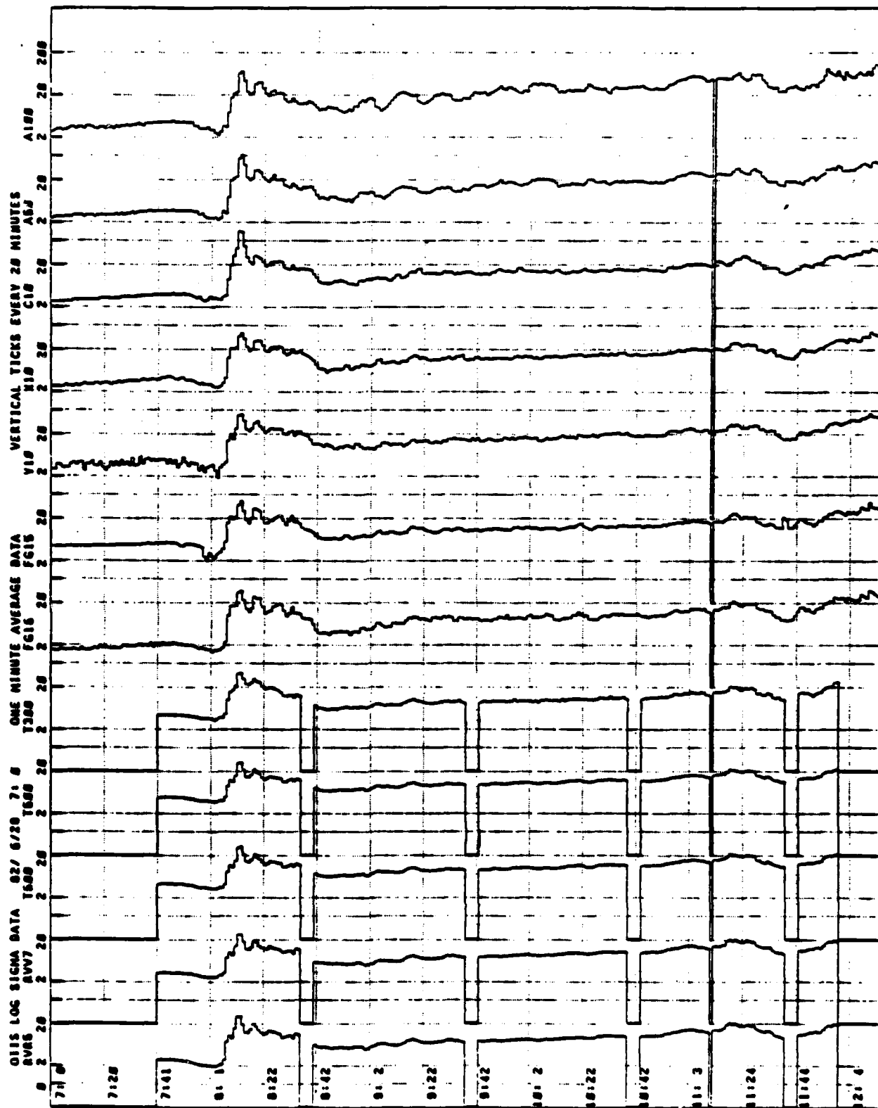
FIGURE 5-8. EXTINCTION COEFFICIENT STRIPCHART FOR EVENT #2 (0900-1200).
