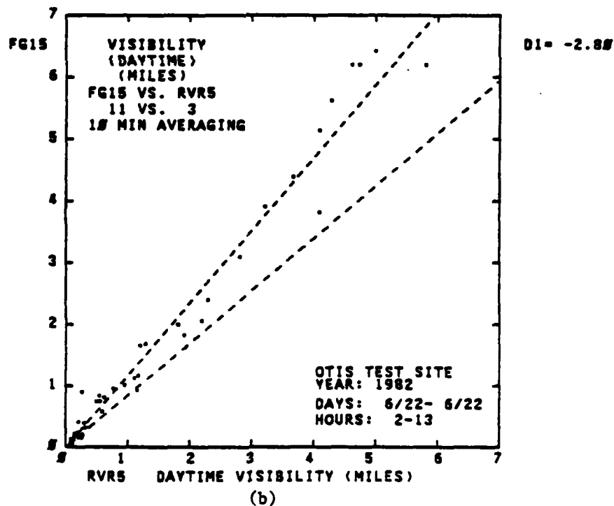
FIGURE 5-24. VISIBILITY SCATTER PLOTS FOR RAPIDLY VARYING EVENTS FOG-15 versus 1000-FOOT RVR 500.
