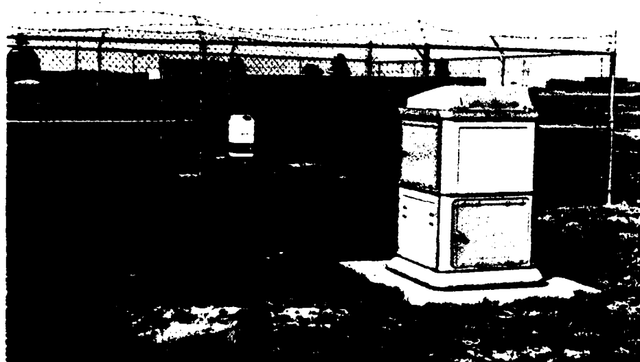
FIGURE 3-4. IMPULSPHYSICS LD-WHL CEILOMETER (a) ALONE (b) WITH ROTATING BEAM CEILOMETER RECEIVER IN FOREGROUND
