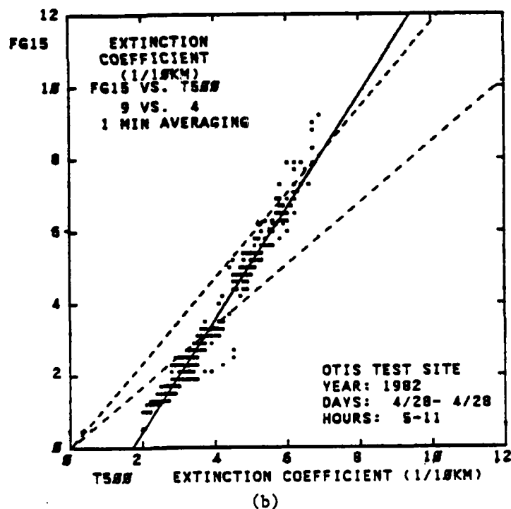
FIGURE 5-26. SCATTER PLOTS COMPARING THE FOG-15 RESPONSE TO THE TRANSMISSOMETER RESPONSE FOR A FOG/RAIN EVENT: HOURS (a) 1300-1800, (b) 0500-1100.
