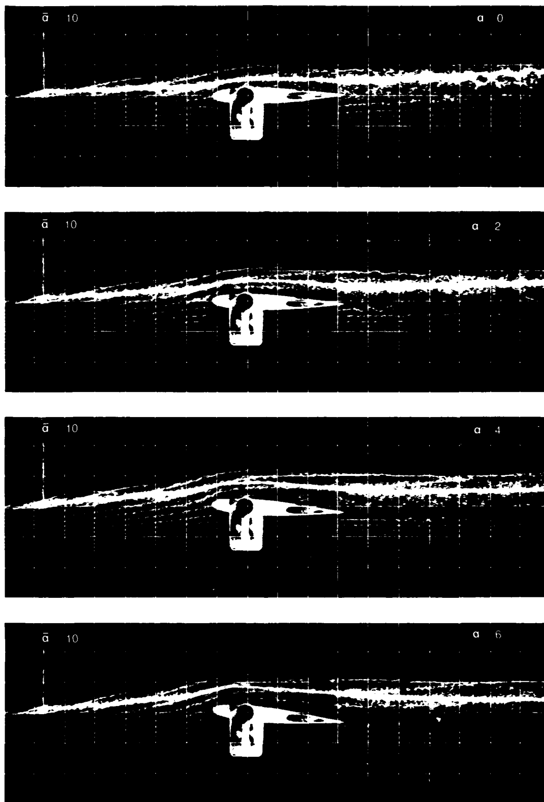
Figure 12.— Visualization of flow at Re = 120,000 with generator on centerline and set at \bar{\alpha} = 10^\circ (strong-vortex case).
