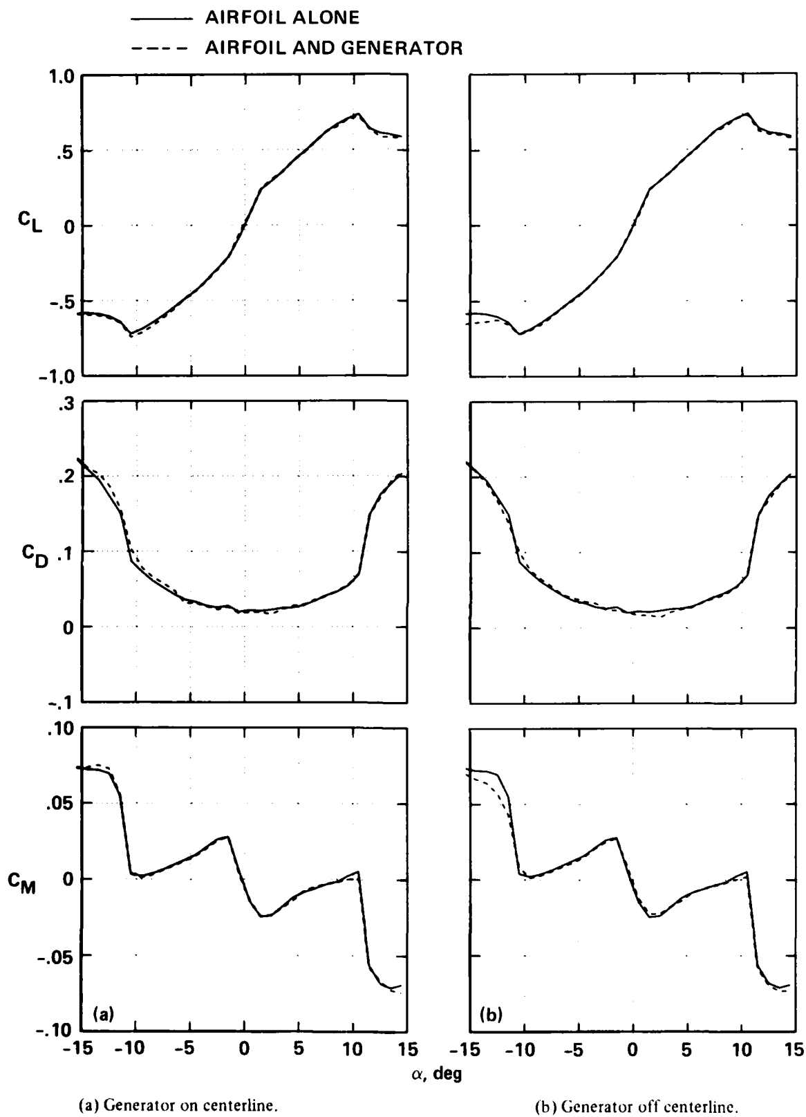
Figure 22.— Generator wake effects on airfoil loads when \tilde{\alpha} = 0^\circ .
