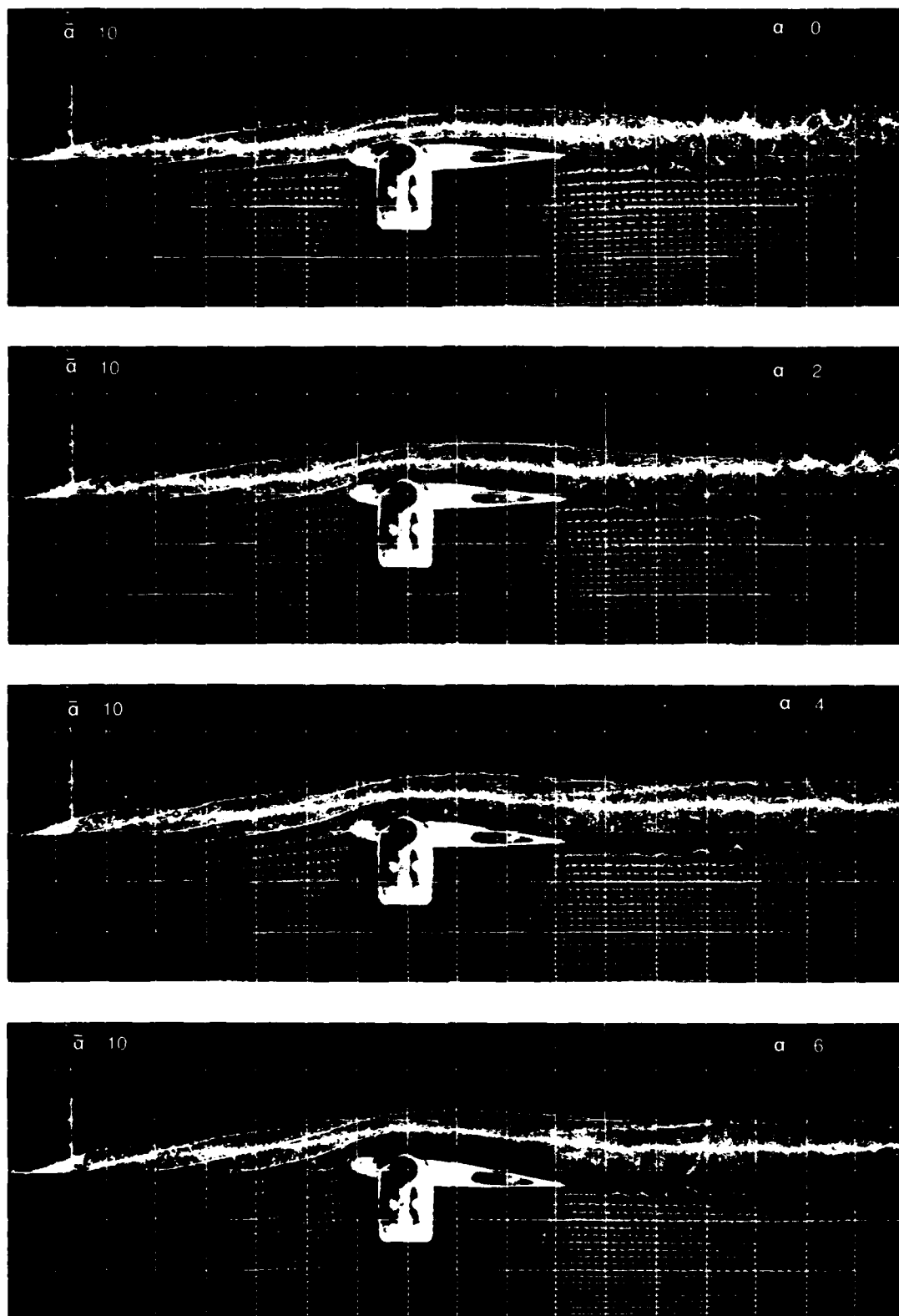
Figure 9.— Visualization of flow at Re = 60,000 with generator on centerline and set at \bar{\alpha} = 10^\circ (strong-vortex case).
