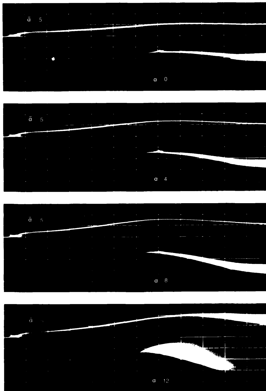
Figure 20.— Long-exposure visualization of flow at Re = 120,000 with generator off centerline and set at \tilde{\alpha} = 5^\circ (weak-vortex case).
