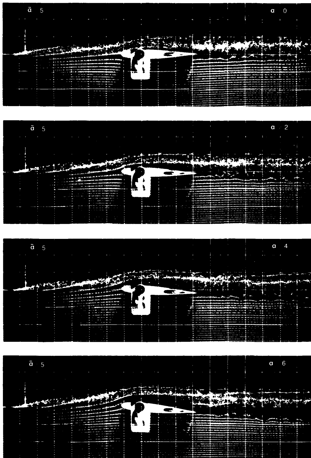
Figure 8. Visualization of flow at Re = 60,000 with generator on centerline and set at \alpha = 5^\circ (weak-vortex case).
