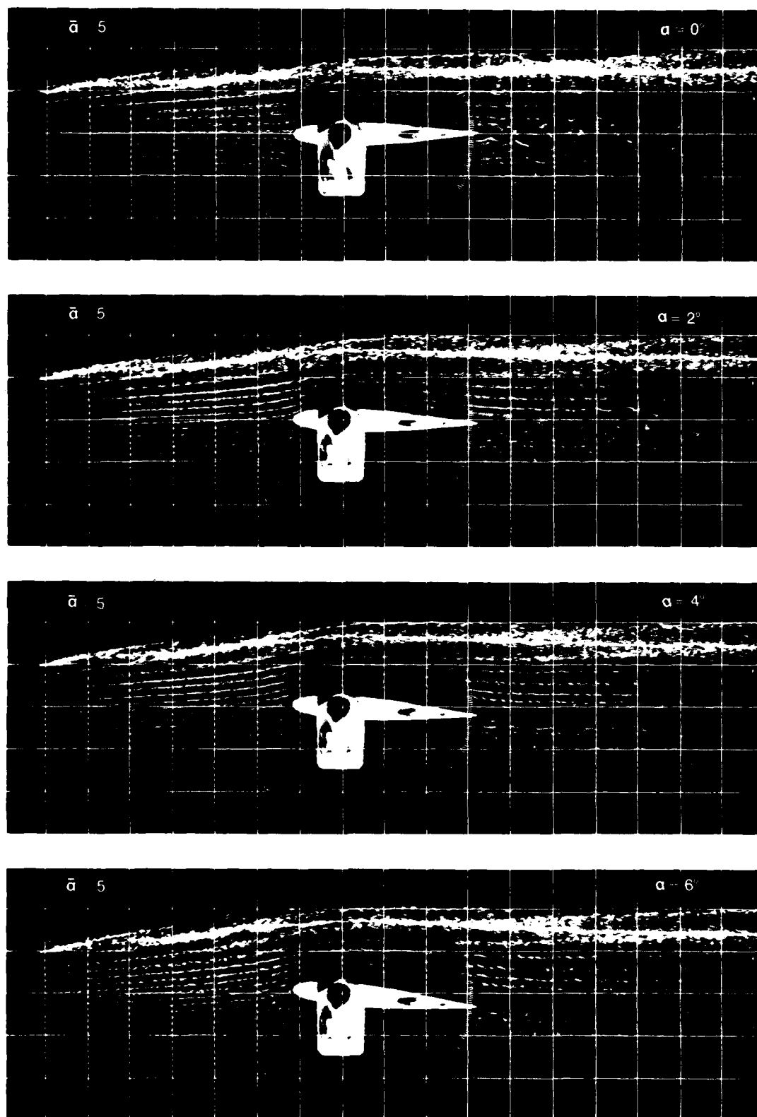
Figure 17. Visualization of flow at Re = 120,000 with generator off centerline and set at \bar{\alpha} = 5 (weak-vortex case).
