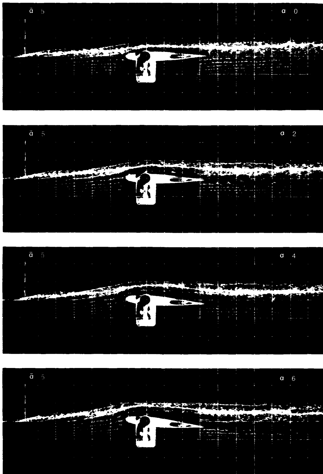
Figure 11.— Visualization of flow at Re = 120,000 with generator on centerline and set at \alpha = 5^\circ (weak-vortex case).
