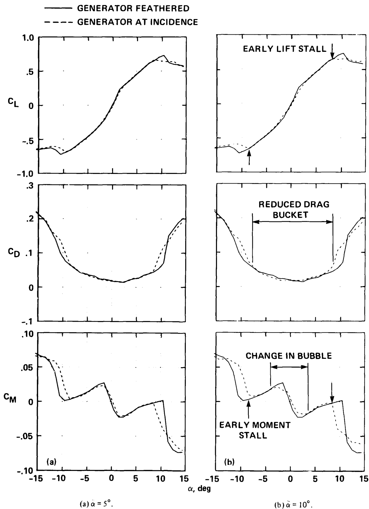
Figure 23.— Airfoil loads during vortex encounter with generator on centerline.
