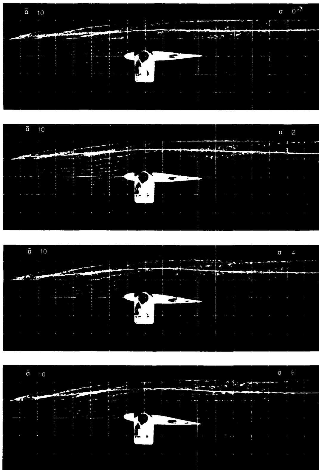
Figure 18.— Visualization of flow at Re = 120,000 with generator off centerline and set at \bar{\alpha} = 10^\circ (strong-vortex case).
