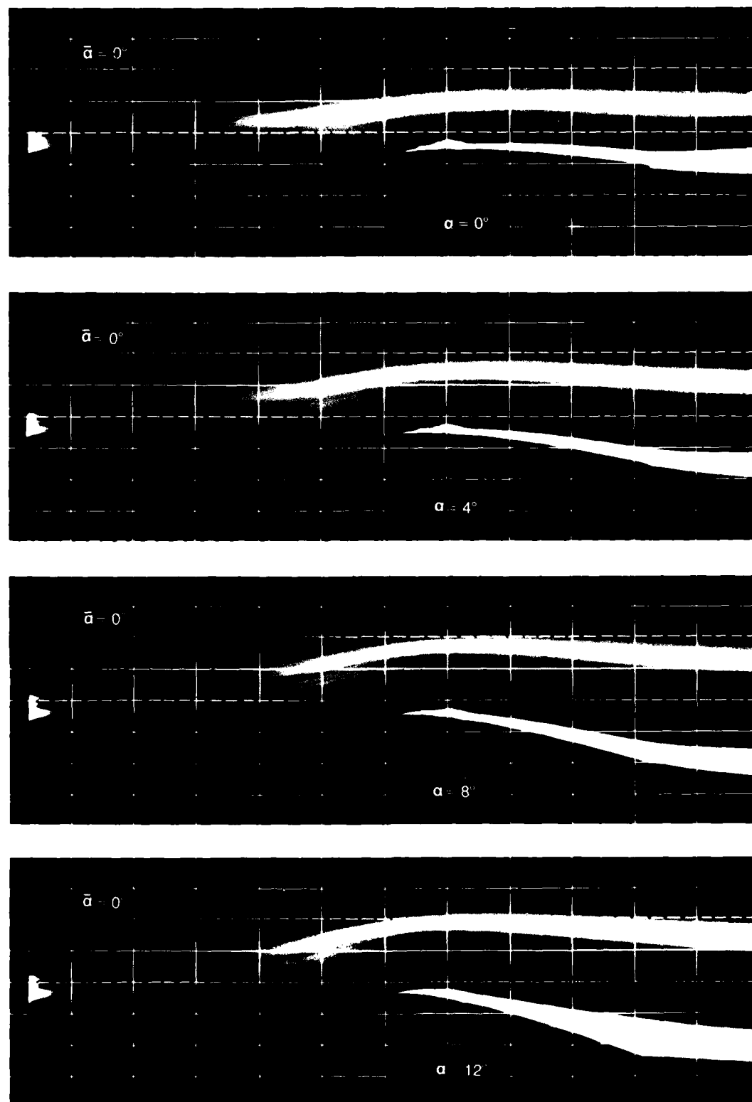
Figure 13. Long-exposure visualization of flow at Re = 120,000 with generator on centerline and set at \dot{\alpha} = 0^\circ (no-vortex case).
