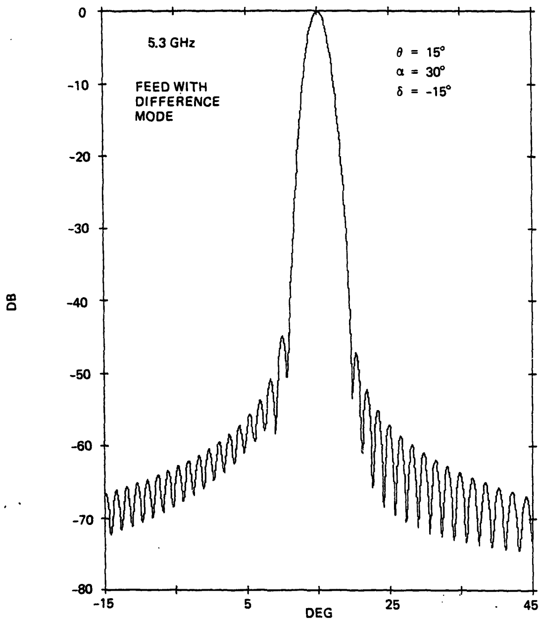
Figure 5-30. Azimuth Pattern of Antenna with Feed Difference Mode, \theta = 15^\circ
