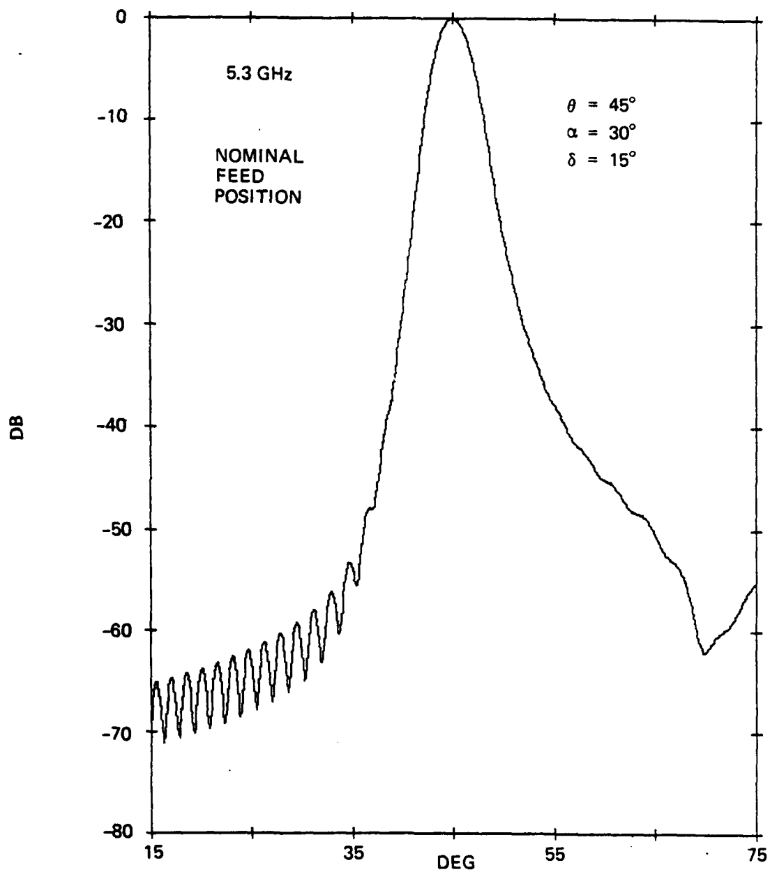
Figure 5-13. Azimuth Pattern of Antenna with Nominal Feed Position for \alpha = 30^\circ and \theta = 45^\circ
