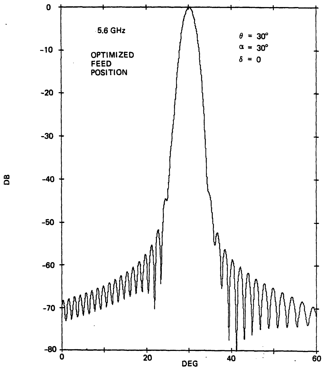
Figure 5-23. Azimuth Pattern of Antenna at 5.6 GHz with Optimized Feed Position, \theta = 30^\circ
