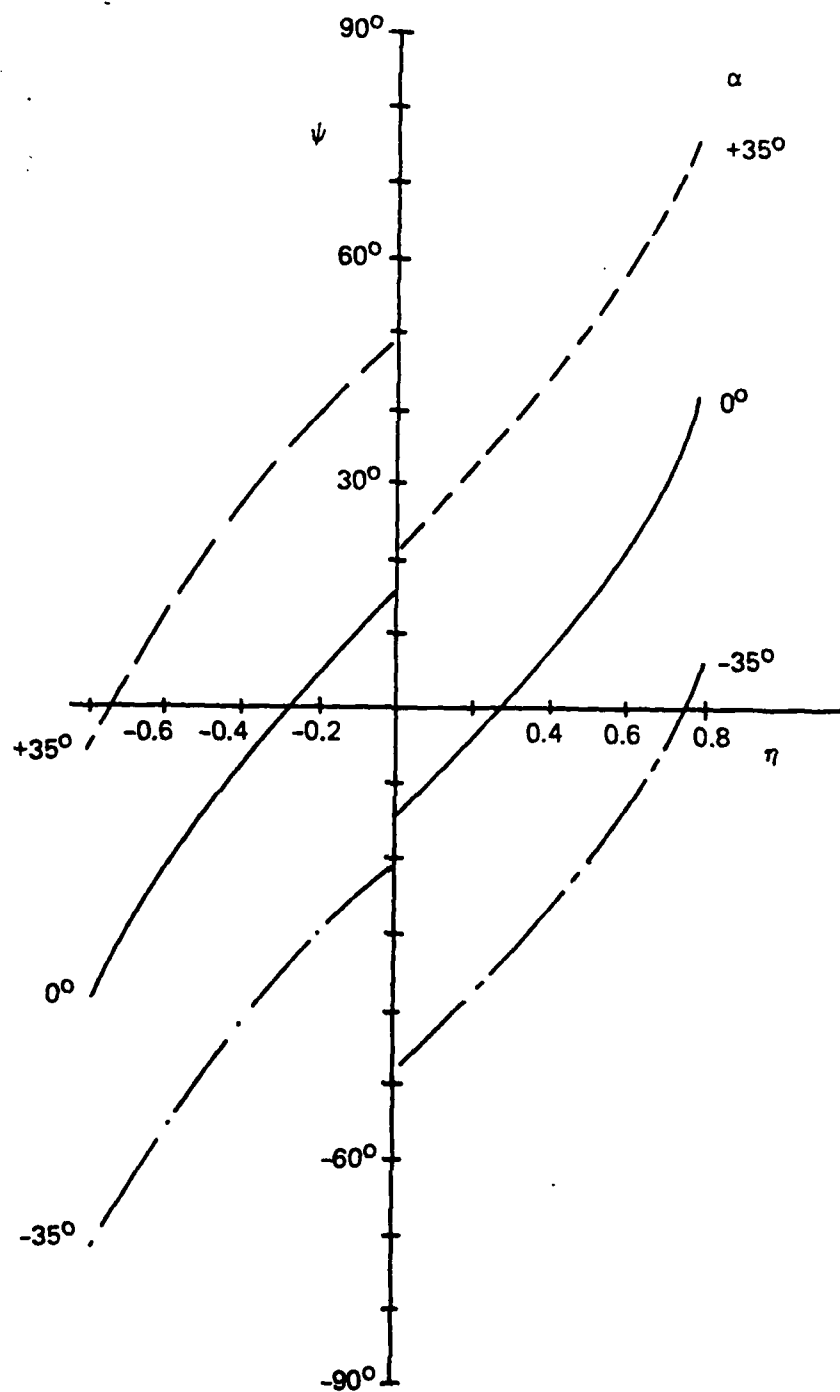
Figure 4-13. Incidence Angles for Outer Surface of Dimpled Lens
