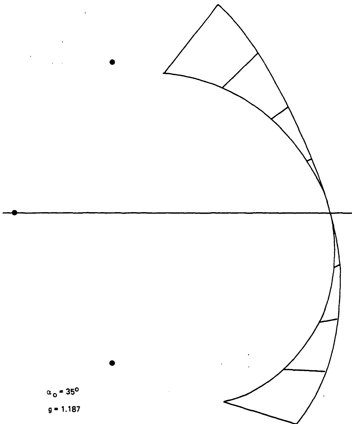
Figure 4-4. Hybrid Lens Contours
