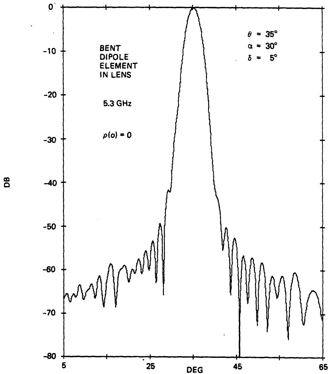
Figure 6-33. Azimuth Pattern of Antenna with Bent-Dipole Element, \alpha = 30^\circ , \delta = 5^\circ
