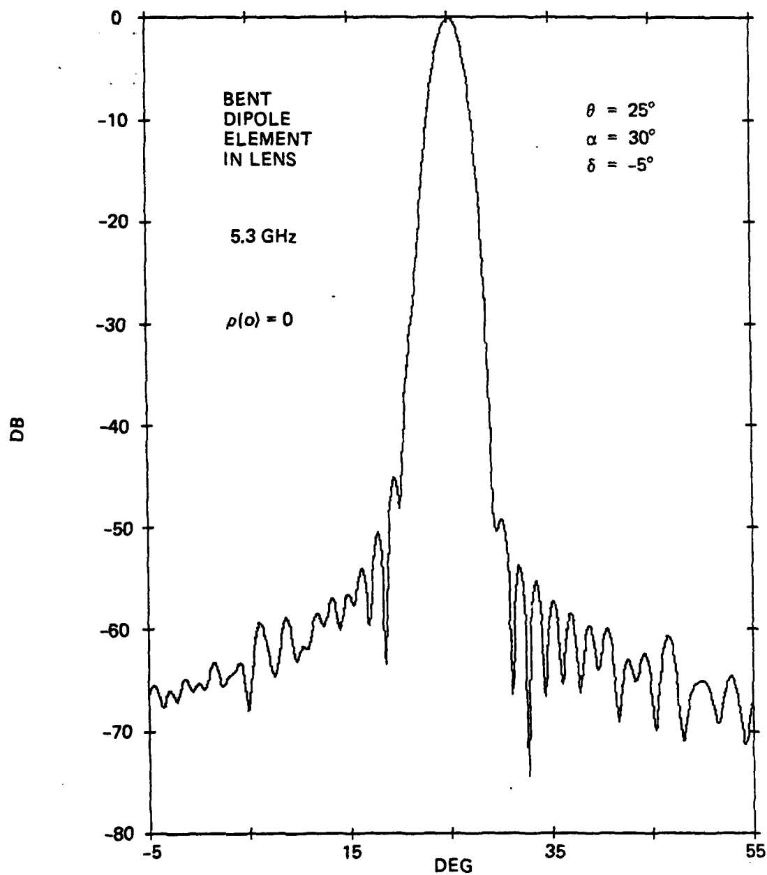
Figure 6-32. Azimuth Pattern of Antenna with Bent-Dipole Element, \alpha = 30^\circ , \delta = -5^\circ
