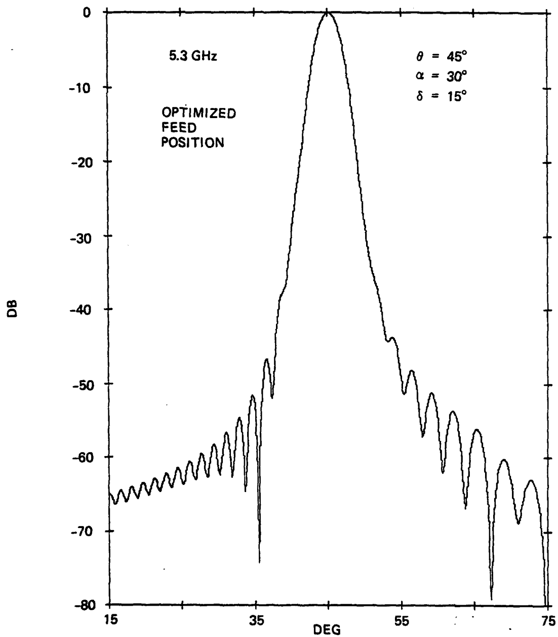
Figure 5-19. Azimuth Pattern of Antenna with Optimized Feed Position, \theta = 45^\circ
