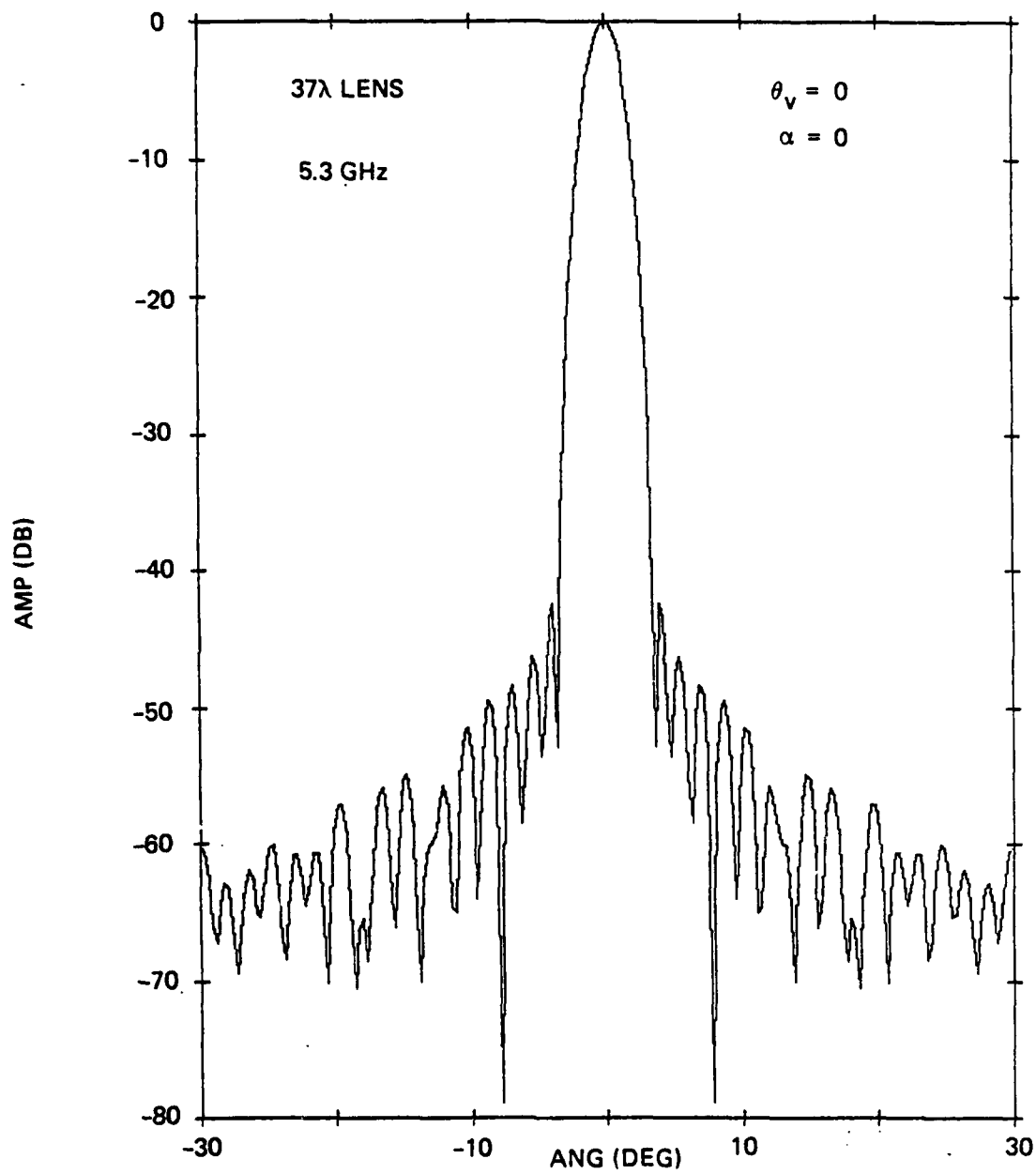
Figure 5-37. Elevation Pattern of Antenna, \theta_v = 0 , 37 \lambda Lens
