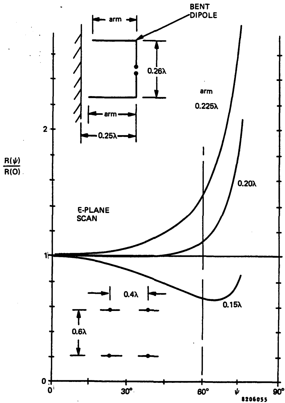
Figure 6-26. Bent Dipole Array Resistance vs Angle and Arm Length
