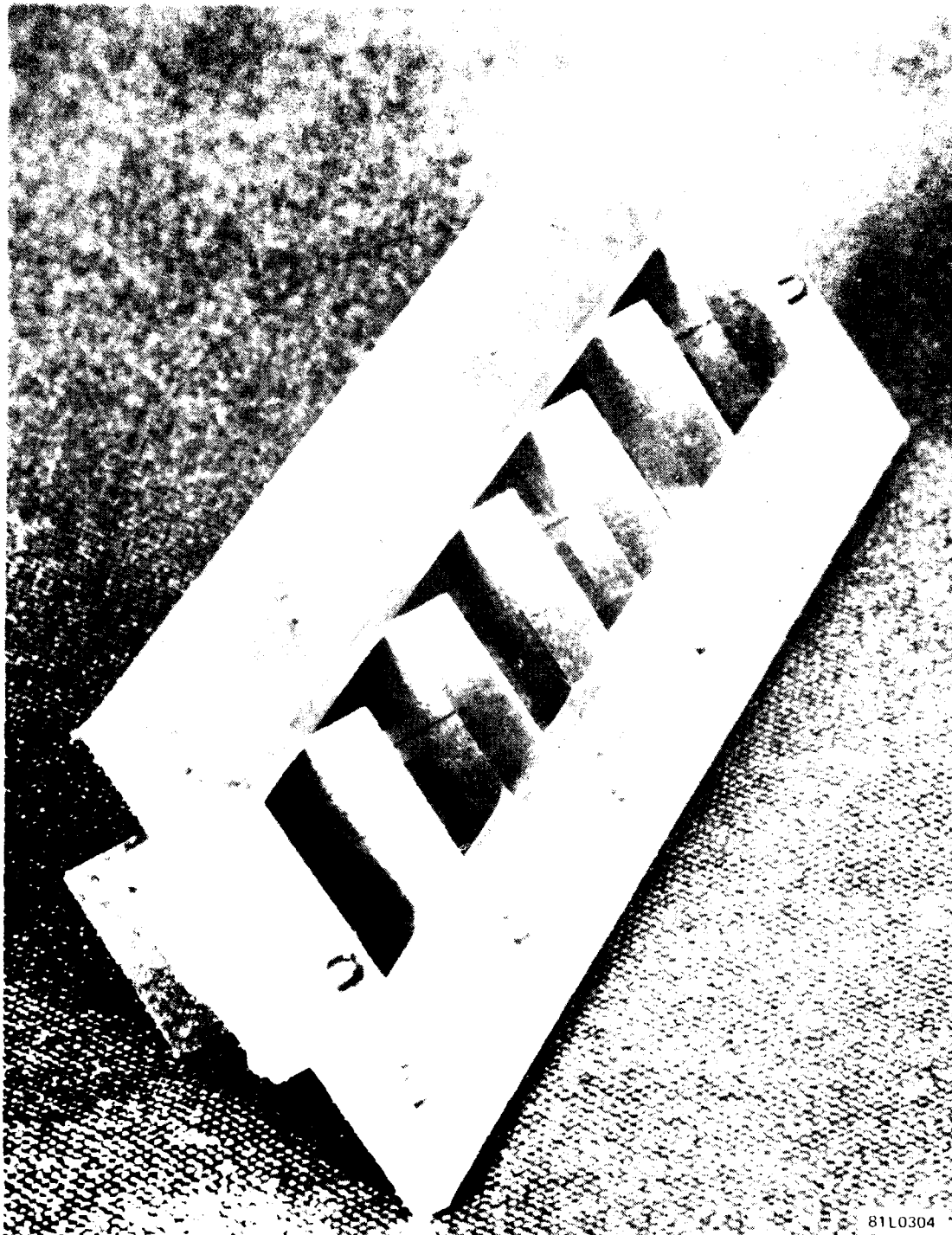
Figure 6-38. Infinite Array of Bent Dipoles Near Broadside Incidence Simulated in Waveguide
