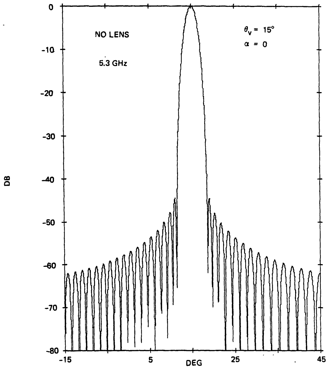
Figure 5-35. Elevation Pattern of Line Feed, \theta_v = 15^\circ
