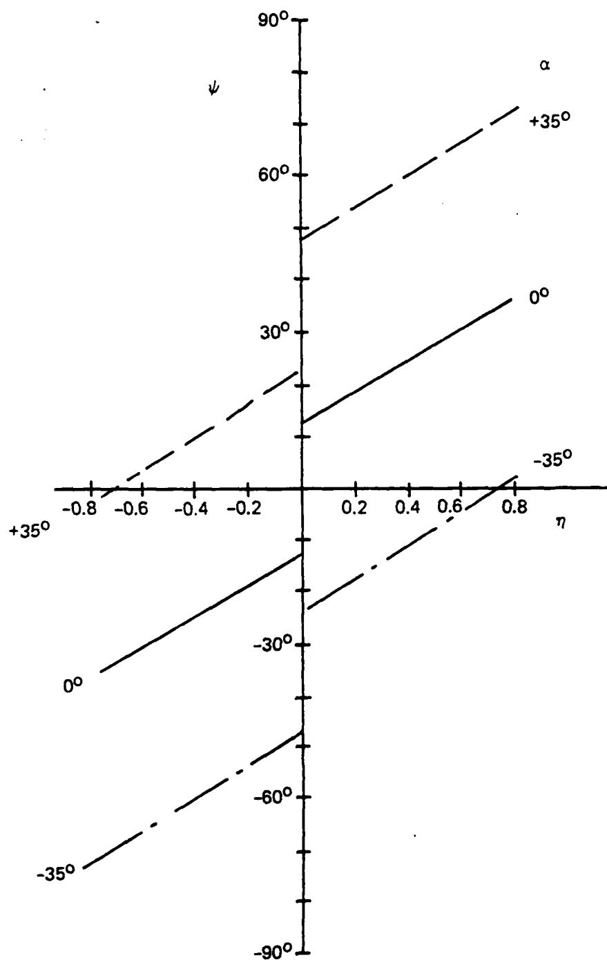
Figure 4-12. Incidence Angles for Outer Surface of Pointed Lens
