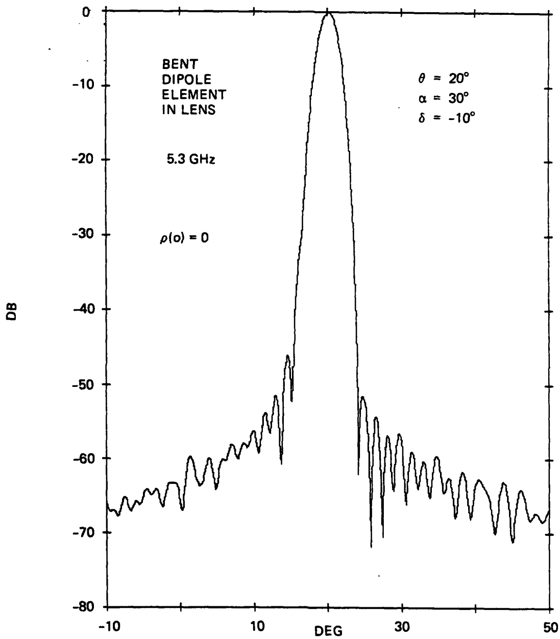
Figure 6-34. Azimuth Pattern of Antenna with Bent-Dipole Element, \alpha = 30^\circ , \delta = -10^\circ
