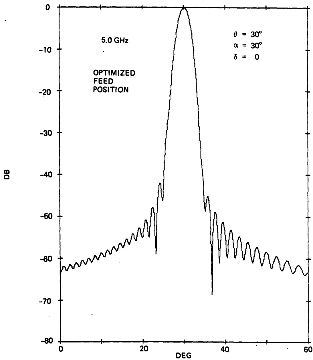
Figure 5-22. Azimuth Pattern of Antenna at 5.0 GHz with Optimized Feed Position, \theta = 30^\circ
