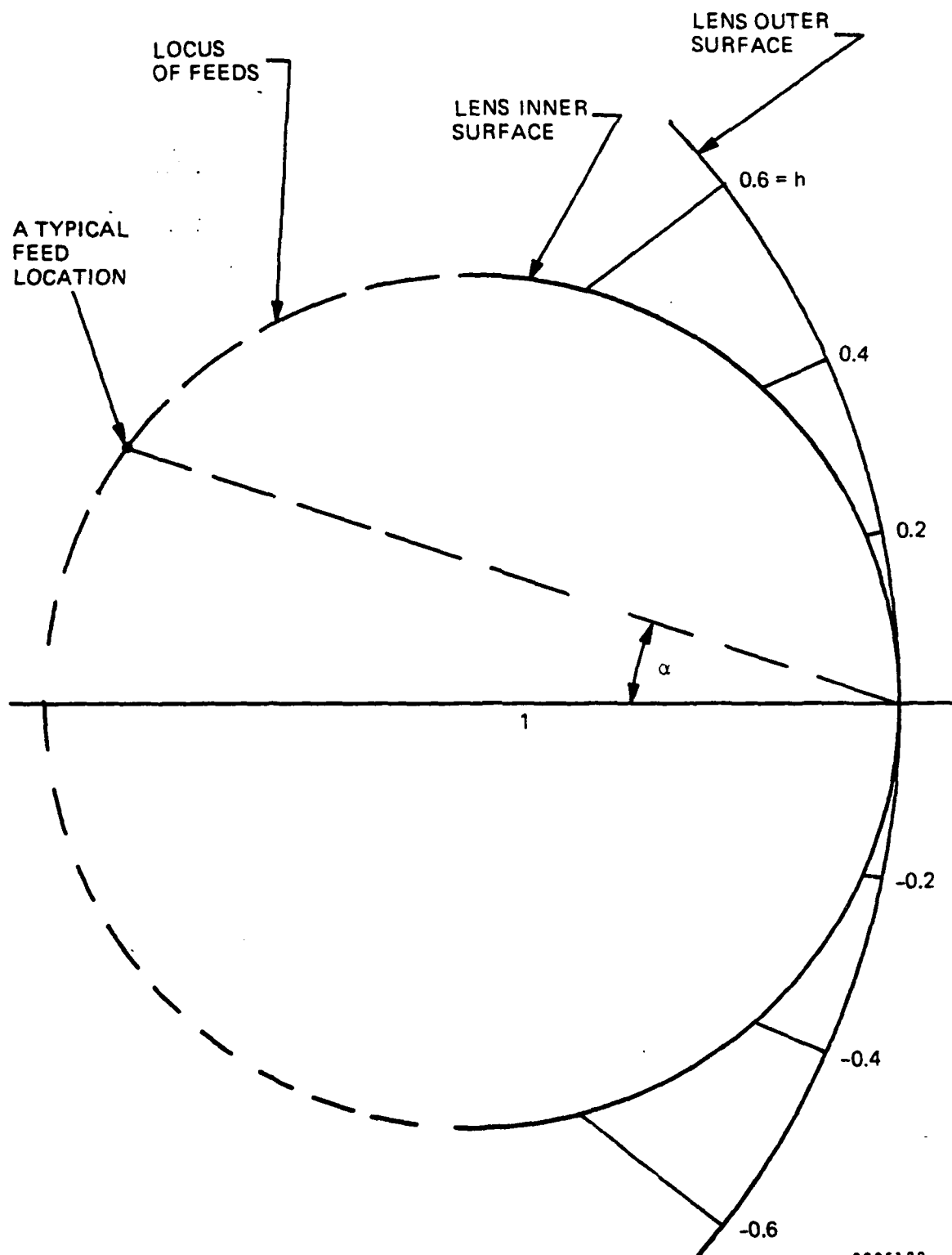
Figure 4-5. R-2R Lens Contours
