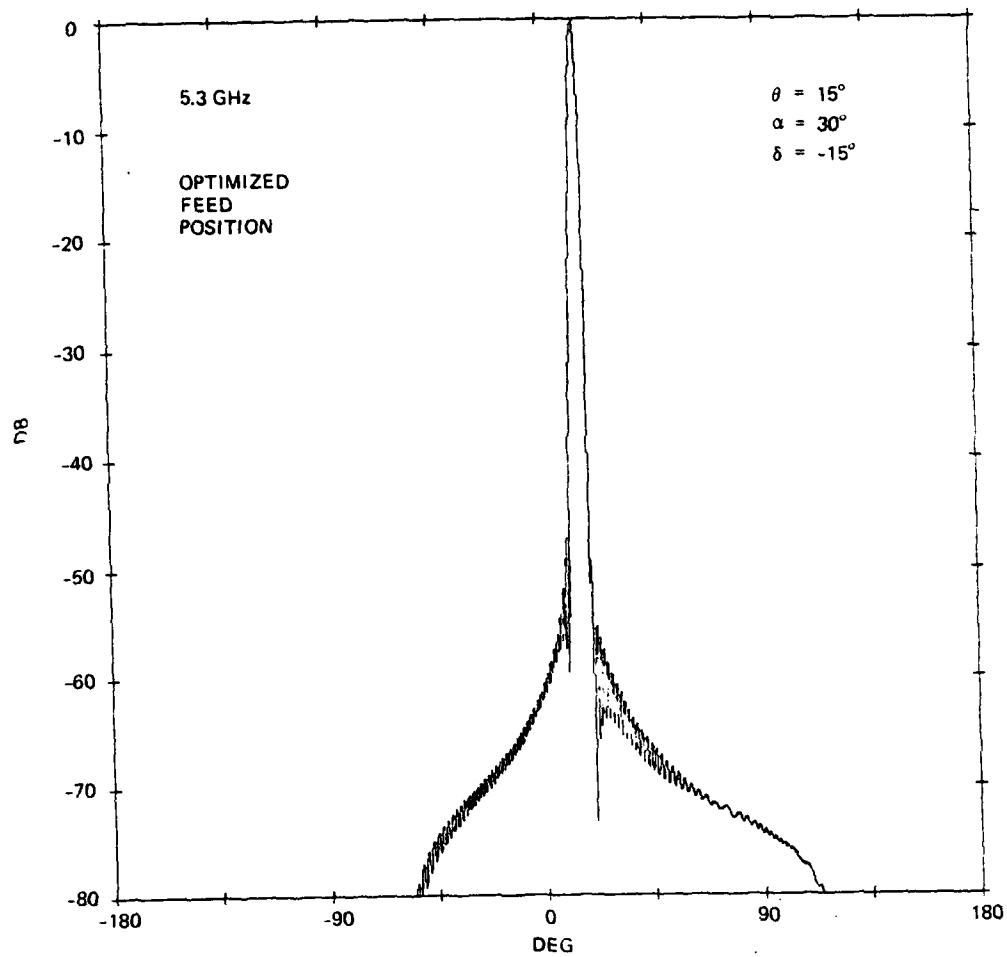
Figure 5-26. Wide-Angle Azimuth Pattern of Antenna at 5.3 GHz with Optimized Feed Position, \theta = 15^\circ
