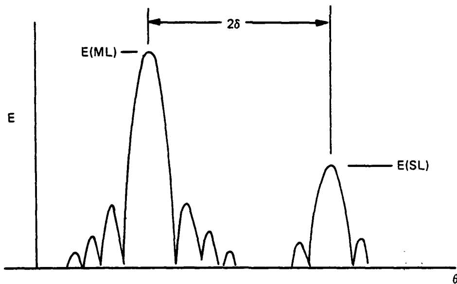
Figure 6-2. Effect of Lens Internal Reflections With Fine Steering
