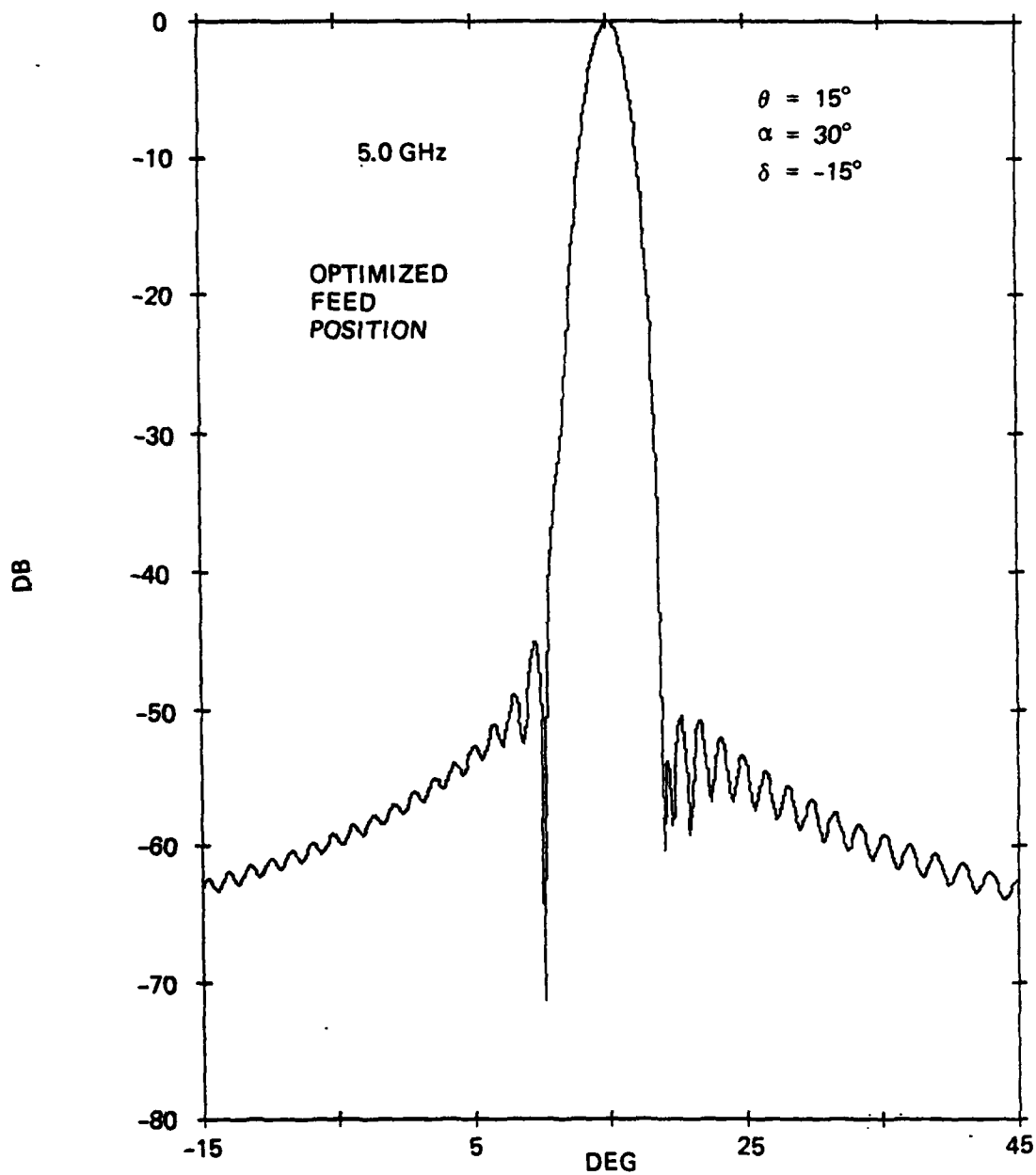
Figure 5-20. Azimuth Pattern of Antenna at 5.0 GHz with Optimized Feed Position, \theta = 15^\circ
