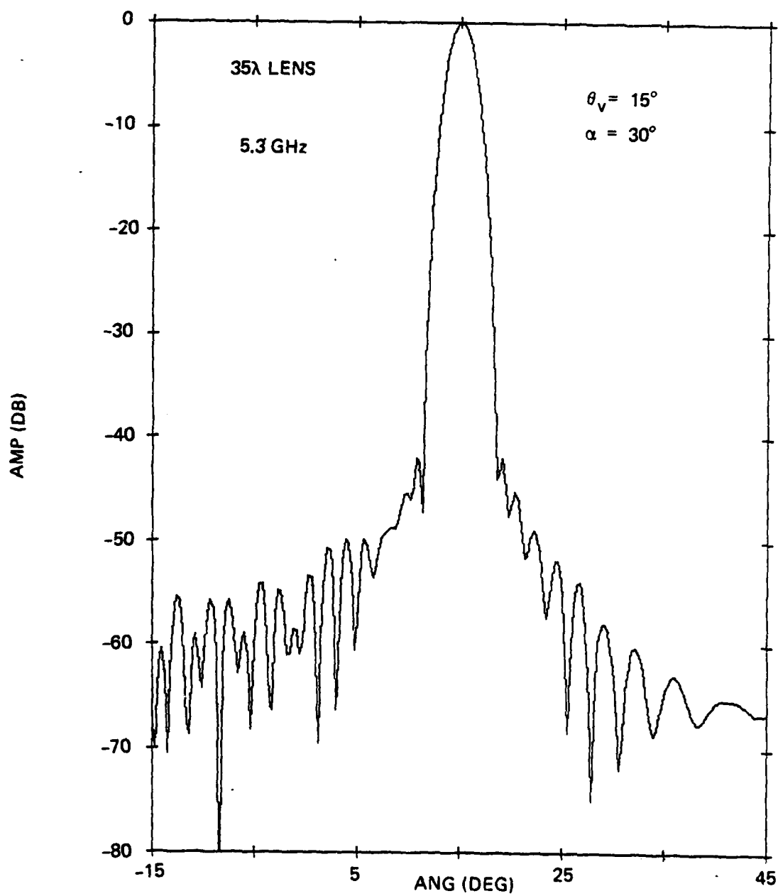
Figure 5-44. Elevation Pattern of Antenna, \theta_v = 15^\circ , \alpha = 30^\circ , 35 \lambda Lens
