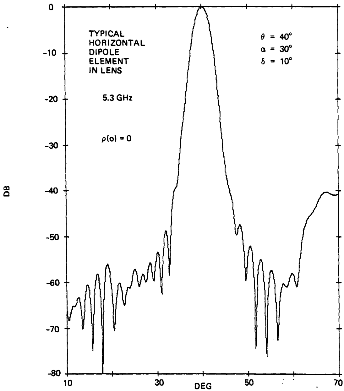
Figure 6-16. Azimuth Pattern of Antenna with Typical Horizontal-Dipole Element, \alpha = 30^\circ , \delta = 10^\circ
