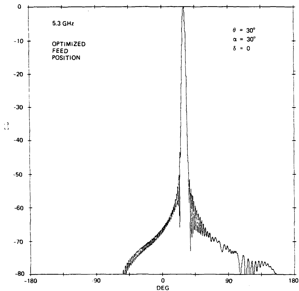
Figure 5-27. Wide-Angle Azimuth Pattern of Antenna at 5.3 GHz with Optimized Feed Position, \theta = 30^\circ
