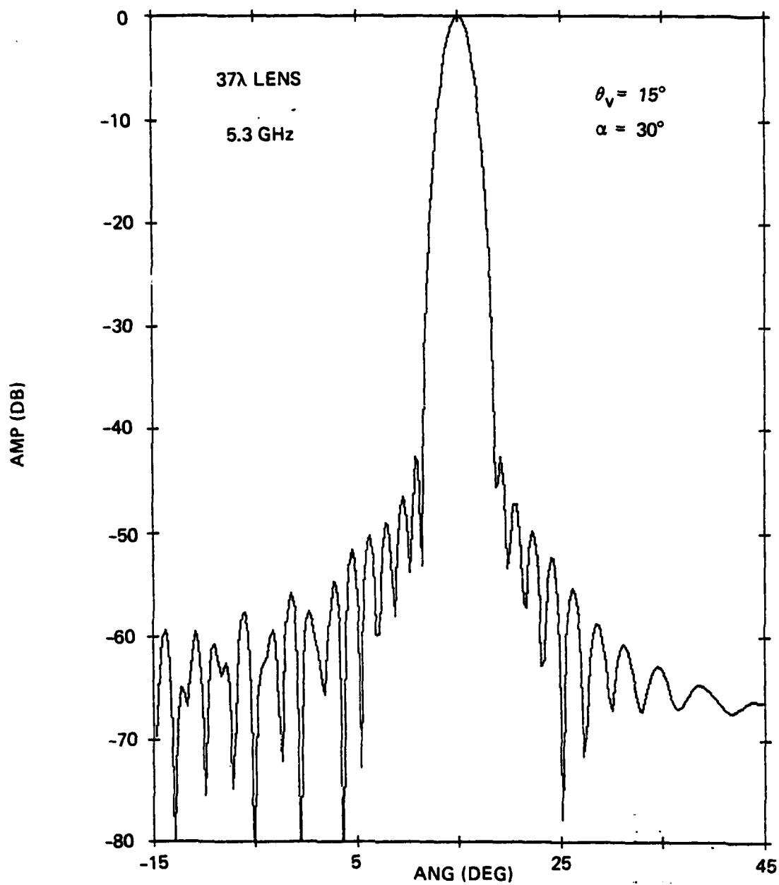
Figure 5-43. Elevation Pattern of Antenna \theta_v = 15^\circ , \alpha = 30^\circ , 37 λ Lens
