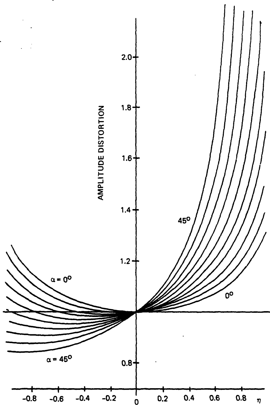
Figure 4-10. Amplitude Distortion of R-2R Lens
