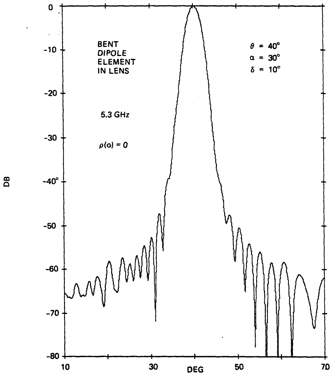
Figure 6-35. Azimuth Pattern of Antenna with Bent-Dipole Element, \alpha = 30^\circ , \delta = 10^\circ
