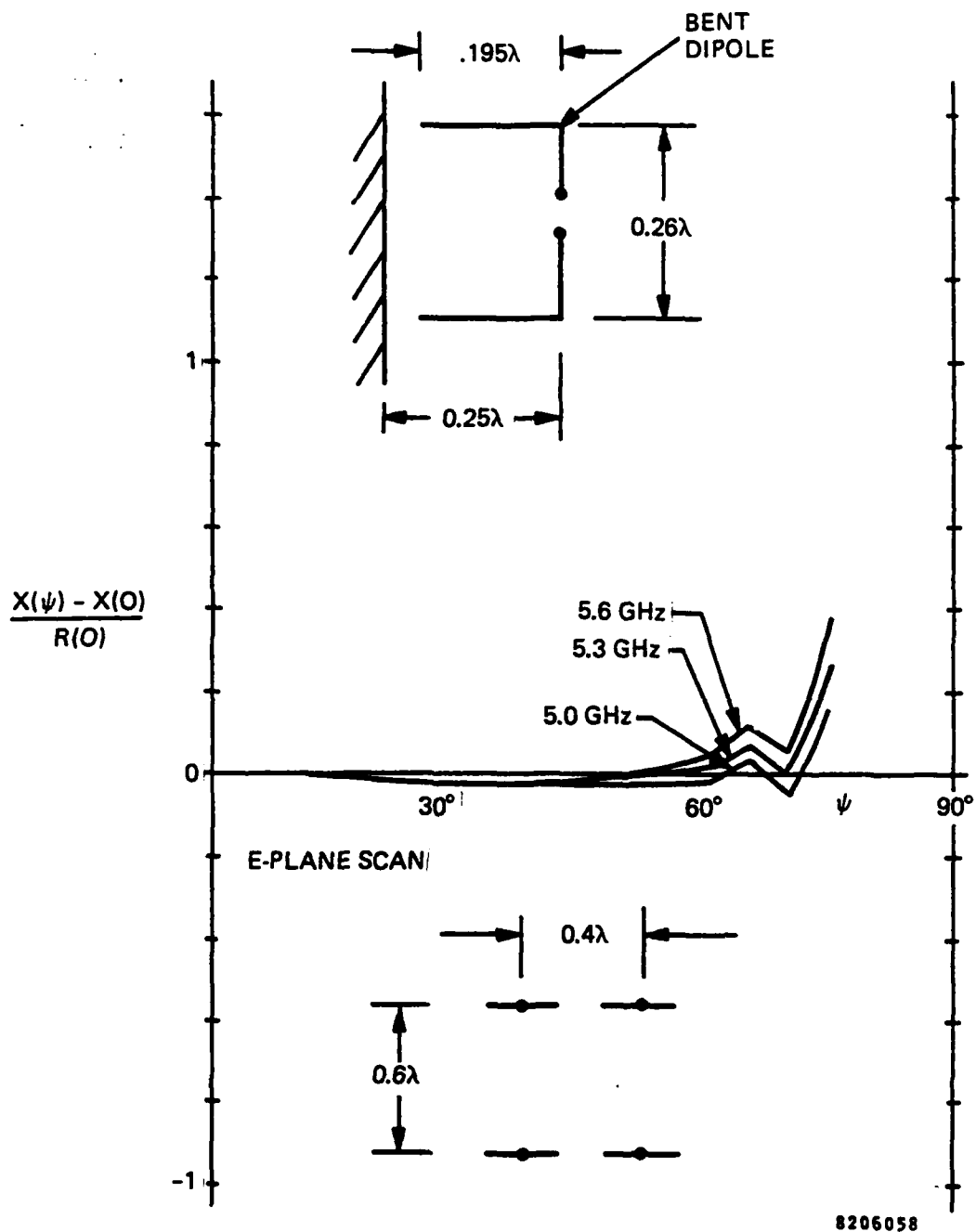
Figure 6-29. Optimum Bent Dipole Array Reactance vs Angle at Three Frequencies
