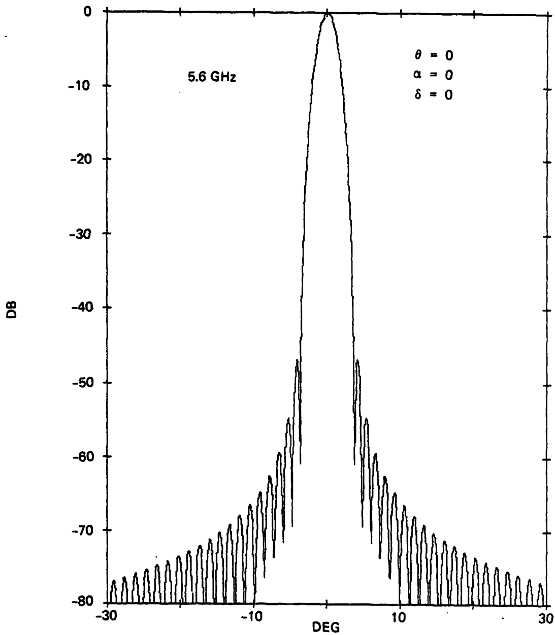
Figure 5-8. Azimuth Pattern of Antenna at 5.6 GHz for \theta = 0
