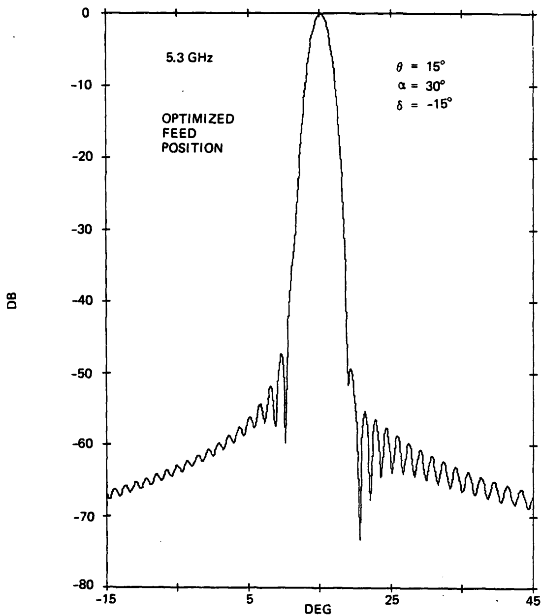
Figure 5-17. Azimuth Pattern of Antenna with Optimized Feed Position, \theta = 15^\circ
