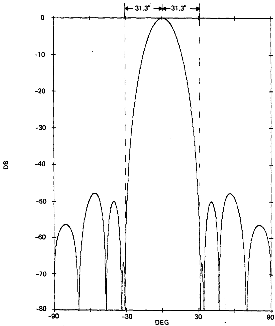
Figure 5-5. Line Feed Azimuth Pattern
