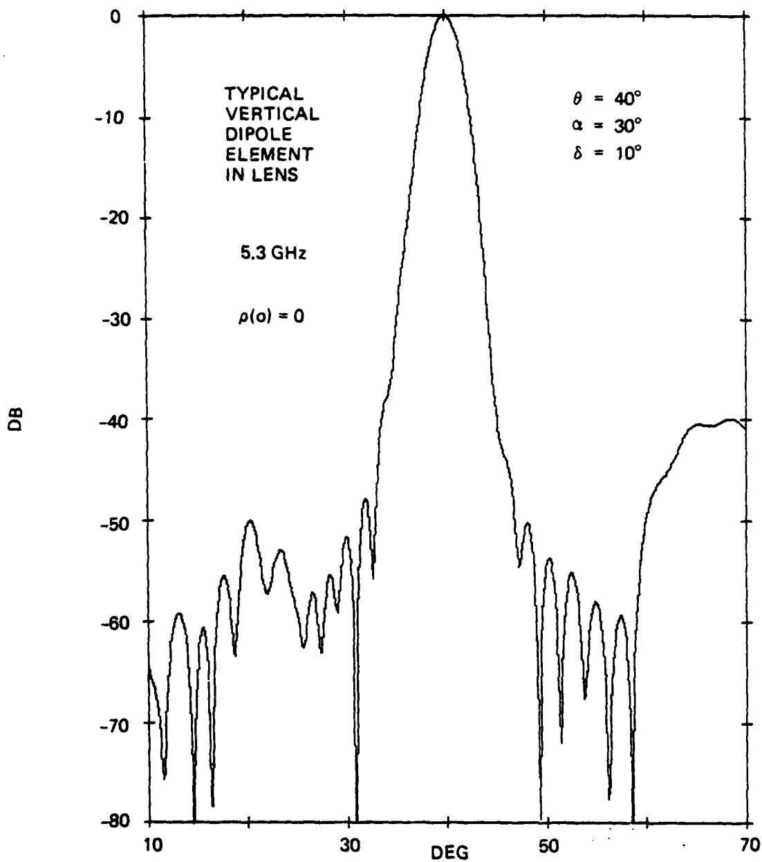
Figure 6-14. Azimuth Pattern of Antenna with Typical Vertical-Dipole Element, \alpha = 30^\circ , \delta = 10^\circ
