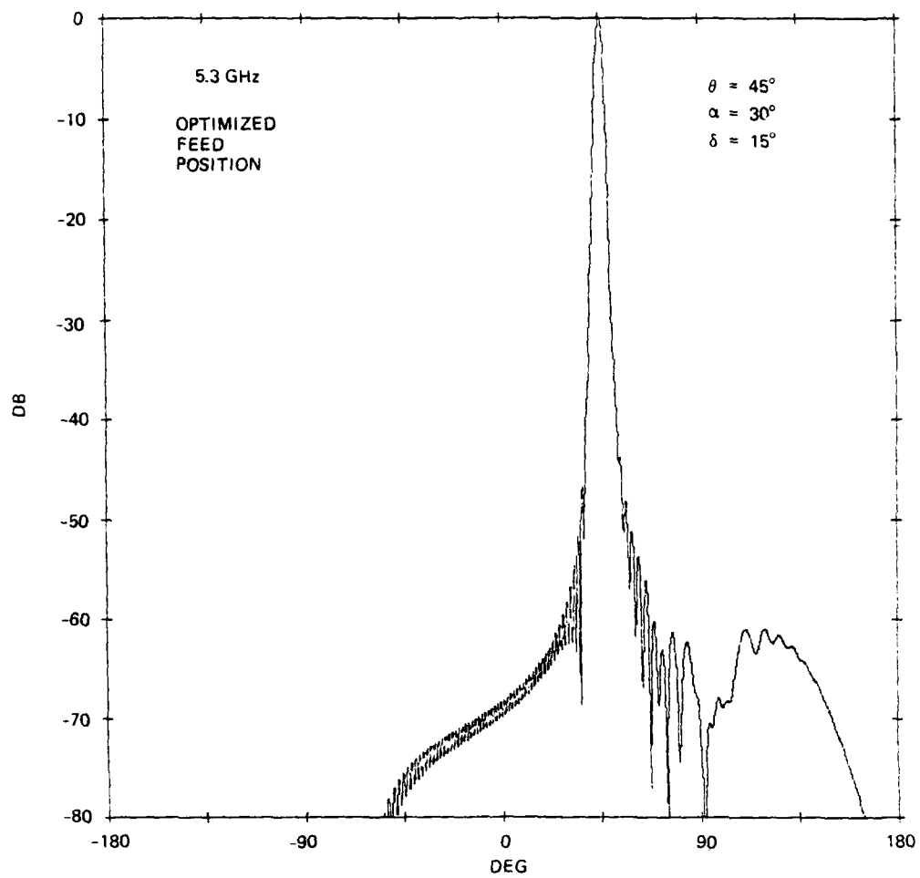
Figure 5-28. Wide-Angle Azimuth Pattern of Antenna at 5.3 GHz with Optimized Feed Position, \theta = 45^\circ
