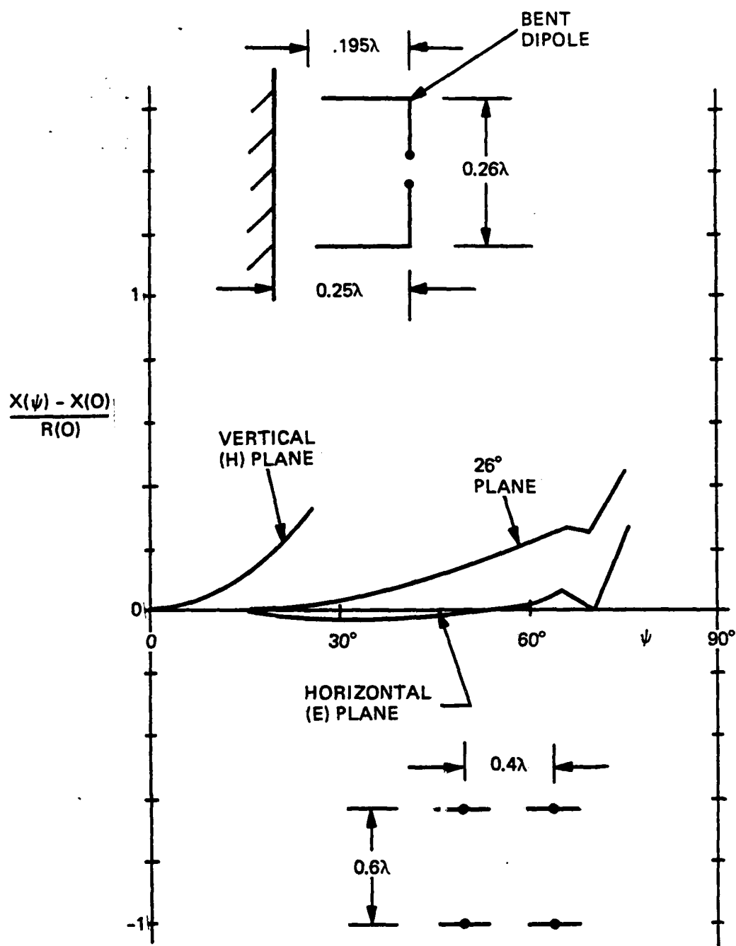
Figure 6-31. Optimum Bent Dipole Array Reactance vs Angle in Three Incidence Planes
