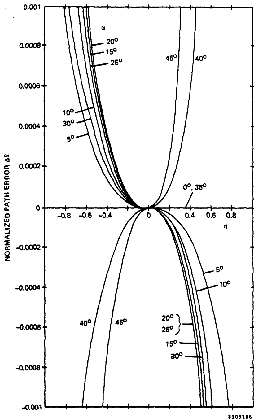
Figure 4-6. Phase Aberration of Pointed Lens
