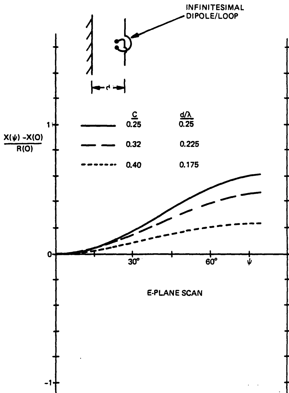
Figure 6-21. Infinitesimal Dipole/Loop Array First-Term Reactance vs Angle and Distance to Ground Plane
