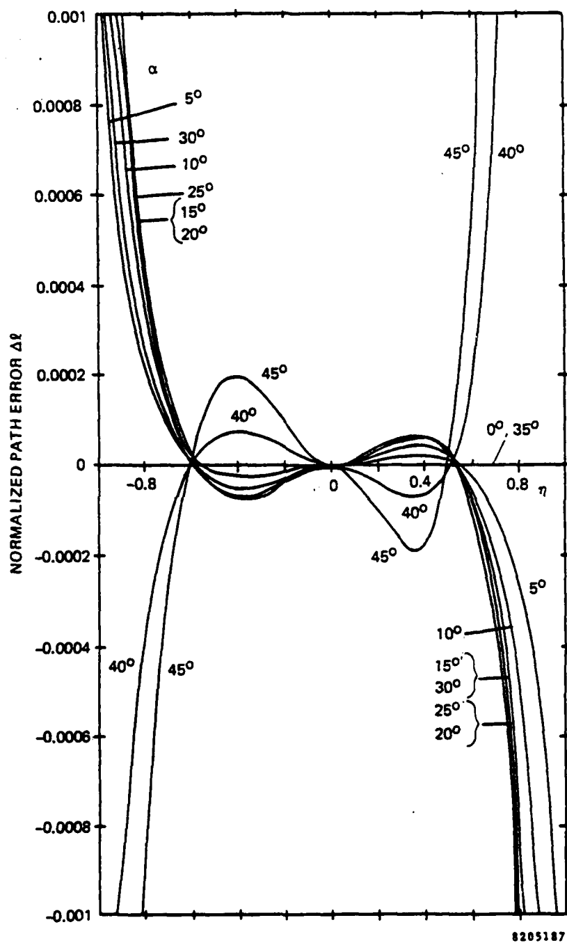
Figure 4-7. Phase Aberration of Dimpled Lens
