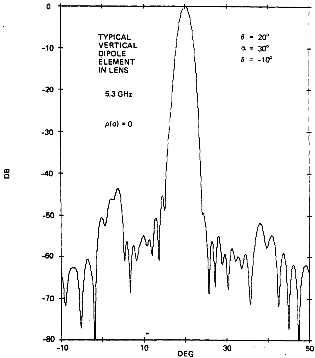
Figure 6-13. Azimuth Pattern of Antenna with Typical Vertical-Dipole Element, \alpha = 30^\circ , \delta = -10^\circ
