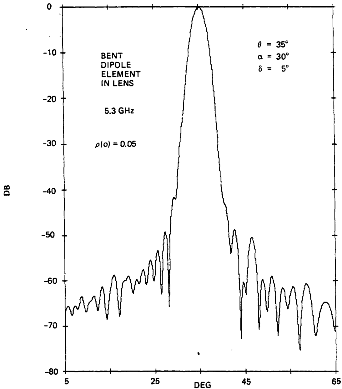
Figure 6-41. Azimuth Pattern of Antenna with Bent-Dipole Element, \rho(o) = 0.05 , \alpha = 30^\circ , \delta = 5^\circ
