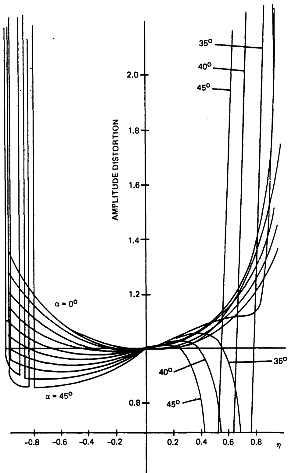
Figure 4-8. Amplitude Distortion of Pointed Lens
