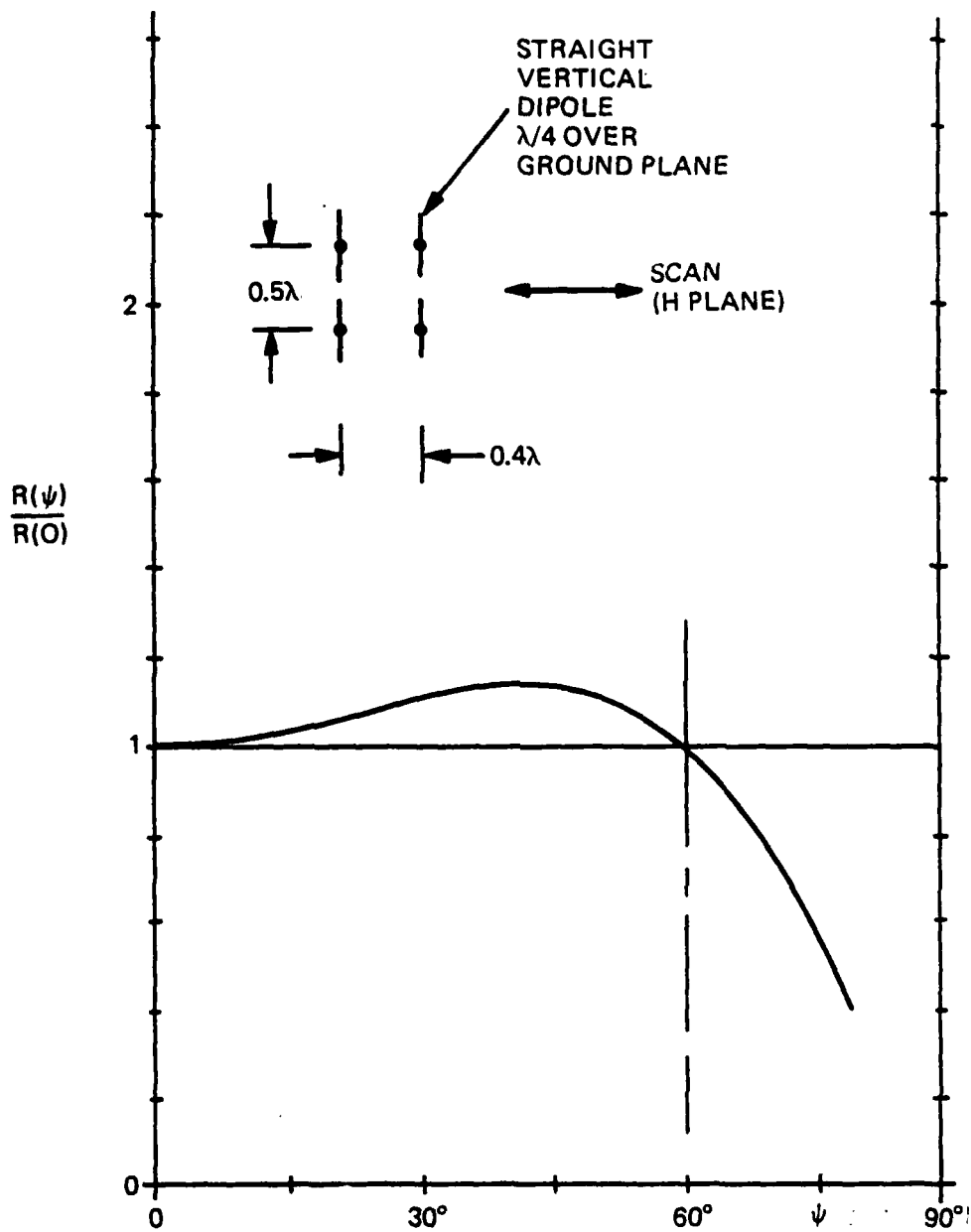
Figure 6-3. Typical Array Resistance vs Angle for Straight Dipole in H Plane
