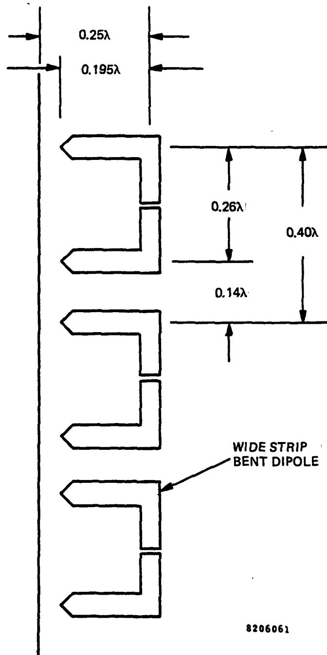
Figure 6-36. Optimum Bent Dipole in Strip Configuration
