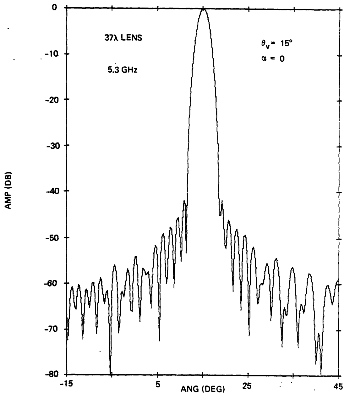
Figure 5-40. Elevation Pattern of Antenna, \theta_v = 15^\circ , 37 \lambda Lens
