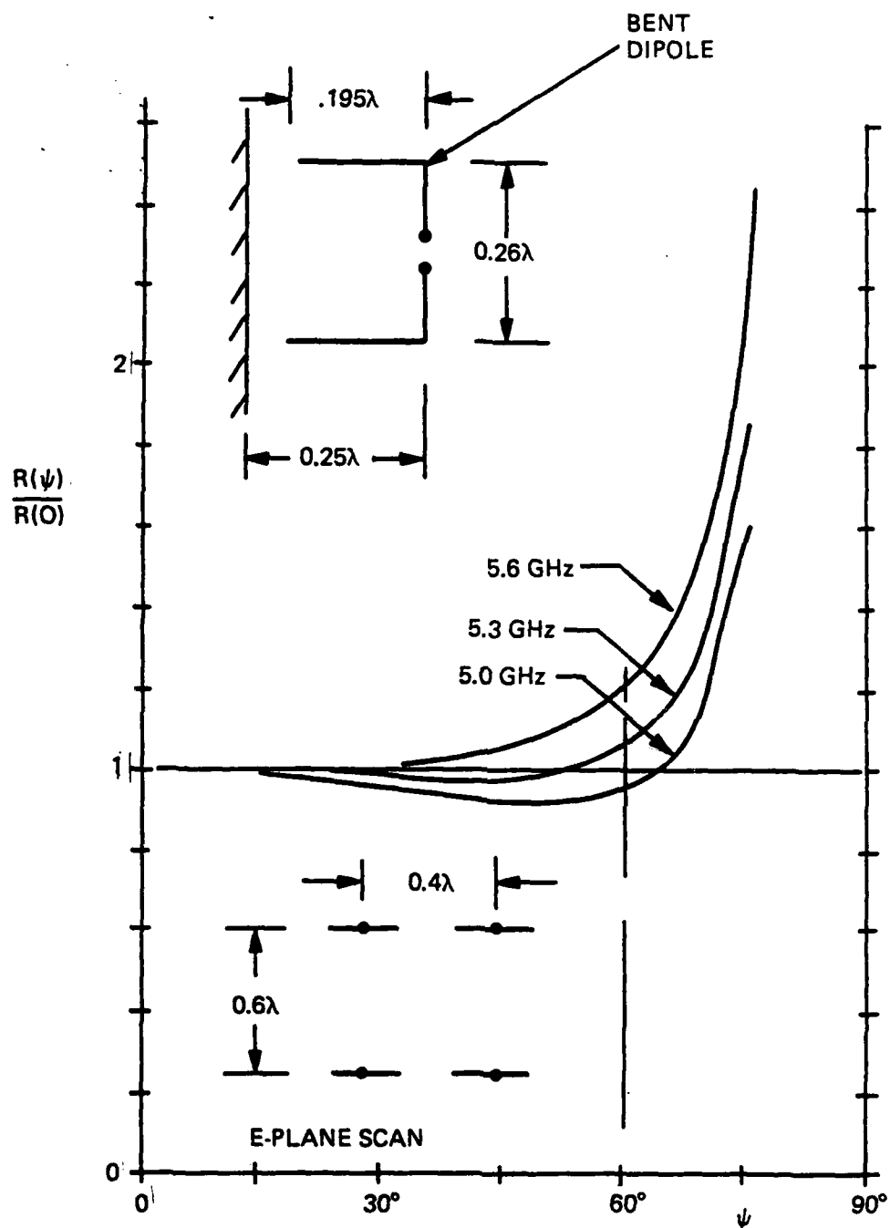
Figure 6-28. Optimum Bent Dipole Array Resistance vs Angle at Three Frequencies
