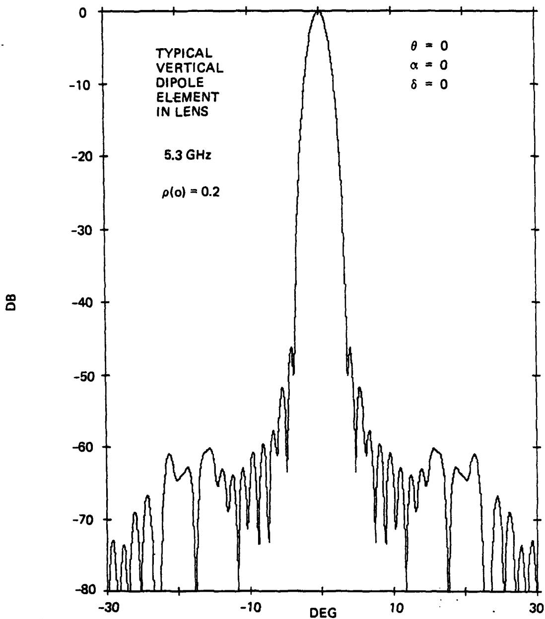
Figure 6-7. Azimuth Pattern of Antenna with Typical Vertical-Dipole Element, \theta = 0
