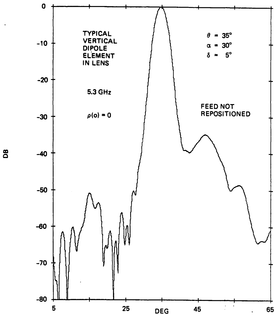
Figure 6-17. Azimuth Pattern of Antenna with Typical Vertical-Dipole Element, but with Line Feed Not Repositioned \alpha = 30^\circ , \delta = 5^\circ
