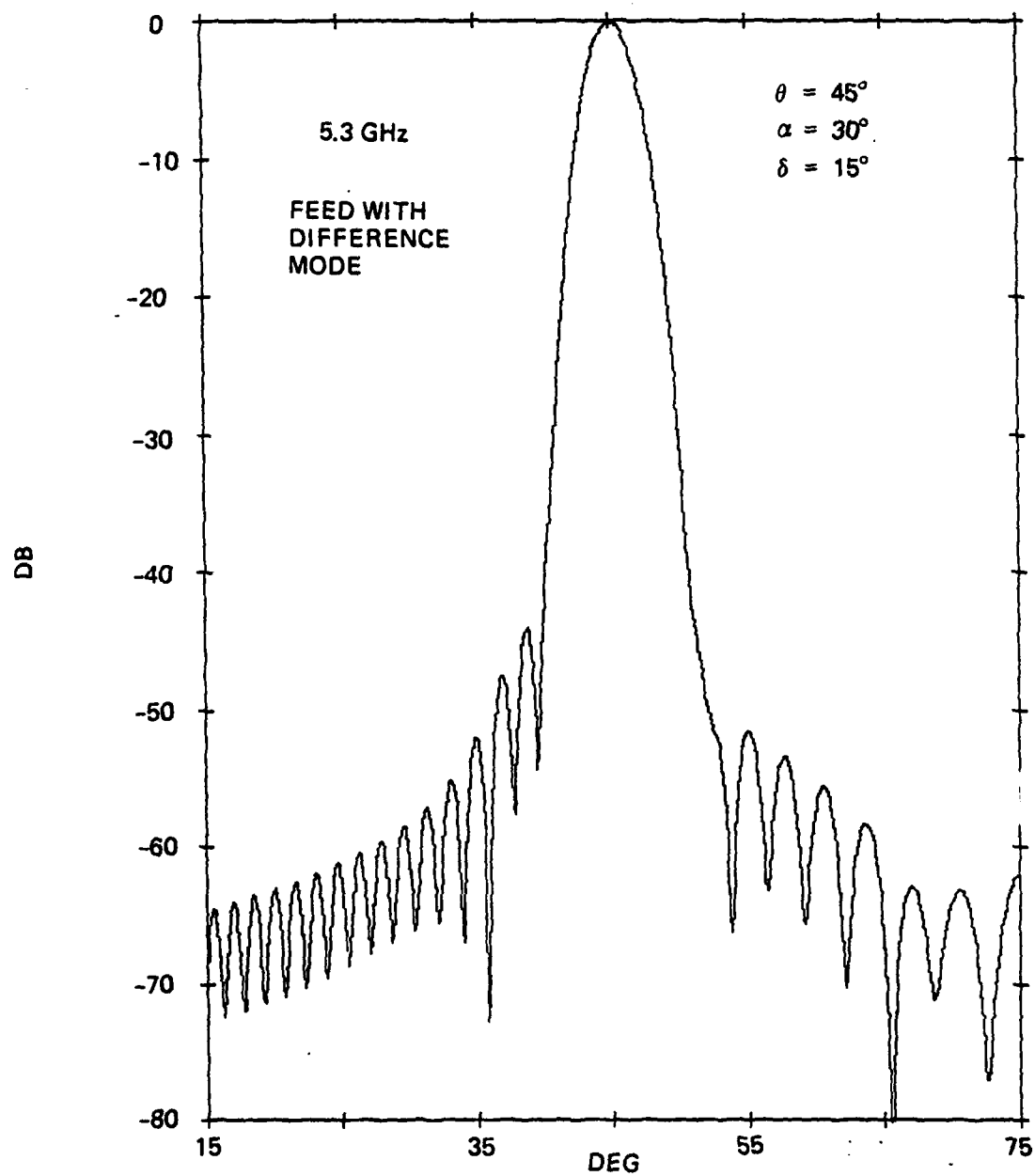
Figure 5-32. Azimuth Pattern of Antenna with Feed Difference Mode, \theta = 45^\circ
