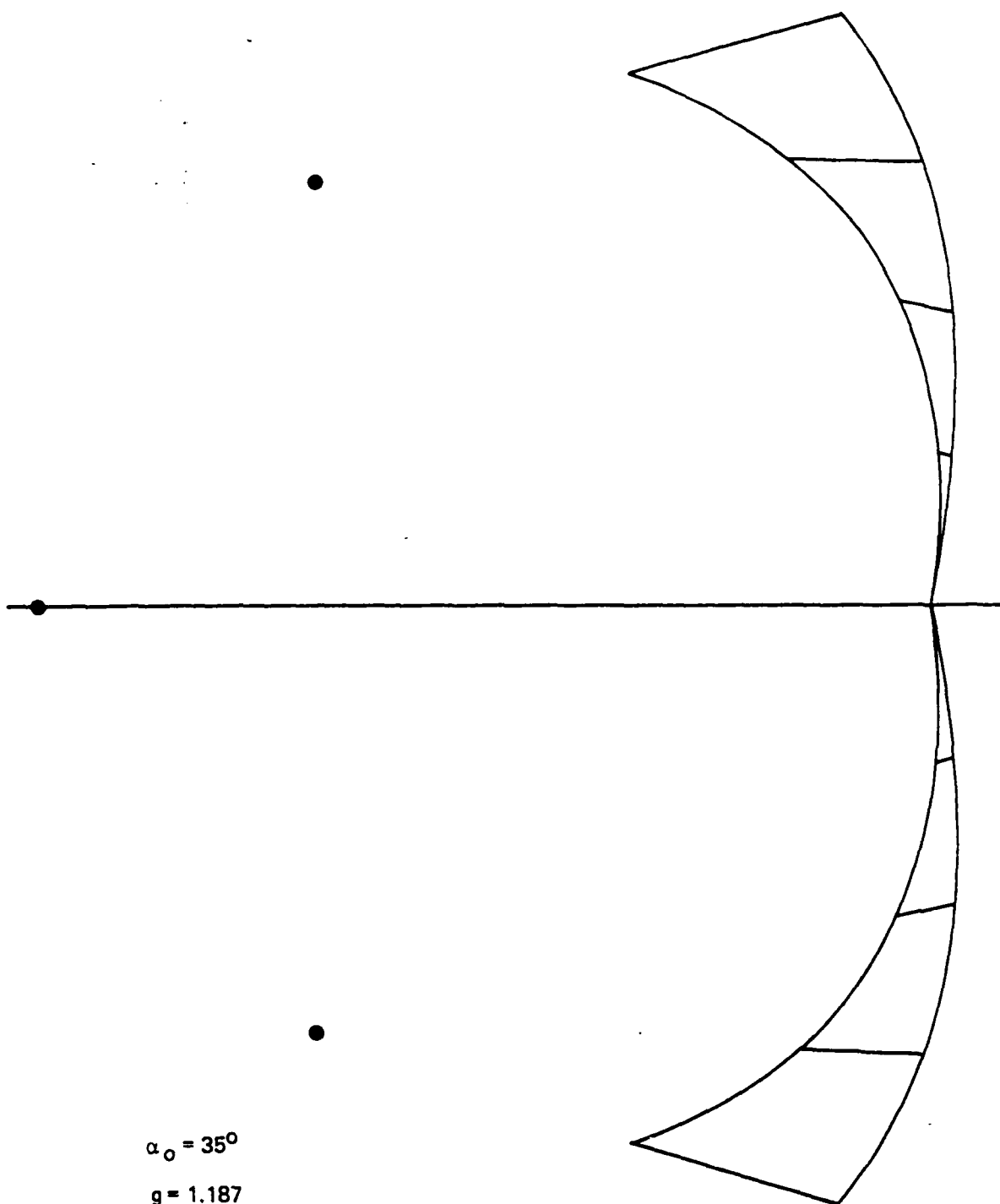
Figure 4-3. Dimpled Lens Contours
