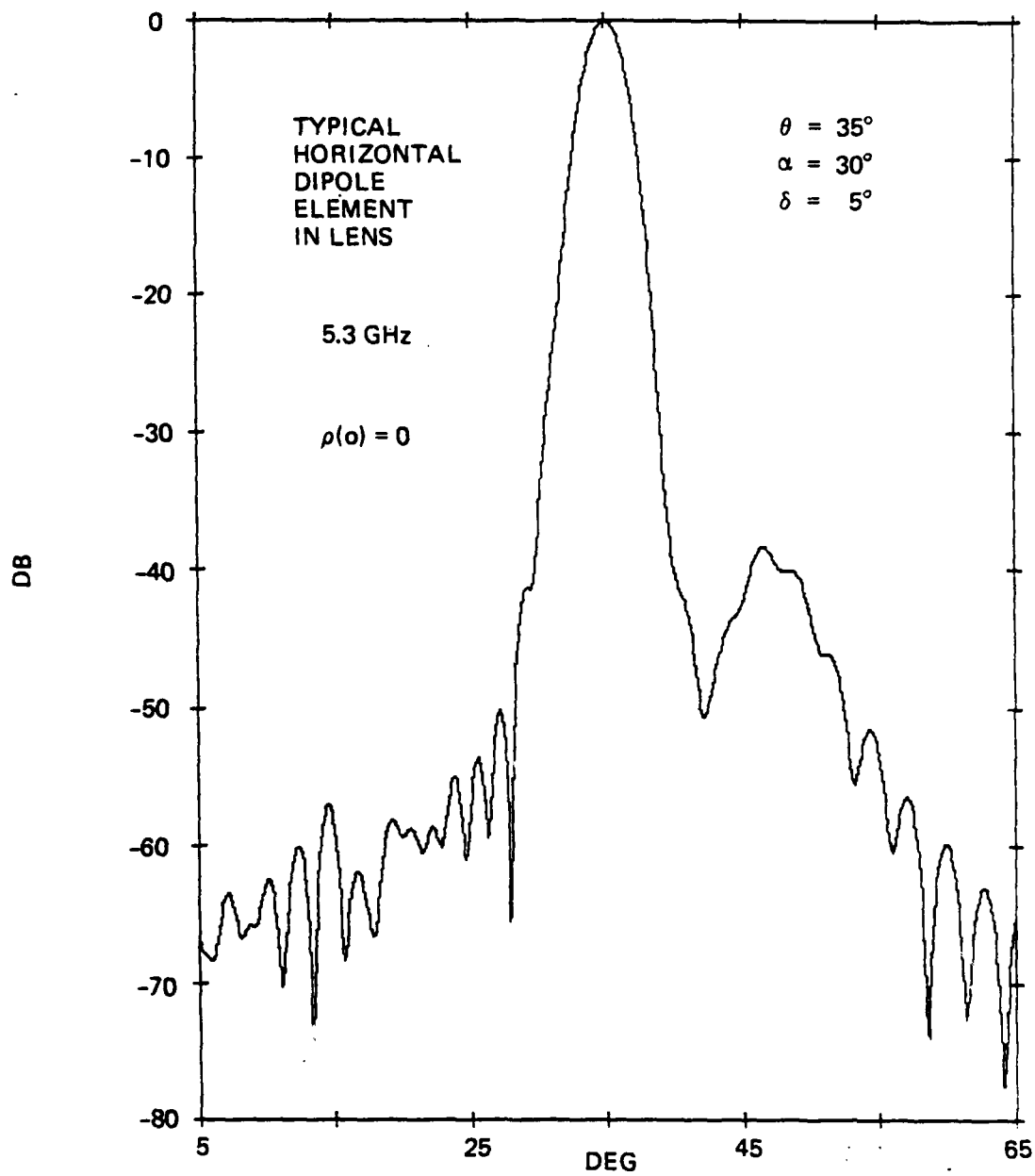
Figure 6-12. Azimuth Pattern of Antenna with Typical Horizontal-Dipole Element, \alpha = 30^\circ , \delta = 5^\circ
