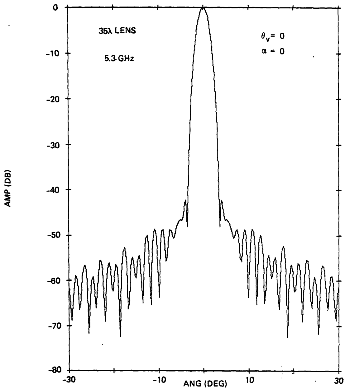
Figure 5-38. Elevation Pattern of Antenna, \theta_v = 0 , 35 λ Lens
