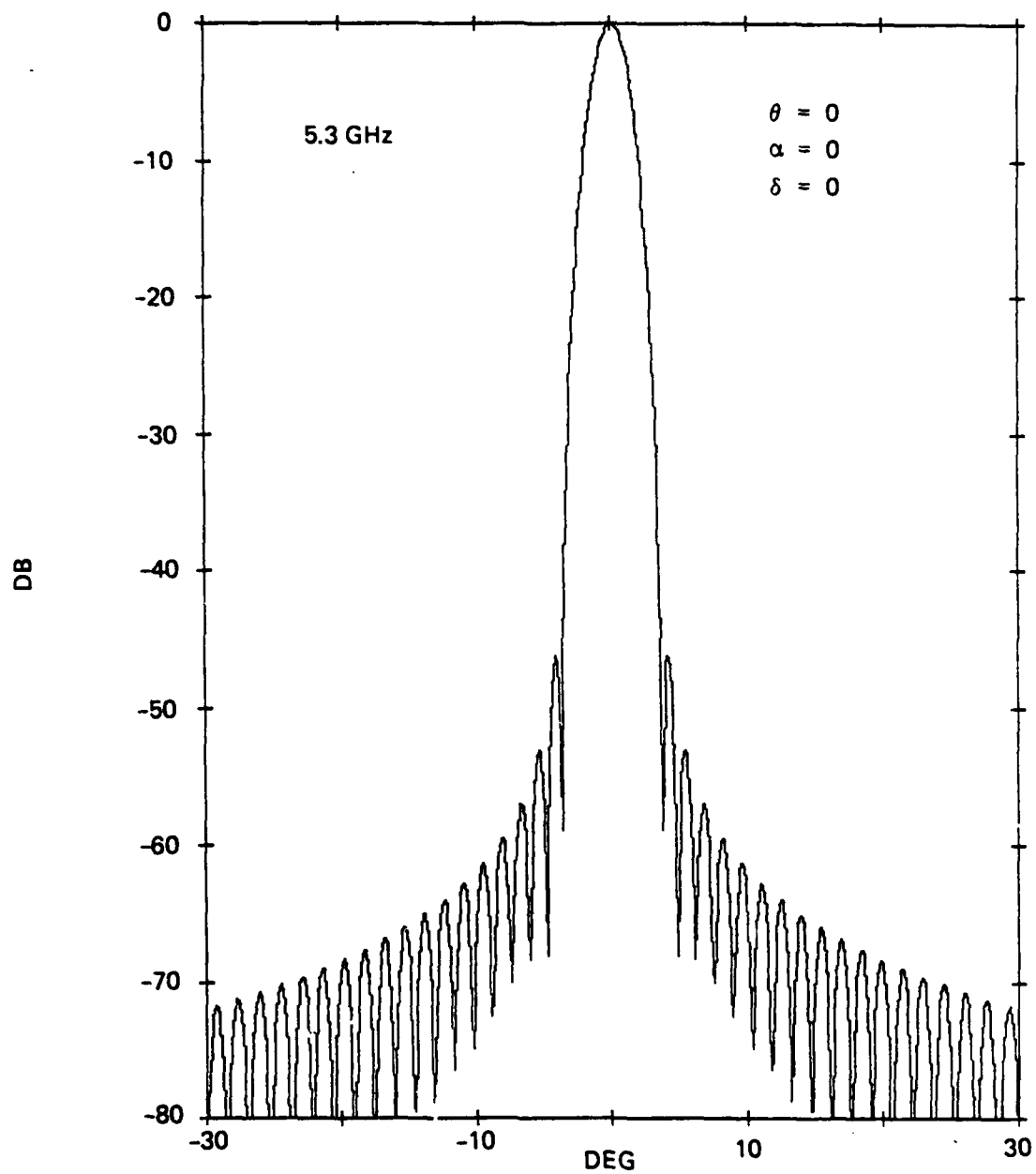
Figure 5-6. Azimuth Pattern of Antenna at 5.3 GHz for \theta = 0
