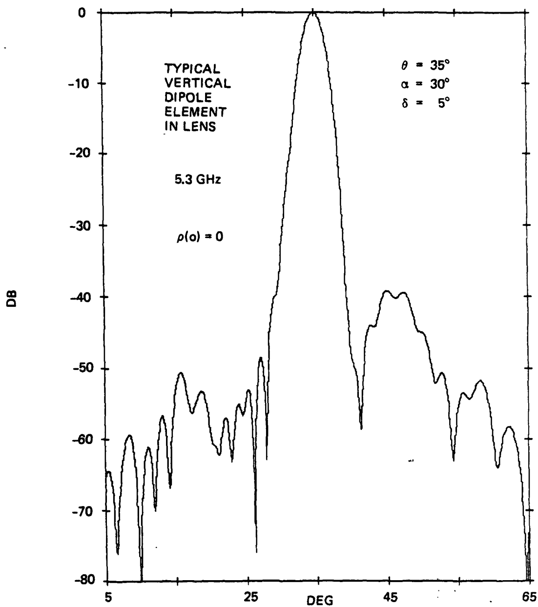
Figure 6-10. Azimuth Pattern of Antenna with Typical Vertical-Dipole Element, \alpha = 30^\circ , \delta = 5^\circ
