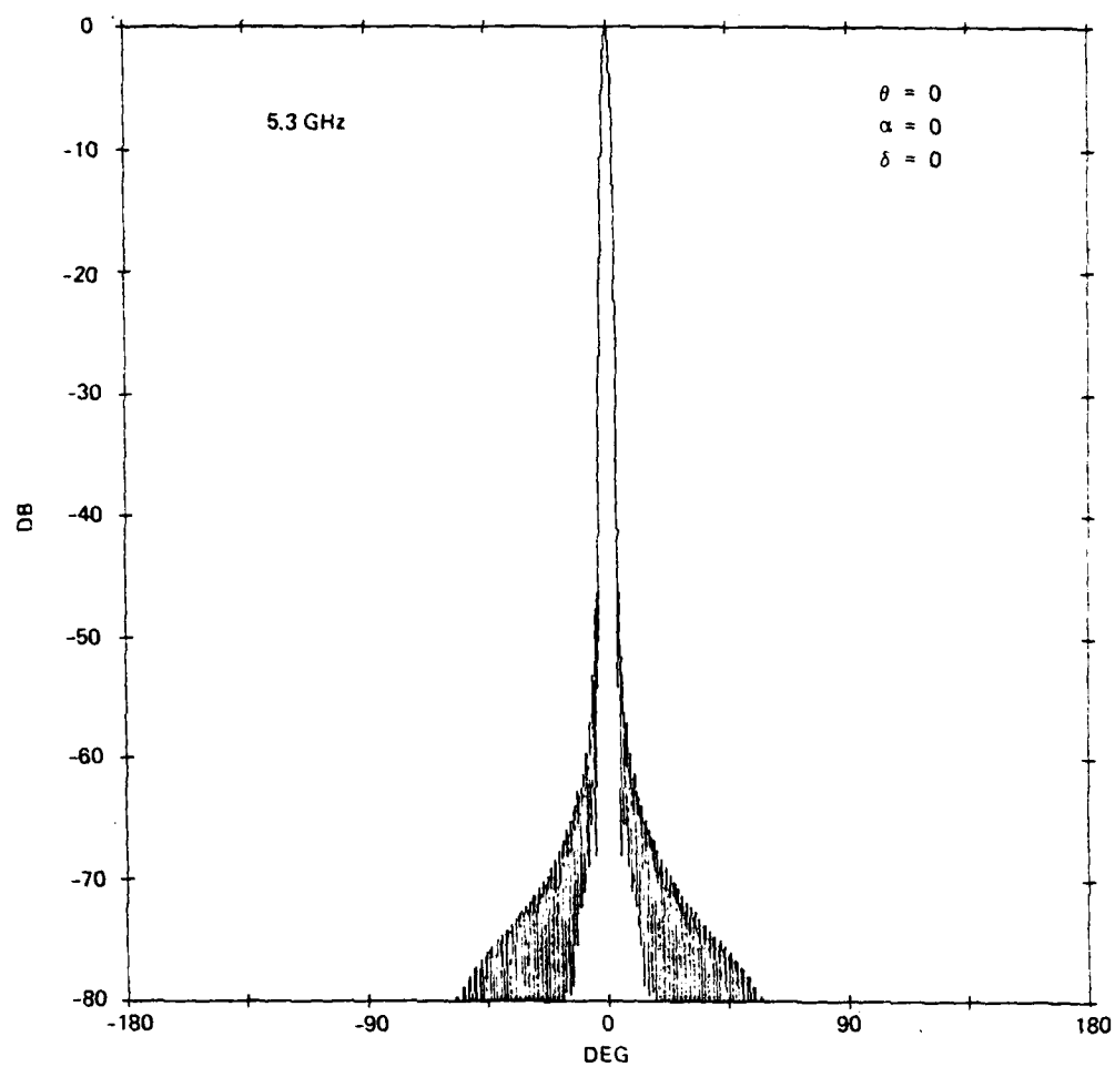
Figure 5-9. Wide-Angle Azimuth Pattern of Antenna at 5.3 GHz for \theta = 0
