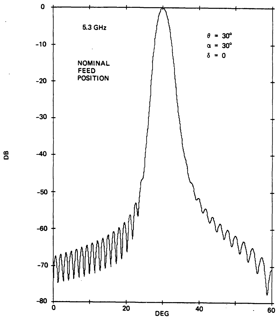
Figure 5-12. Azimuth Pattern of Antenna with Nominal Feed Position for \alpha = 30^\circ and \theta = 30^\circ
