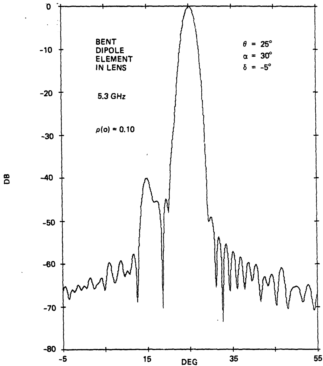
Figure 6-42. Azimuth Pattern of Antenna with Bent-Dipole Element \rho(o) = 0.10 , \alpha = 30^\circ , \delta = -5^\circ
