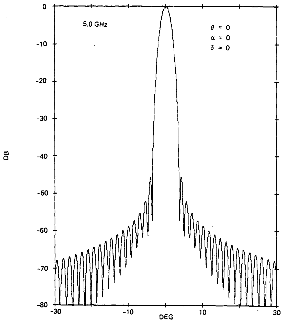
Figure 5-7. Azimuth Pattern of Antenna at 5.0 GHz for \theta = 0
