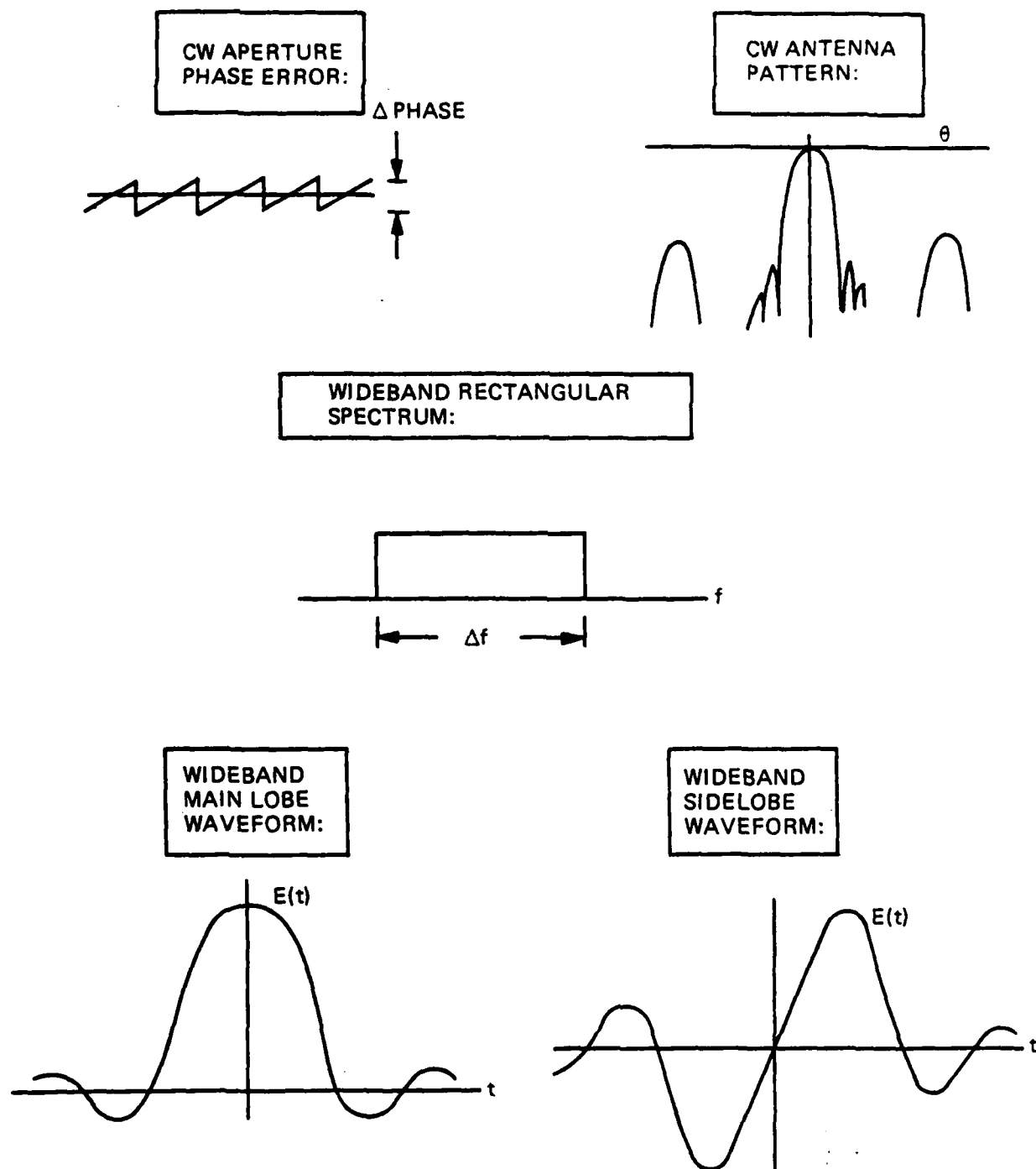
8206040 Figure 5-46. Comparison of Theoretical Waveforms for Mainlobe and Wideband Sidelobes Caused by Switched-Line Phase Shifters
