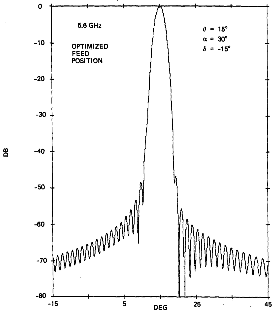
Figure 5-21. Azimuth Pattern of Antenna at 5.6 GHz with Optimized Feed Position, \theta = 15^\circ
