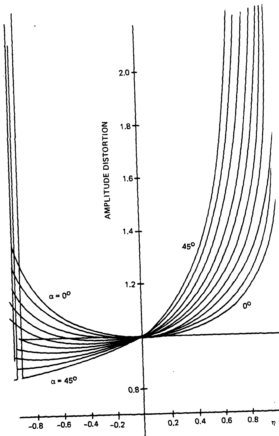
Figure 4-9. Amplitude Distortion of Dimpled Lens
