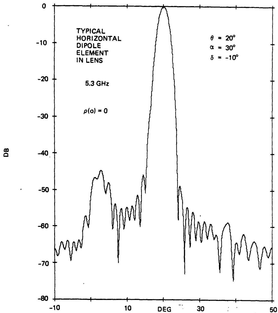
Figure 6-15. Azimuth Pattern of Antenna with Typical Horizontal-Dipole Element, \alpha = 30^\circ , \delta = -10^\circ
