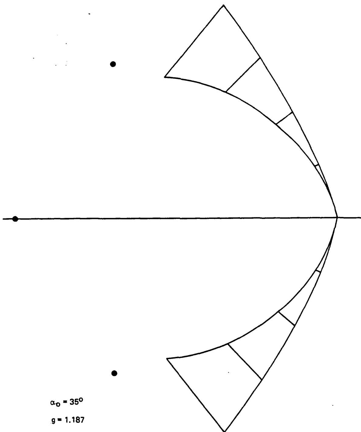
Figure 4-2. Pointed Lens Contours
