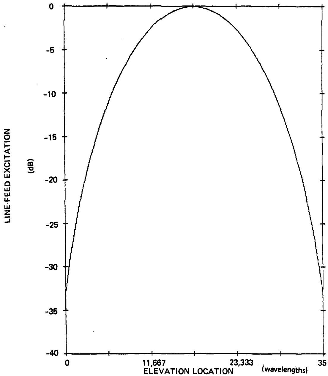
Figure 5-33. Vertical Distribution of Line-Feed Excitation
