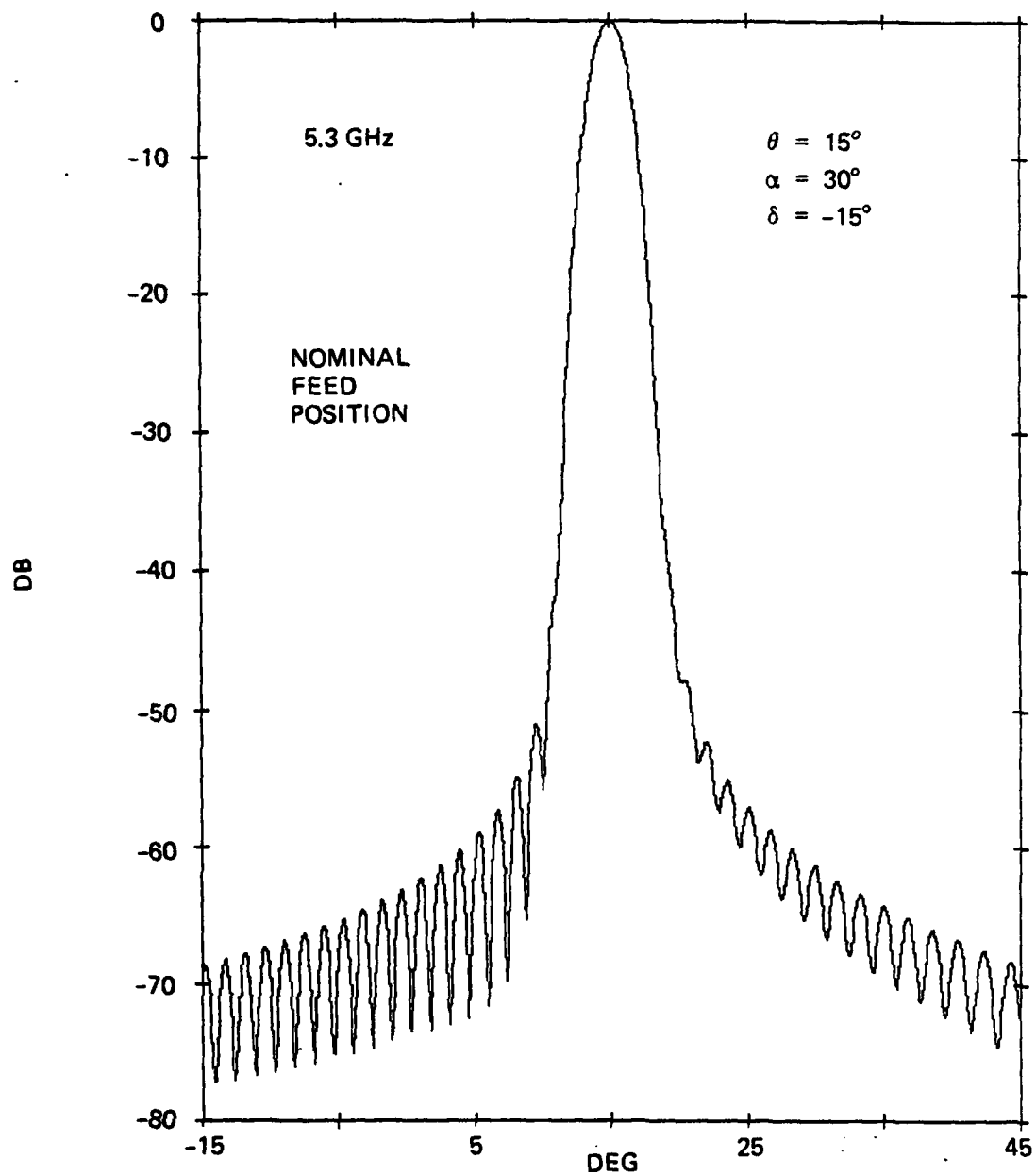
Figure 5-11. Azimuth Pattern of Antenna with Nominal Feed Position for \alpha = 30^\circ and \theta = 15^\circ
