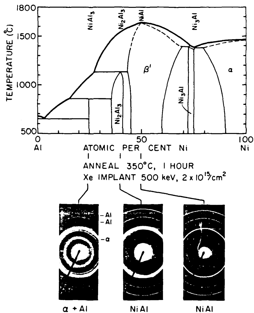
Figure 2.3. TEM diffraction patterns of the multilayered Ni/Al samples preannealed at 350°C for 1 hr., followed by 2 \times 10^{15} \text{ Xe cm}^{-2} implant, showing the formation of the amorphous or the crystalline NiAl phase, depending on the original compounds.
