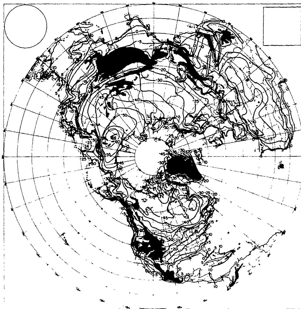
Figure 15.5. Temperature Equalled or Colder 1 Percent of the Time During the Coldest Month
