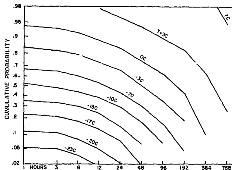
Figure 15.12. The Frequency of Duration (h) of the Temperature ( \leq T ) in the Mid-Winter Month (1 January to 1 February) at Minneapolis, Minn. (Based on 1943-1952 Data)
