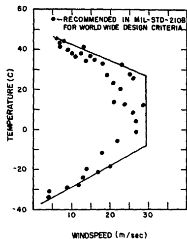
Figure 15.17. Extremes of Temperature in Combination With Windspeed. Windspeeds, in general, were observed 12 to 30 m above the surface. The 35 observations were taken over a 5-yr period at some 22 stations widely scattered in the United States. The envelope is for the recommended U.S. design criteria
