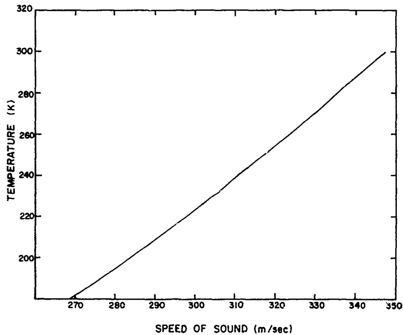
Figure 15.15. Speed of Sound vs Temperature (K)
