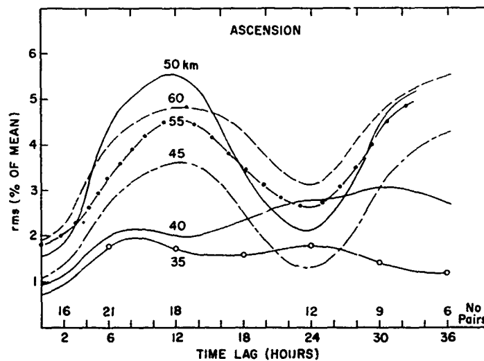
Figure 15.22. Root Mean Square (rms) Lag Variability of Density With Time at Ascension
