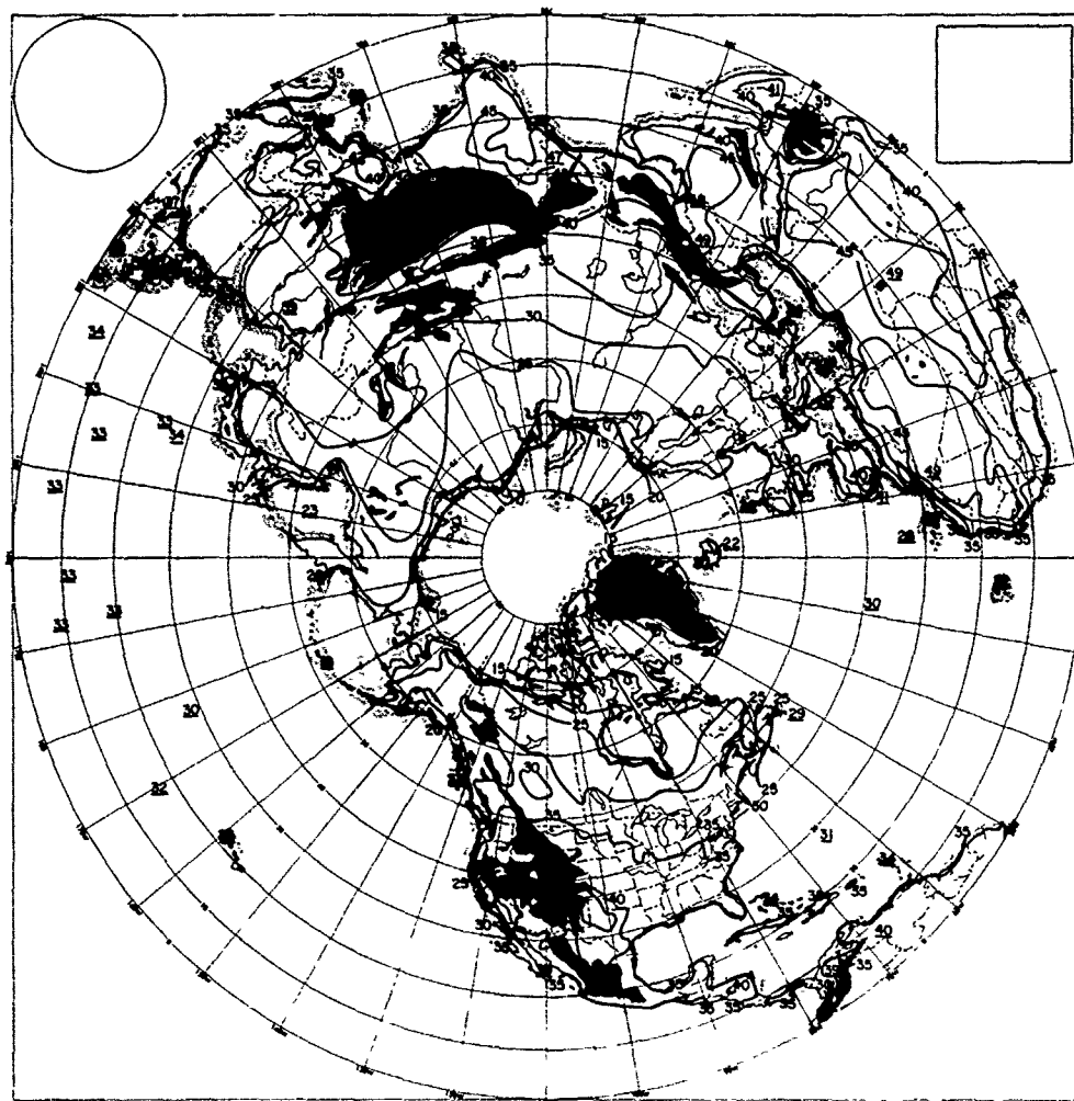
Figure 15.4. Temperature Equalled or Exceeded 1 Percent of the Time During the Warmest Month
