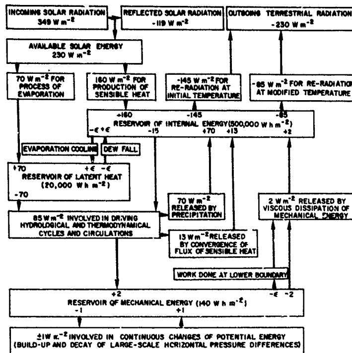
Figure 15.1. Global Mean Energy Cycles of the Atmosphere. A solar constant of 1395 \text{ W/m}^2 and a global albedo value of 0.34 are assumed. The average total incoming radiation to the globe is 1/4 of the solar constant. \epsilon denotes an average rate of less than 0.5 \text{ W/m}^2 . The estimated reliability of the solar constant is 3 percent; of the derived energy rates, this totals approximately 10 percent 1
