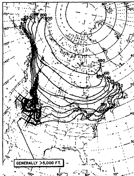
Figure 15.9. Expected Longest Duration (h) of Temperature \leq -23 C ( -10 F) During a Single Winter Season, From Tattelman 7
