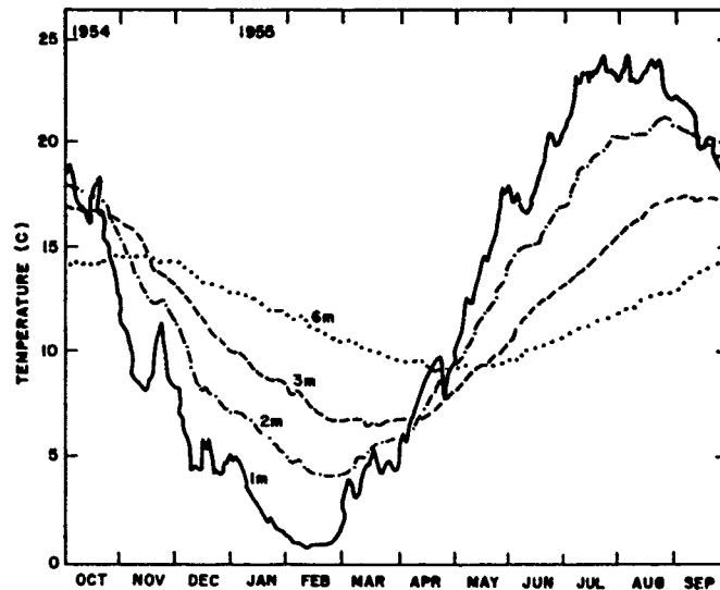
Figure 15.16. Variations of Soil Temperature at Indicated Depths, North Station, Brookhaven, Long Island, October 1954 Through September 1955, After Singer and Brown 14
