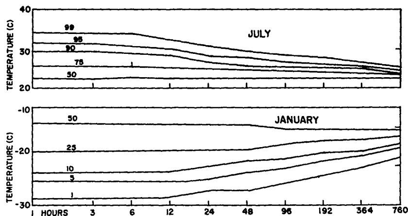
Figure 15.10. The Distribution of the Averages of Consecutive Hours of Temperature at Minneapolis, Minn. The upper half is for the mid-summer month from 1 July to 1 August; the lower half is for the mid-winter month from 1 January to 1 February. Each curve is labelled with percent probability of occurrence
