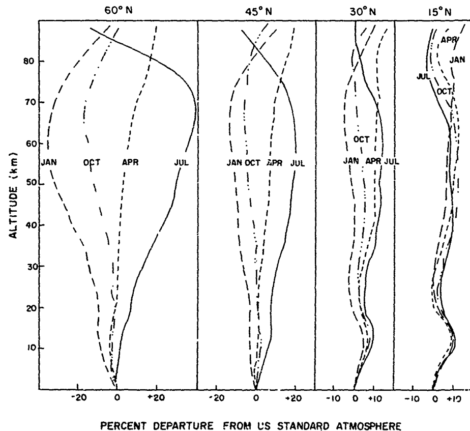
Figure 15.25. Pressure-Altitude Profiles for Midseason Months
