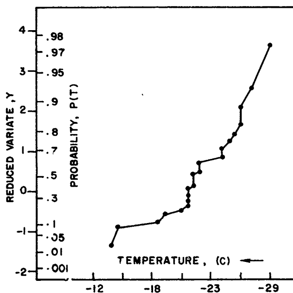
Figure 15.6b. Lowest Temperatures Occurring at Hanscom AFB, Mass. During 22 Winter Seasons (1943-1965) Ordered From Warmest to Coldest, and Plotted as the Probability That the Coldest Temperature Will Not Be Below the Given Value
