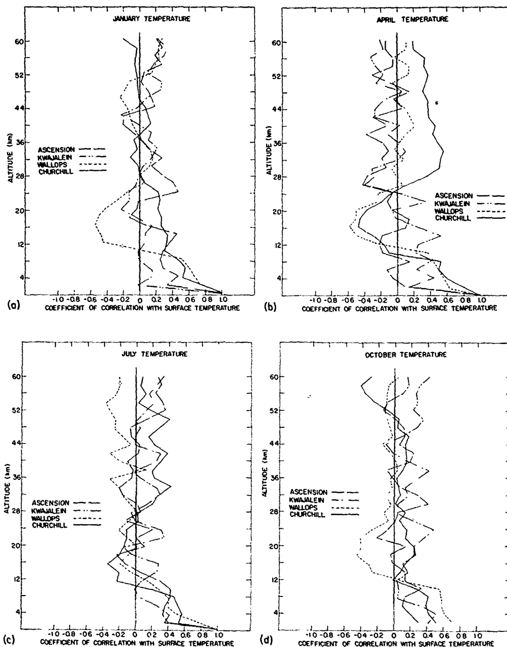
Figure 15.14. Vertical Profiles of Interlevel Coefficients of Correlation of Surface Temperature With Temperature at Other Altitudes up to 60 km for the Mid-Season Months at Ascension Island, Kwajalein, Wallops Island, and Ft. Churchill
