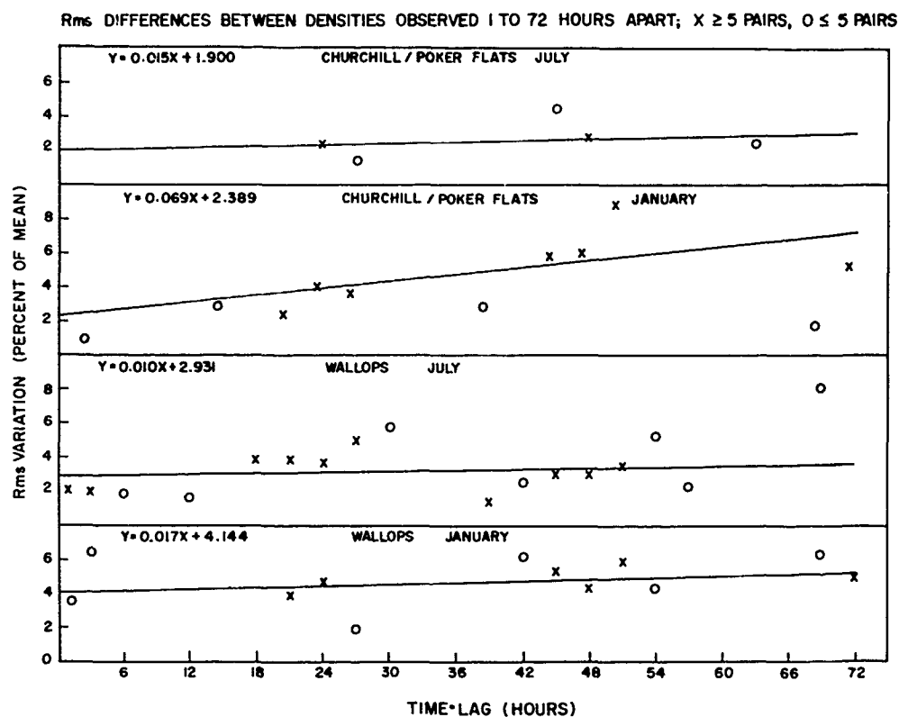
Figure 15.24. The rms Differences Between Densities Observed 1 to 72 h Apart at 50 km (x ≥ 5 pairs, o ≤ 5 pairs)
