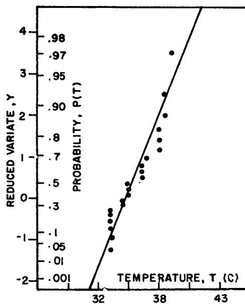
Figure 15.6a. Annual Highest Temperature, Hanscom AFB, Mass., 21 Ordered Values (1944-1964)
