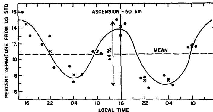
Figure 15.21. Diurnal Density (50 km) Variation at Ascension (Dots Indicate Observed Values, x's Represent 3-h Averages, and the Solid Line Depicts the Computed Diurnal Cycle)
