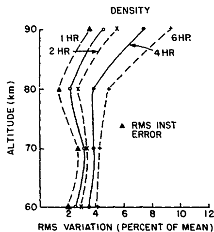
Figure 15.23. The rms Variation in Density for Time Lags of 1 to 6 h at Kwajalein.
