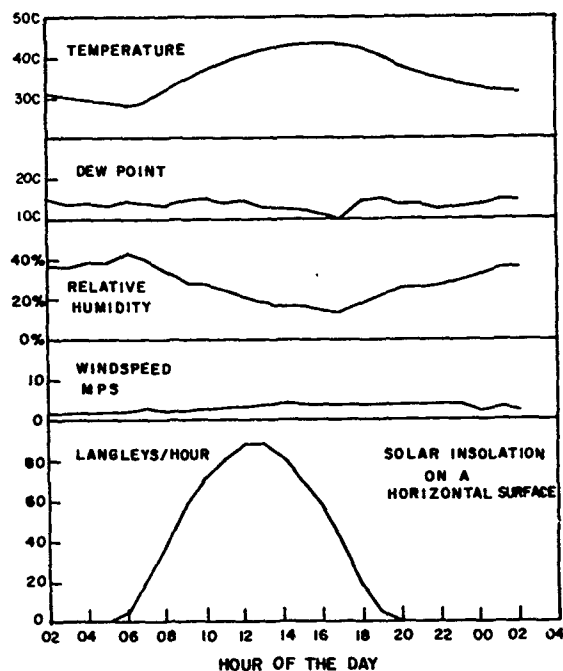
Figure 15.7. Yuma, Arizona Typical July Diurnal Cycles When Maximum Daily Temperature Equals or Exceeds 44 C (111 F), Based on 1961-1968 Data
