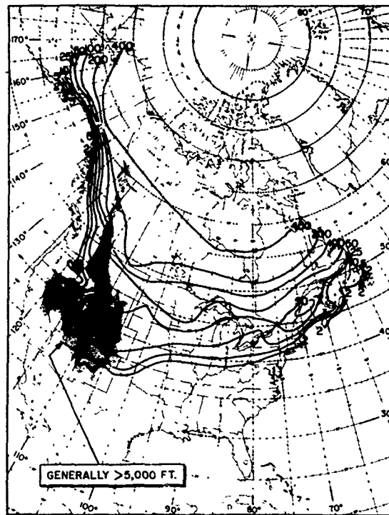
Figure 15.8. Longest Duration (h) of Temperature \leq -23^{\circ}\text{C} ( -10^{\circ}\text{F} ) in 10 Winters, From Tattelman 7
