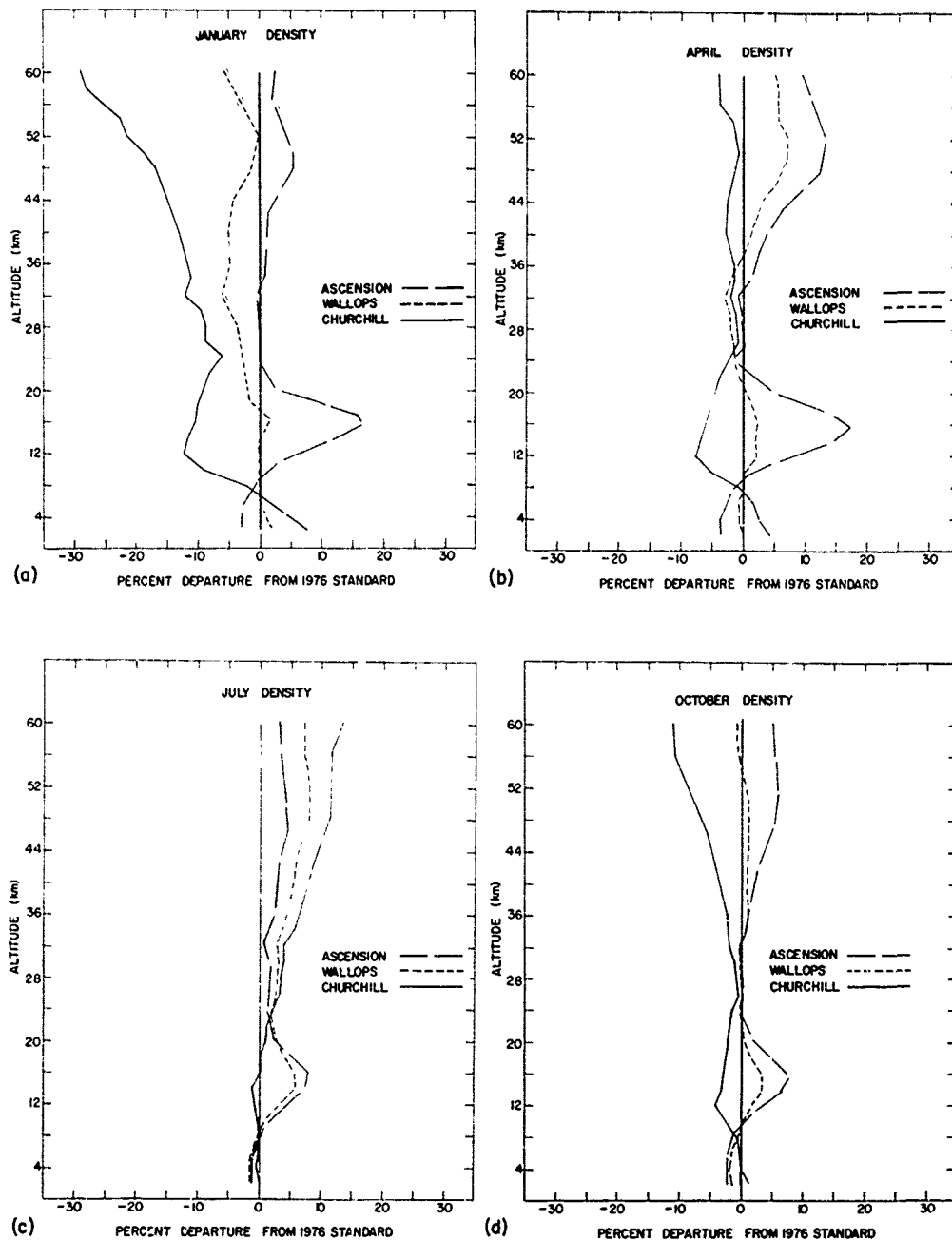
Figure 15.18. Latitudinal Differences in the Density-Altitude Profiles for the Mid-Season Months at Ascension Island, Wallops Island, and Ft. Churchill
