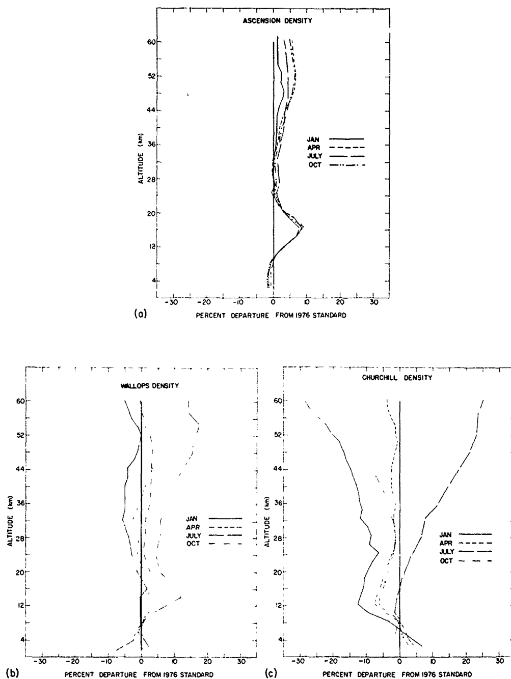
Figure 15.19. Seasonal Differences in the Density-Altitude Profiles at Ascension Island, Wallops Island, and Ft. Churchill
