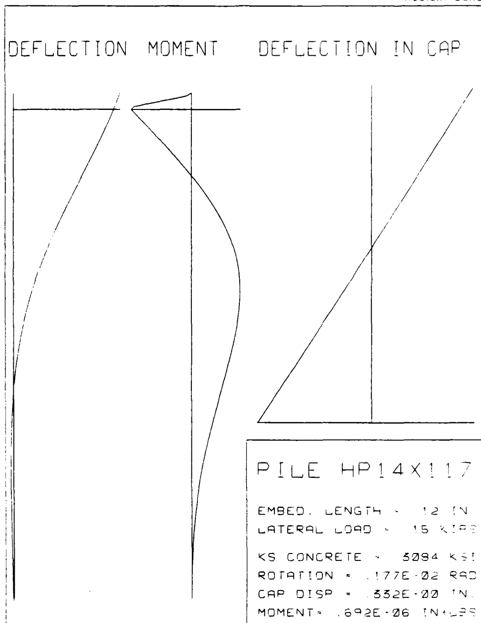
Figure 8. Typical moment and deflection curves for HP 14X117 pile with 12 in. embedment.
