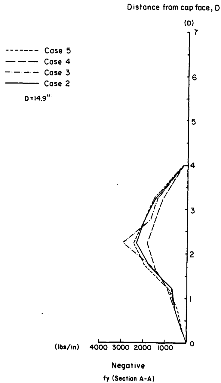
Figure 41. Shear force distribution at Section A-A for cap thickness of 4D.
