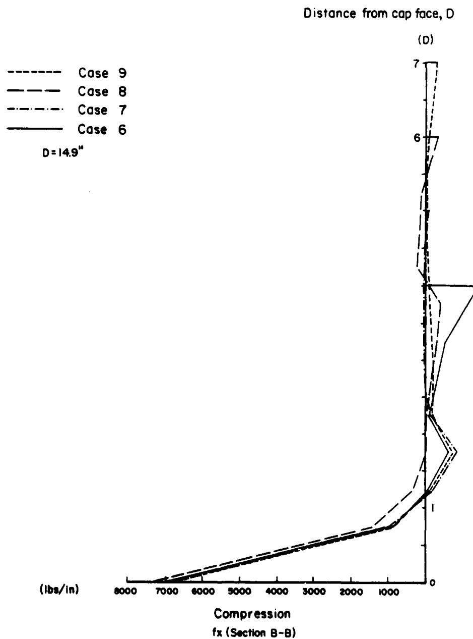
Figure 48. Normal force distribution at Section B-B for cap thicknesses of 4D to 7D.
