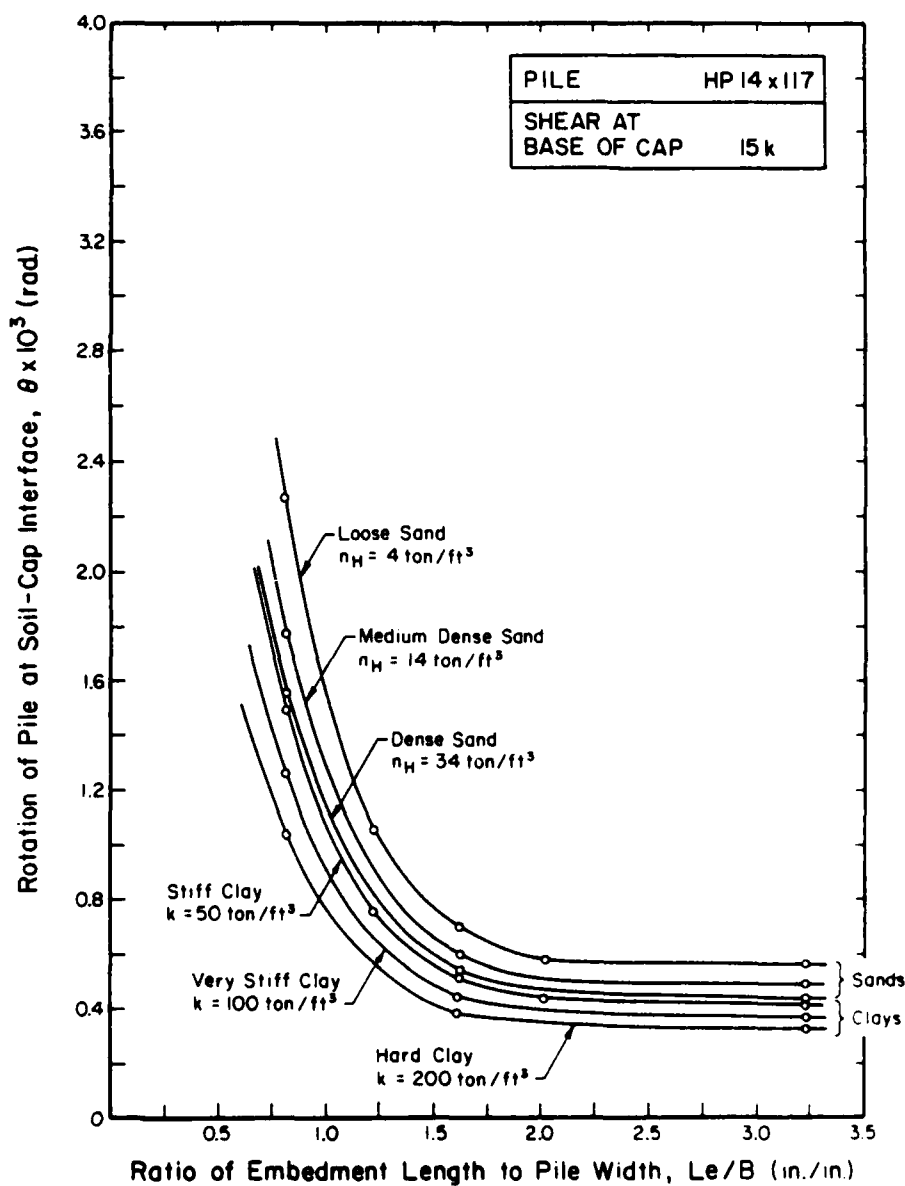
Figure 13. Effect of L_e/B ratio on pile rotation at soil-cap interface, HP 14X117 pile with 15 kip shear at base of cap.
