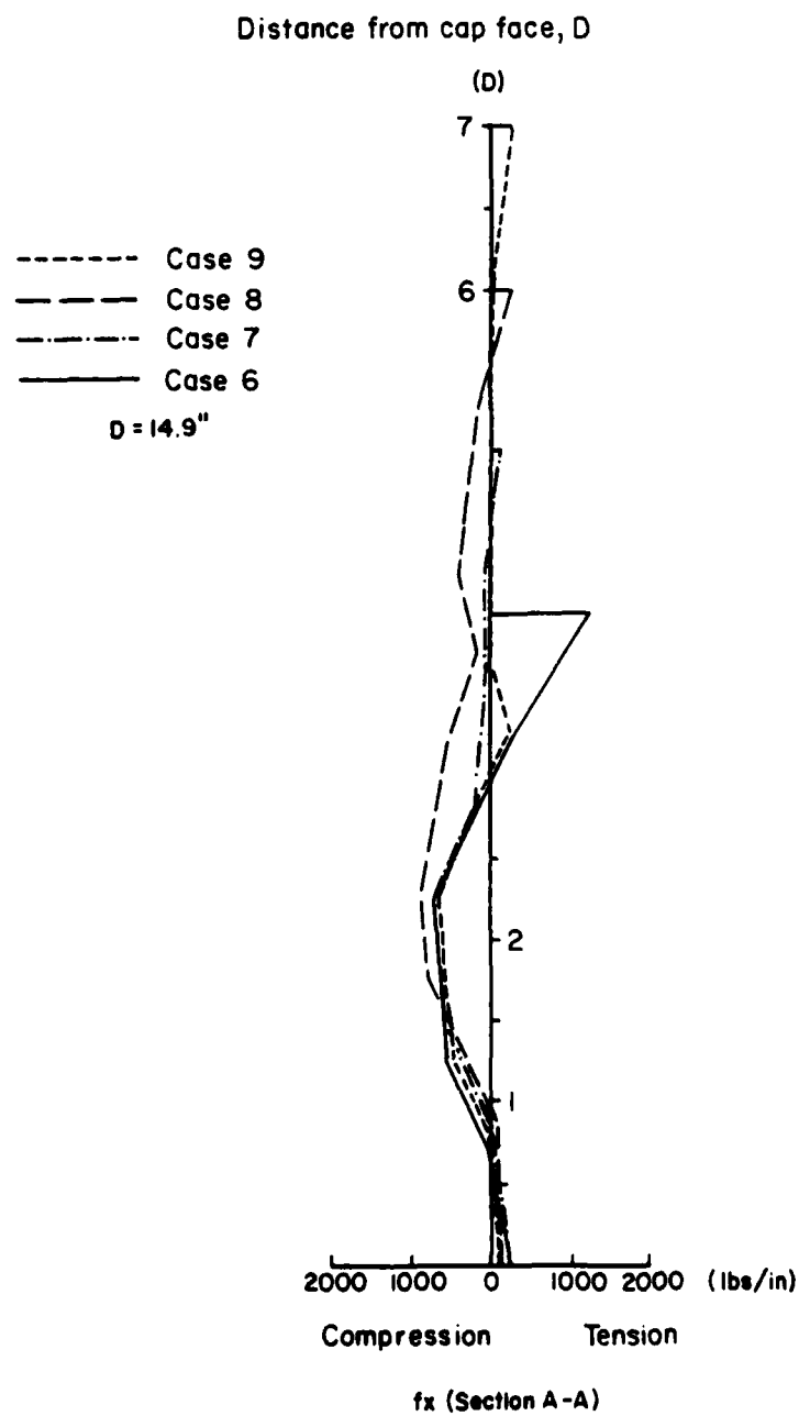
Figure 46. Normal force distribution at Section A-A for cap thicknesses of 4D to 7D.
