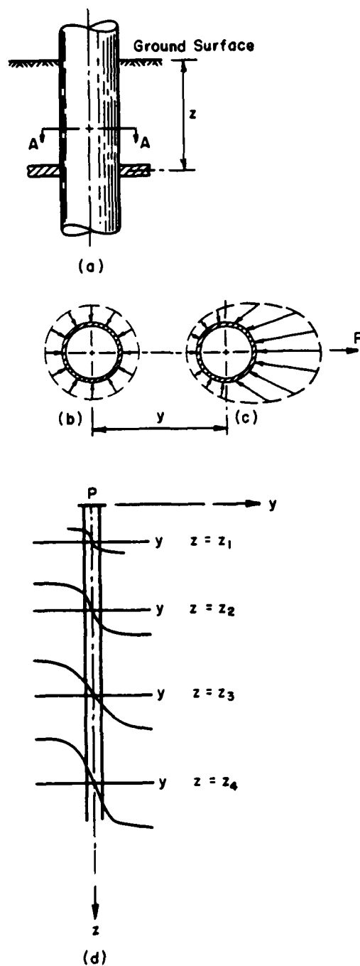
Figure 3. Graphical definition of p and y.
