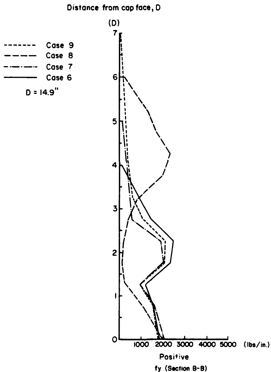
Figure 49. Shear force distribution at Section B-B for cap thicknesses of 4D to 7D.
