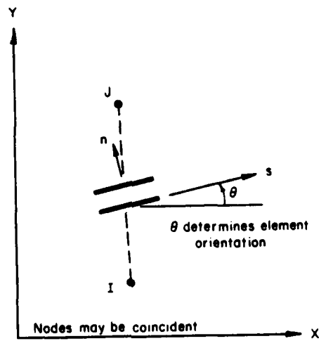
Figure 24. Two-dimensional interface element.
