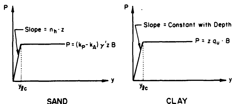
Figure 4. Typical load-deformation curves ( p - y curves) for sands and clays.
