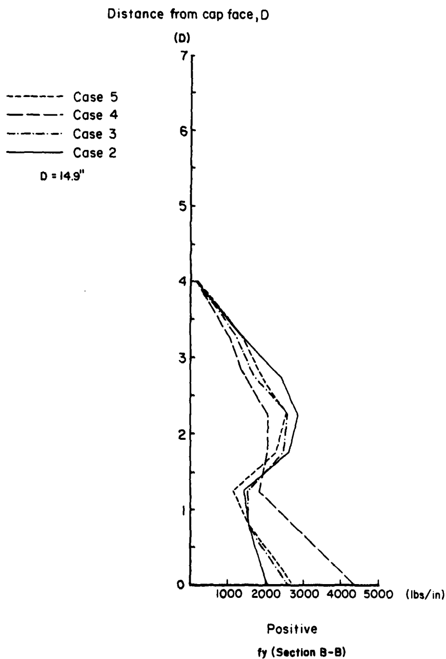
Figure 43. Shear force distribution at Section B-B for cap thickness of 4D.
