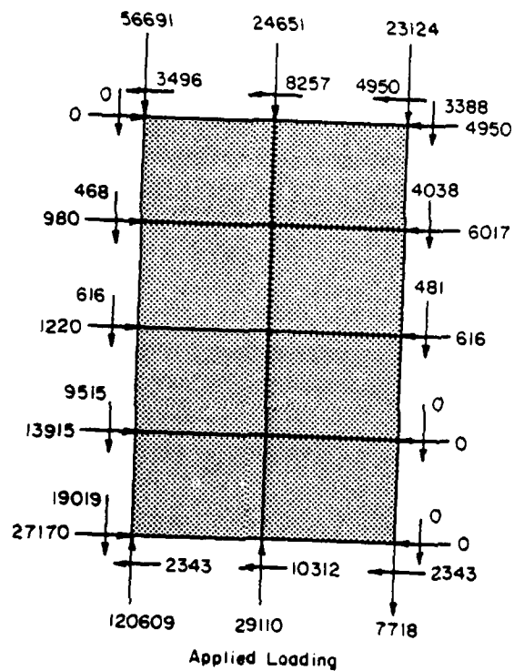
Figure 37. Interface element forces for HP 14X117 pile with 2D embedment, \mu = 0.7 .
