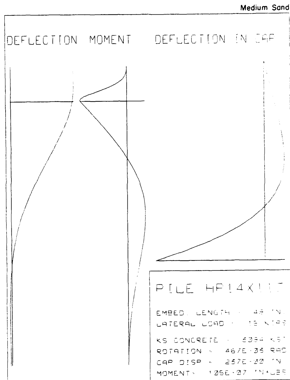
Figure 9. Typical moment and deflection curves for HP 14X117 pile with 48 in. embedment.
