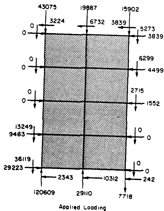
Figure 38. Interface element forces for HP 14X117 pile with 2D embedment, \mu = 1.4 .
