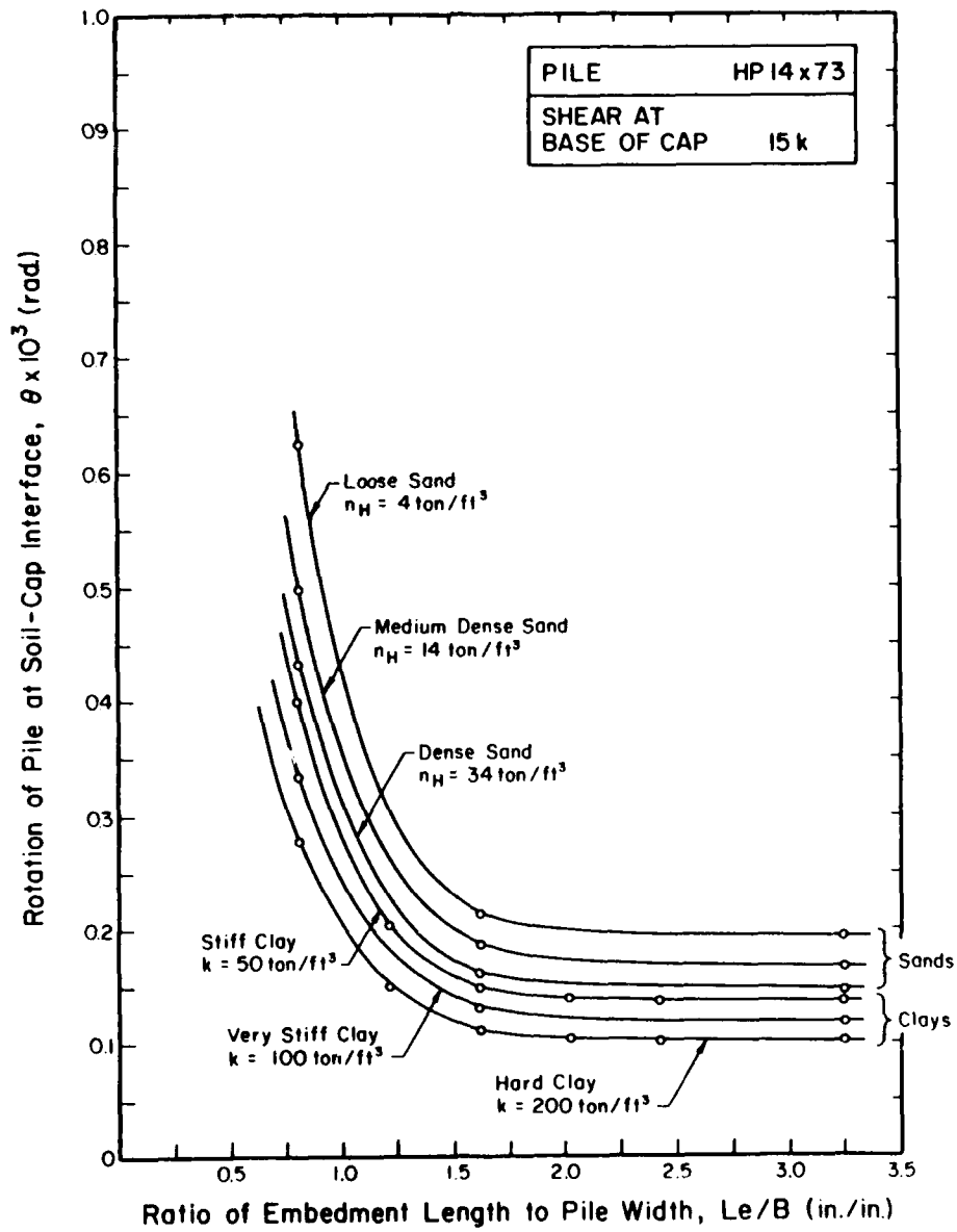
Figure 12. Effect of L_e/B ratio on pile rotation at soil-cap interface, HP 14X73 pile with 15 kip shear at base of cap.
