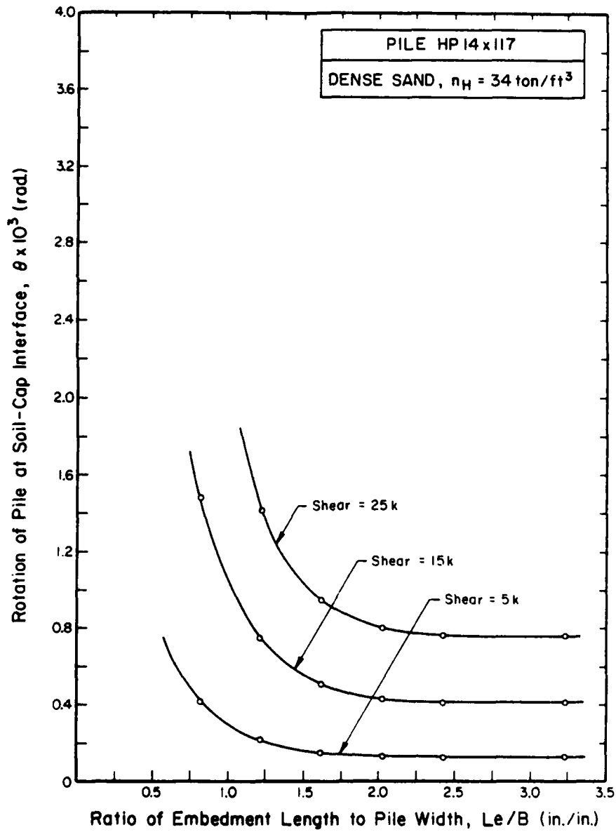
Figure 15. Effect of L_e/B ratio on pile rotation at soil-cap interface, HP 14X117 pile in dense sand, n_h = 34 \text{ ton/cu ft} .
