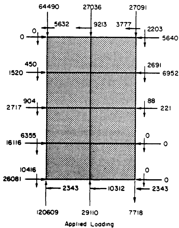
Figure 34. Interface element forces for HP 14X117 pile with 2D embedment, \mu = 0.4 .
