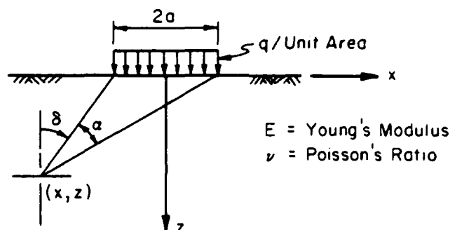
Figure 5. Elastic half-space under a strip load, generalized solution.
