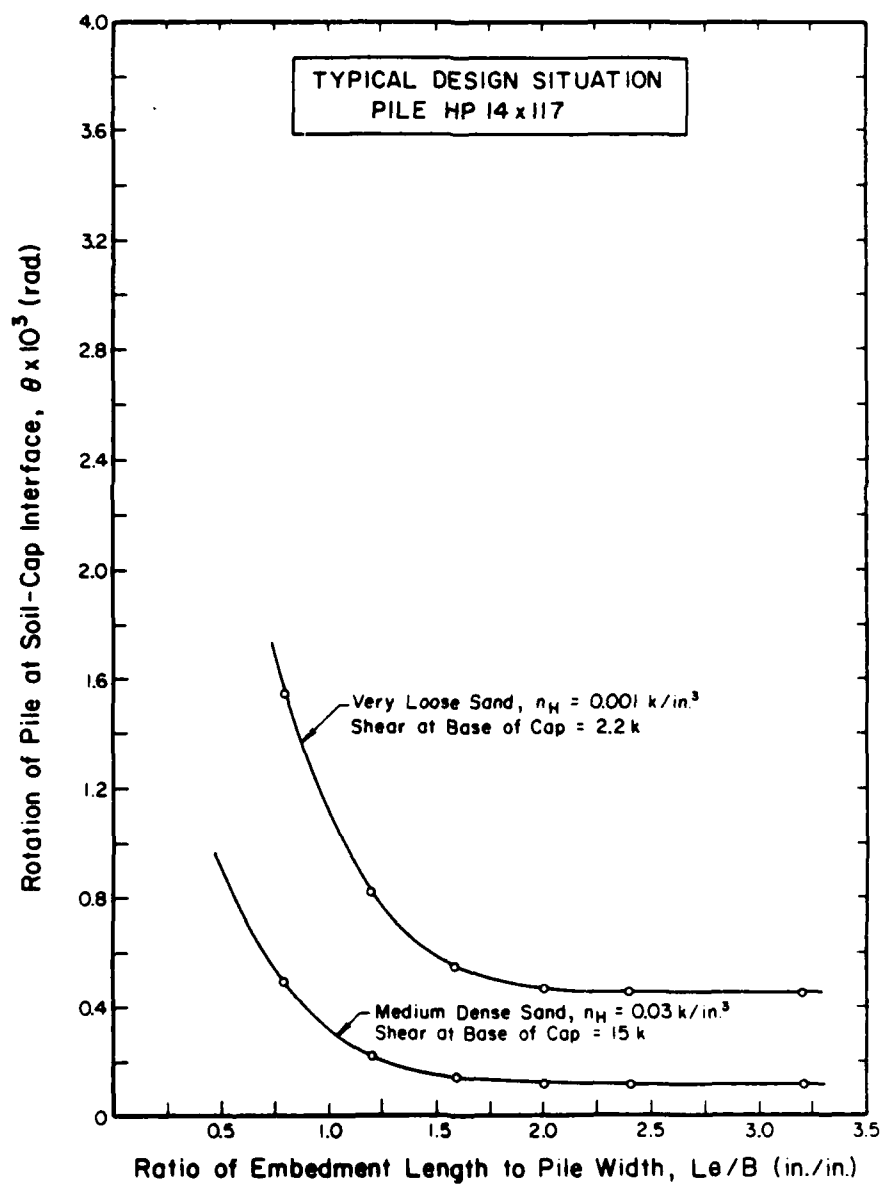
Figure 11. Effect of L_e/B ratio on pile rotation at soil-cap interface, typical design situation for HP 14X117 pile.
