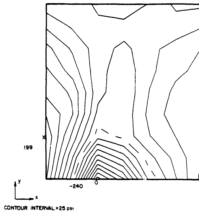
Figure 30. Typical Stress Contour Plot for \sigma_{max} .
