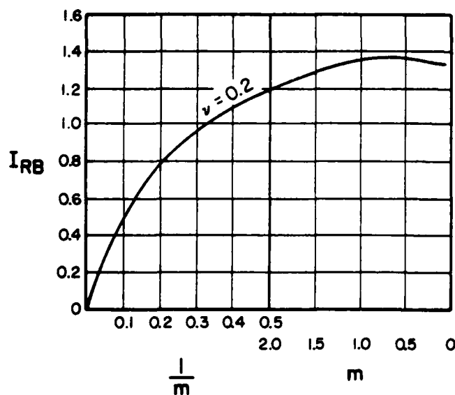
Figure 7. Plot of I_{RB} in terms of m = 4a and \nu = 0.2 .
