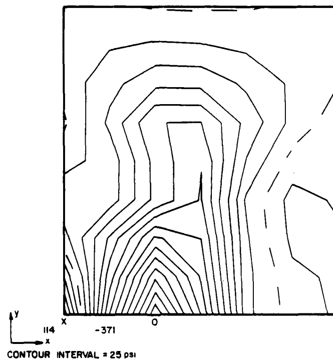
Figure 28. Typical Stress Contour Plot for \sigma_y .
