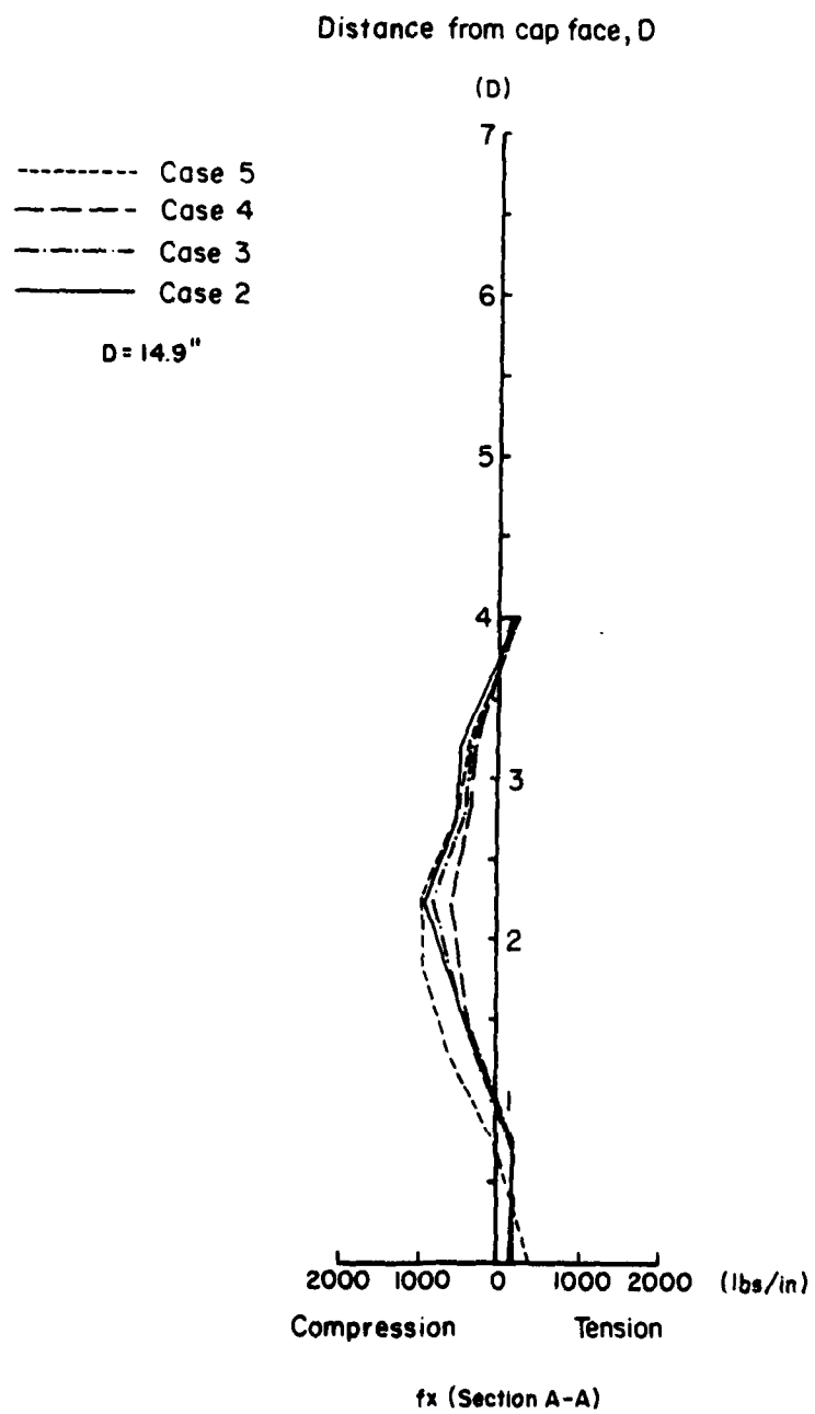
Figure 40. Normal force distribution at Section A-A for cap thickness of 4D.
