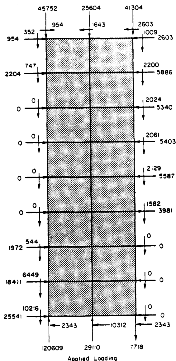
Figure 35. Interface element forces for HP 14X117 pile with 4D embedment, \mu = 0.4 .
