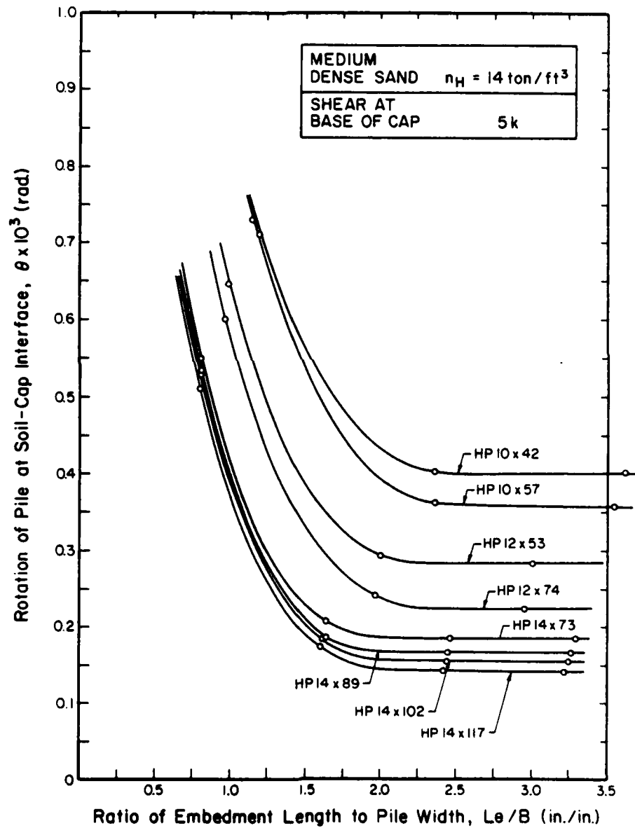
Figure 18. Effect of L_e/B ratio on pile rotation at soil-cap interface, various pile sections in medium dense sand with 5 kip shear at base of cap.
