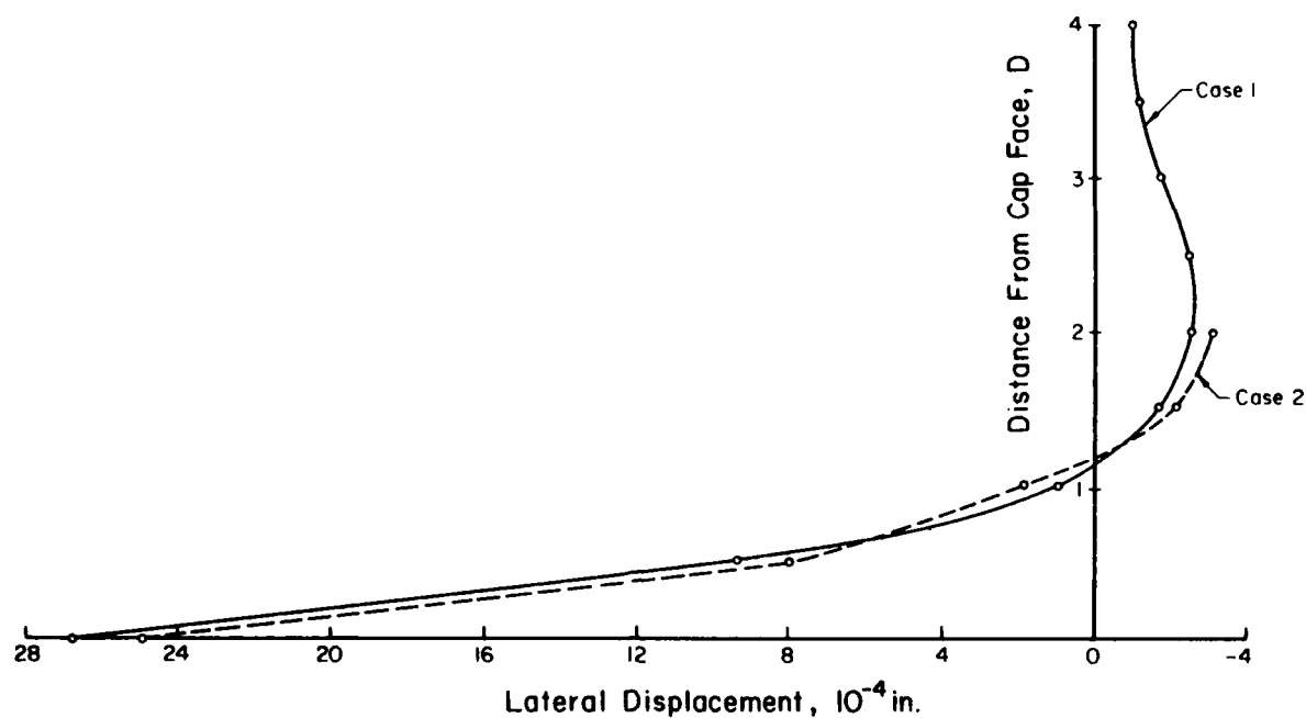
Figure 33. Lateral displacement curves for centerline of HP 14X117 pile with 2D and 4D embedments, \mu = 0.4 .
