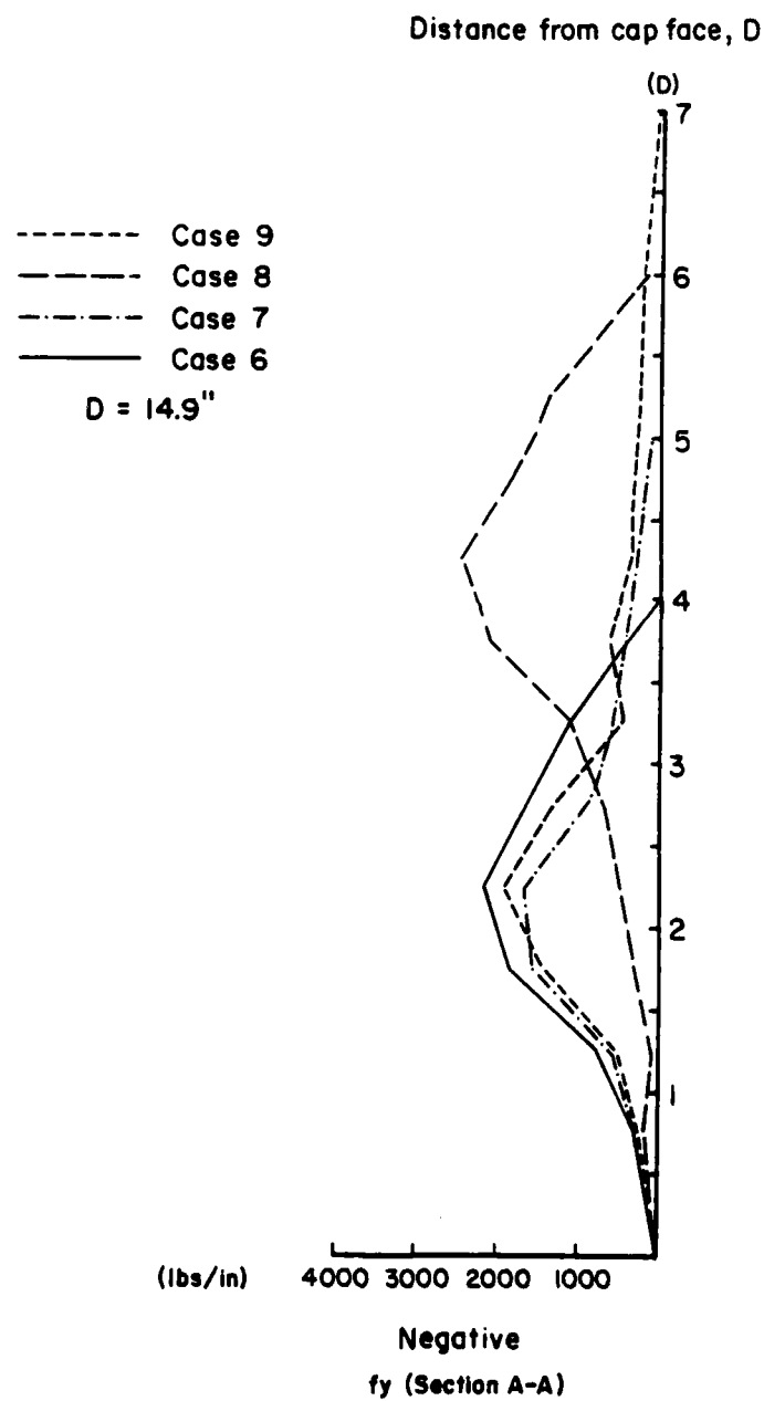
Figure 47. Shear force distribution at Section A-A for cap thicknesses of 4D to 7D.
