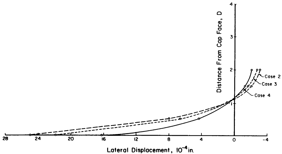
Figure 36. Lateral displacement curves for centerline of HP 14X117 pile with 2D embedment, \mu = 0.4, 0.7 , and 1.4 .
