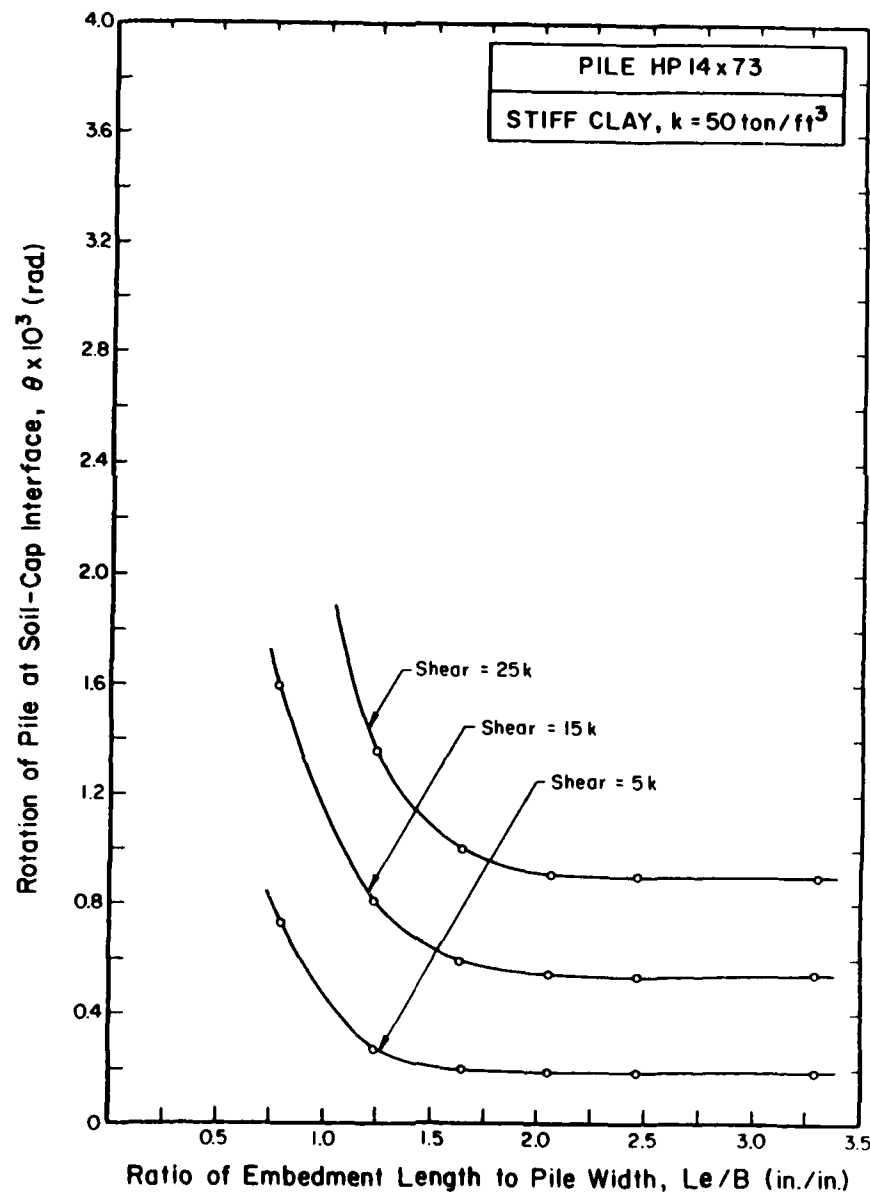
Figure 16. Effect of L_e/B ratio on pile rotation at soil-cap interface, HP 14X73 pile in stiff clay, k = 50 \text{ tons/cu ft}
