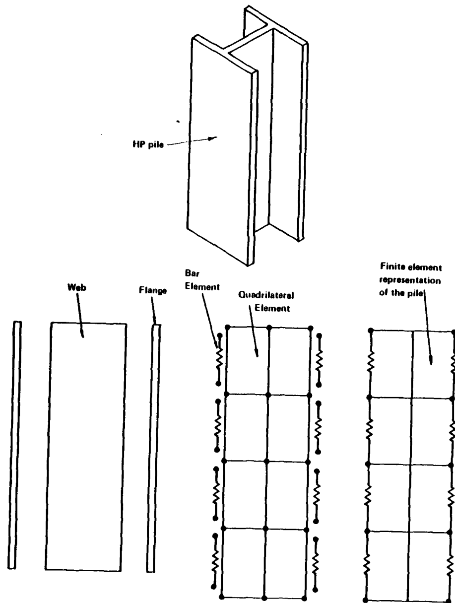
Figure 23. Finite element representation of HP pile.
