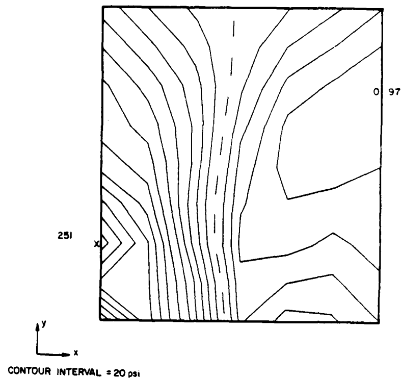
Figure 29. Typical Stress Contour Plot for \tau_{xy} .
