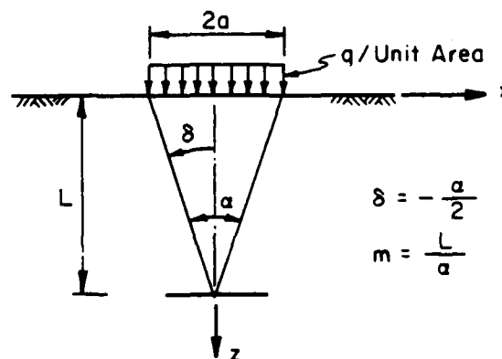
Figure 6. Elastic half-space under a strip load, centralized solution.
