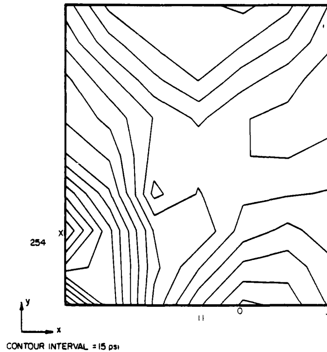
Figure 32. Typical Stress Contour Plot for \tau_{\max} .
