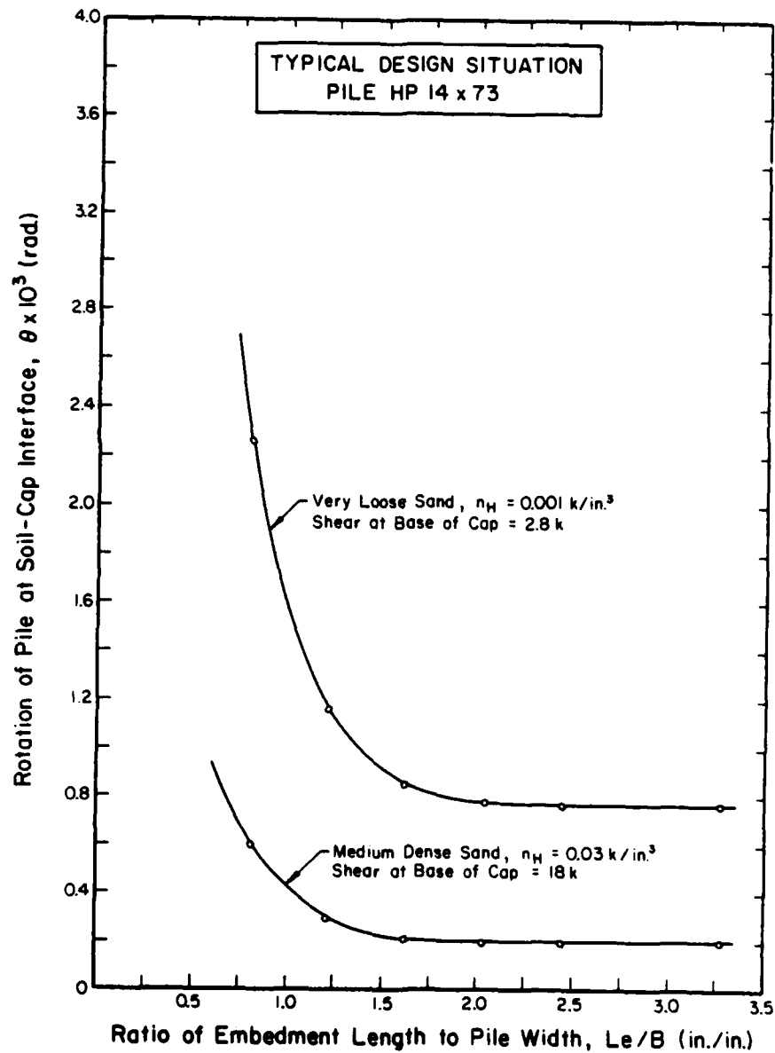
Figure 10. Effect of L_e/B ratio on pile rotation at soil-cap interface, typical design situation for HP 14X73 pile.
