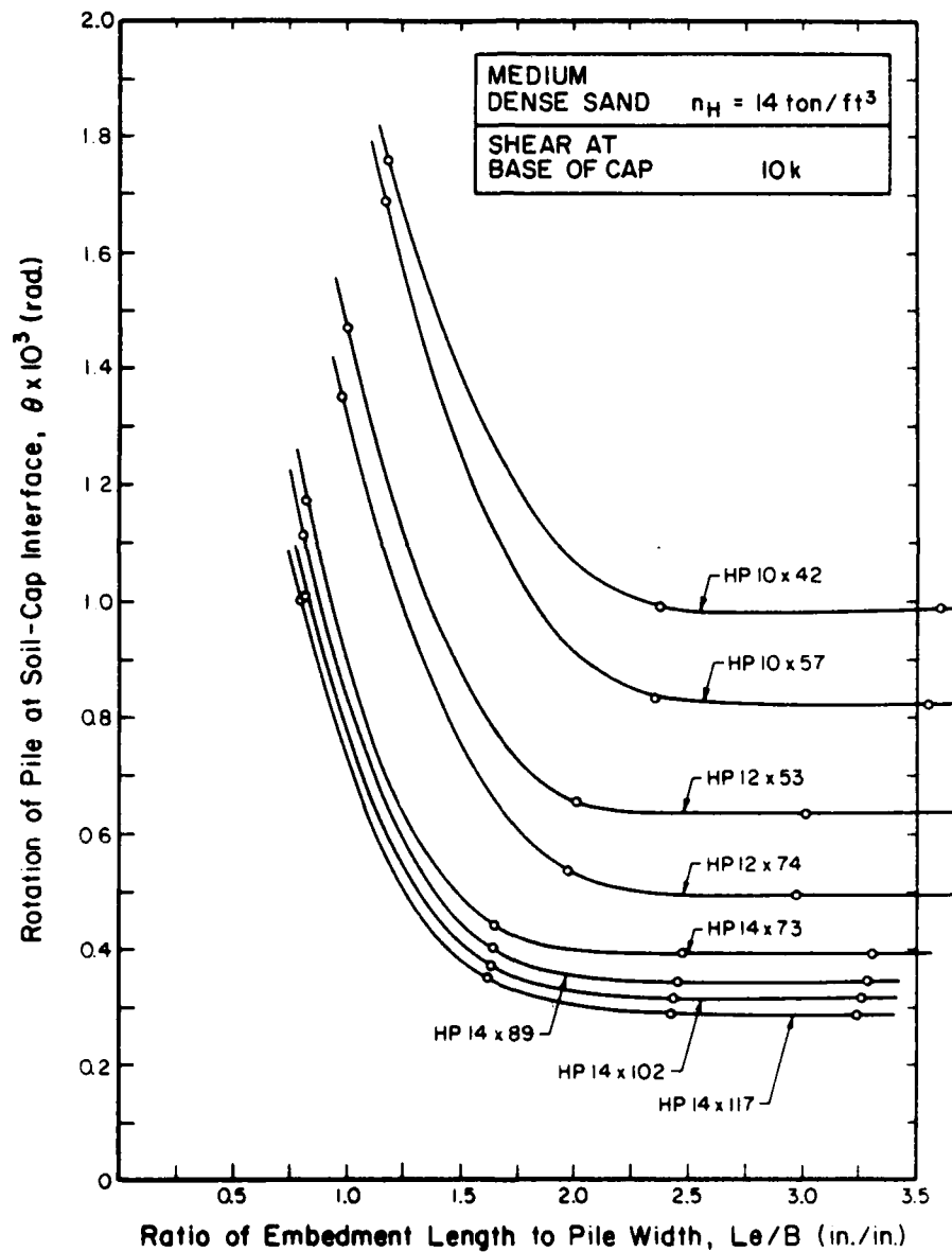
Figure 19. Effect of L_e/B ratio on pile rotation at soil-cap interface, various pile sections in medium dense sand with 10 kip shear at base of cap.
