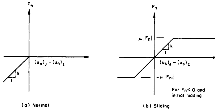
Figure 25. Force-deflection relationship for the interface element.
