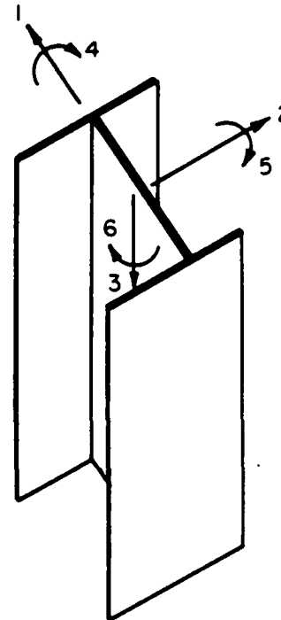
Figure 2. Design loadings for HP 14X73 and HP 14X117 piles.
