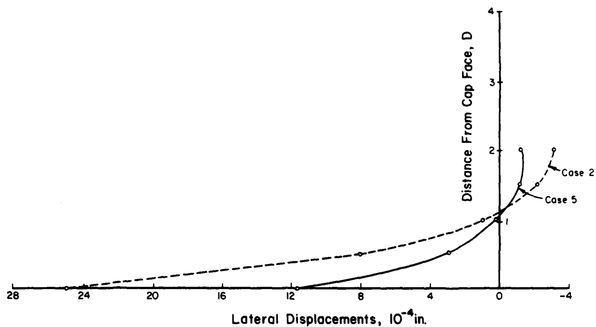
Figure 44. Lateral displacement curves for centerline of HP 14X117 pile for effective widths of concrete cap of 14.9 in. and 44.7 in.
