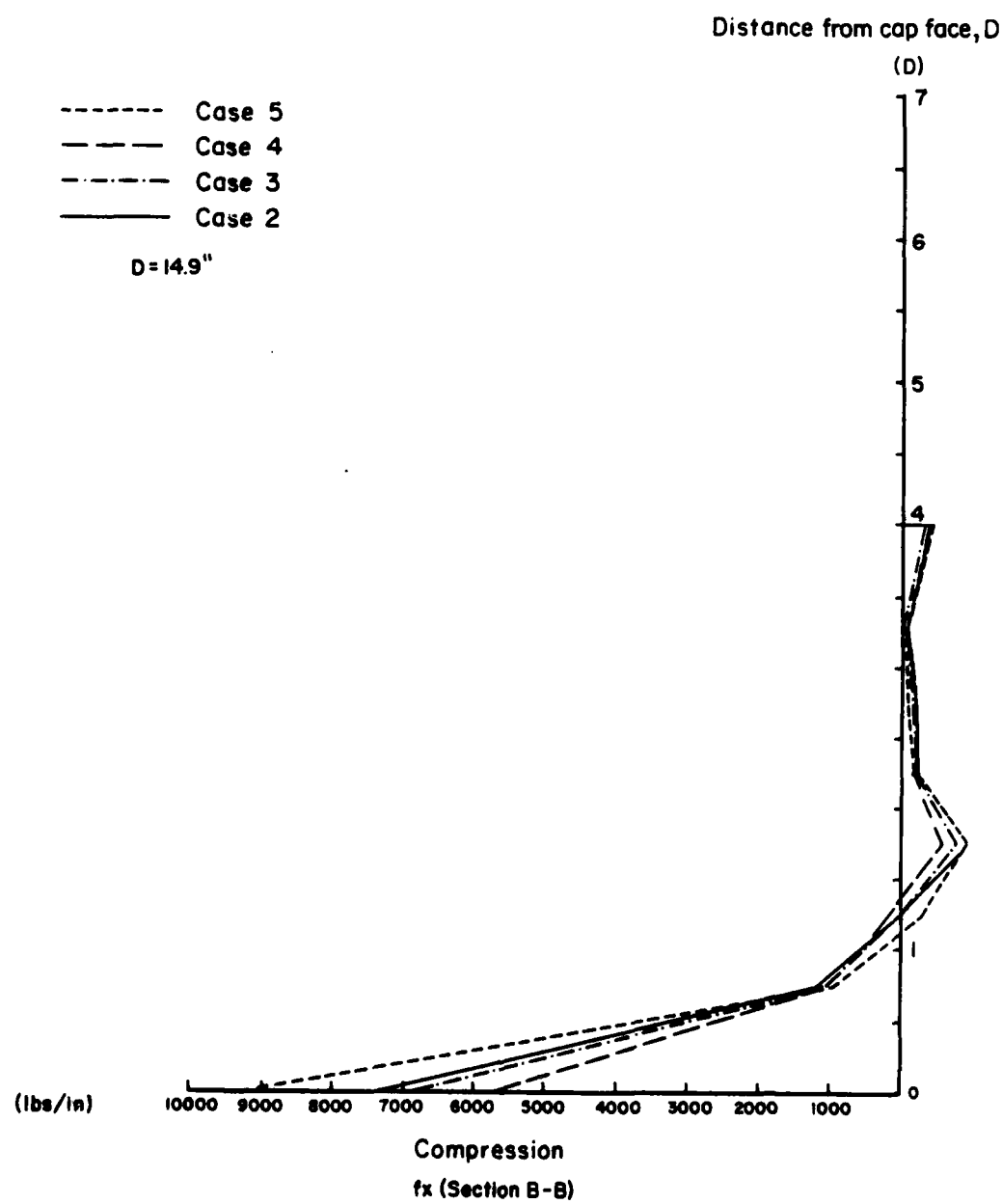
Figure 42. Normal force distribution at Section B-B for cap thickness of 4D.
