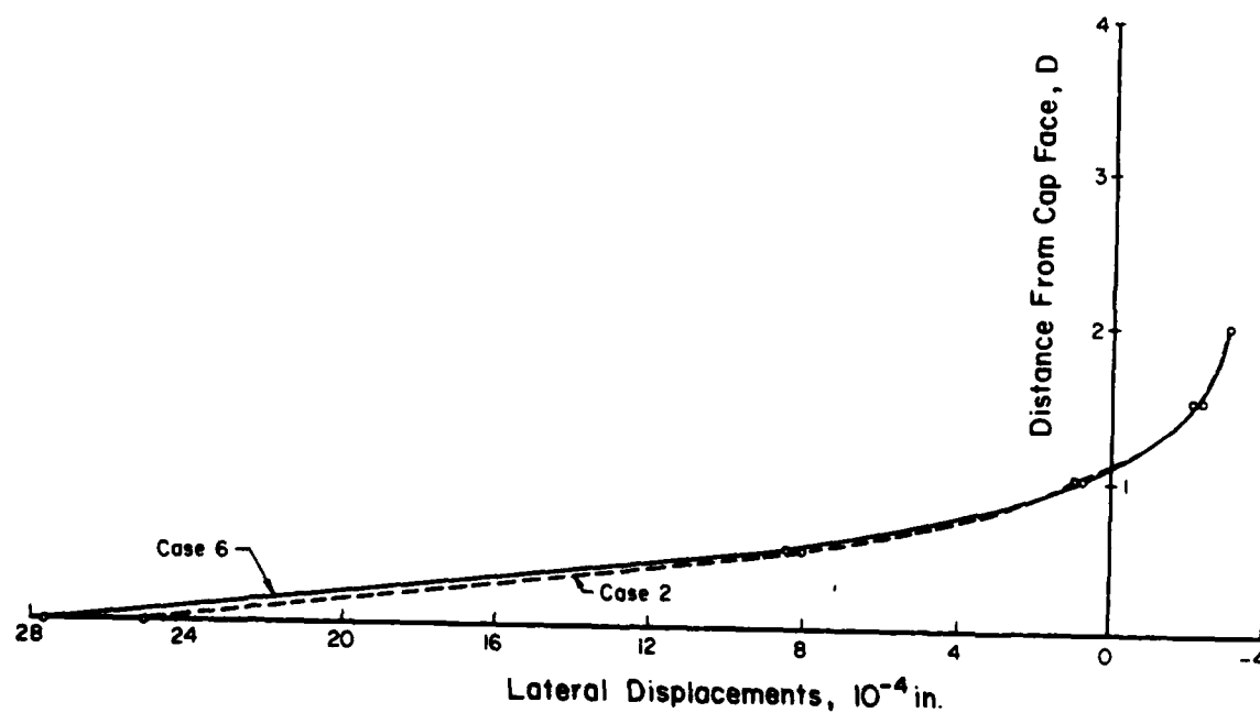
Figure 45. Lateral displacement curves for centerline of HP 14X117 pile for pile spacings of 3D to 5D.
