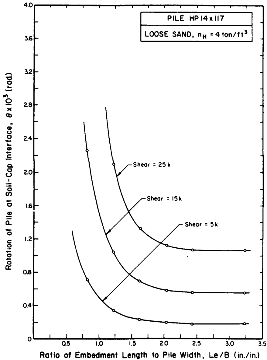
Figure 14. Effect of L_e/B ratio of pile rotation at soil-cap interface, HP 14X117 pile in loose sand, n_h = 4 \text{ ton/cu ft.}
