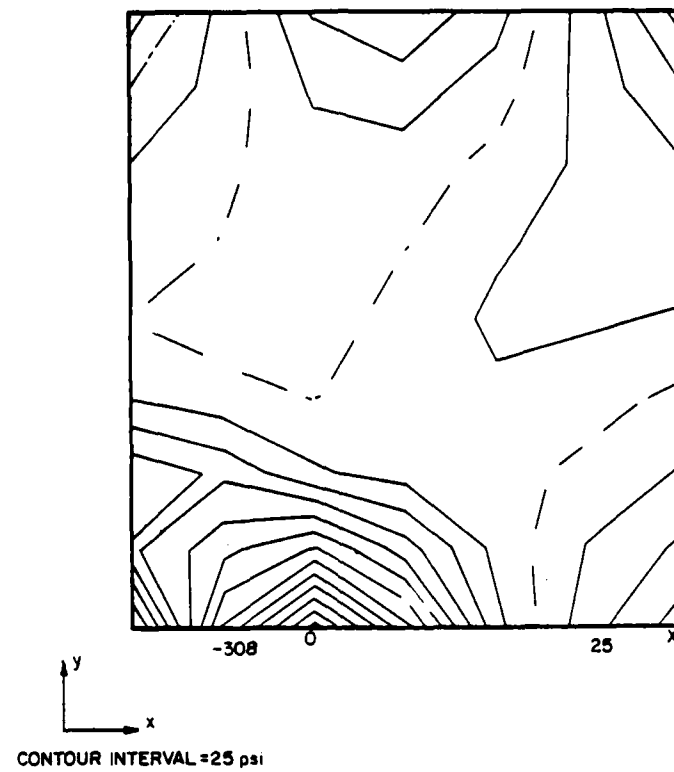
Figure 27. Typical Stress Contour Plot for \sigma_x .
