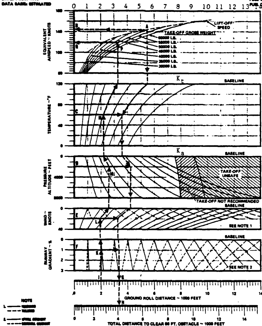
Figure 11-12 Normal Takeoff Distance and Line Speed Check
