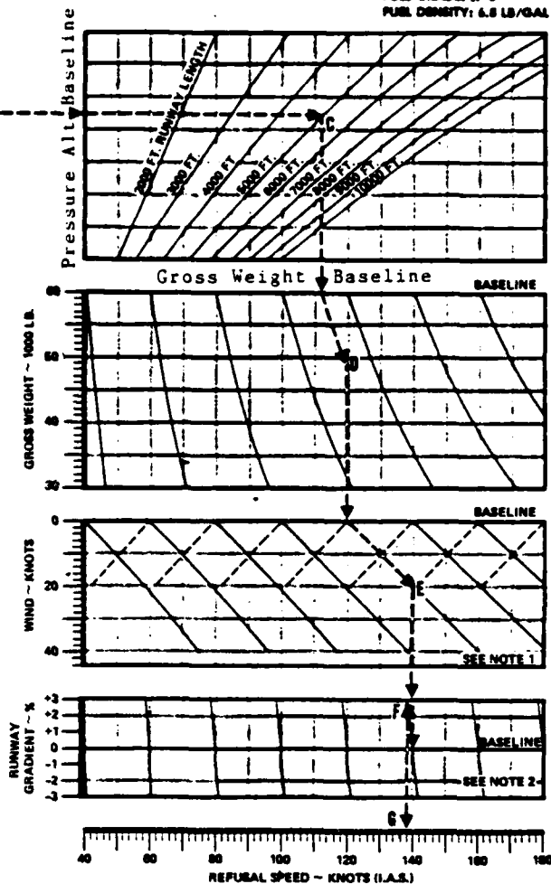
Figure 11-11 Maximum Refusal Speed (Single Engine)
