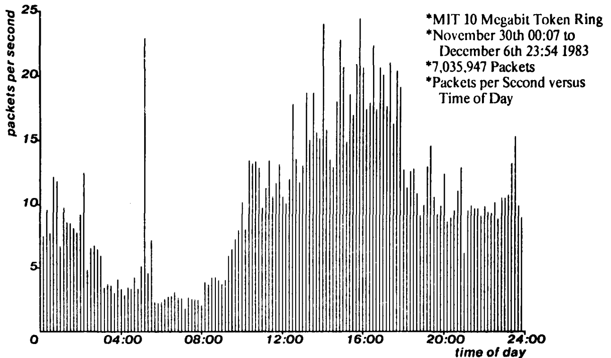
Figure 4-1: Packets per Second versus Time of Day
