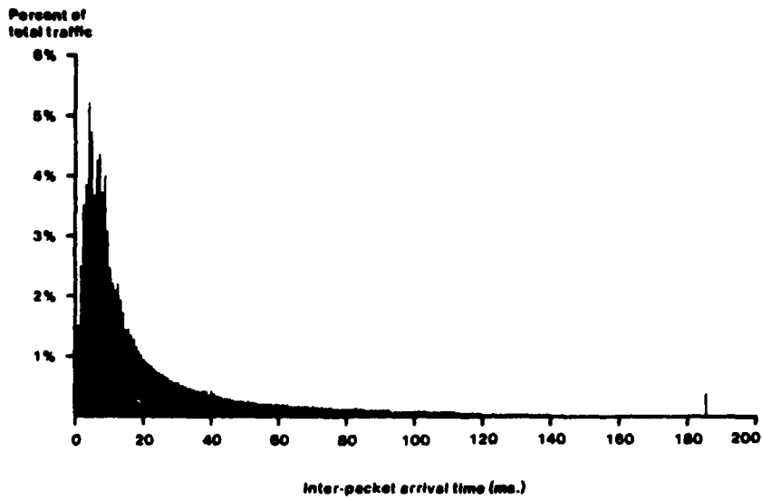
Figure 5-10: Ethernet Histogram of Interpacket Arrival Time
