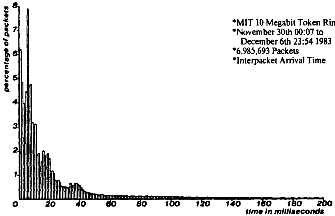
Figure 5-11: Version 2 Ring Histogram of Interpacket Arrival Time
