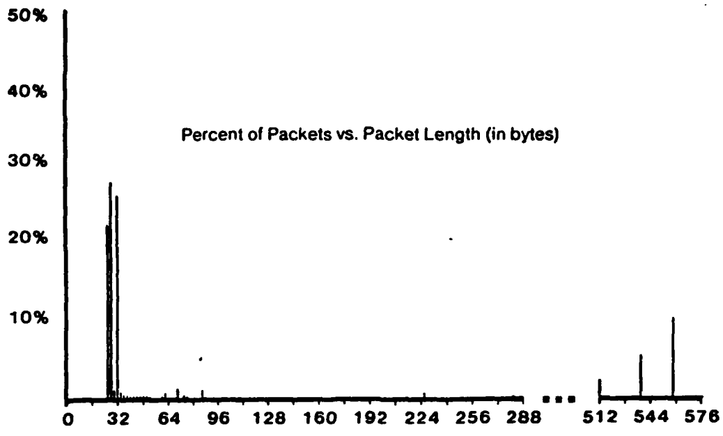
Figure 5-4: Ethernet Percentage of Packets versus Packet Length
