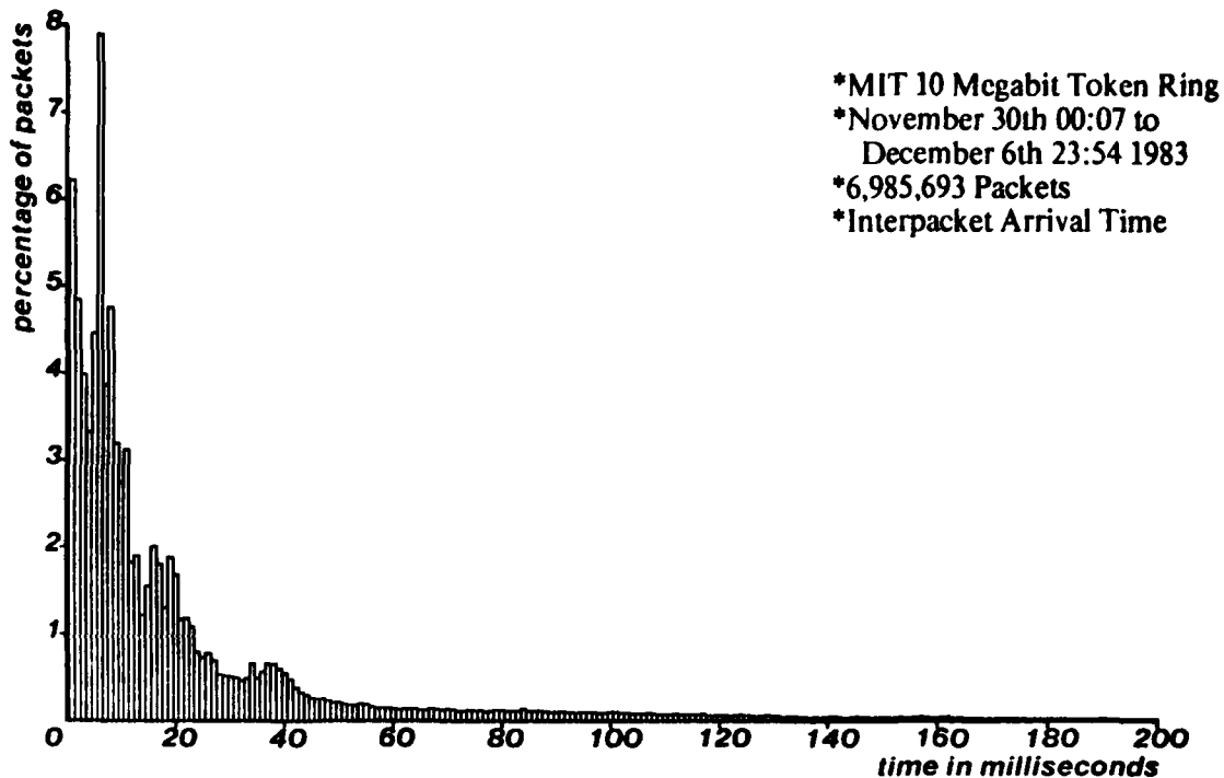
Figure 4-5:Percentage of Packets versus Interpacket Arrival Time
