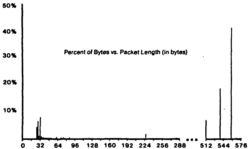
Figure 5-6: Ethernet Percentage of Bytes versus Packet Length
