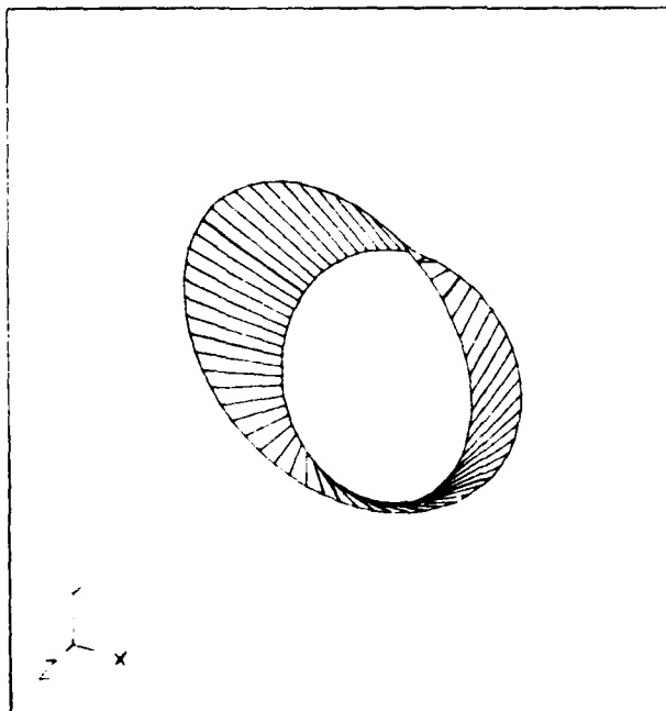
Figure 17 - Undistorted Mobius Strip
