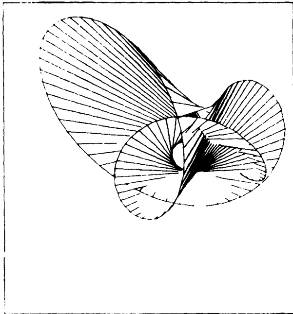
Figure 16 - Distorted Mobius Strip
