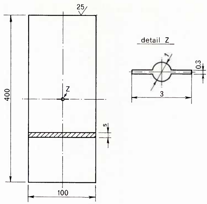
Fig. 4.2-13 Crack propagation specimen, (Ref. 25).
