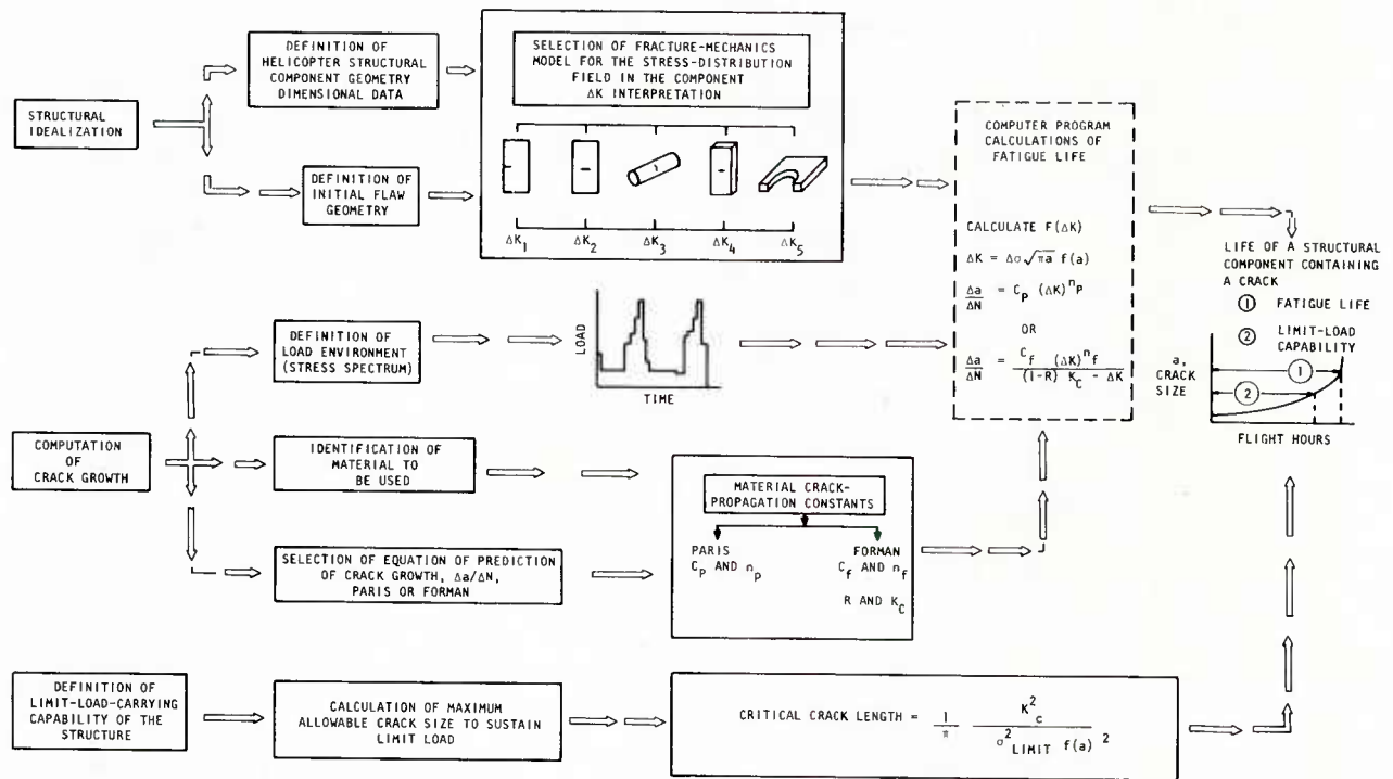
FIGURE 5.17 METHODOLOGY FOR PREDICTING LIMITED DAMAGE GROWTH IN HELICOPTER STRUCTURAL COMPONENTS
