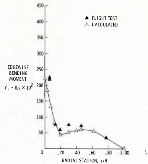
FIG. 321-26 CORRELATION OF WG 30 MAIN ROTOR EDGEWISE BENDING MOMENT WITH R150 ANALYSIS RESULTS
