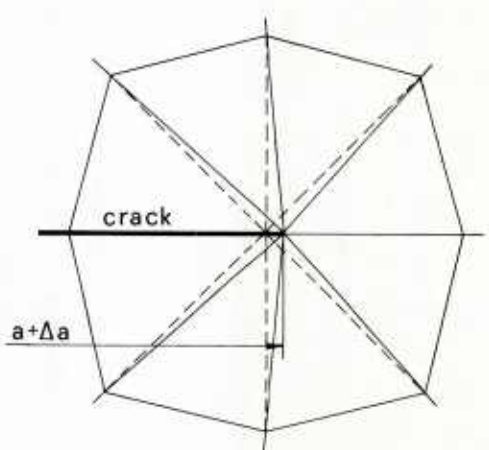
Fig. 4.2-25 Evaluation of energy rate per crack increment, \Delta a .
