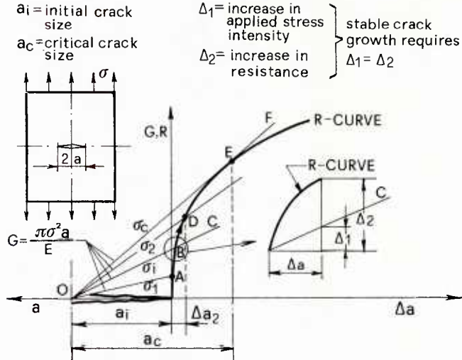
Fig. 4.2-41 R-curve concept in unstiffened panels (From Ref. 40).
