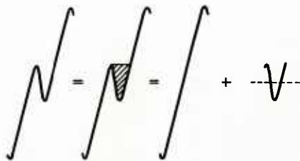
Fig. 34.4 Range pair counting principle
