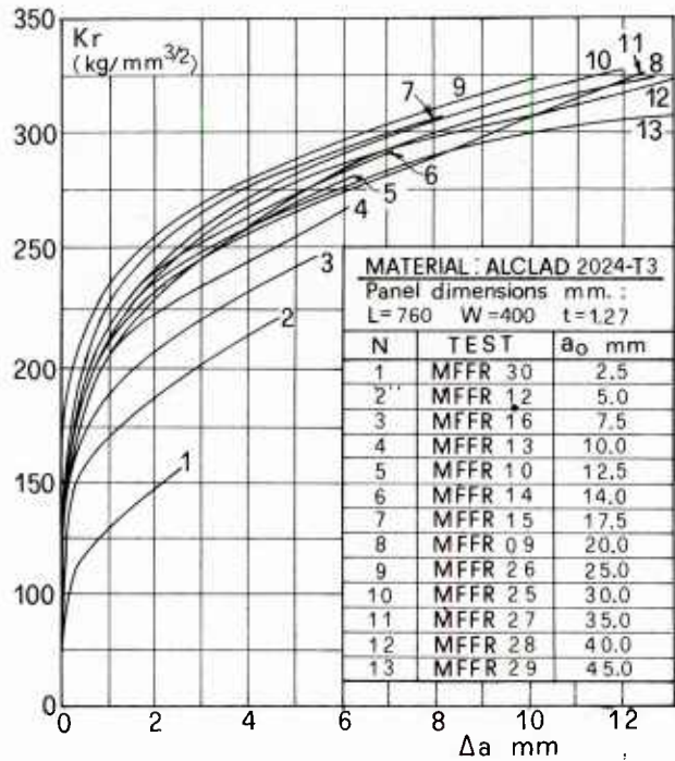
Fig. 4.2-42 Experimental R-curves for aluminum alloy 2024-T3. Kr is defined as (ER)^{\frac{1}{2}} . (From Ref. 48).
