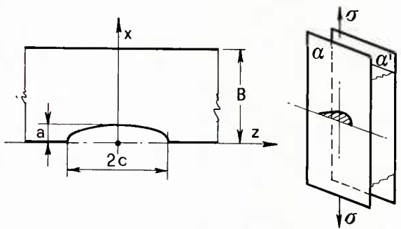
Fig. 4.2-27 Surface elliptical crack.
