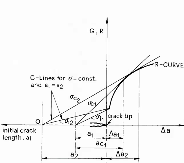
Fig. 4.2-40 R-curve in plane stress (schematic) (From Ref. 40).
