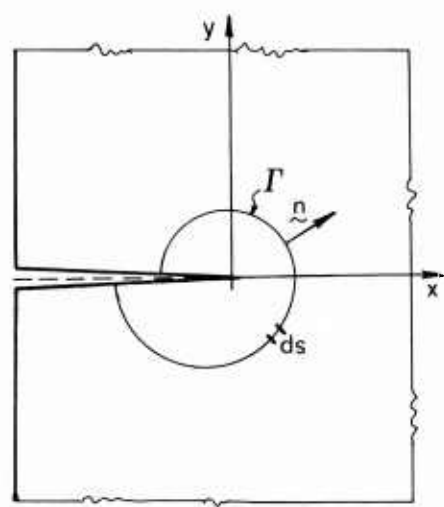
Fig. 4.2-26 J-Integral integration path.
