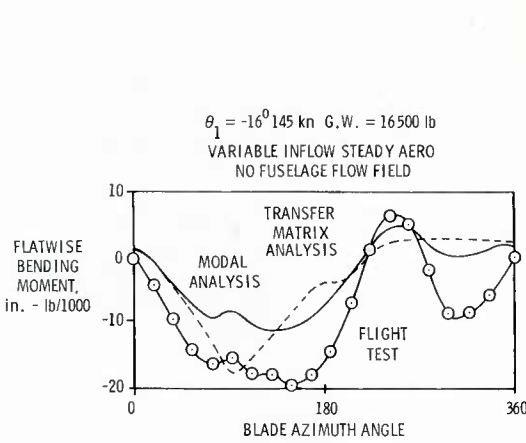
FIG. 321-7 COMPARISON OF MODAL ANALYSIS AND TRANSFER MATRIX ANALYTIC RESULTS WITH FLIGHT TEST
