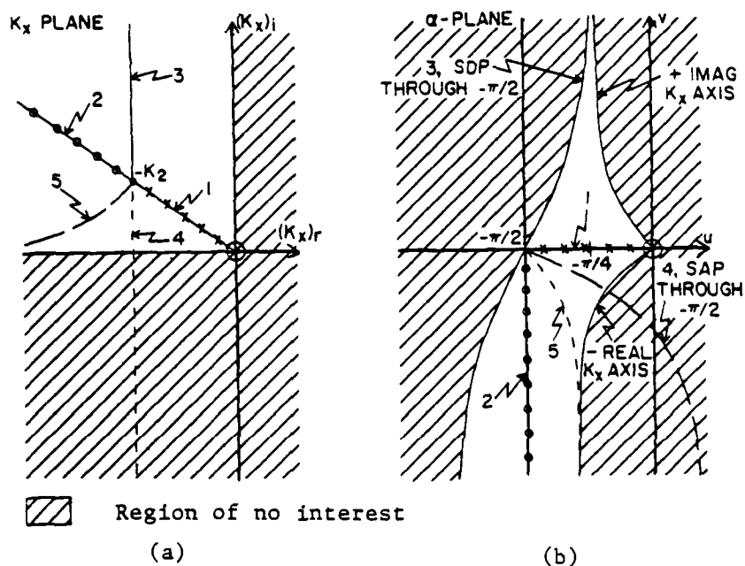
Figure A.3. Prominent lines in the k_x plane and their projections in the \alpha plane.
