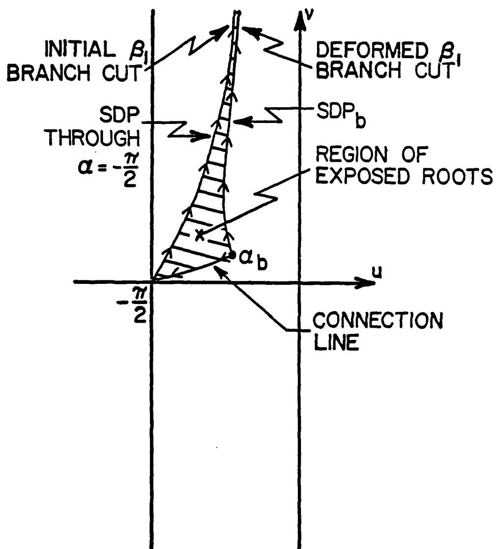
Figure C.5. Possible region of exposed roots of G_- in the \alpha plane.
