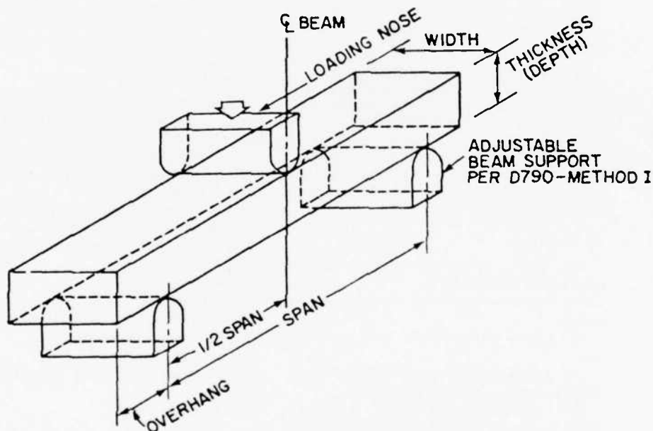
FIG. 1 Type B Specimen Geometry and Loading
