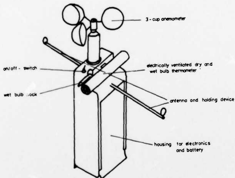
Fig. 1.8 Tethersonde package. Sensors and housing of the electronics and the battery.
