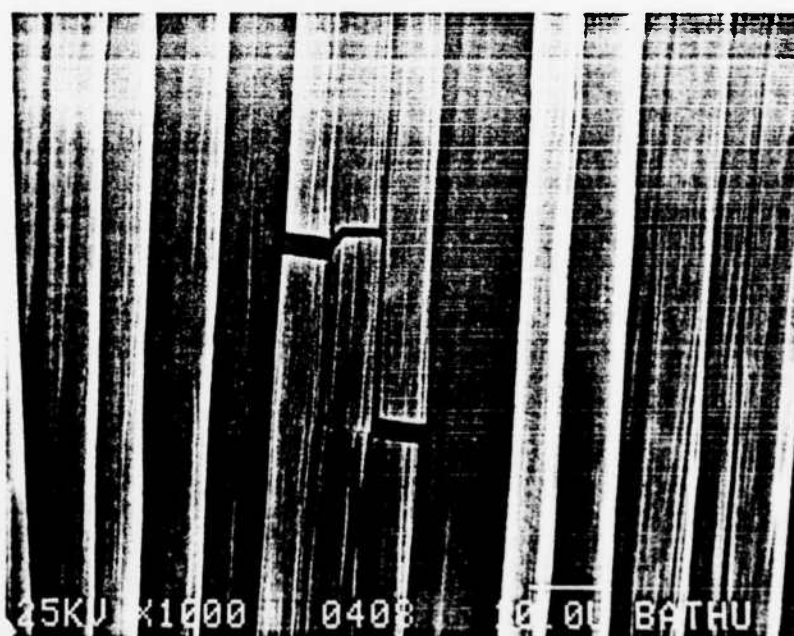
Fig. 25. Details of multiple fiber fractures in [0,0]_s laminates.
