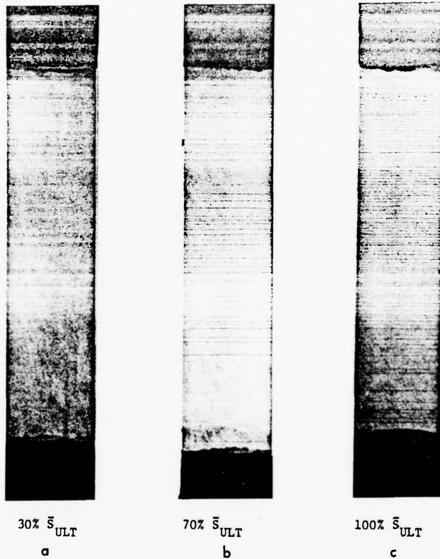
Fig. 2. X-ray radiographs of [0,90]_s laminates at tensile loads of (a) 30\% \bar{S}_{ult} , (b) 70\% \bar{S}_{ult} and (c) 100\% \bar{S}_{ult} .
